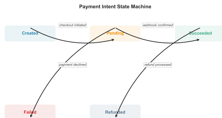
Figure 4.11: Payment Intent State Machine
