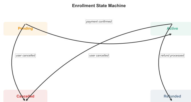
Figure 4.12: Enrollment State Machine
