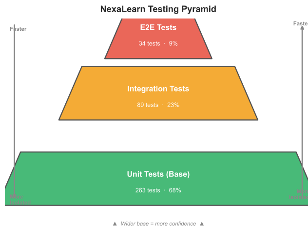
Figure 5.1: NexaLearn Testing Pyramid: unit tests form the base (263 tests), integration tests occupy the middle layer (89 tests), and E2E tests sit at the apex (34 tests).
