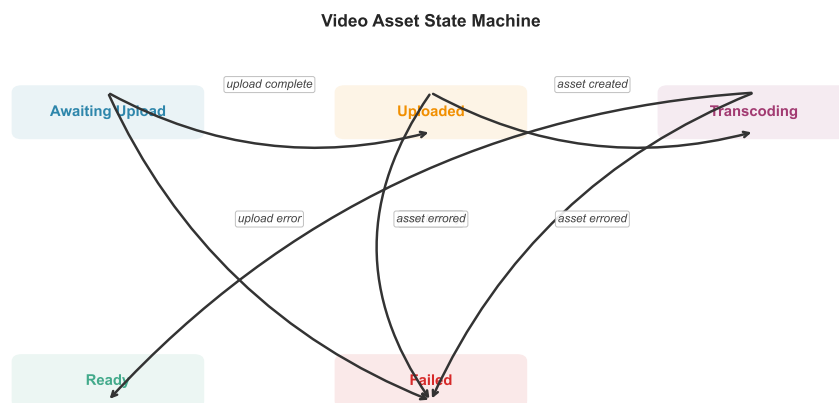
Figure 4.6: Video Asset State Machine
