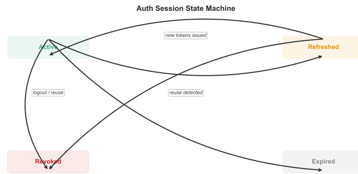
Figure 4.4: Auth Session State Machine
