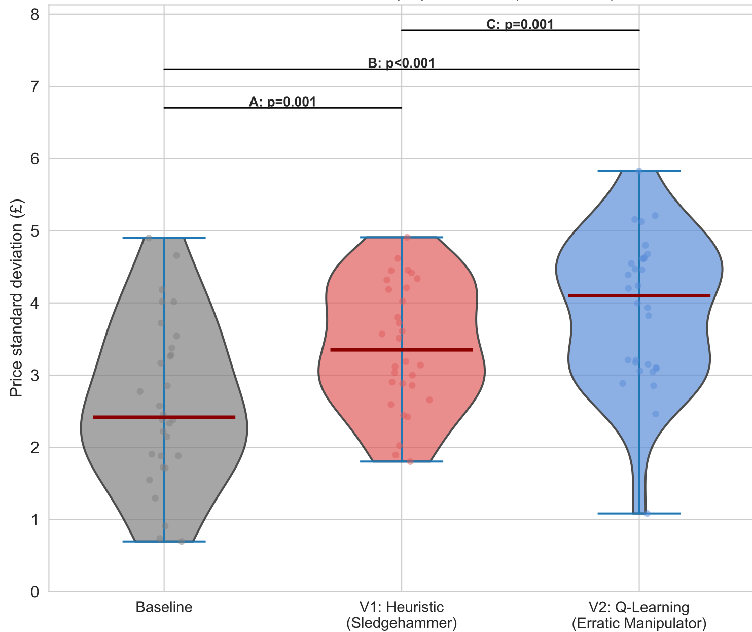
Intra-Session Price Volatility by Condition (n=30 seeds)
