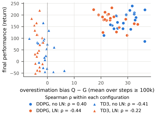
(b) Bias vs performance pooled \rho = 0.57 (Bonferroni p < 0.001 )
