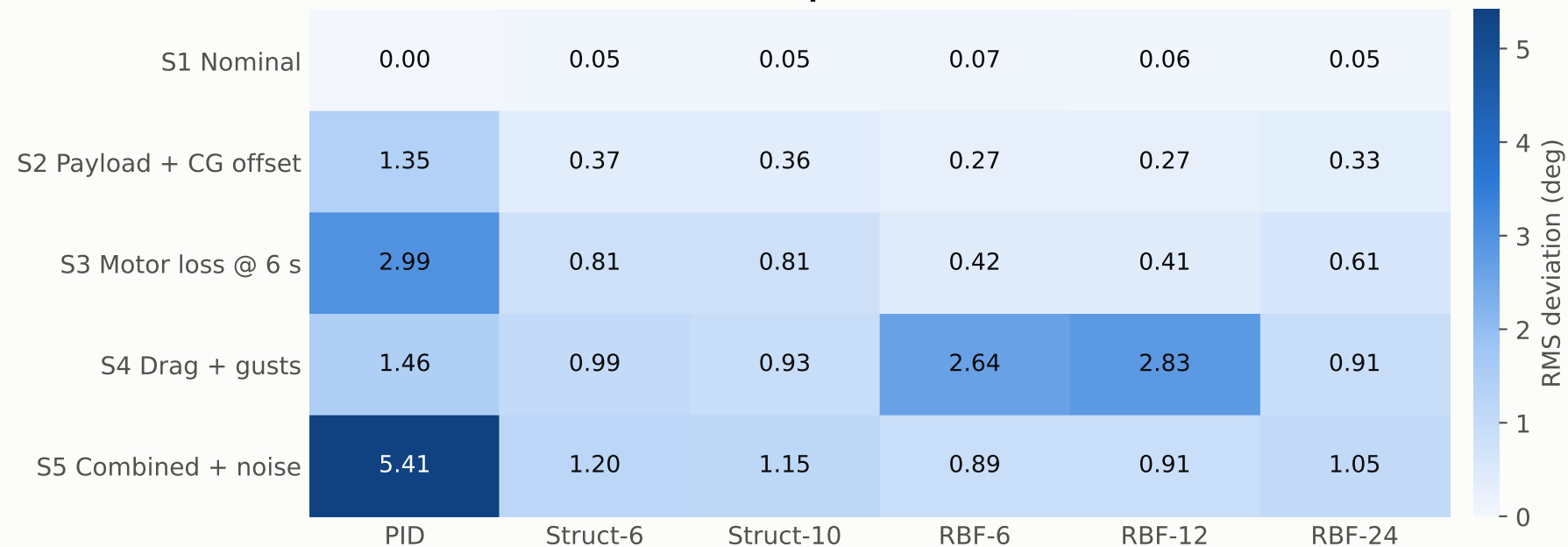
RMS roll deviation from nominal per scenario (lower is better)
