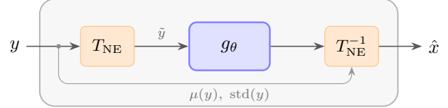
Figure 1. Normalization-equivariant wrapper (WNE). Given a noisy input y , we compute instance statistics \mu(y) and \text{std}(y) , normalize to \tilde{y} = T_{NE}(y) , apply an arbitrary backbone g_\theta , and denormalize with the stored statistics to produce \hat{x} = \text{std}(y) g_\theta(\tilde{y}) + \mu(y)\mathbf{1} . This enforces input-output normalization equivariance without modifying the backbone.
