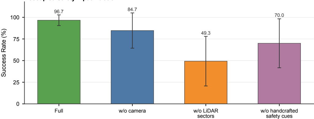
Decoupled Safety-Input Ablation
