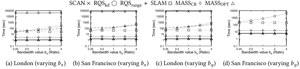
Figure 3: Response times for computing the product KDV with the uniform kernel function on the London and San Francisco datasets, varying the bandwidth parameters: b_x for (a,b) and b_y for (c,d).
