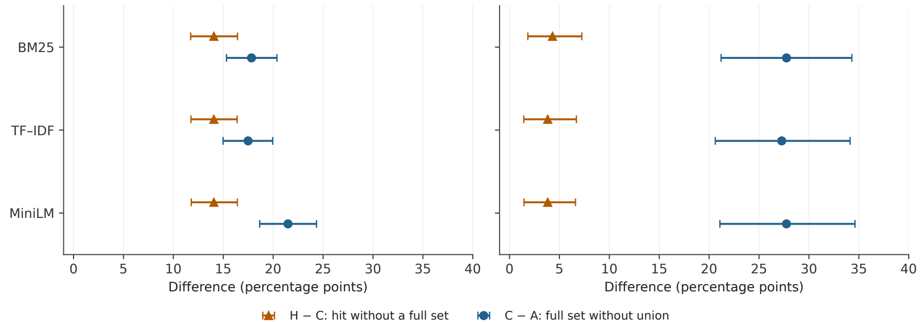
QASPER · k = 5
