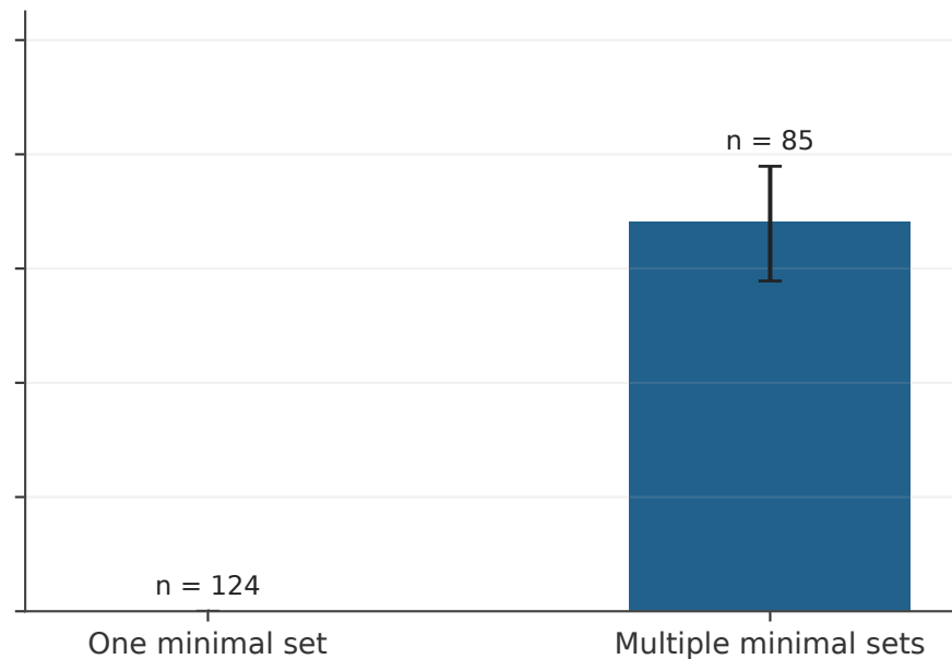
SciFact
