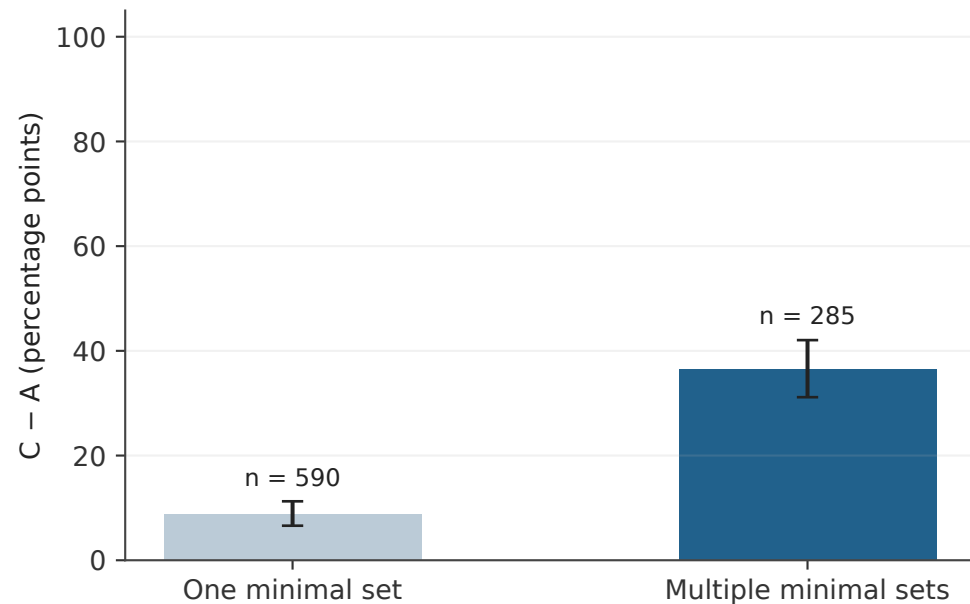
QASPER
