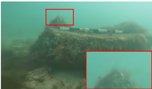
Water-Splatting
