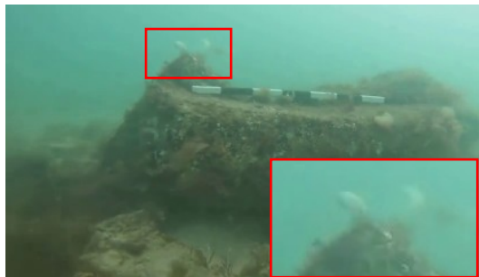
Groundtruth
