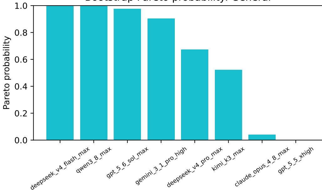
Bootstrap Pareto probability: General
