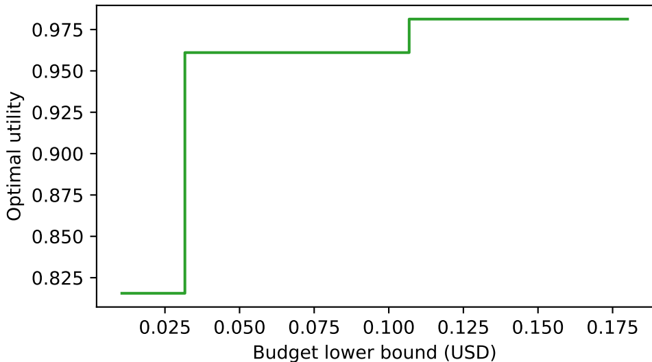
Budget-constrained choice: Coding
