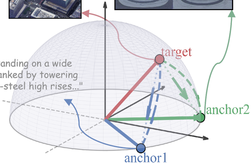
Pairwise Cosine → Conflicting Pulls
