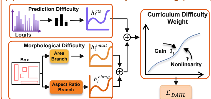
(c) Defect-aware Hard-example Learning (DAHL)
