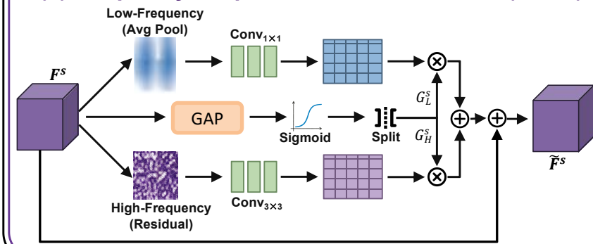
(b) Frequency-adaptive Feature Modulation (FAFM)
