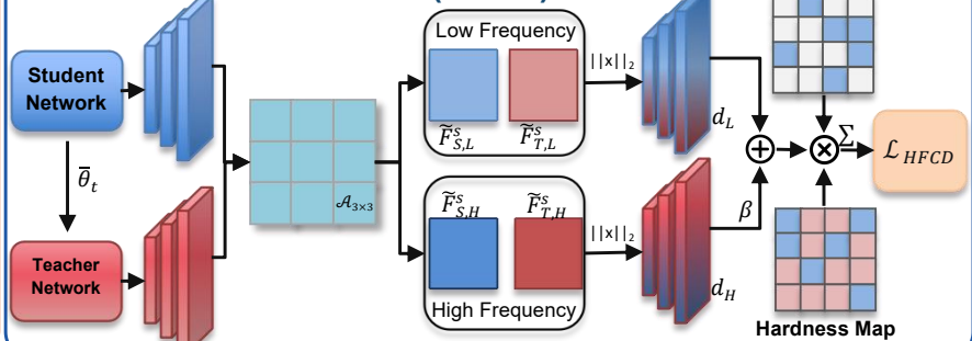
(d) Hardness-guided Frequency Consistency Distillation (HFCD)
