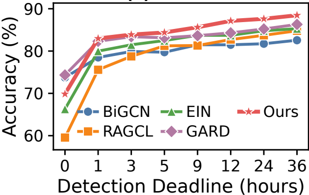
(a) DRWeibo
