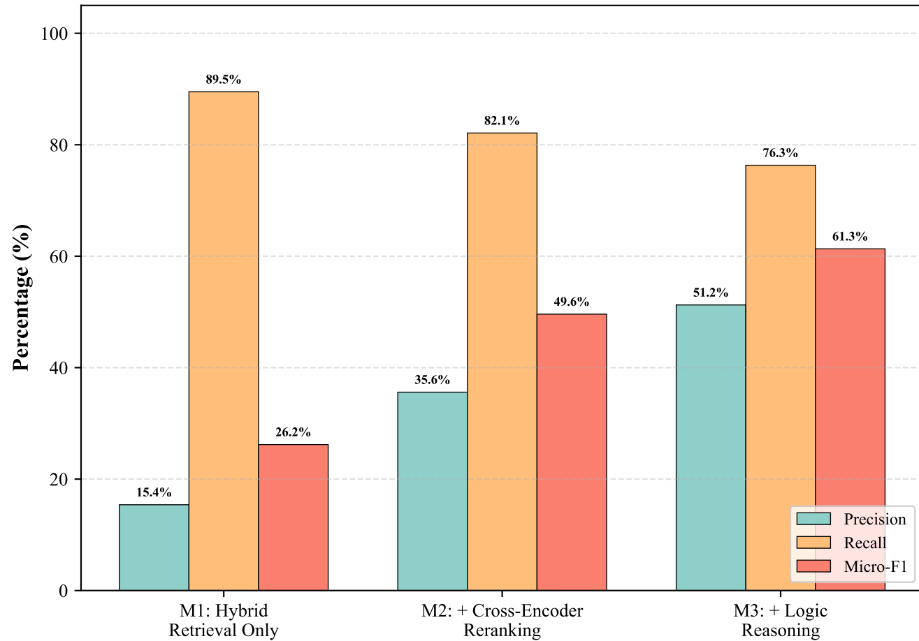
(b) Incremental Ablation Study
