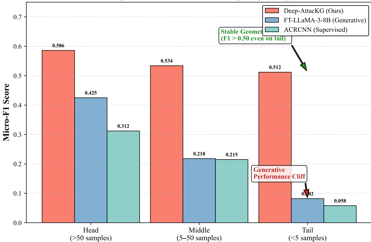
Long-Tail Robustness Across Frequency Groups
