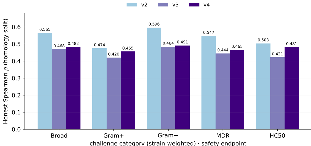
Figure 2: Version progression v2 \rightarrow v3 \rightarrow v4 , category-level honest ranking. Bars are category-level Spearman \rho on the honest (homology) split — strain-weighted per-species MIC via the panel aggregation of §7, plus the HC50 safety endpoint — coloured by version. Random-split numbers are omitted here (they are in Table 5). v2 is evaluated on its own pre-re-clustering split; v3 and v4 share the common, harder re-clustered honest test, so v4 vs v3 is the apples-to-apples comparison : v4 (data-clean MIC head + soft-rank HC50 head) improves every category over v3 , most on HC50 (+0.060) and the resistance-relevant Gram+/MDR. v2 ’s higher bars reflect its easier split, not a regression at v3 (see the † note).
