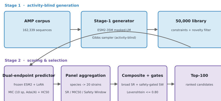
Figure 1: AMPGen submission pipeline. Stage 1 (activity-blind generation): the domain-adapted ESM2-35M masked-LM Gibbs sampler turns the AMP corpus into a constraint- and novelty-filtered 50,000-sequence library. Stage 2 (scoring & selection): the dual-endpoint predictor (frozen ESM2 + LoRA; 10-species AdaLN MIC head + HC50 head) scores each candidate; panel aggregation maps species predictions to the 20-strain challenge panel (Success Rate / MIC50 / Safety Window); a safety-gated composite plus the strict Levenshtein novelty gate yields the ranked top-100. The whole pipeline is one reproducible command, uv run generate .
