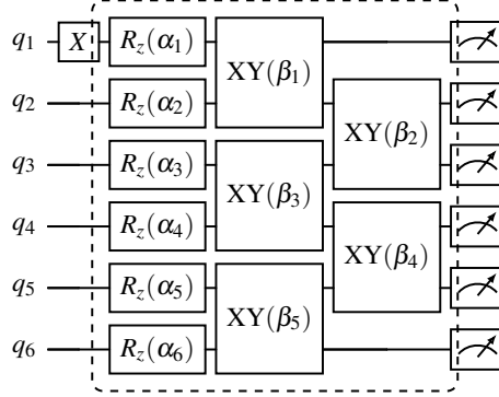
Figure 1: The propagation circuit at K = 6 ; production runs use K = 8\text{--}16 with identical structure. The dashed block is one Trotter step, repeated r times. State preparation is the single X gate, since |\psi_S\rangle is e_1 in the Krylov basis; each step applies the diagonal \alpha_r as parallel R_z rotations, then the off-diagonal \beta_r as two layers of XY(\beta) = \exp[-i\beta(XX + YY)/2] on odd and even bonds, each compiling to two CNOTs plus single-qubit rotations. Measurement is in the computational basis; shots outside Hamming weight one are discarded.
