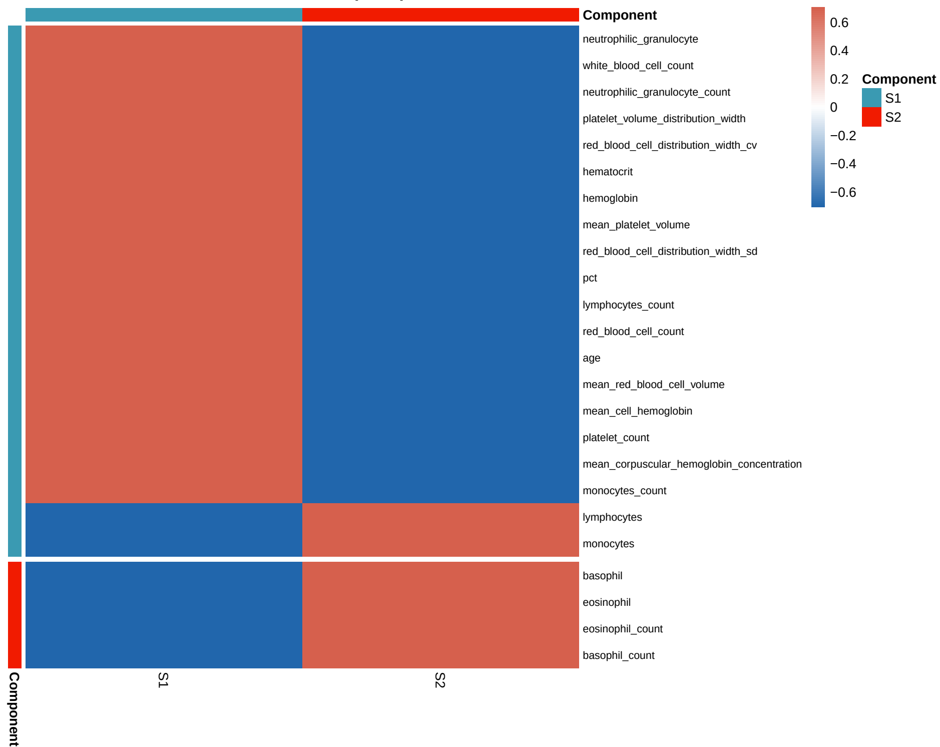
NMF Basis Matrix (K = 2)
