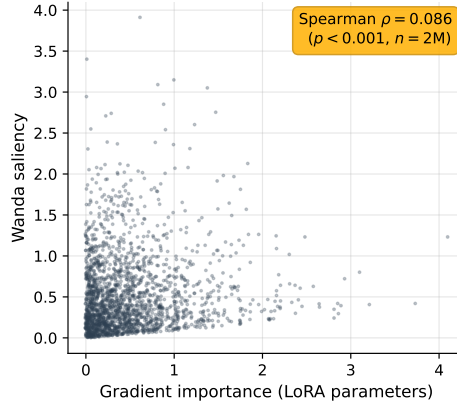
Figure 5: Spearman \rho = 0.086 between Wanda and gradient importance (LoRA parameters) on Qwen2.5-3B. These metrics rank parameters nearly independently.
