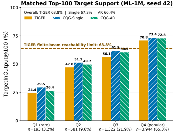
Figure 2: Maximum-list-size-matched target support on ML-1M (seed 42), stratified by held-out target popularity. Bars show user-weighted TargetInOutput@100 with at most 100 returned items: TIGER uses beam width 100, while CQG-Single and CQG-AR use dense Top-100 retrieval. The dashed line marks TIGER’s overall finite-beam support of 63.8%. All analyses use the same 6,040 users and popularity-quartile mapping as Figure 3 and Table 11.
