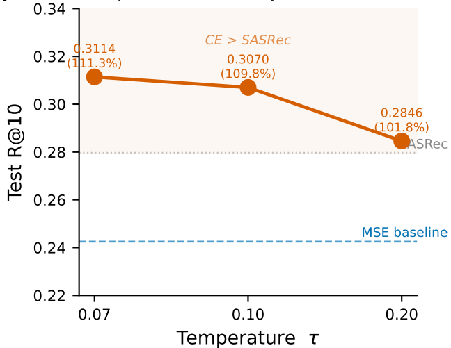
(b) Temperature sensitivity (CE > MSE at all \tau )
