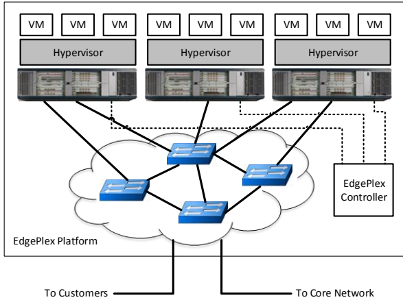
Figure 1: Architecture of EdgePlex platform.
