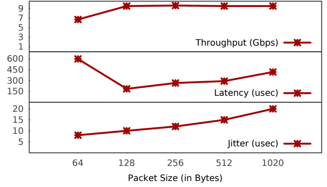
Figure 4: Throughput, Latency and Jitter for various packet sizes with 16 PVMs.
