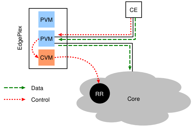
Figure 2: Split of control- and data-plane functions in EdgePlex.
