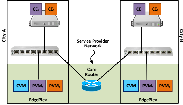
Figure 3: Testbed setup of a prototype implementation of EdgePlex.
