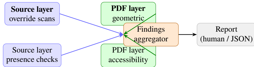
Figure 2-1. High-level architecture of the two-layer validator. The source layer (blue) and the PDF layer (green) feed into a findings aggregator (orange), which produces a grouped report (gray).
