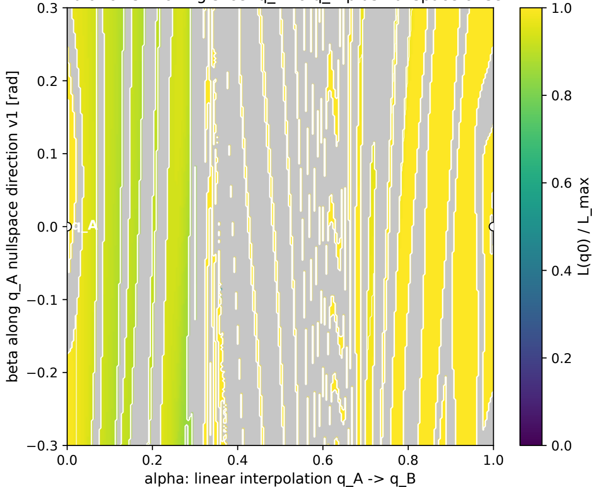
IK branch switching slice: q_A to q_B plus nullspace offset
