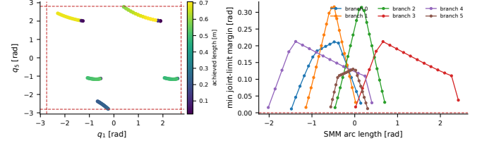
Fig. 4. Self-motion manifold branches for a fixed end-effector pose.
