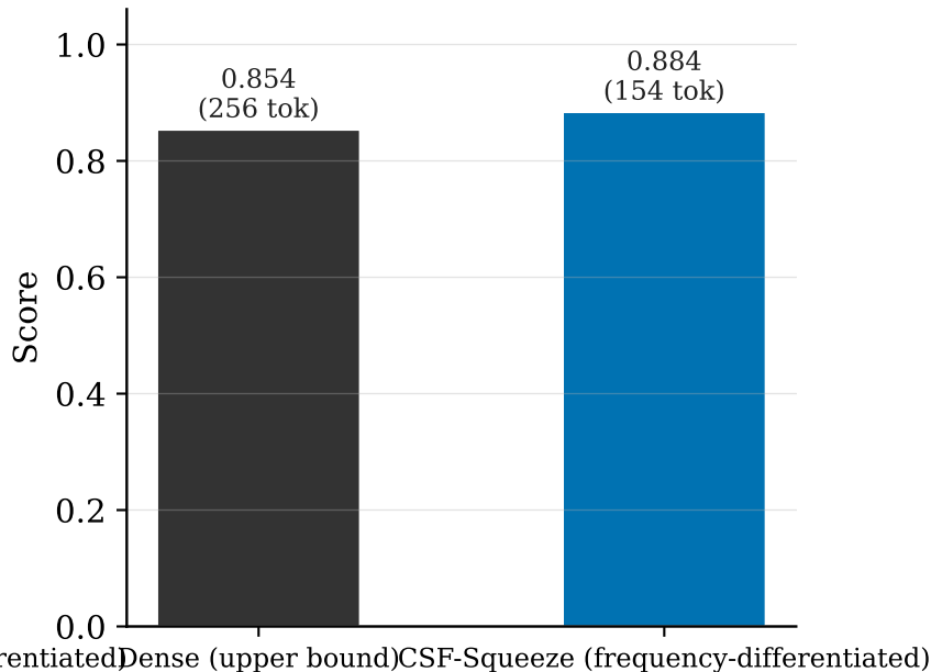
POPE (hallucination, accuracy)
