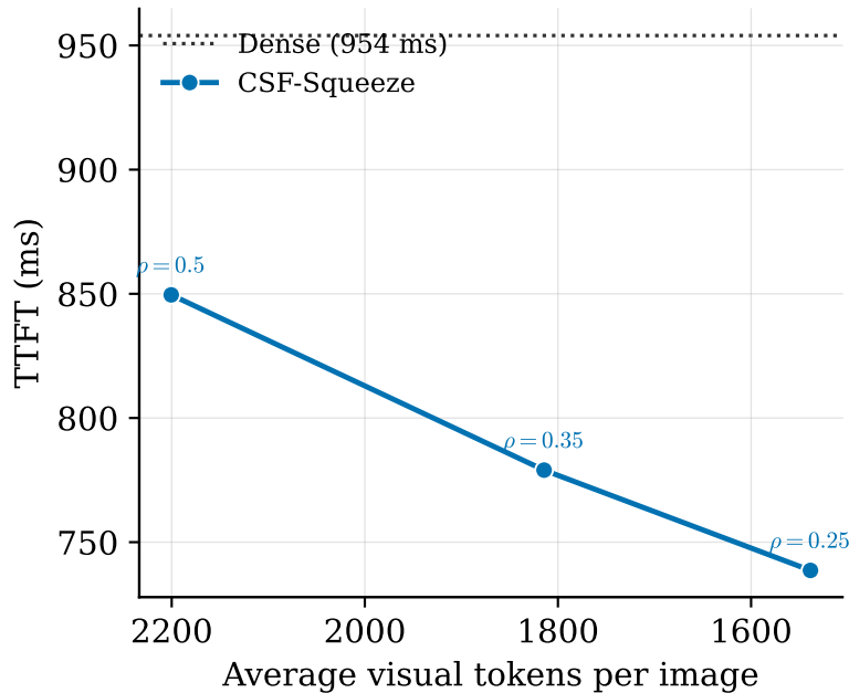
Time-to-first-token vs. compression
