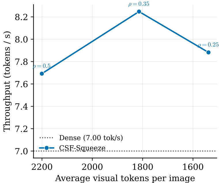
Decoding throughput vs. compression
