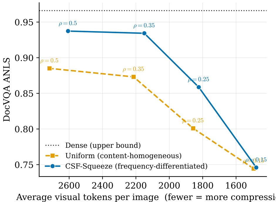
Accuracy vs. compression on DocVQA (Qwen3-VL-4B)
