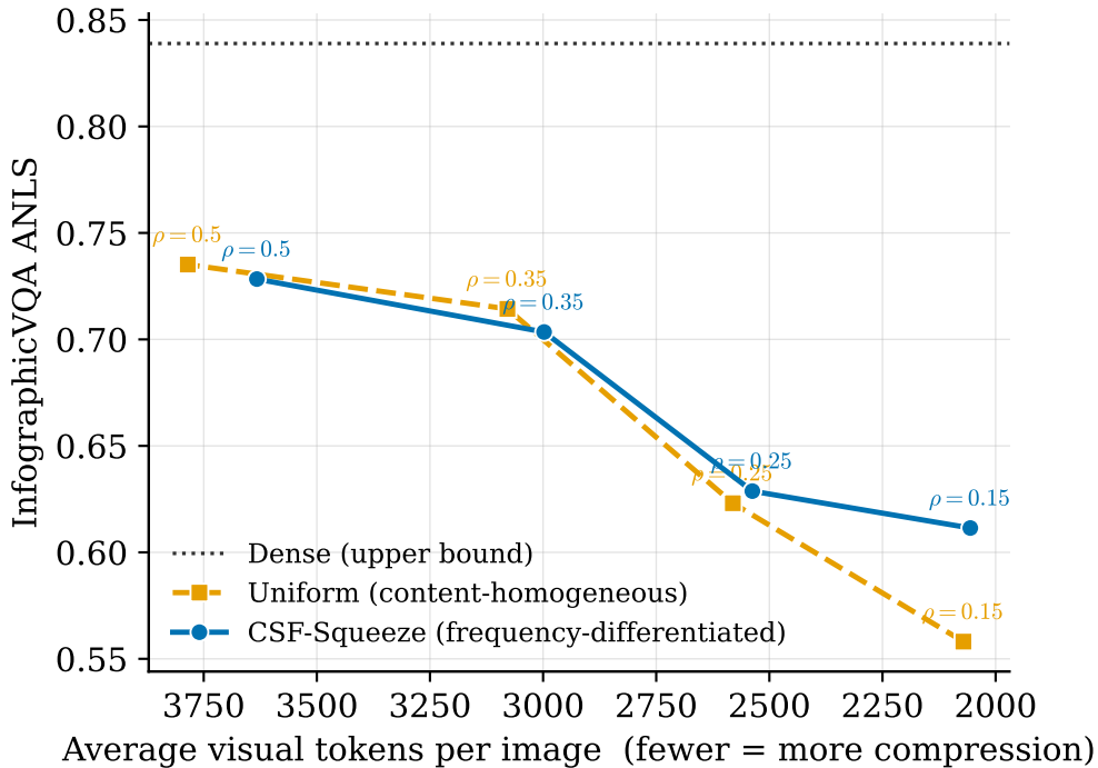
Accuracy vs. compression on InfographicVQA (Qwen3-VL-4B)
