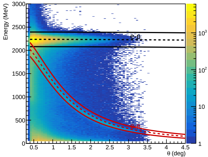
X17 2.2 GeV Calib. Run Reconstructed Energy vs. Angle
