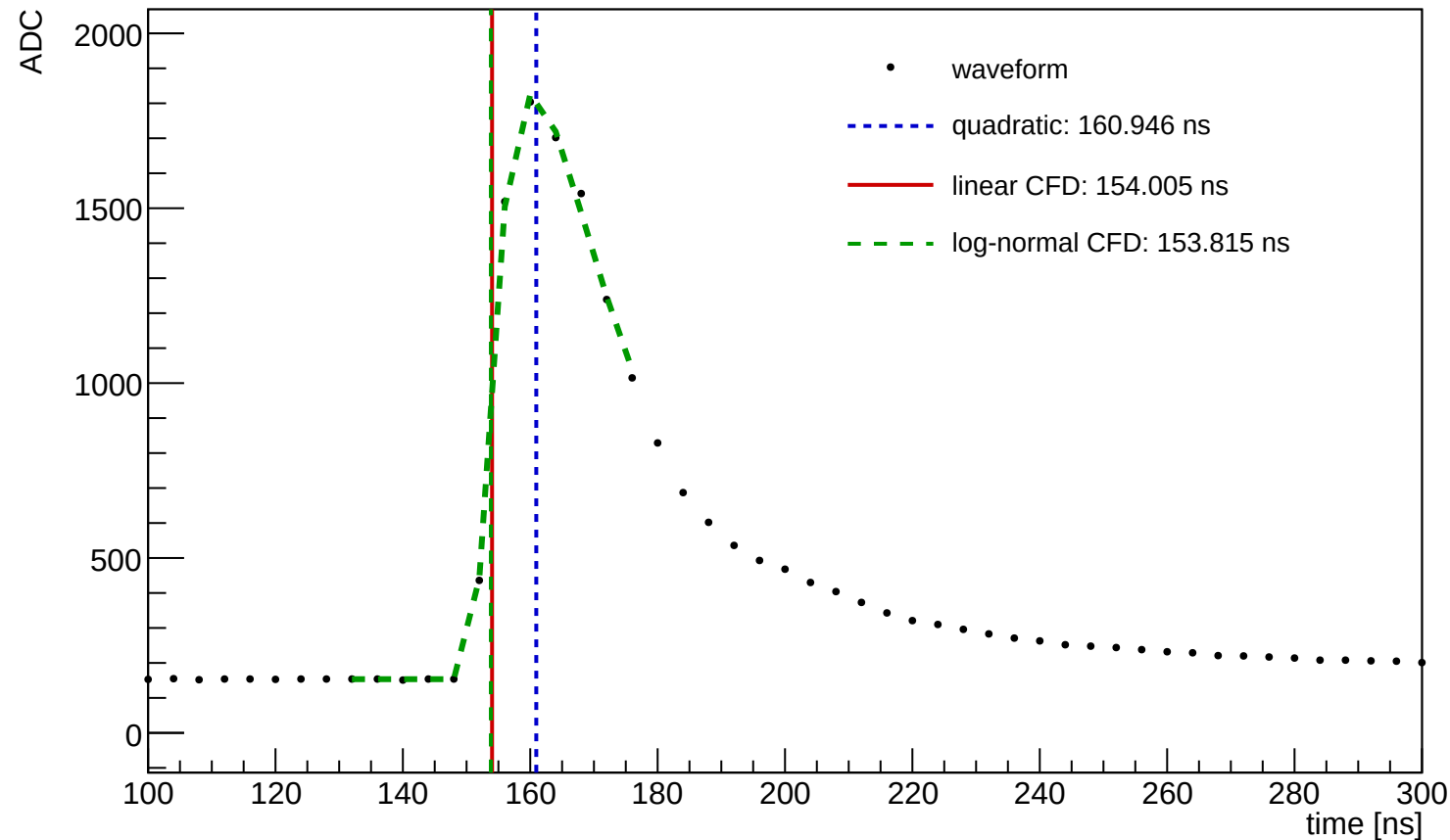
Waveform Time Demo (entry=18811, ch=8, module=1043, trigger=SUM)
