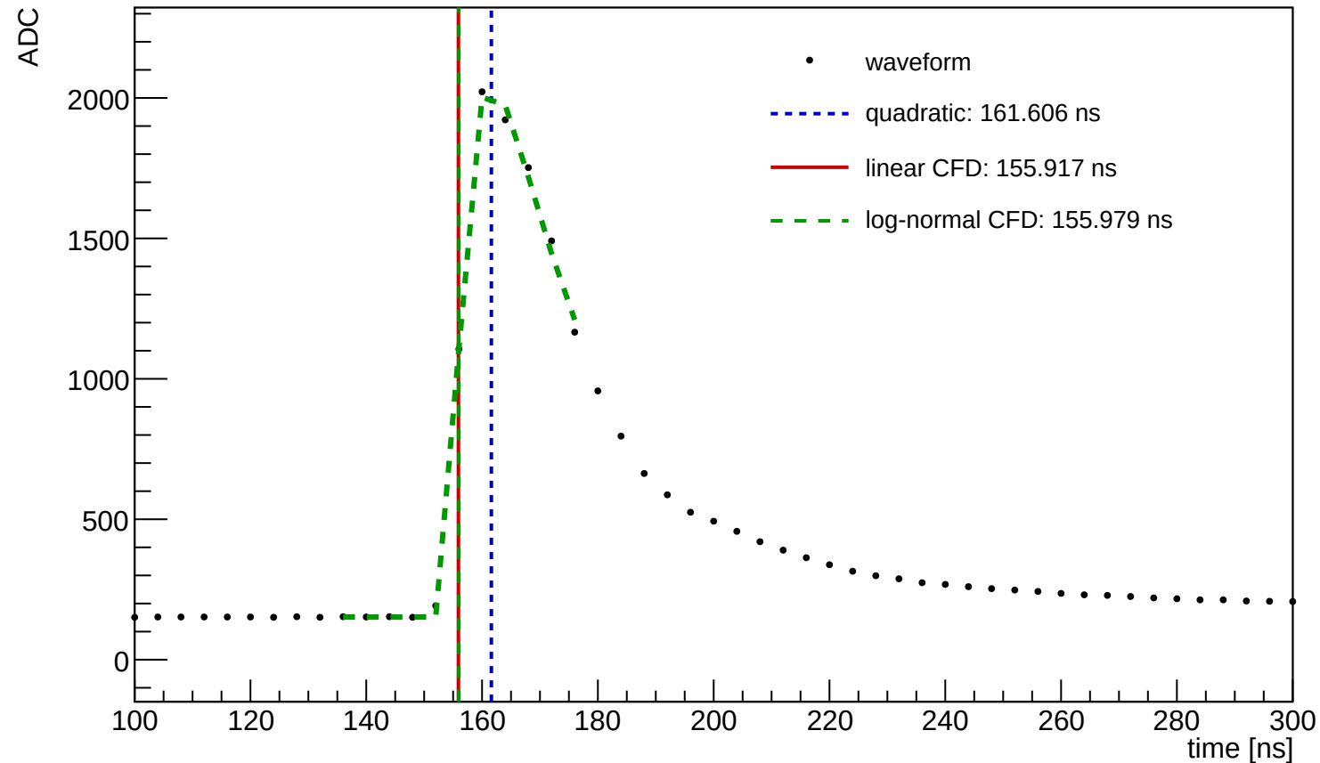
Waveform Time Demo (entry=60936, ch=6, module=1119, trigger=SUM)
