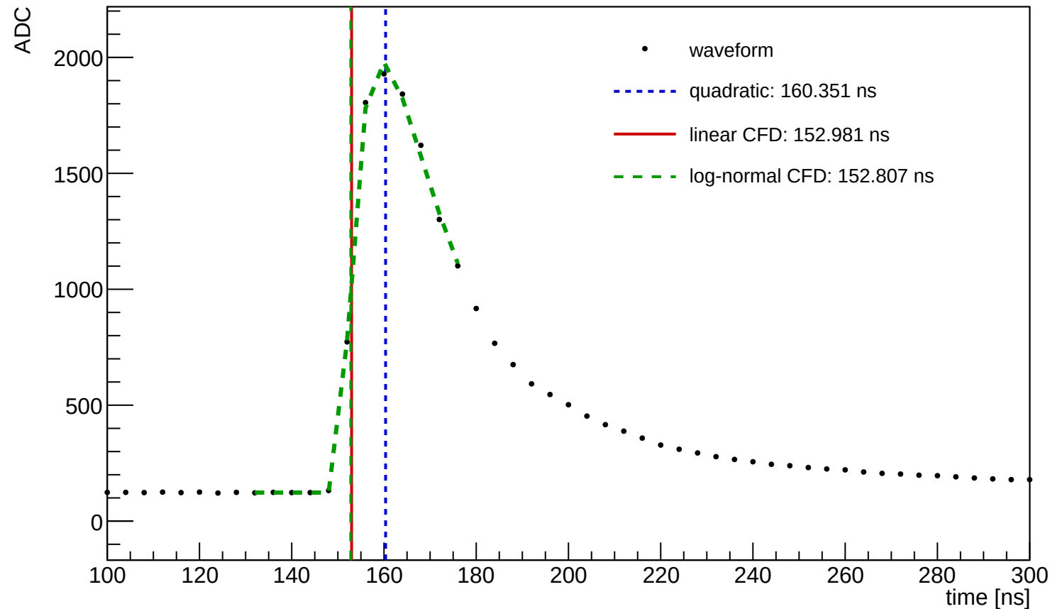
Waveform Time Demo (entry=32924, ch=6, module=1013, trigger=SUM)
