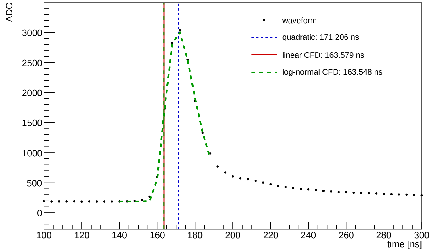
Waveform Time Demo (entry=16657, ch=1, module=1001, trigger=SUM)
