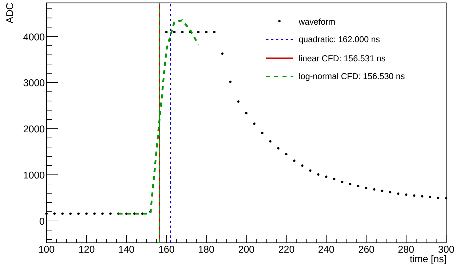
Waveform Time Demo (entry=67764, ch=1, module=1109, trigger=SUM)
