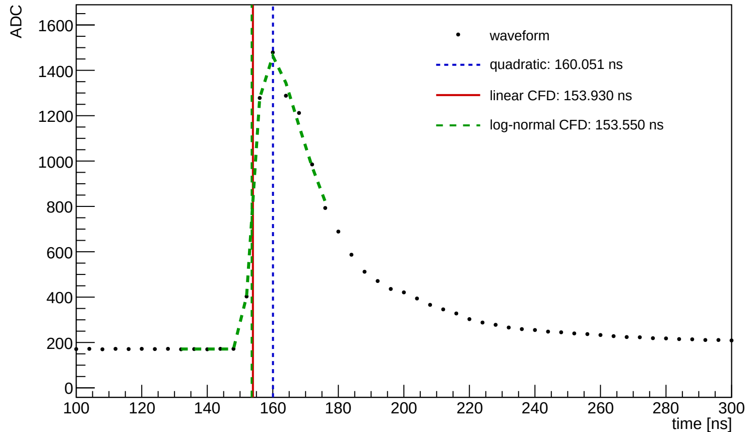
Waveform Time Demo (entry=37918, ch=1, module=1116, trigger=SUM)
