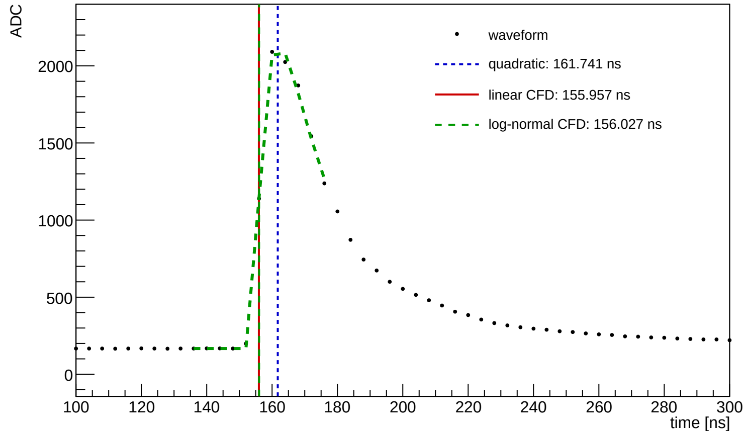
Waveform Time Demo (entry=54467, ch=9, module=1051, trigger=SUM)
