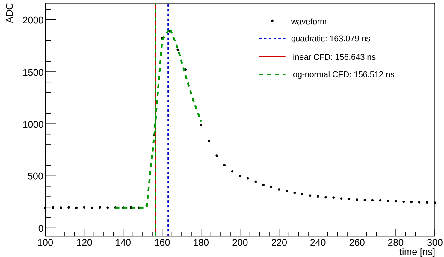
Waveform Time Demo (entry=7529, ch=5, module=1150, trigger=SUM)
