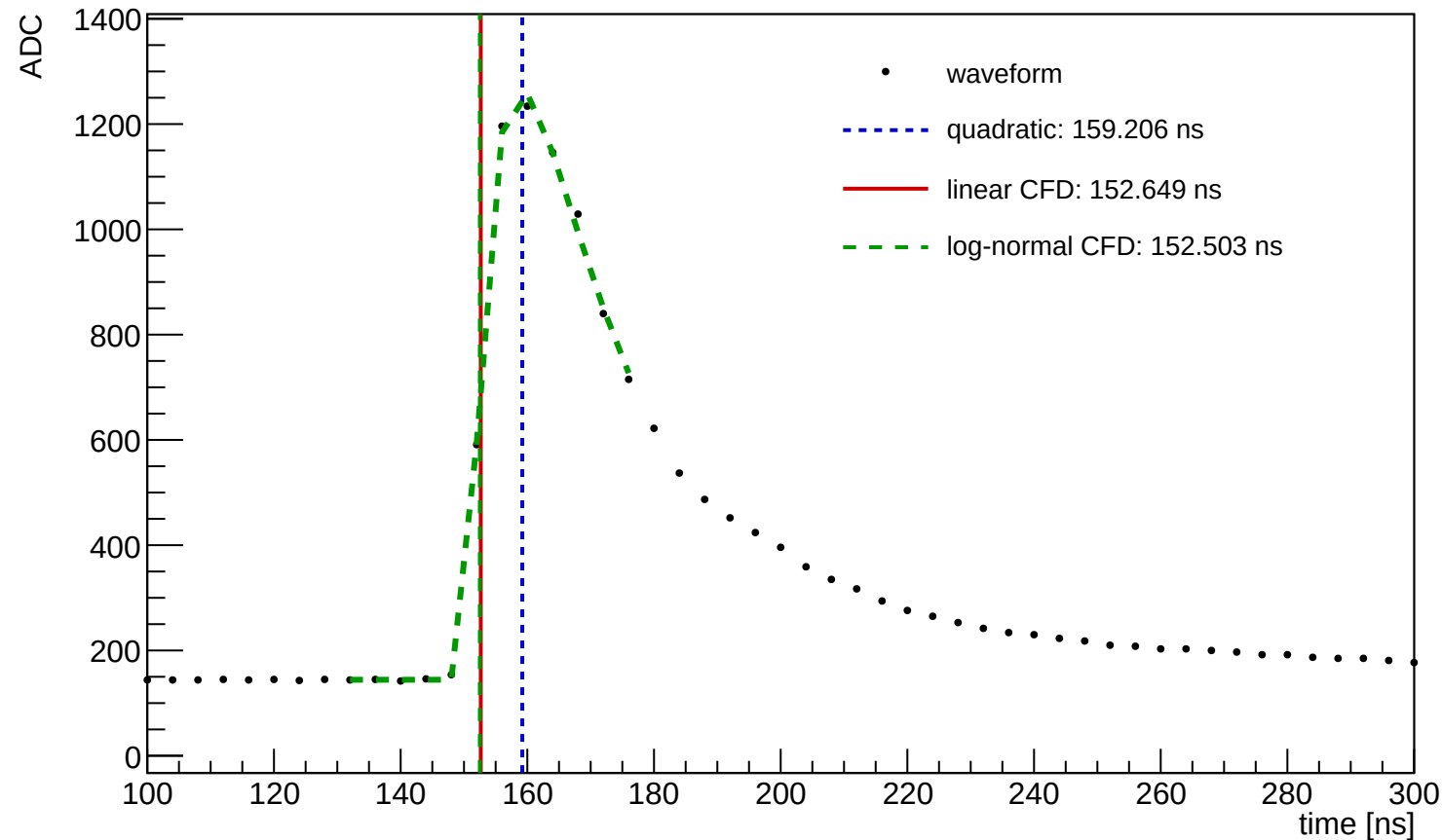
Waveform Time Demo (entry=37840, ch=3, module=1125, trigger=SUM)
