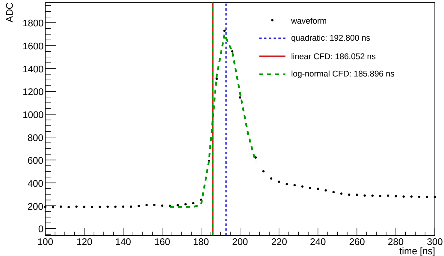
Waveform Time Demo (entry=48541, ch=1, module=1001, trigger=SUM)
