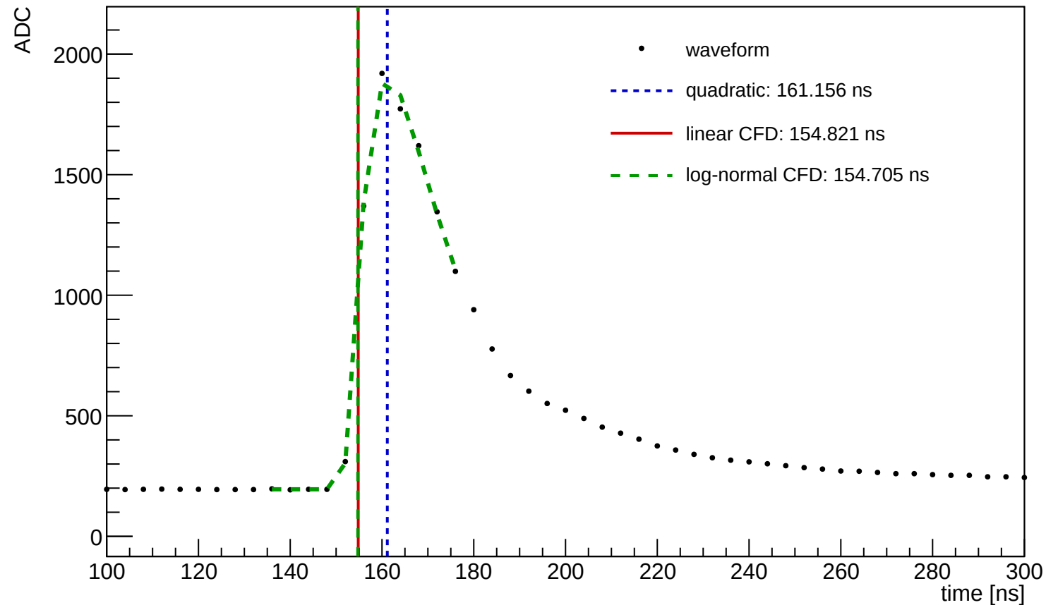
Waveform Time Demo (entry=49805, ch=7, module=1149, trigger=SUM)
