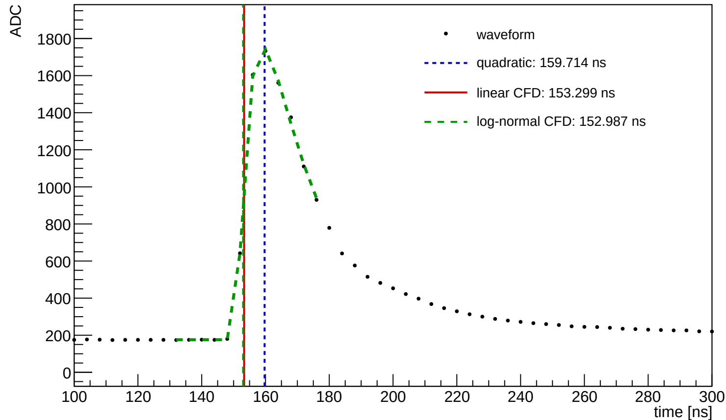
Waveform Time Demo (entry=12537, ch=3, module=1142, trigger=SUM)
