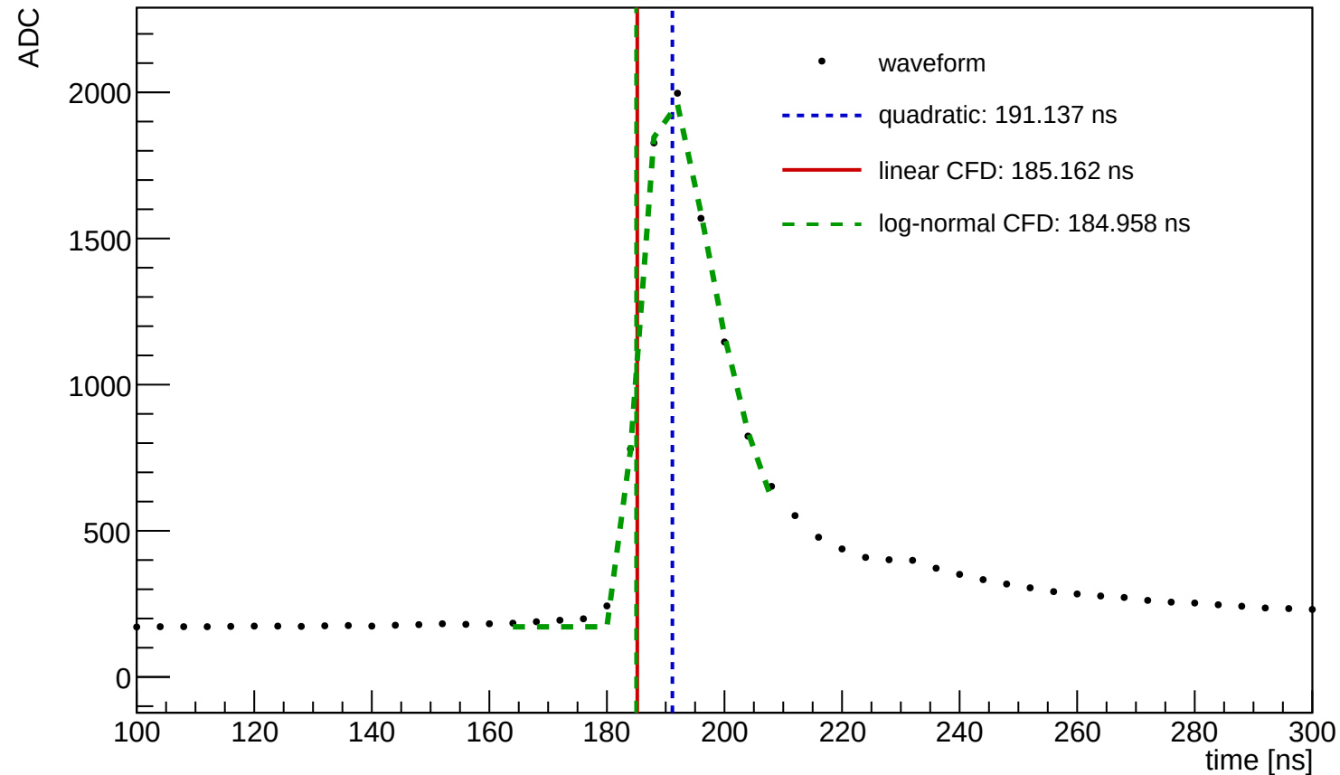
Waveform Time Demo (entry=59230, ch=1, module=1096, trigger=SUM)
