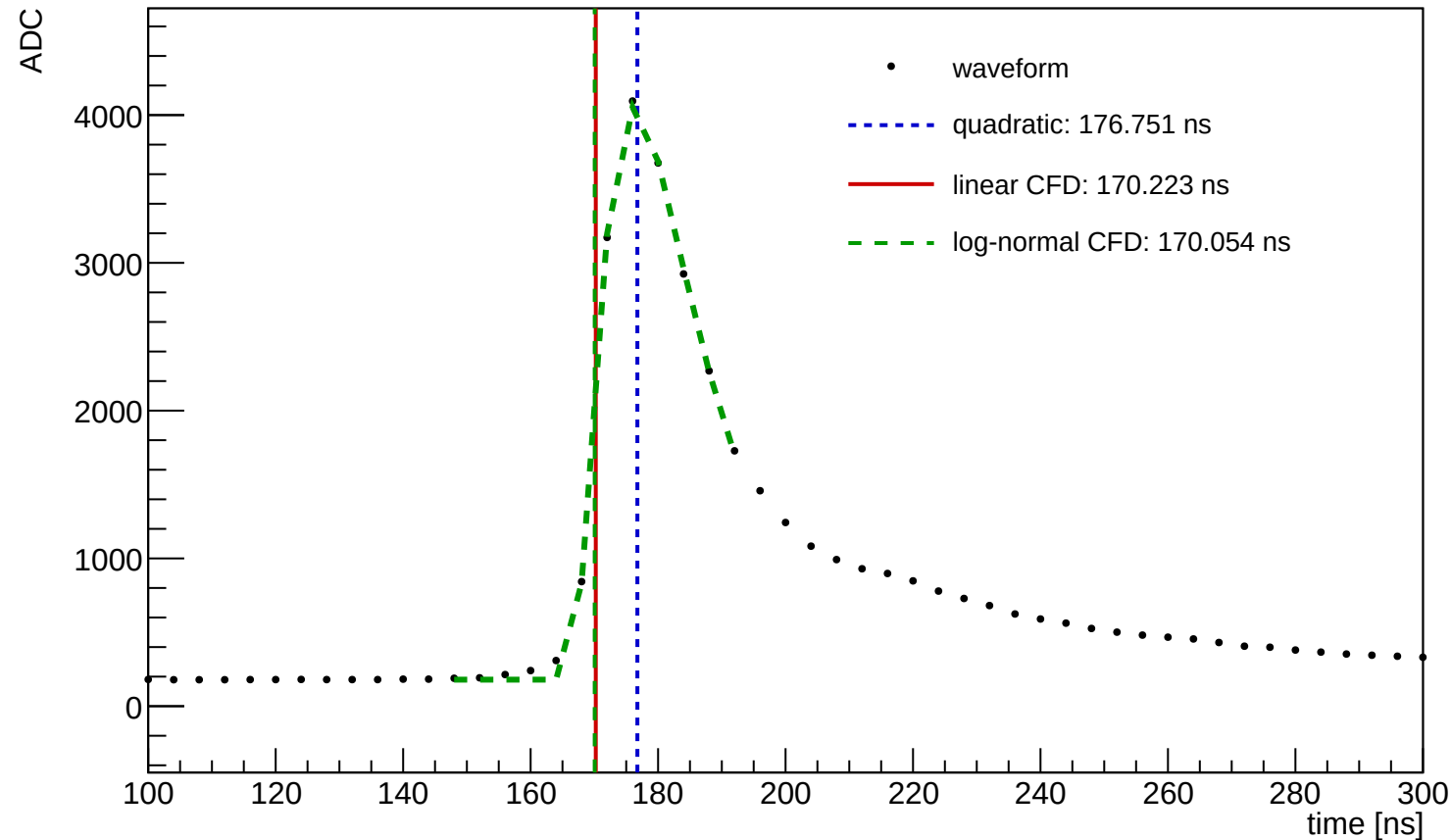
Waveform Time Demo (entry=37714, ch=1, module=1127, trigger=SUM)
