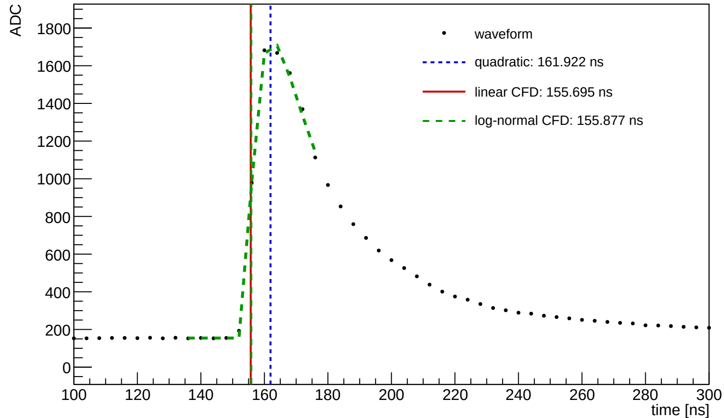
Waveform Time Demo (entry=20974, ch=7, module=1022, trigger=SUM)
