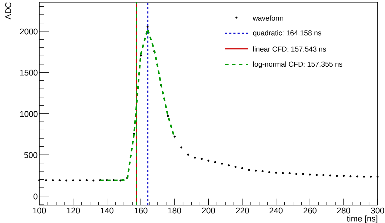
Waveform Time Demo (entry=41064, ch=1, module=1001, trigger=SUM)
