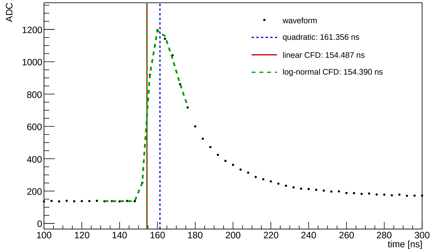
Waveform Time Demo (entry=4774, ch=7, module=1054, trigger=SUM)
