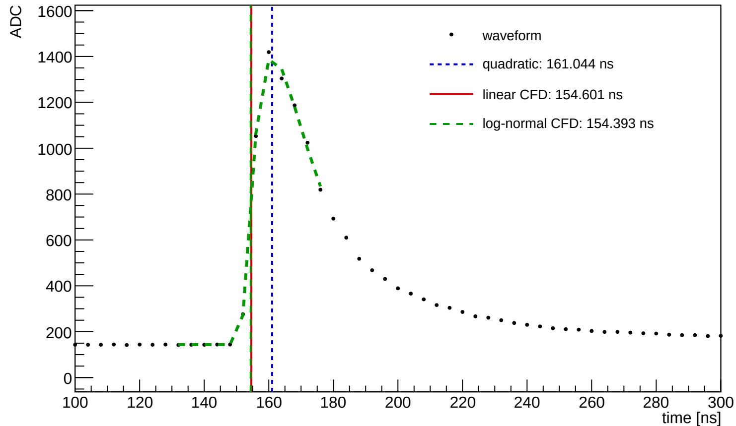
Waveform Time Demo (entry=9112, ch=11, module=1122, trigger=SUM)
