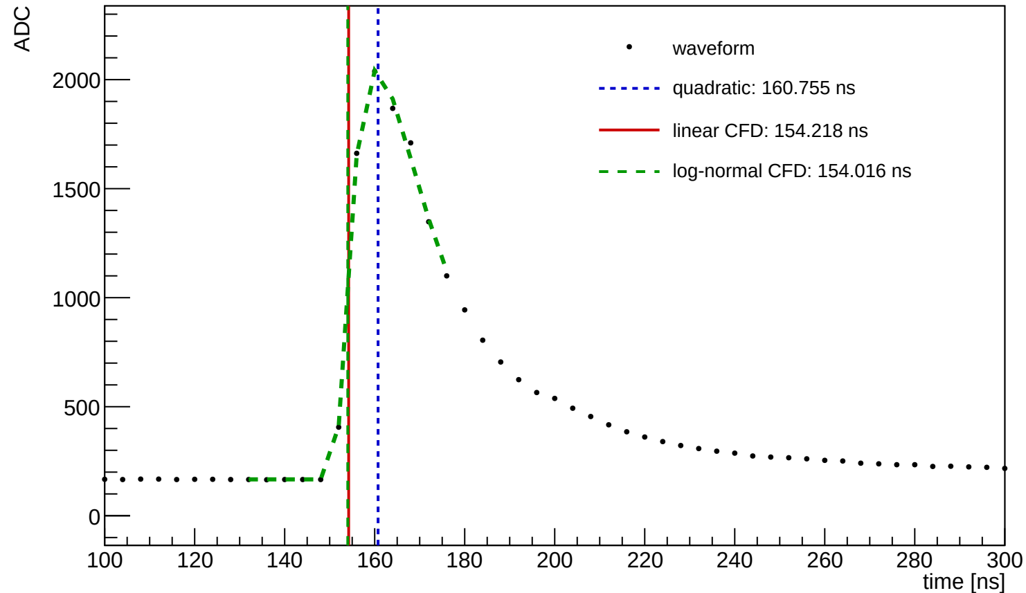
Waveform Time Demo (entry=65785, ch=7, module=1051, trigger=SUM)
