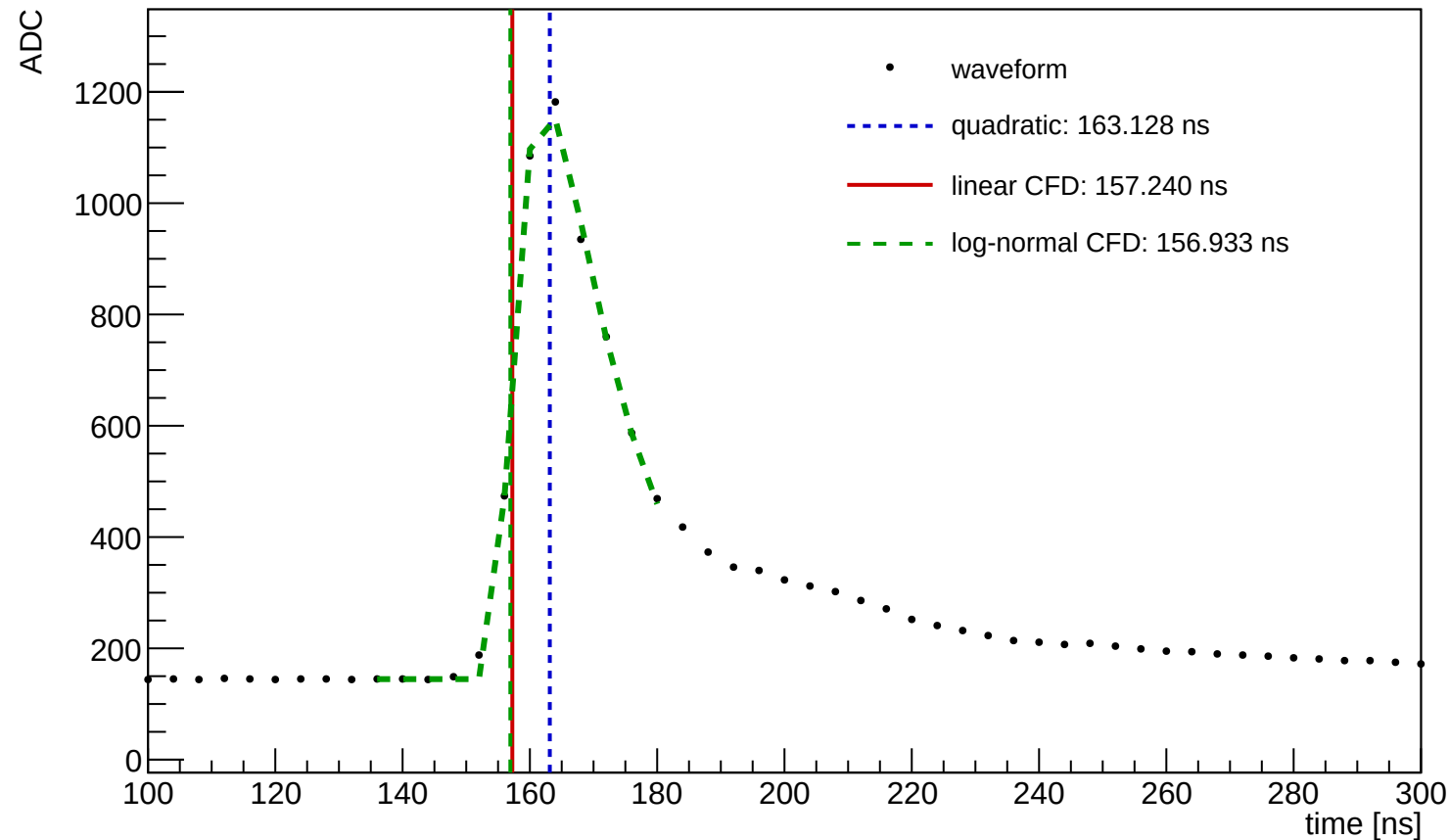
Waveform Time Demo (entry=53284, ch=3, module=1125, trigger=SUM)
