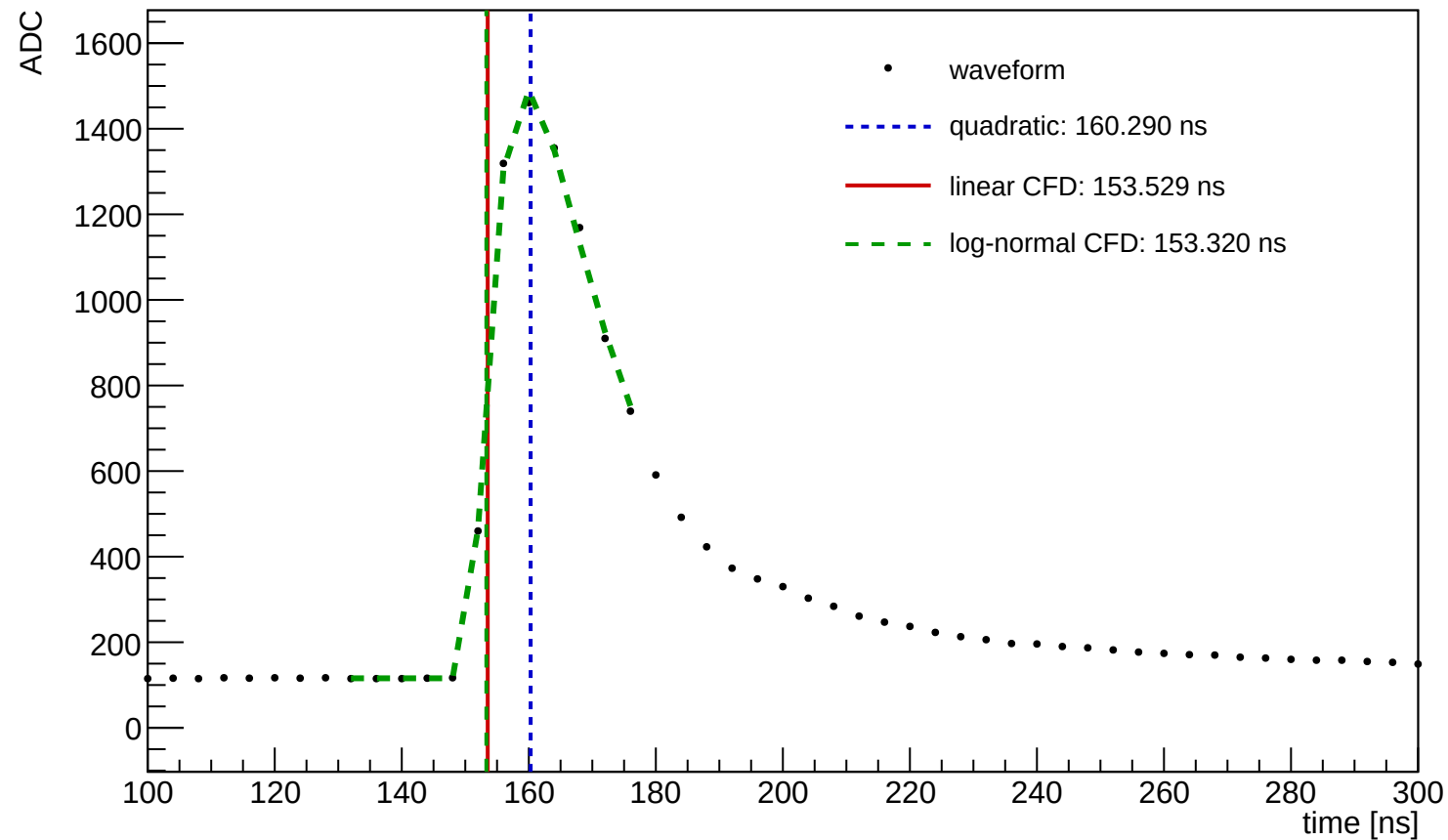
Waveform Time Demo (entry=67886, ch=10, module=1080, trigger=SUM)
