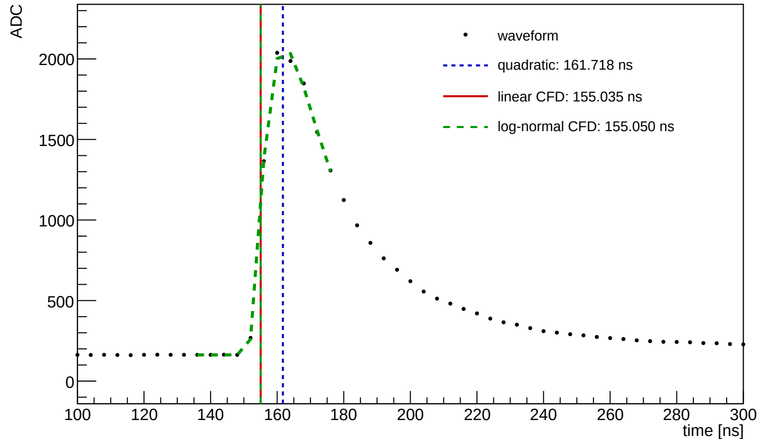
Waveform Time Demo (entry=21678, ch=5, module=1128, trigger=SUM)
