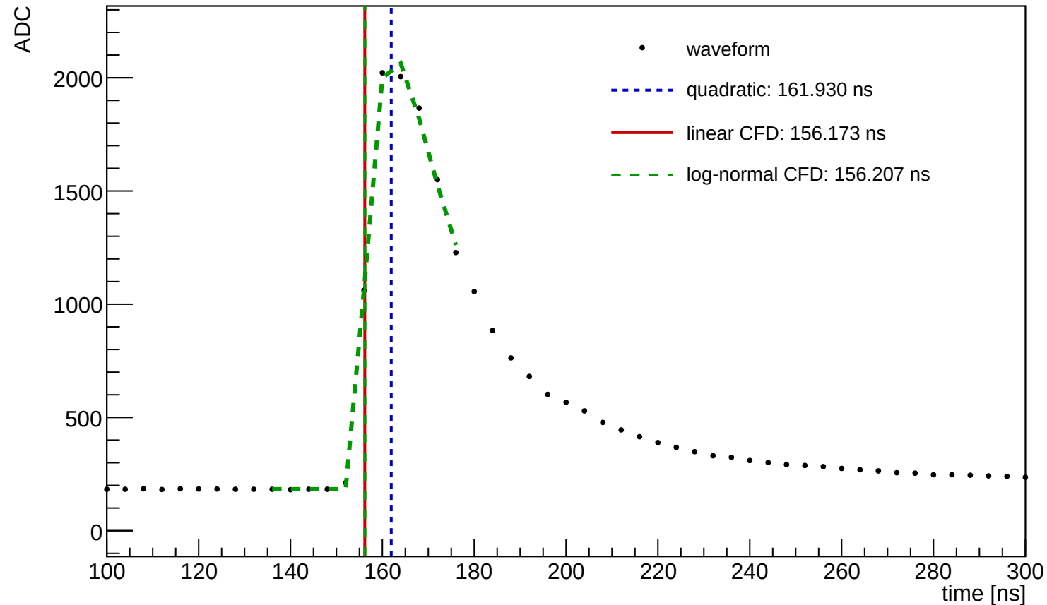
Waveform Time Demo (entry=14844, ch=19, module=1095, trigger=SUM)
