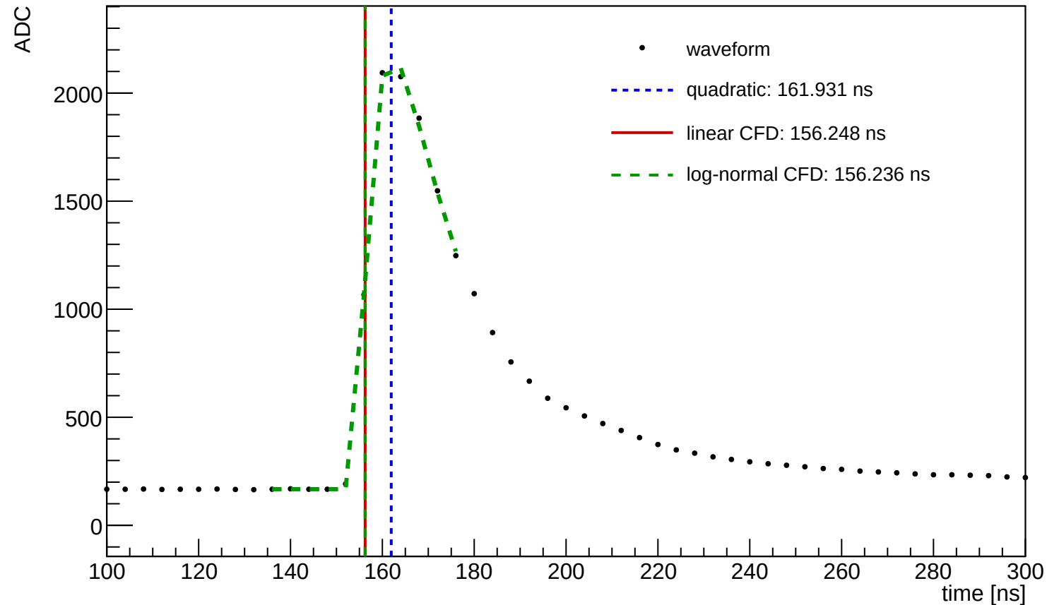
Waveform Time Demo (entry=16428, ch=7, module=1051, trigger=SUM)
