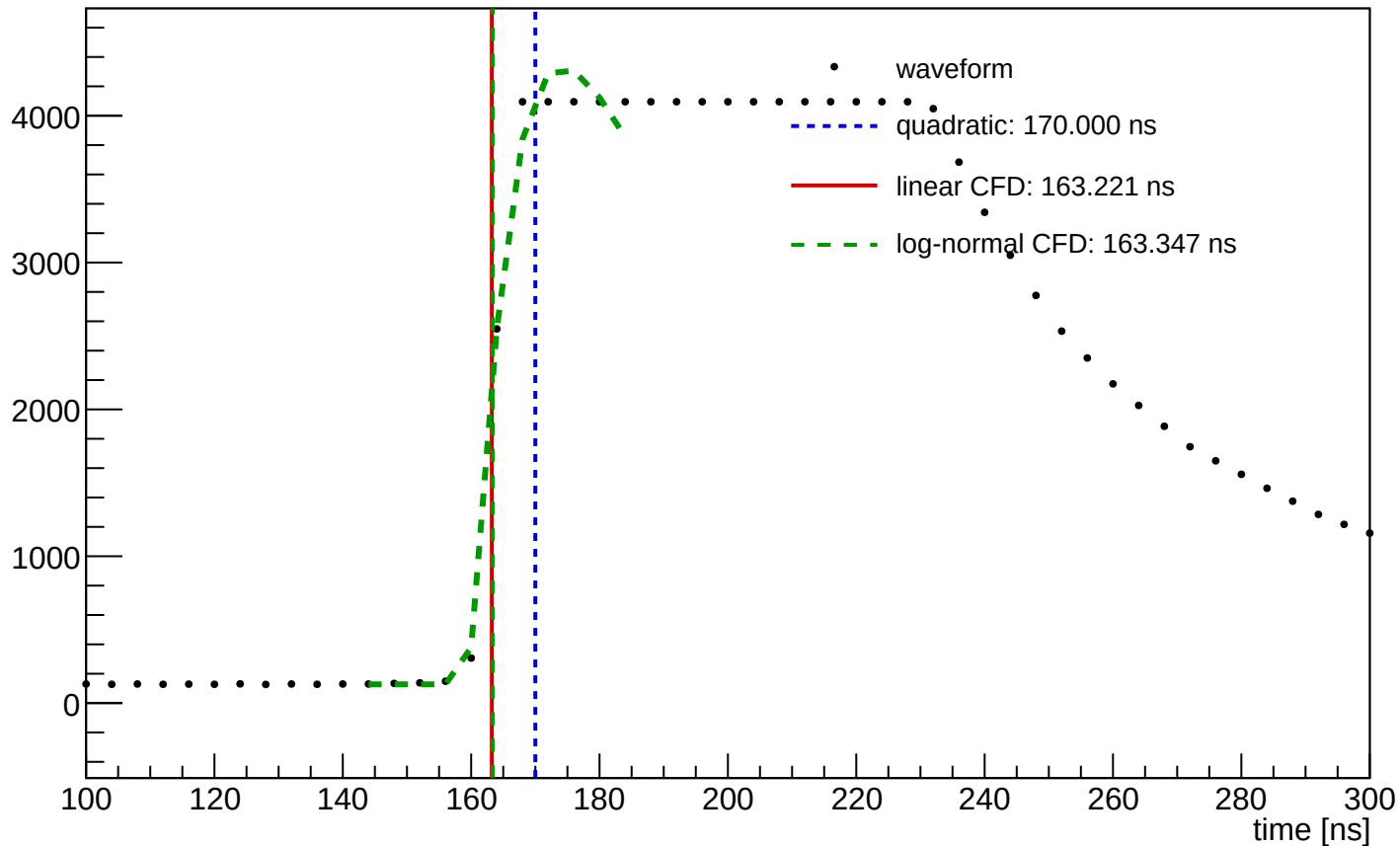
Waveform Time Demo (entry=7883, ch=0, module=1081, trigger=SUM)
