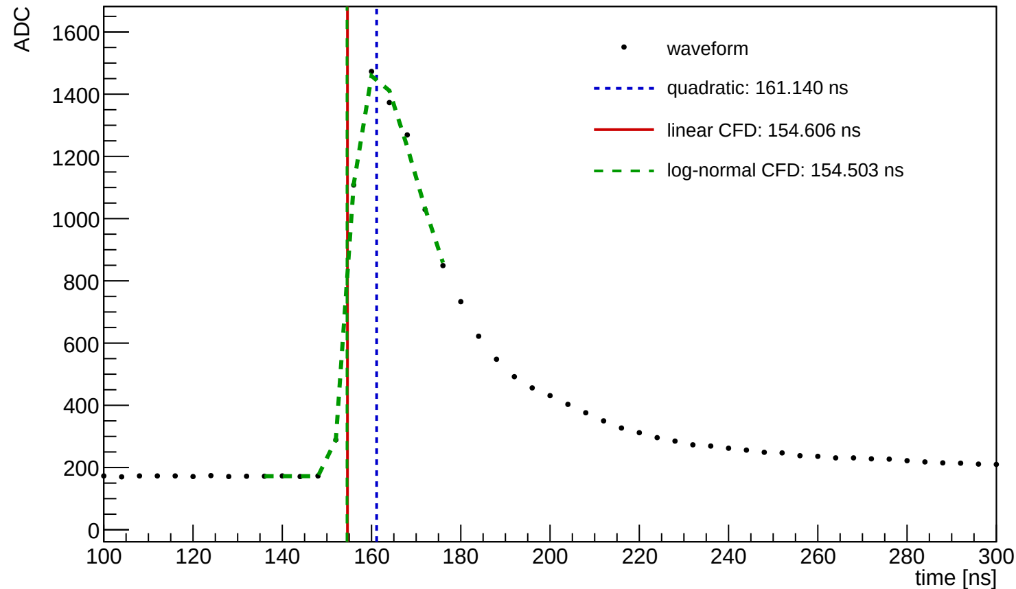
Waveform Time Demo (entry=72102, ch=9, module=1077, trigger=SUM)
