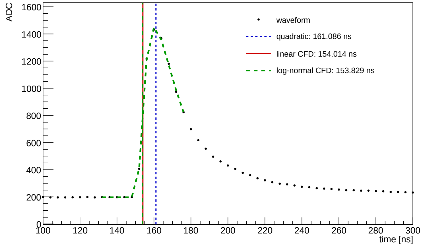
Waveform Time Demo (entry=51494, ch=8, module=1062, trigger=SUM)
