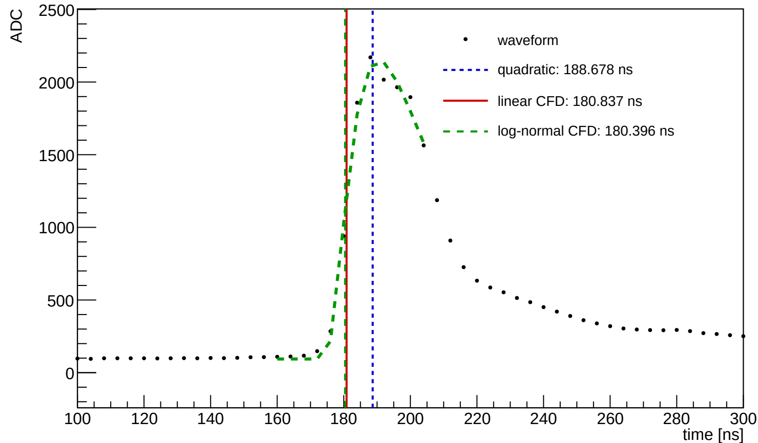
Waveform Time Demo (entry=62125, ch=1, module=1138, trigger=SUM)
