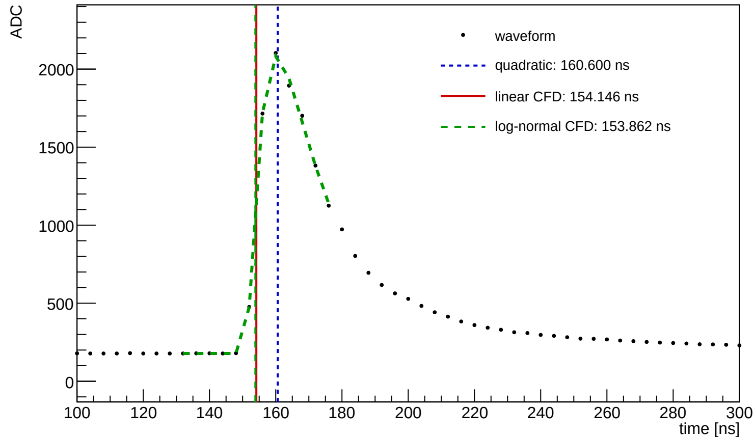
Waveform Time Demo (entry=70893, ch=1, module=1144, trigger=SUM)
