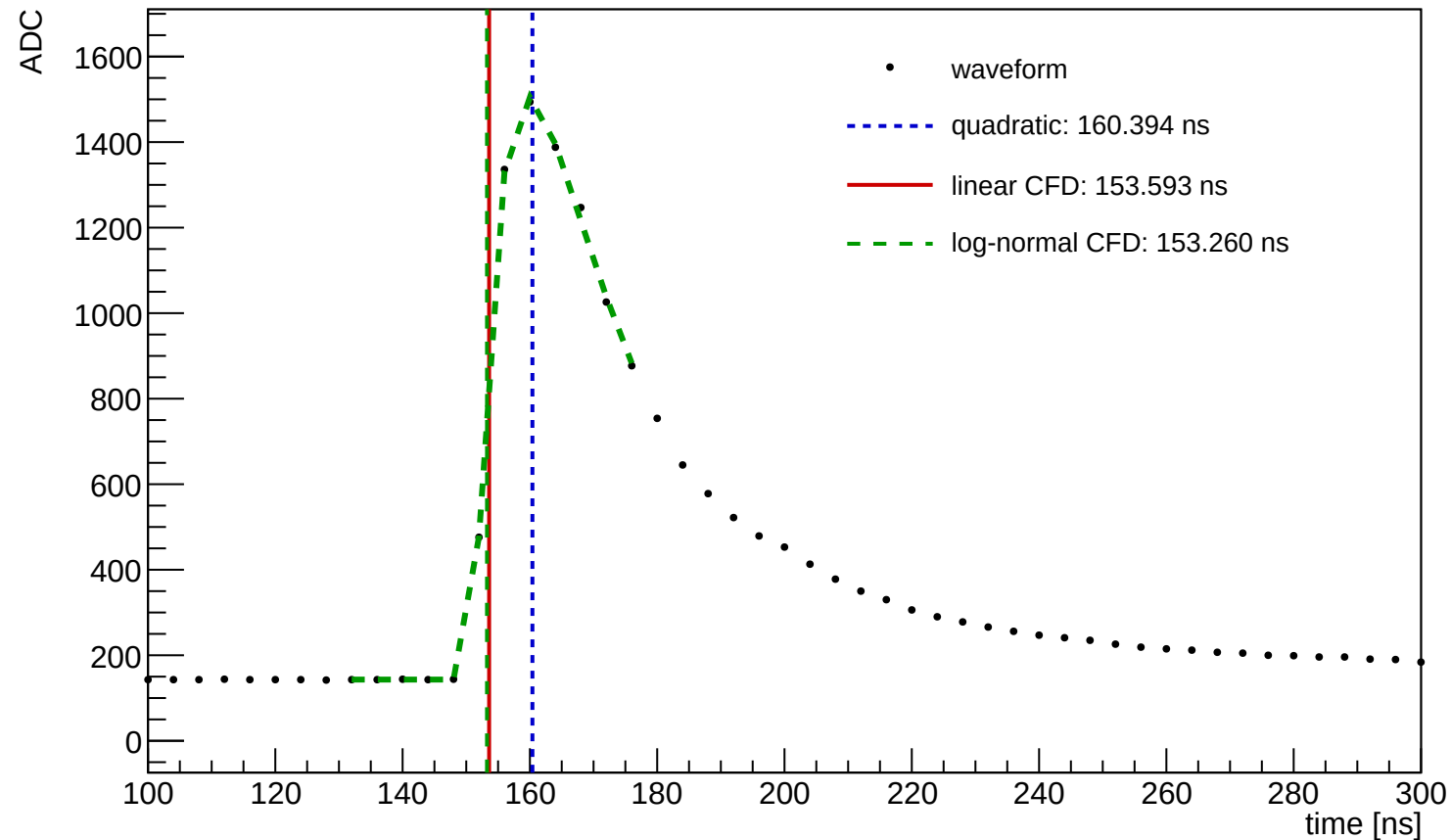
Waveform Time Demo (entry=35284, ch=5, module=1044, trigger=SUM)
