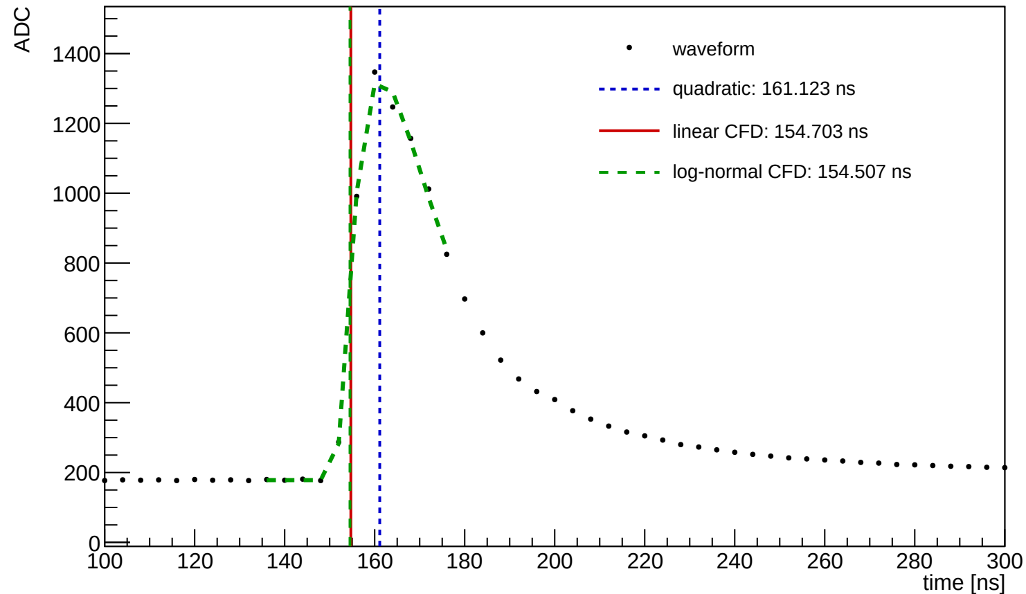
Waveform Time Demo (entry=14172, ch=9, module=1148, trigger=SUM)
