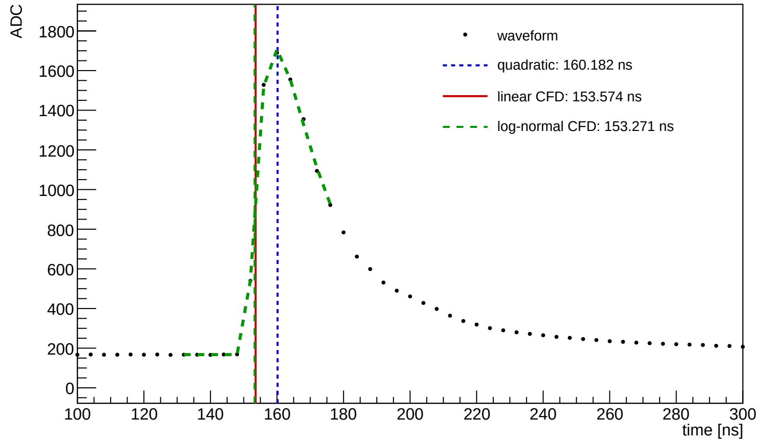
Waveform Time Demo (entry=53278, ch=10, module=1051, trigger=SUM)
