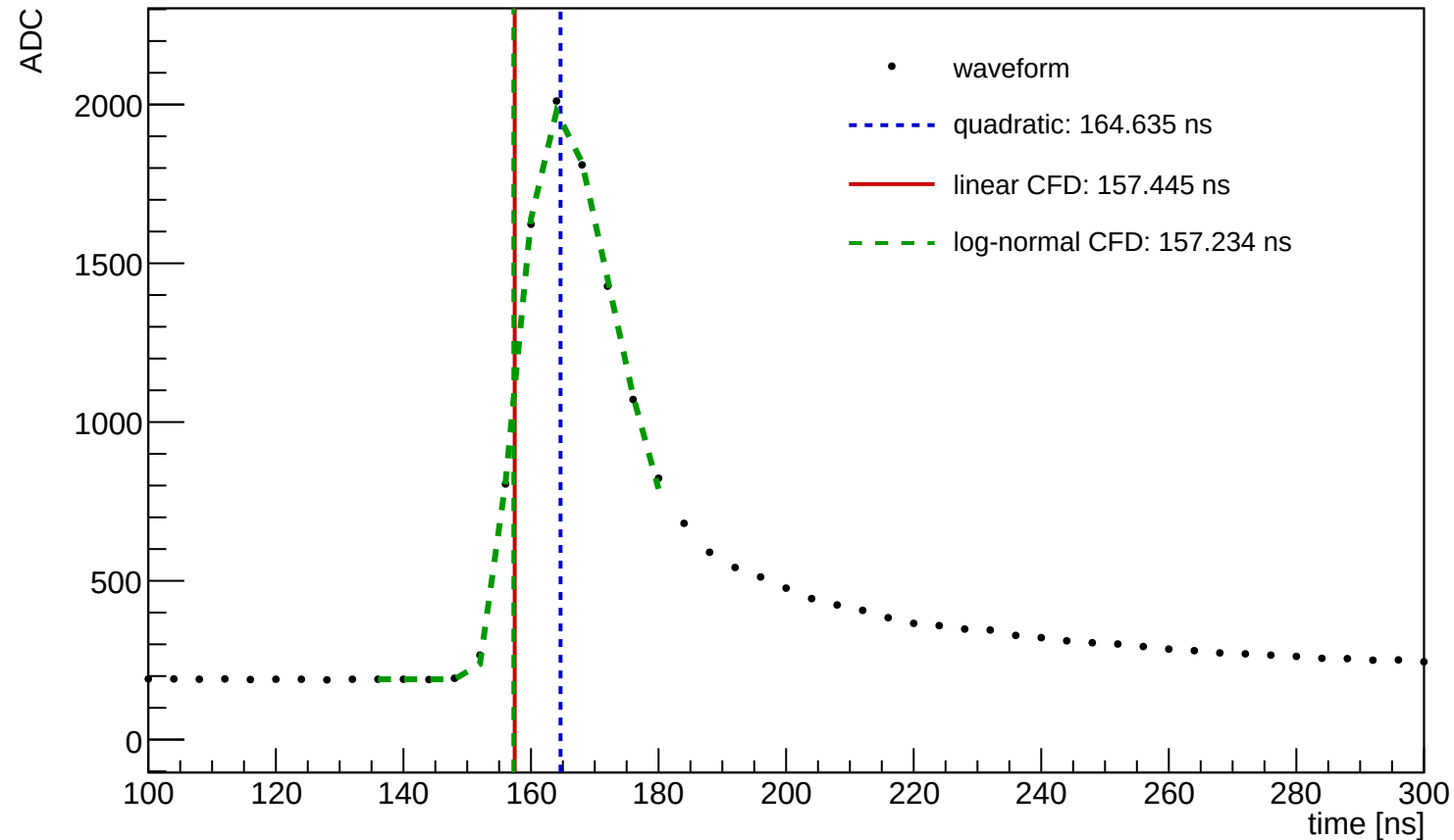
Waveform Time Demo (entry=64499, ch=1, module=1001, trigger=SUM)
