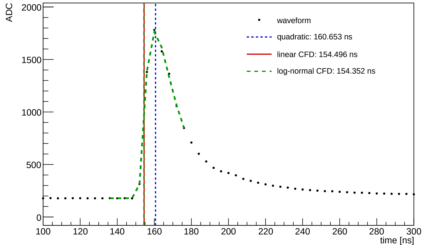
Waveform Time Demo (entry=72010, ch=8, module=1021, trigger=SUM)
