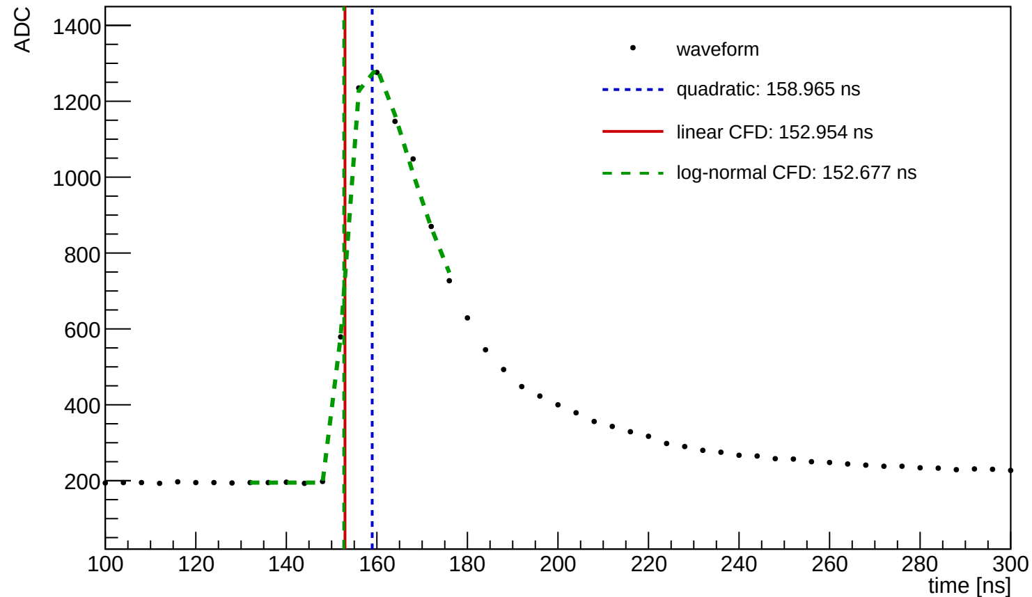
Waveform Time Demo (entry=6114, ch=6, module=1149, trigger=SUM)
