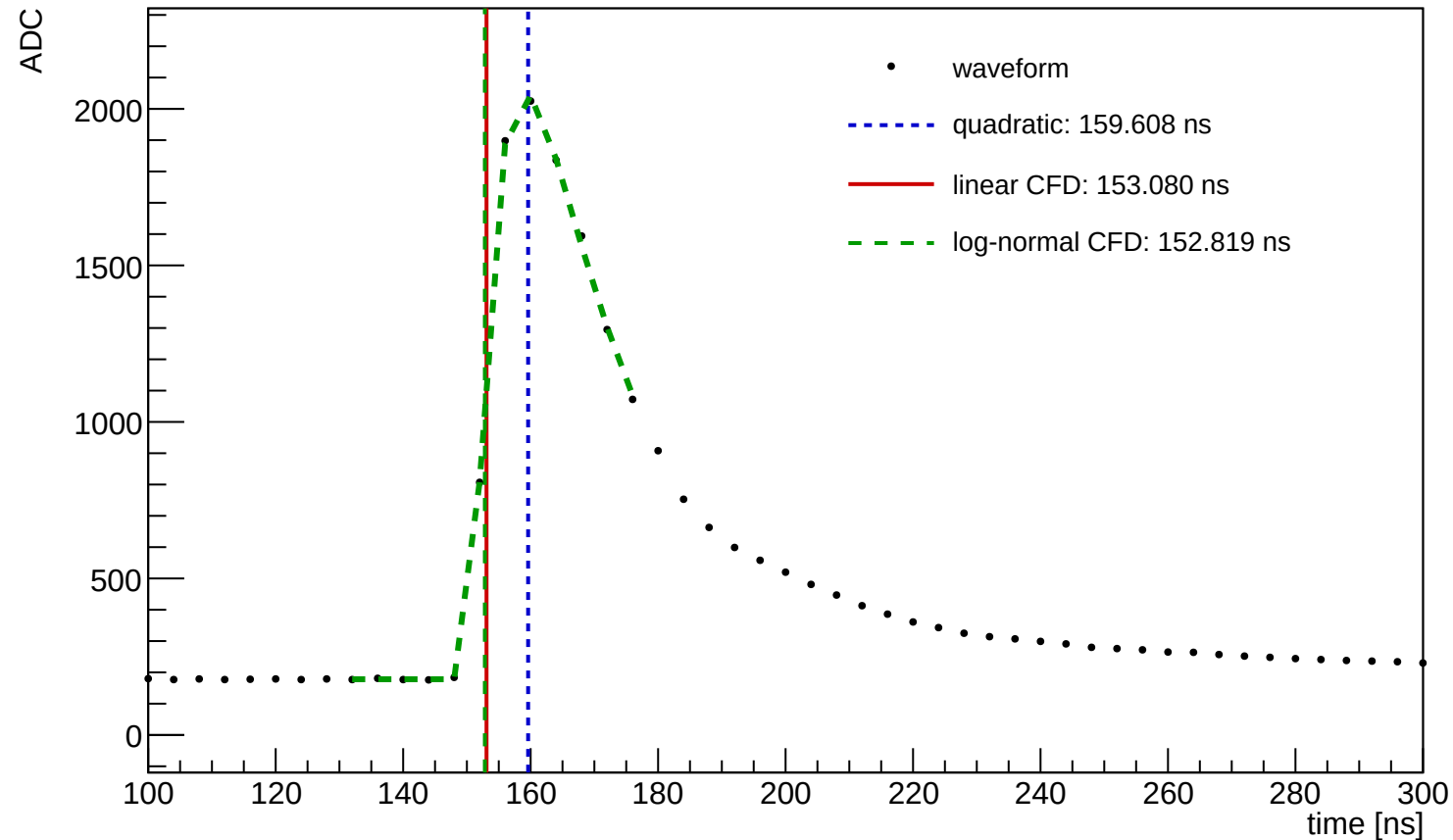
Waveform Time Demo (entry=30394, ch=0, module=1144, trigger=SUM)
