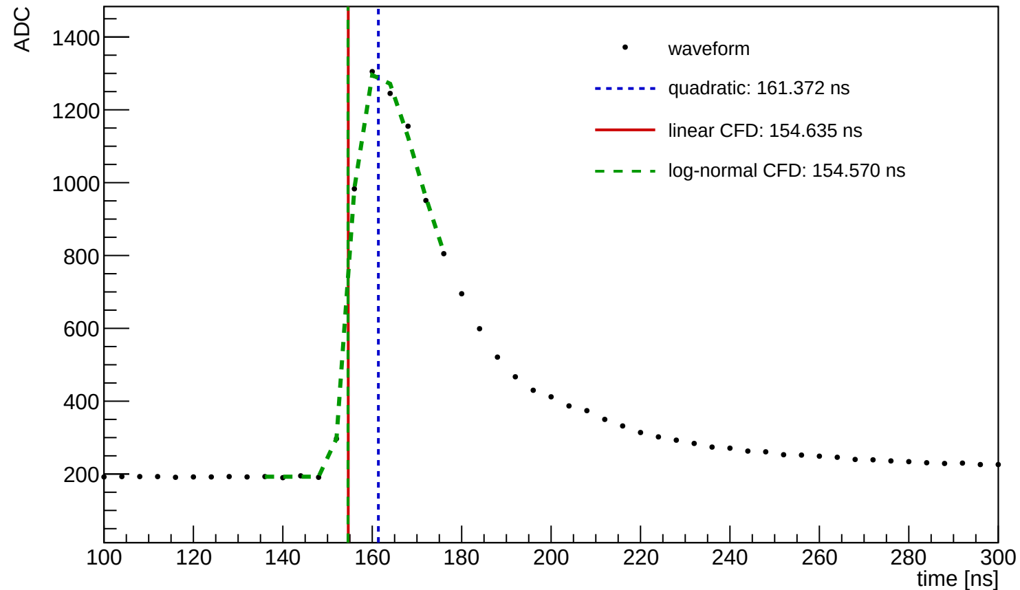
Waveform Time Demo (entry=54361, ch=10, module=1155, trigger=SUM)
