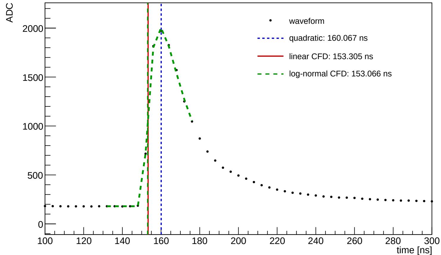
Waveform Time Demo (entry=9190, ch=3, module=1020, trigger=SUM)
