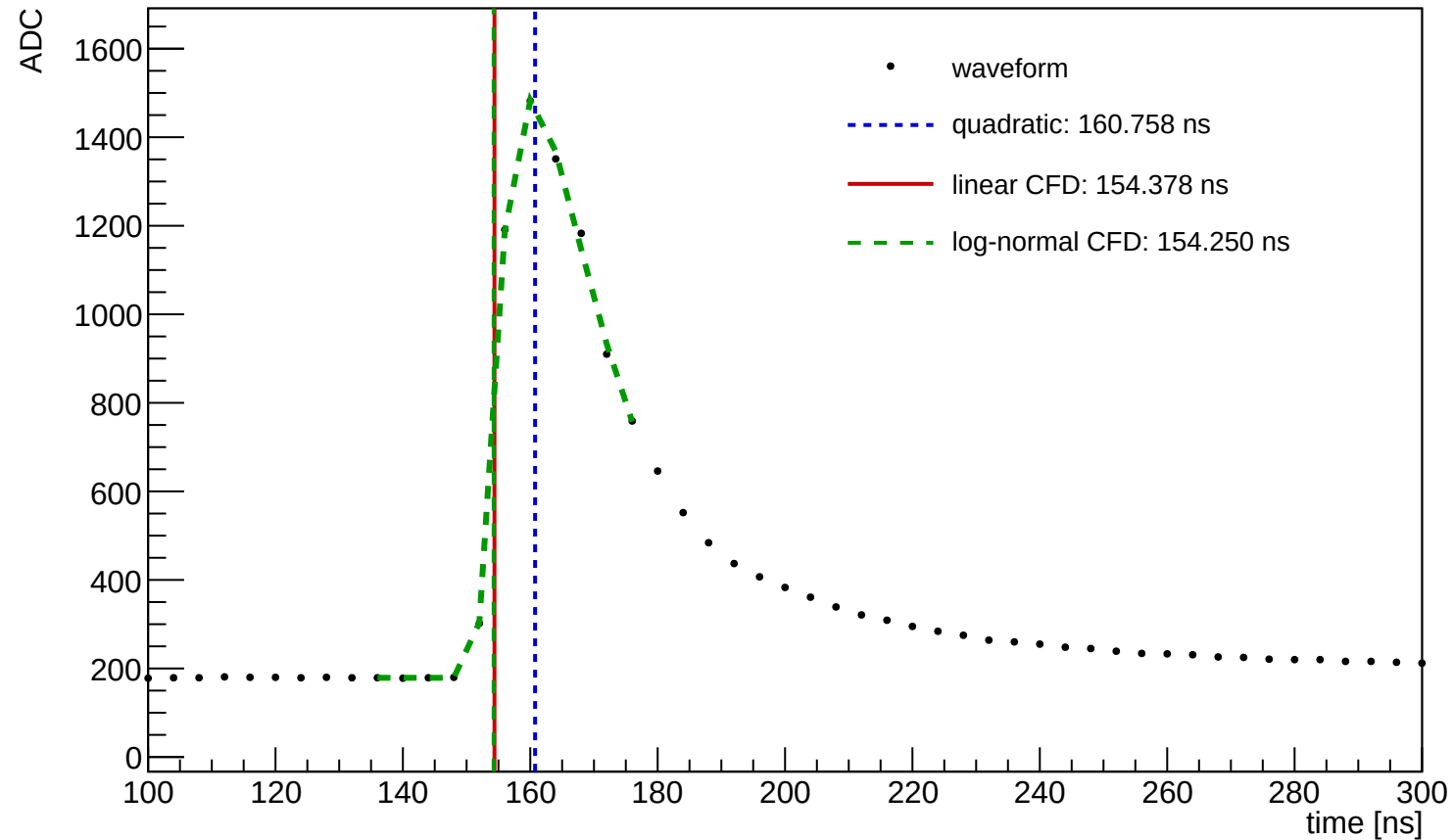
Waveform Time Demo (entry=53276, ch=13, module=1021, trigger=SUM)
