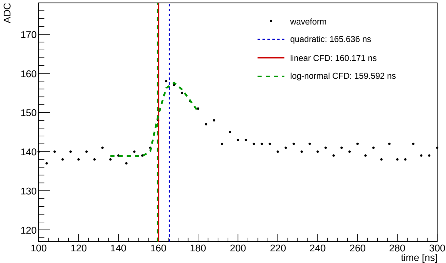
Waveform Time Demo (entry=1013, ch=4, module=1046, trigger=SUM)
