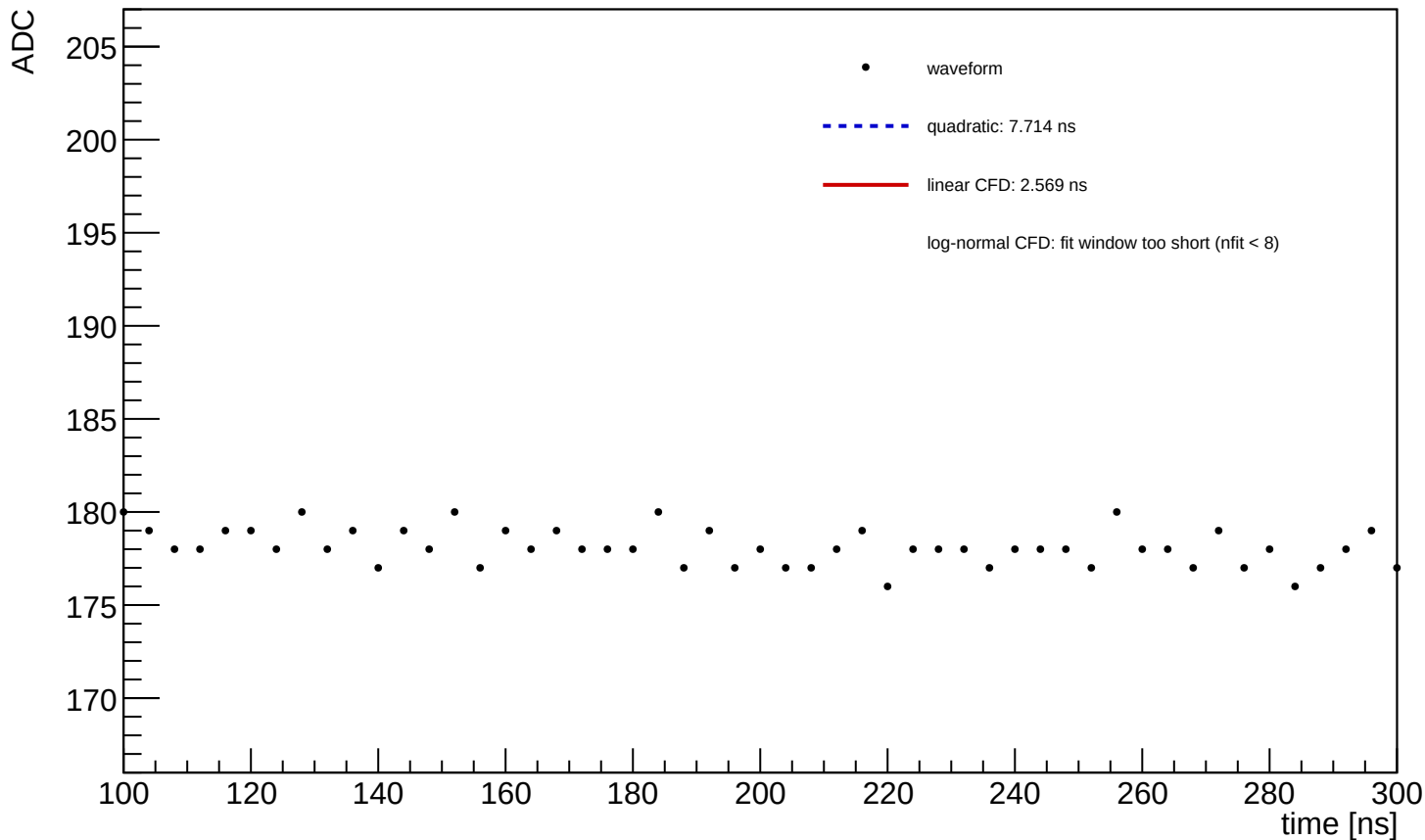
Waveform Time Demo (entry=571, ch=0, module=1038, trigger=SUM)
