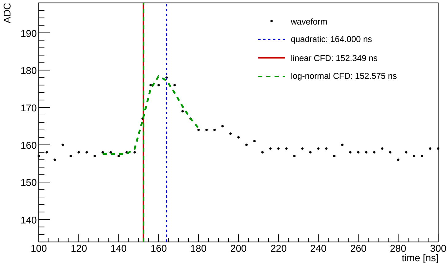
Waveform Time Demo (entry=37, ch=10, module=1118, trigger=SUM)
