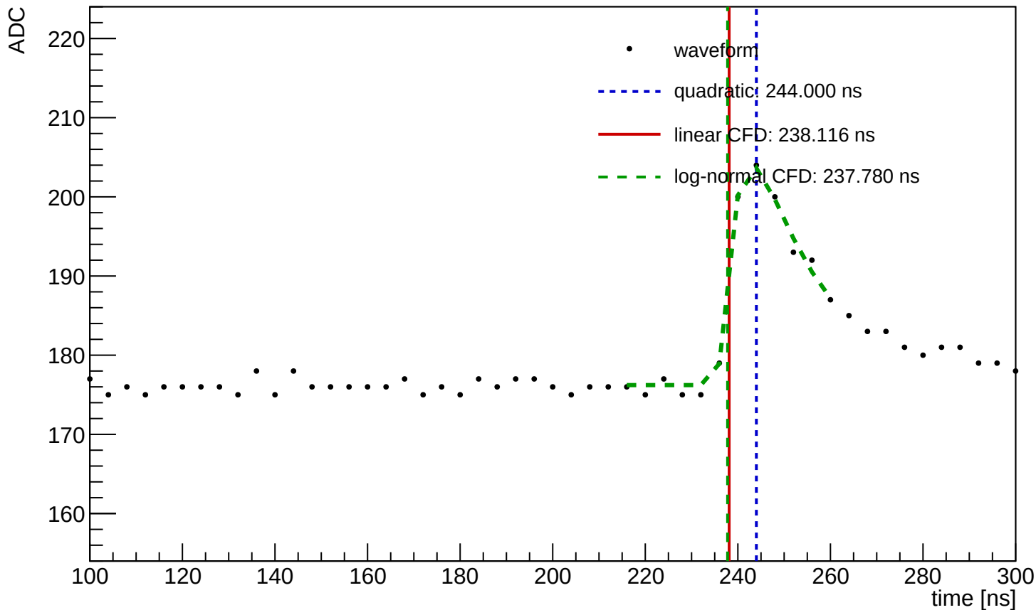
Waveform Time Demo (entry=465, ch=10, module=1147, trigger=SUM)
