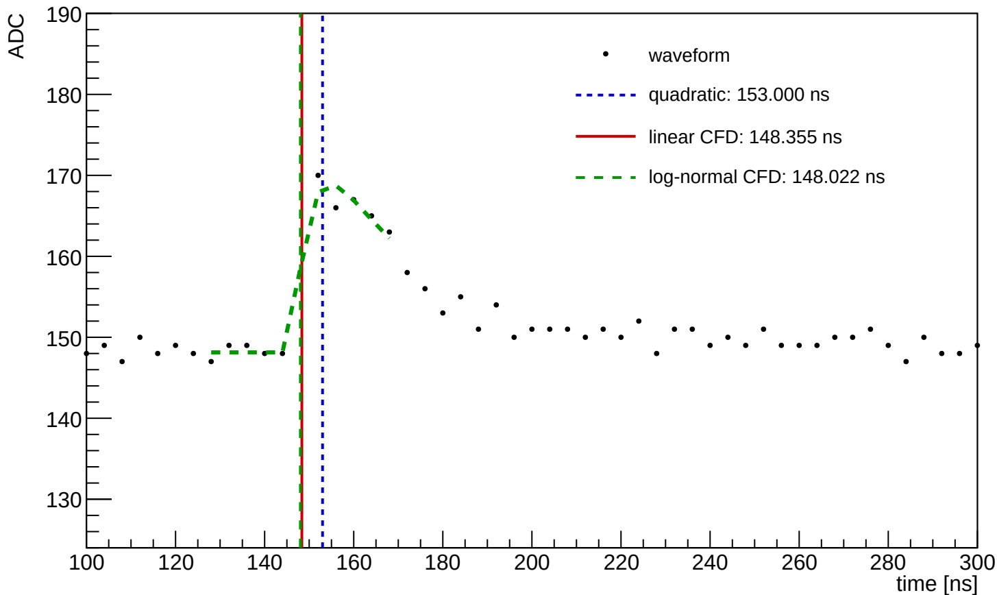
Waveform Time Demo (entry=37, ch=11, module=1117, trigger=SUM)
