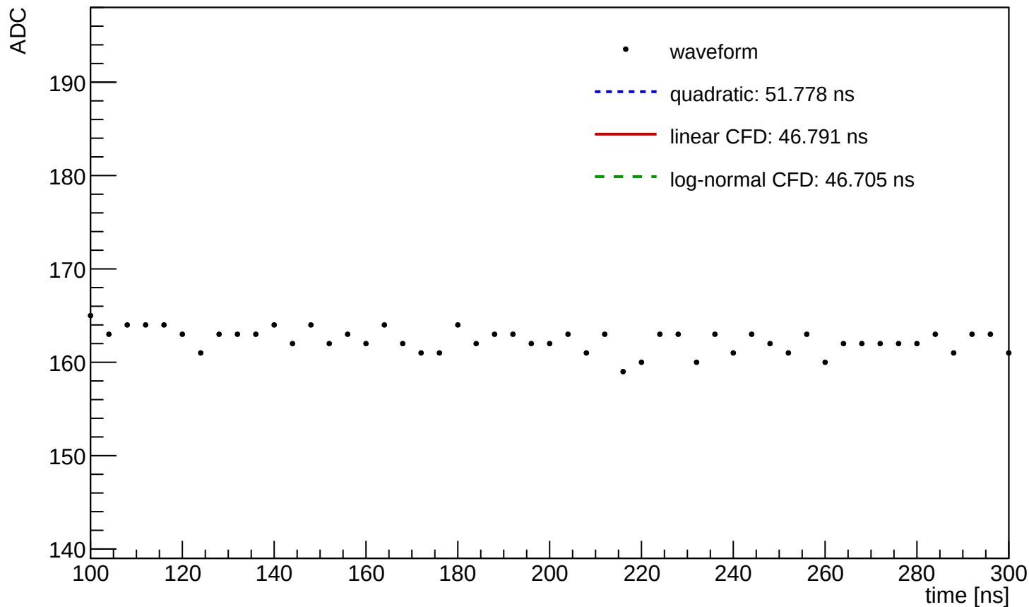
Waveform Time Demo (entry=1202, ch=16, module=1085, trigger=SUM)
