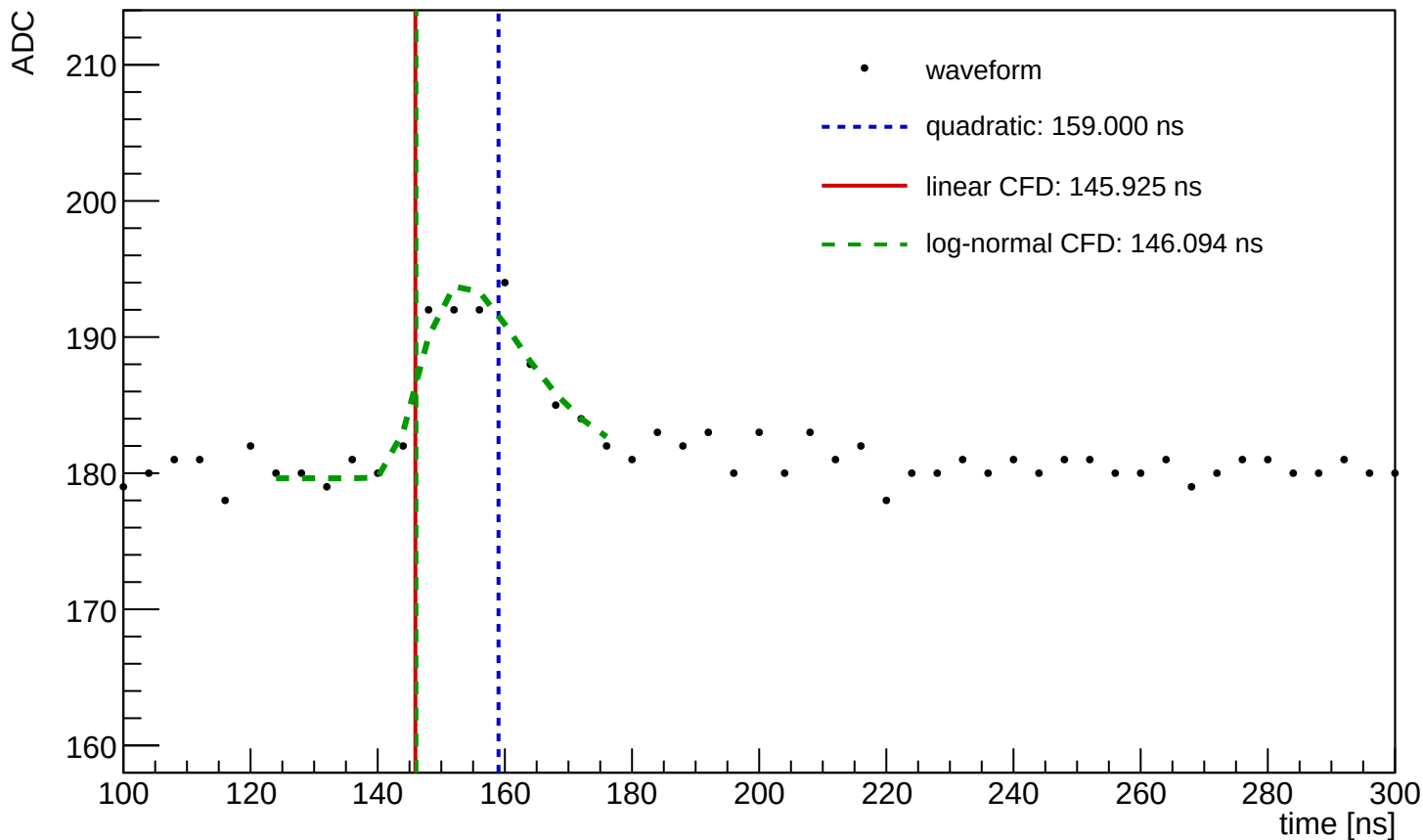
Waveform Time Demo (entry=521, ch=3, module=1121, trigger=SUM)
