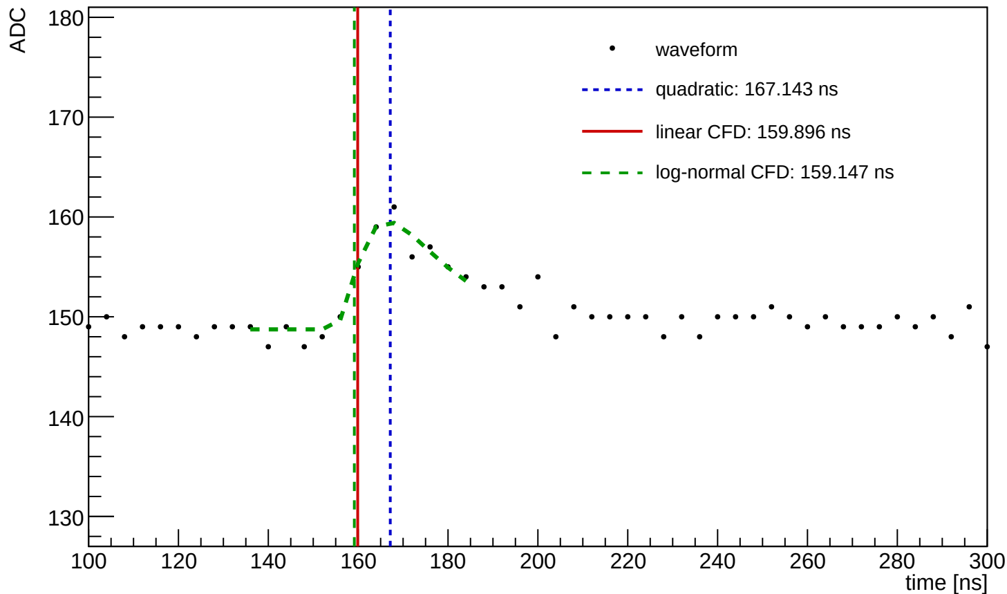
Waveform Time Demo (entry=15, ch=3, module=1112, trigger=SUM)
