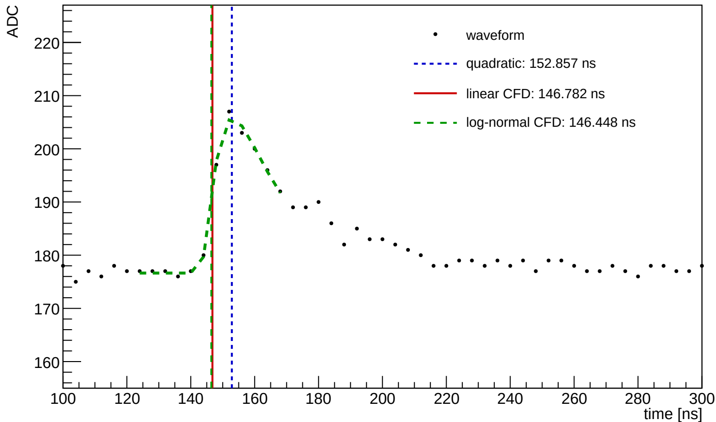
Waveform Time Demo (entry=841, ch=28, module=1065, trigger=SUM)
