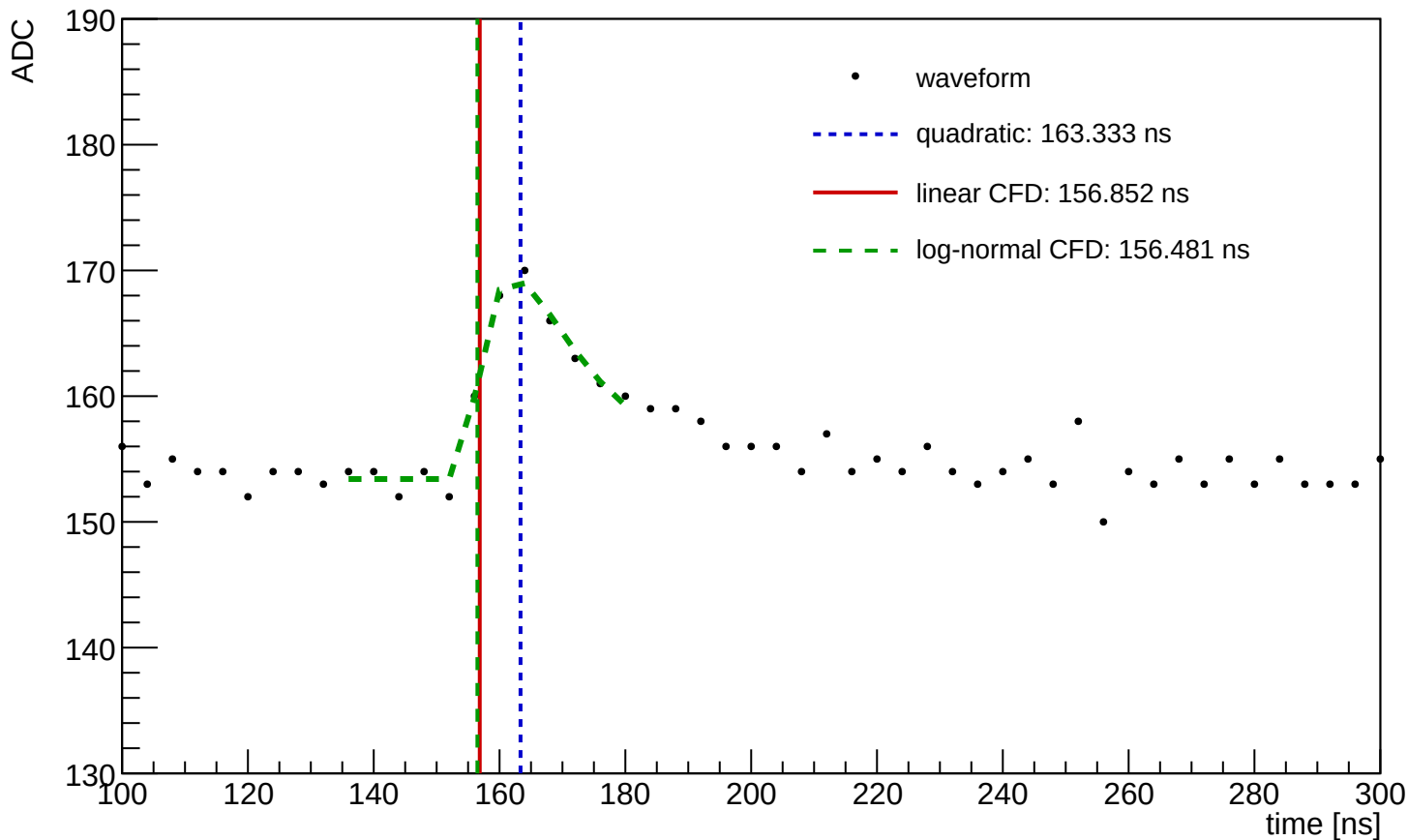
Waveform Time Demo (entry=495, ch=4, module=1113, trigger=SUM)
