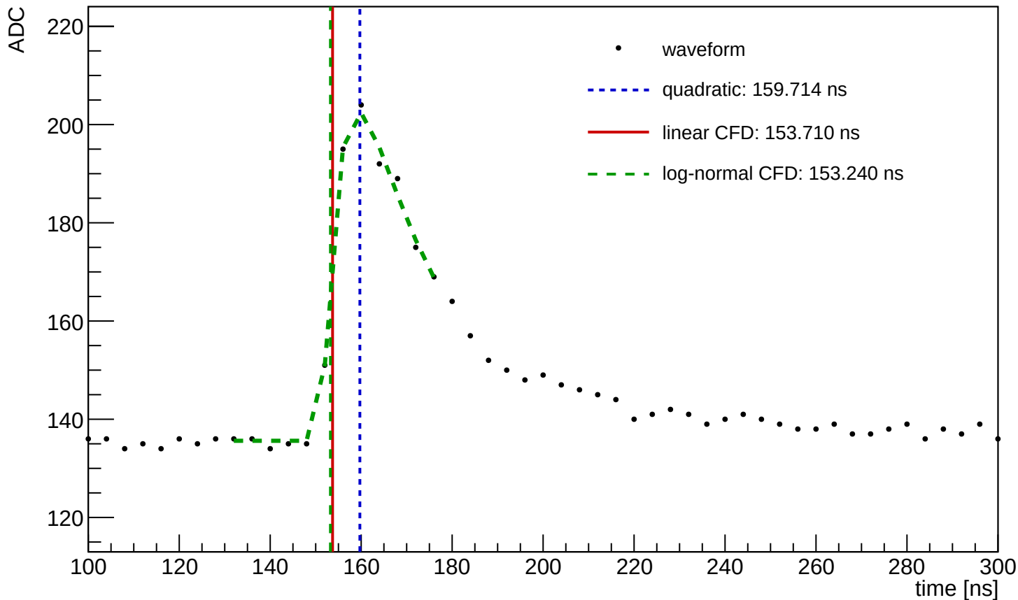
Waveform Time Demo (entry=393, ch=2, module=1003, trigger=SUM)
