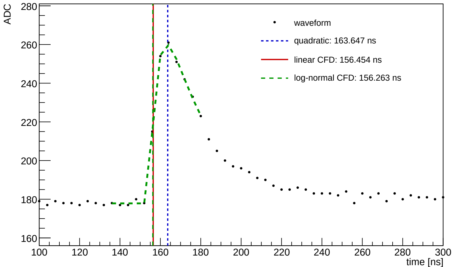
Waveform Time Demo (entry=495, ch=12, module=1148, trigger=SUM)
