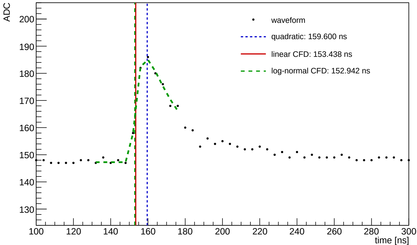
Waveform Time Demo (entry=411, ch=19, module=1102, trigger=SUM)
