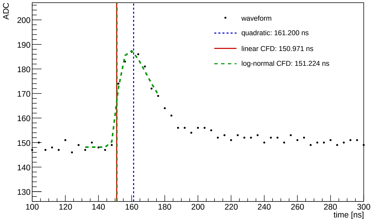
Waveform Time Demo (entry=1127, ch=13, module=1117, trigger=SUM)
