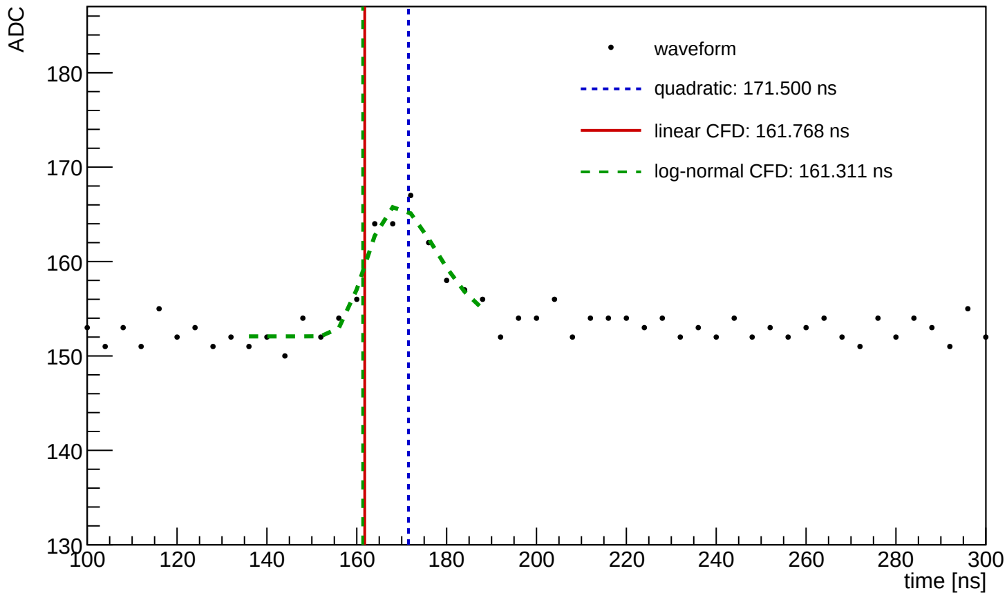
Waveform Time Demo (entry=317, ch=10, module=1119, trigger=SUM)
