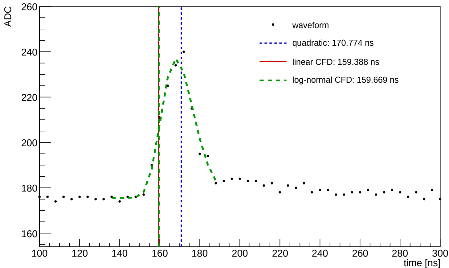
Waveform Time Demo (entry=15, ch=9, module=1146, trigger=SUM)
