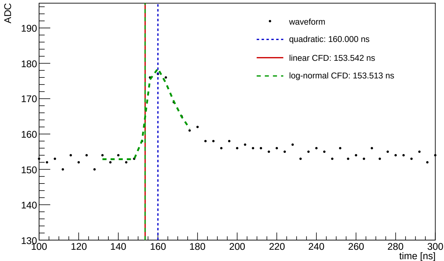
Waveform Time Demo (entry=1077, ch=0, module=1043, trigger=SUM)
