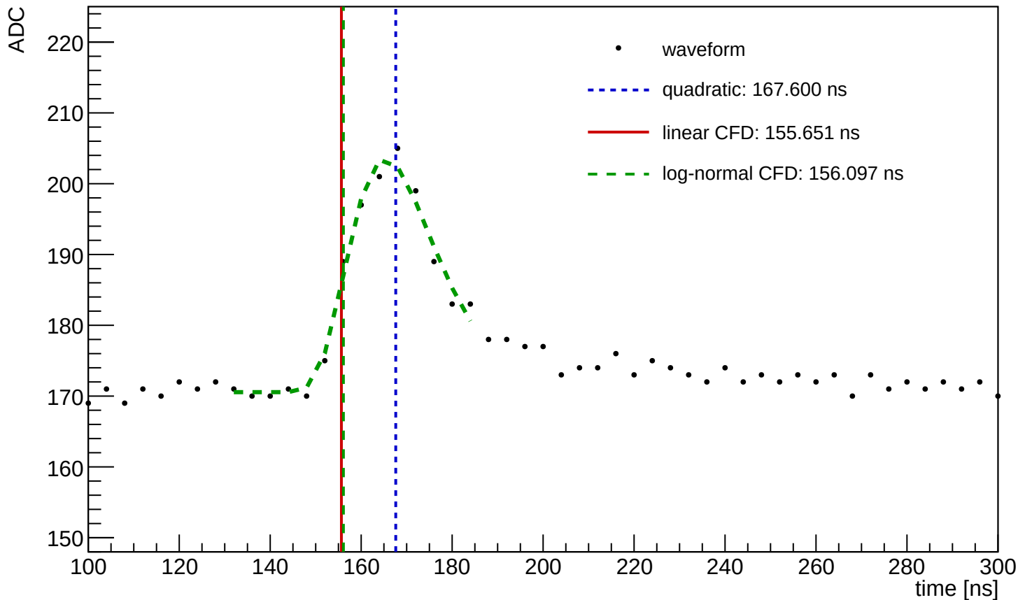
Waveform Time Demo (entry=32, ch=12, module=1129, trigger=SUM)
