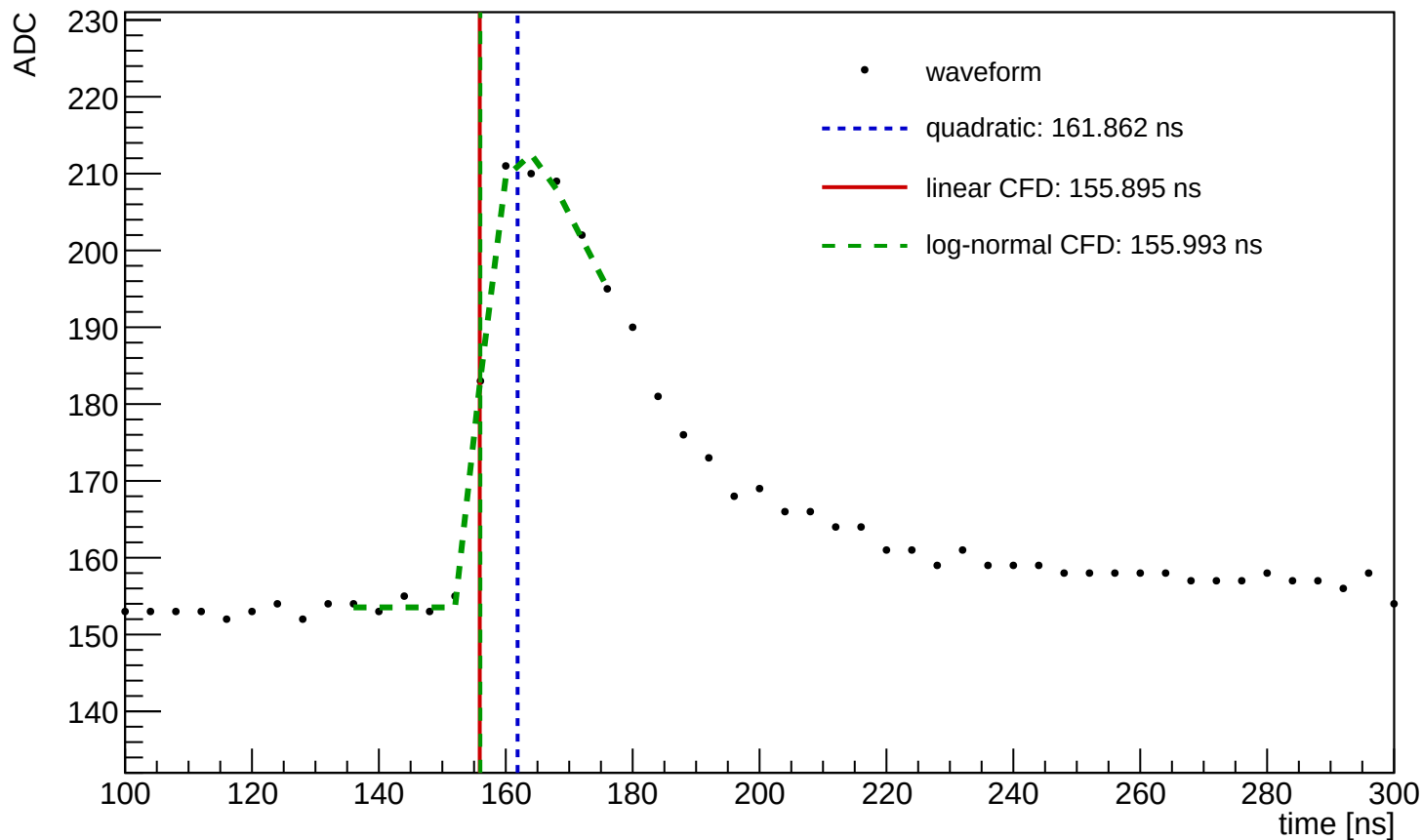
Waveform Time Demo (entry=15, ch=2, module=1113, trigger=SUM)
