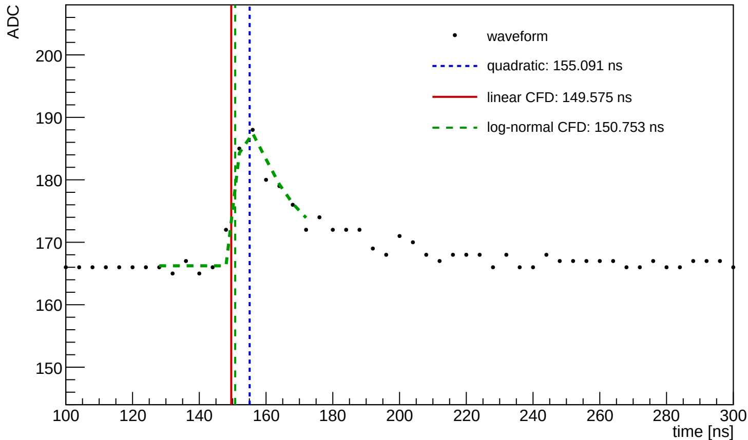
Waveform Time Demo (entry=43, ch=27, module=1097, trigger=SUM)
