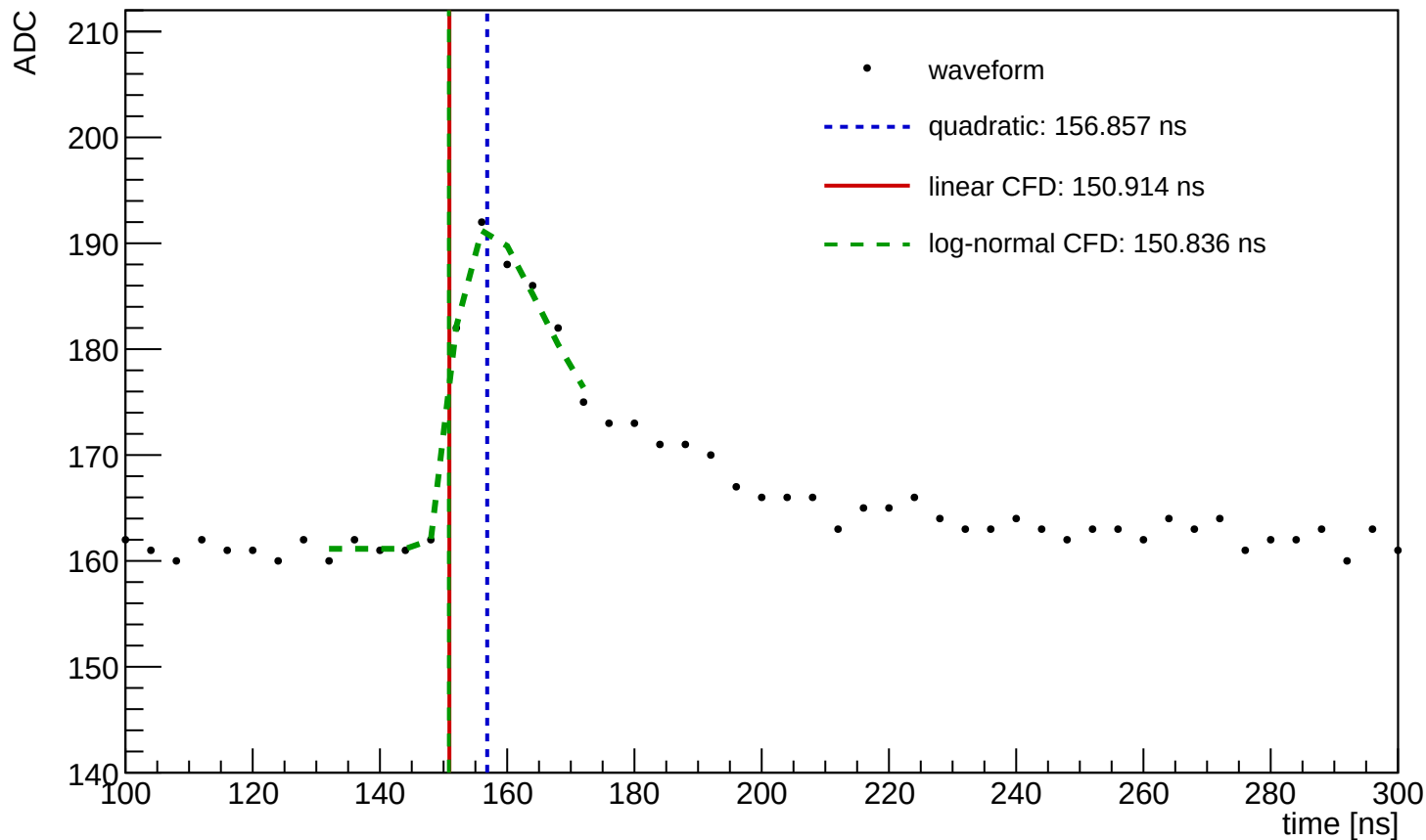
Waveform Time Demo (entry=213, ch=24, module=1033, trigger=SUM)
