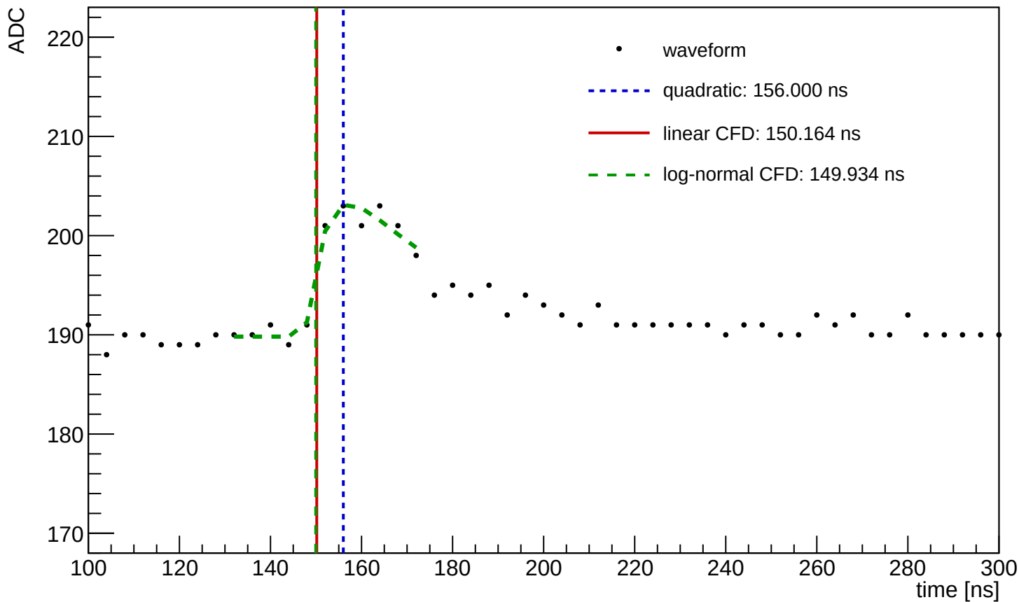
Waveform Time Demo (entry=834, ch=10, module=1019, trigger=SUM)
