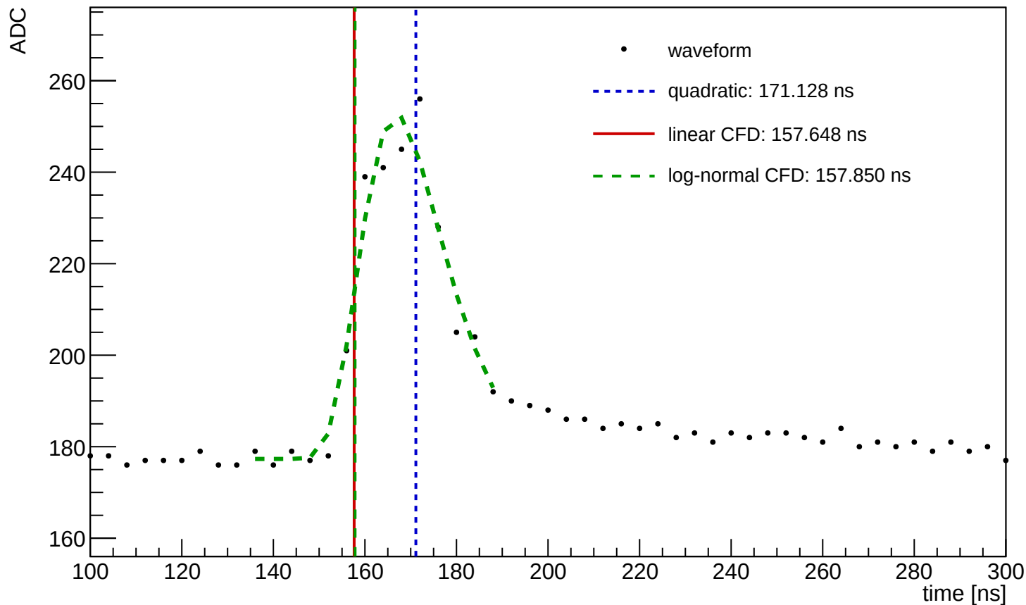
Waveform Time Demo (entry=15, ch=7, module=1148, trigger=SUM)
