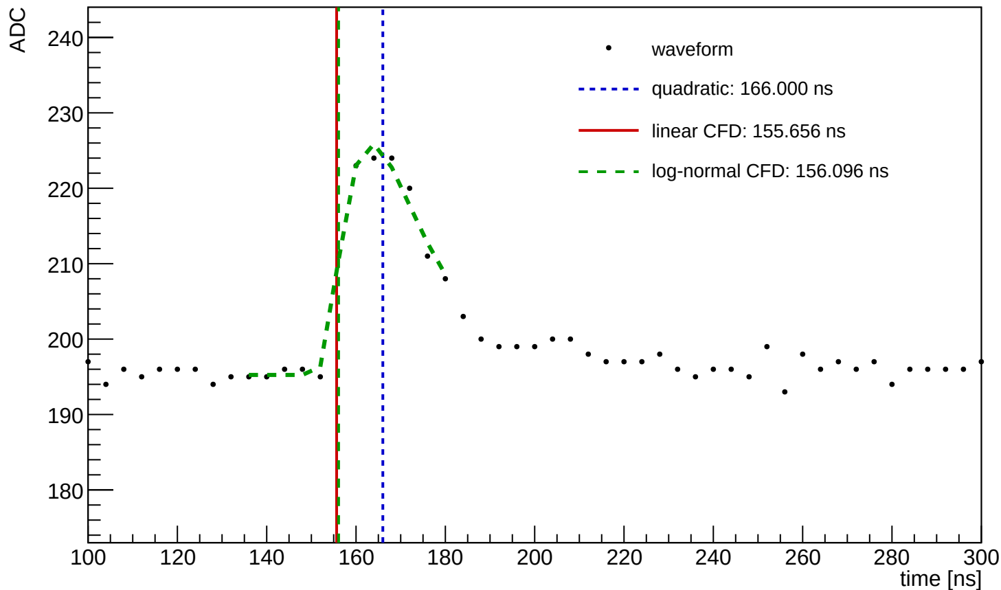
Waveform Time Demo (entry=495, ch=10, module=1150, trigger=SUM)
