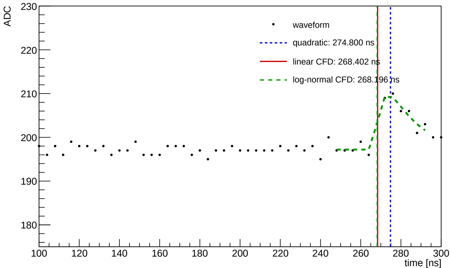
Waveform Time Demo (entry=319, ch=26, module=1055, trigger=SUM)
