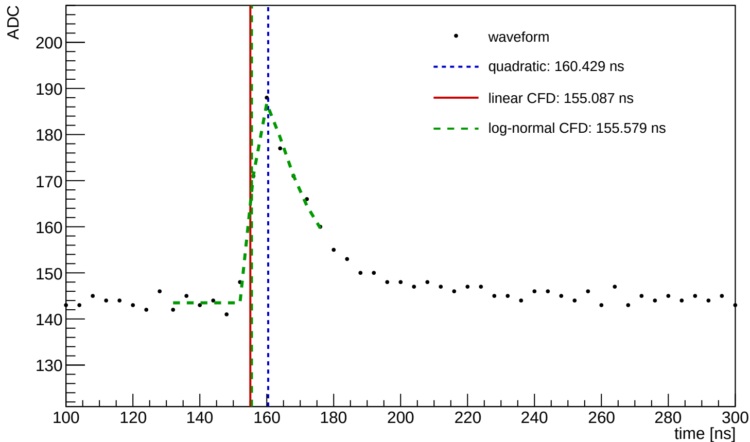
Waveform Time Demo (entry=429, ch=6, module=1156, trigger=SUM)
