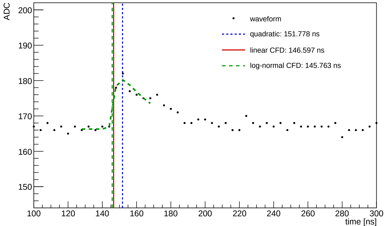
Waveform Time Demo (entry=841, ch=27, module=1097, trigger=SUM)
