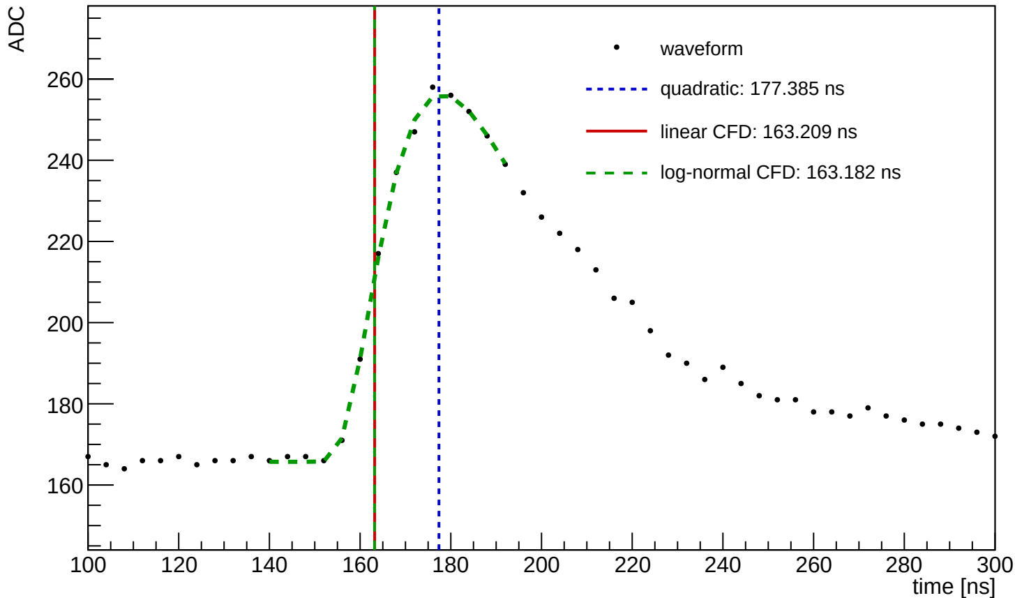
Waveform Time Demo (entry=1186, ch=1332, module=1130, trigger=LMS)
