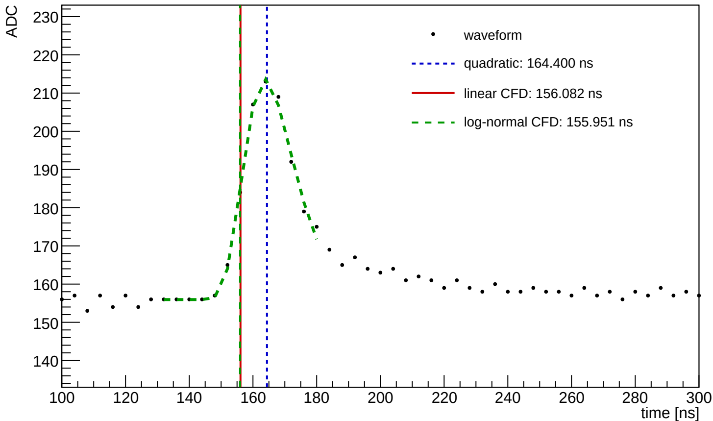
Waveform Time Demo (entry=1127, ch=9, module=1050, trigger=SUM)
