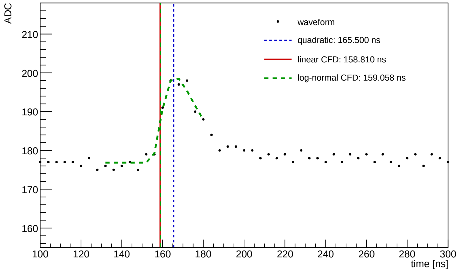
Waveform Time Demo (entry=691, ch=3, module=1147, trigger=SUM)
