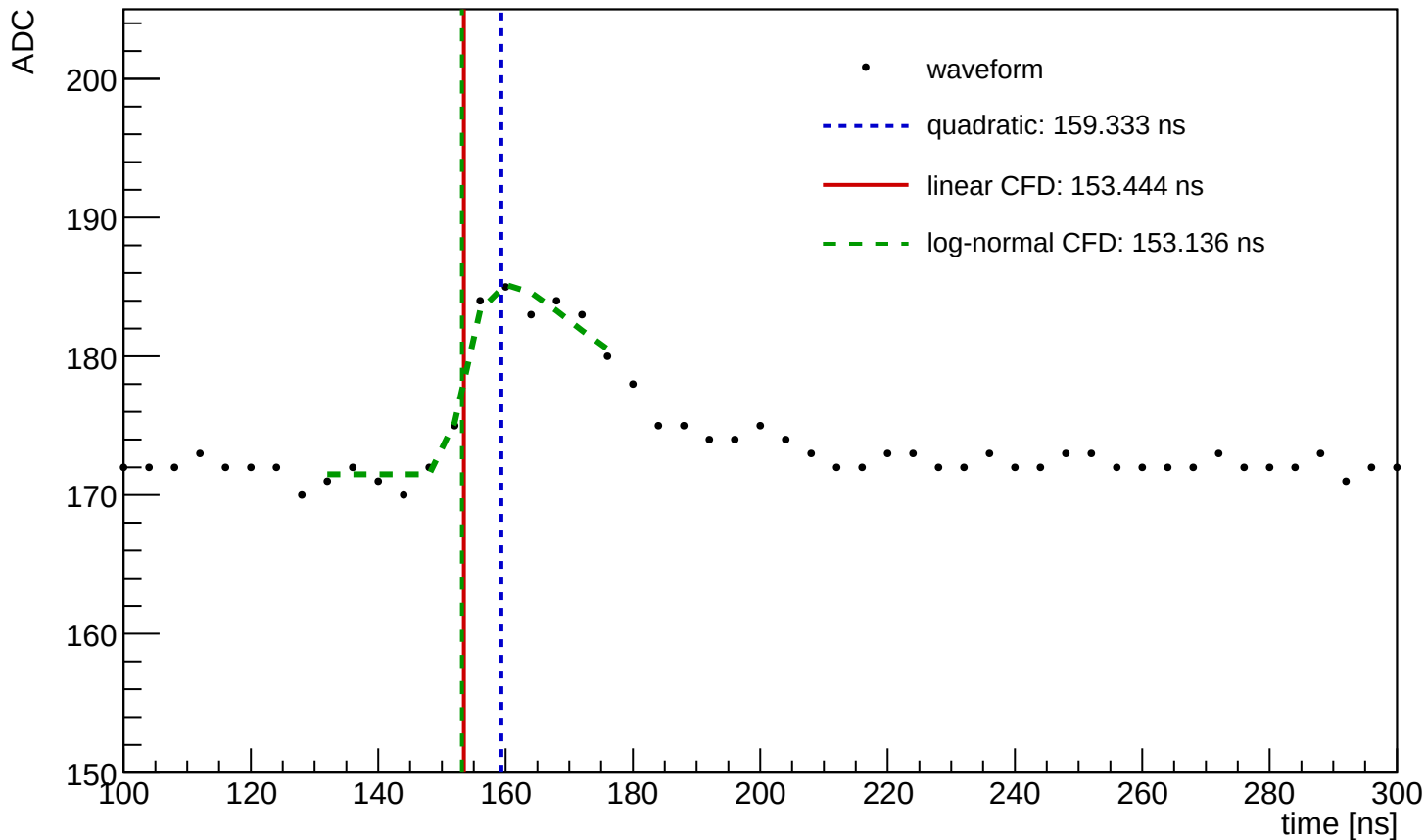
Waveform Time Demo (entry=1212, ch=29, module=1092, trigger=SUM)
