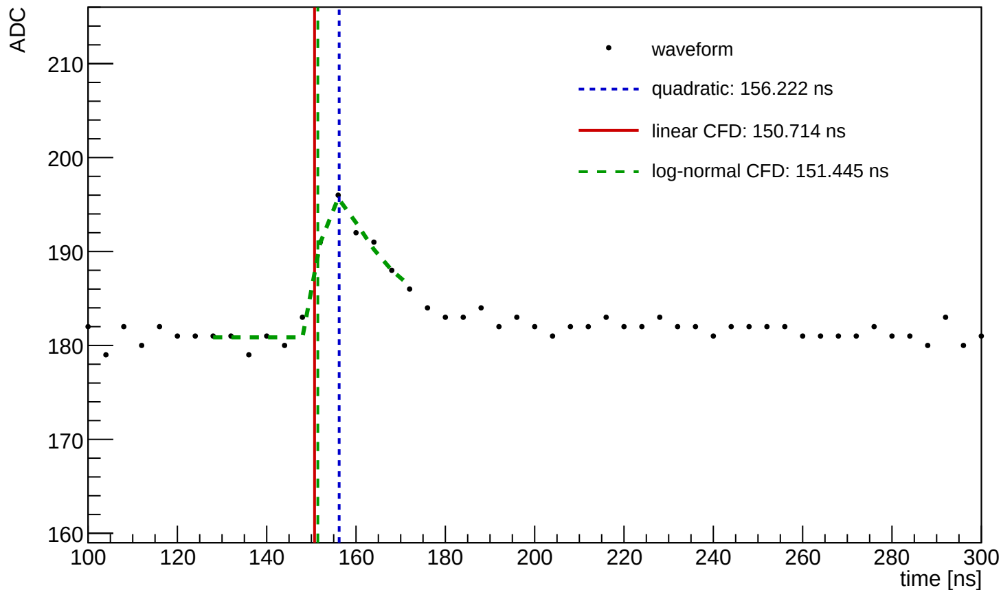
Waveform Time Demo (entry=200, ch=3, module=1020, trigger=SUM)
