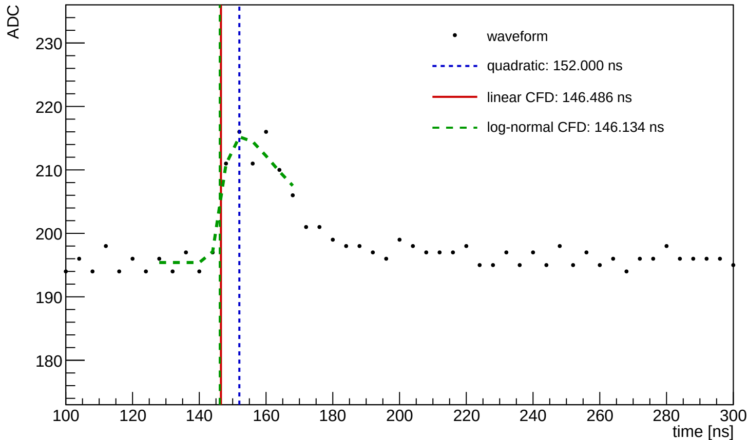
Waveform Time Demo (entry=185, ch=4, module=1149, trigger=SUM)
