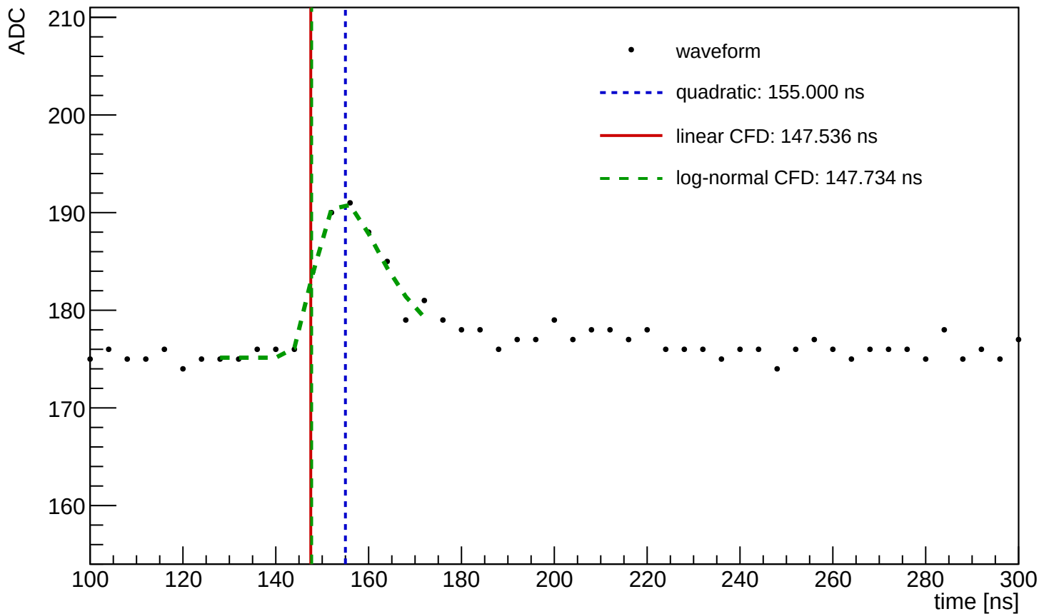
Waveform Time Demo (entry=591, ch=26, module=1027, trigger=SUM)
