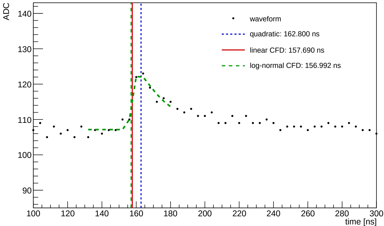
Waveform Time Demo (entry=1127, ch=2, module=1014, trigger=SUM)
