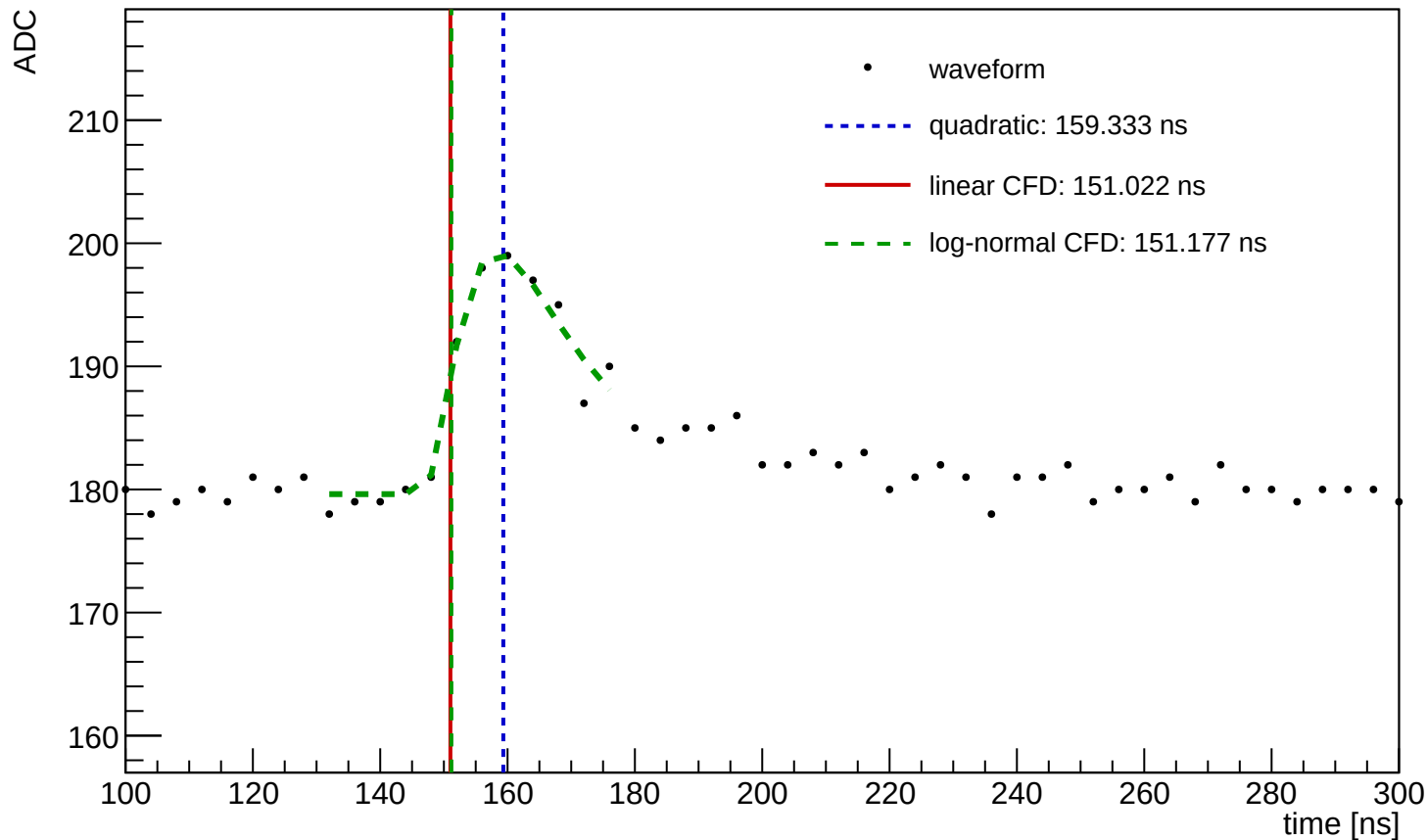
Waveform Time Demo (entry=837, ch=21, module=1089, trigger=SUM)
