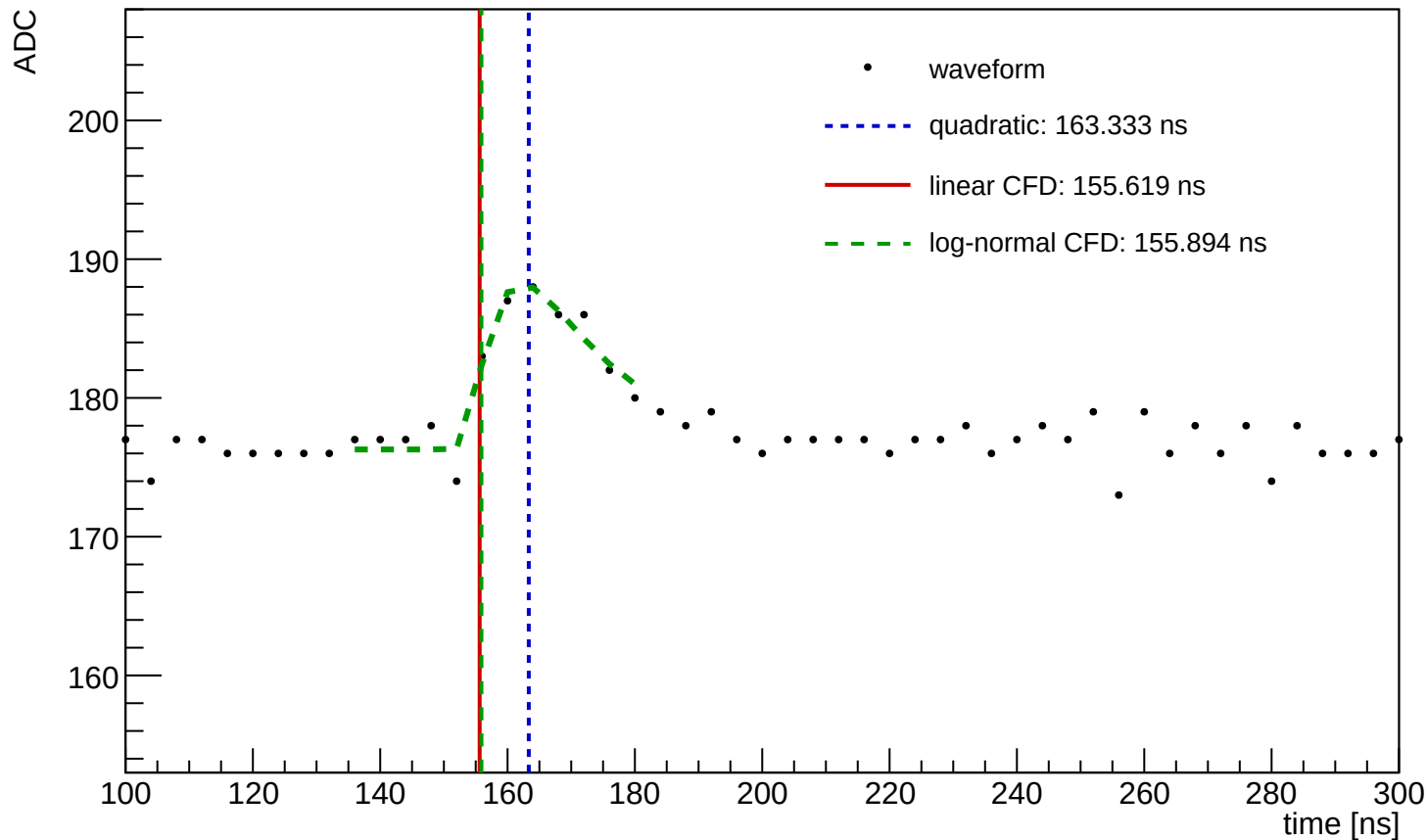
Waveform Time Demo (entry=495, ch=13, module=1147, trigger=SUM)
