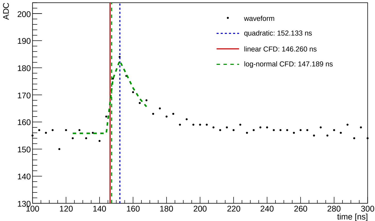
Waveform Time Demo (entry=245, ch=0, module=1137, trigger=SUM)
