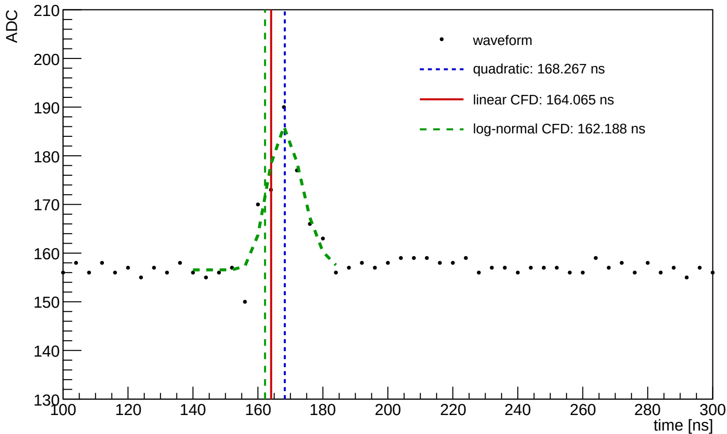
Waveform Time Demo (entry=1127, ch=6, module=1118, trigger=SUM)
