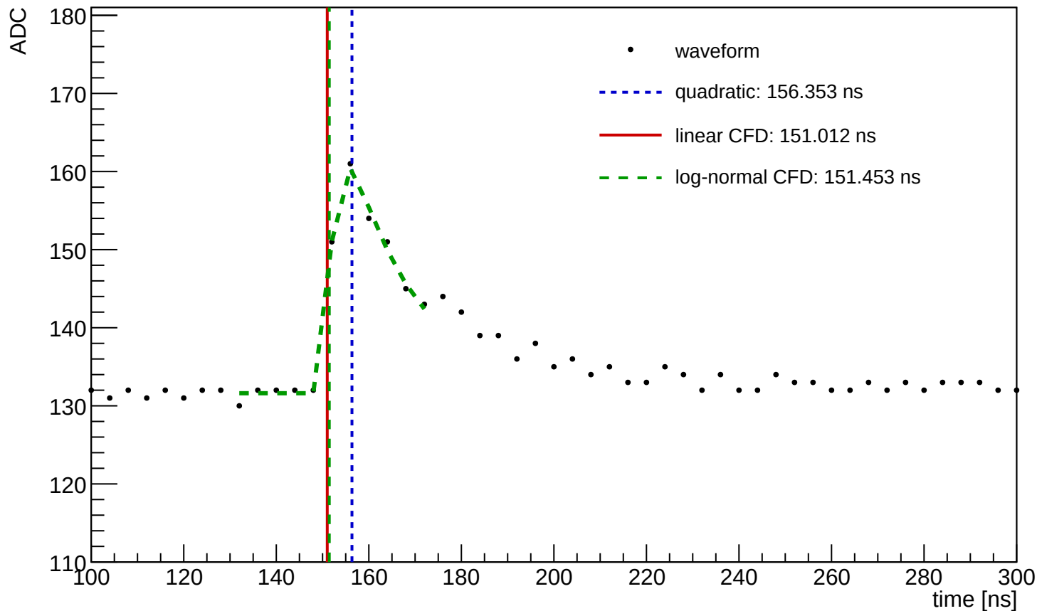
Waveform Time Demo (entry=369, ch=0, module=1071, trigger=SUM)
