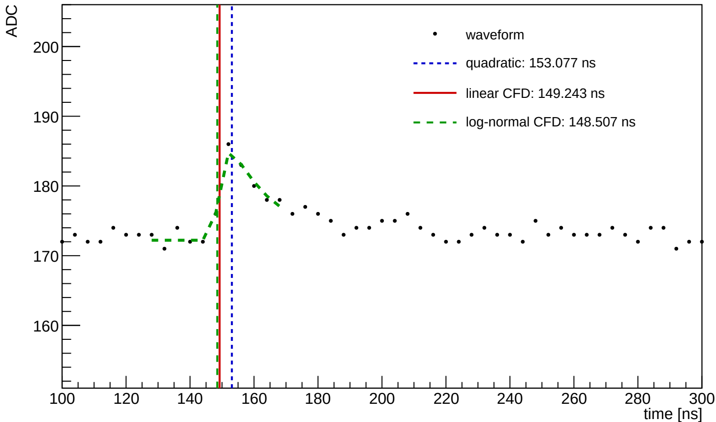
Waveform Time Demo (entry=213, ch=23, module=1029, trigger=SUM)
