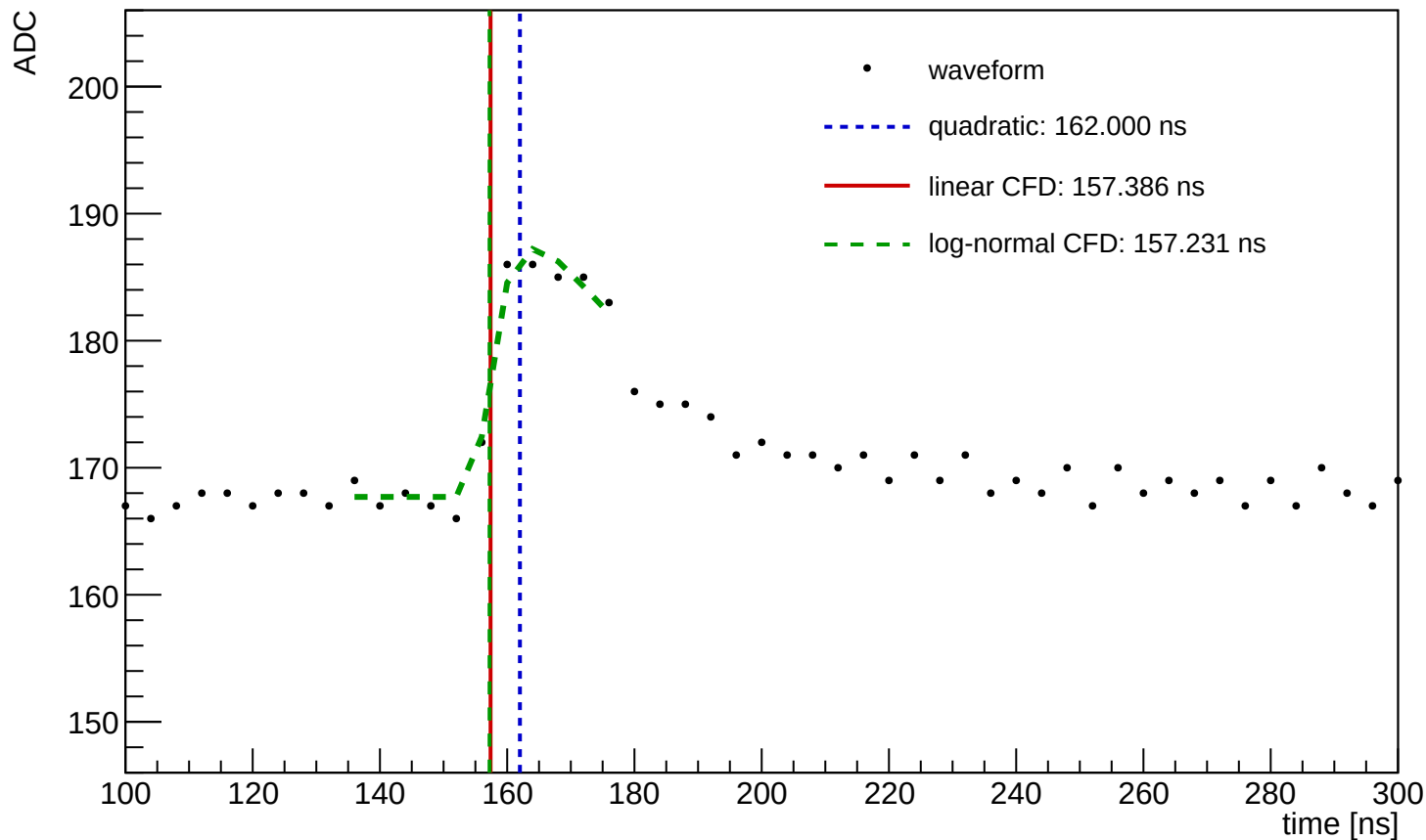
Waveform Time Demo (entry=32, ch=2, module=1126, trigger=SUM)
