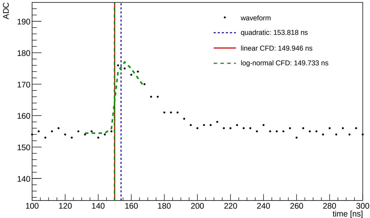
Waveform Time Demo (entry=1155, ch=14, module=1099, trigger=SUM)
