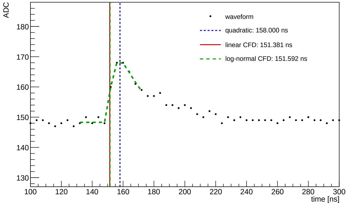
Waveform Time Demo (entry=43, ch=23, module=1124, trigger=SUM)
