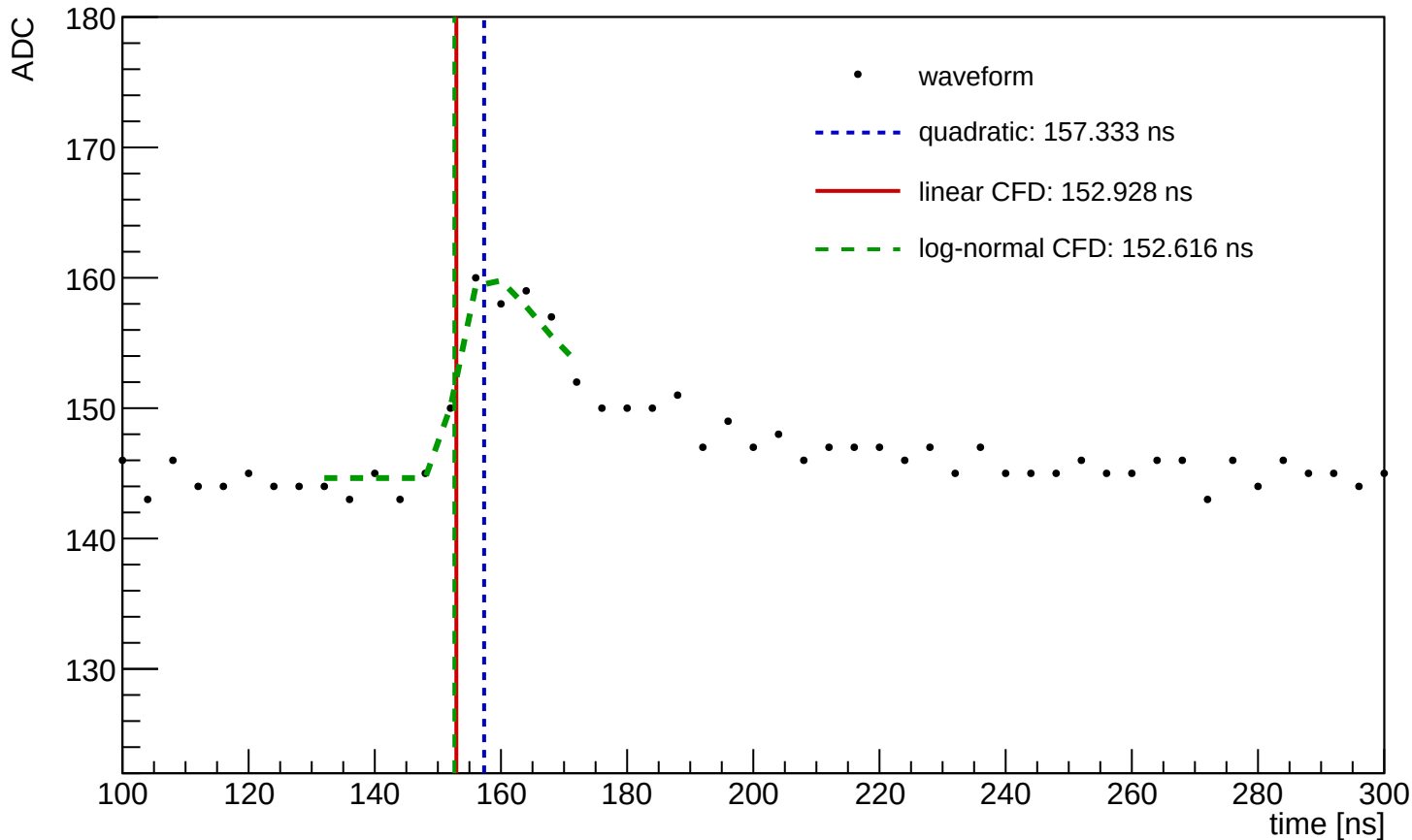
Waveform Time Demo (entry=1231, ch=15, module=1125, trigger=SUM)
