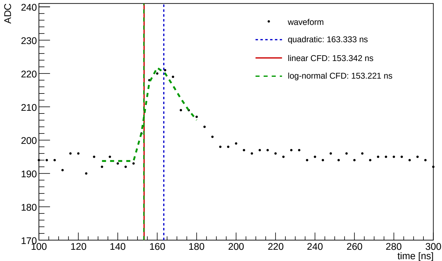
Waveform Time Demo (entry=1126, ch=13, module=1034, trigger=SUM)
