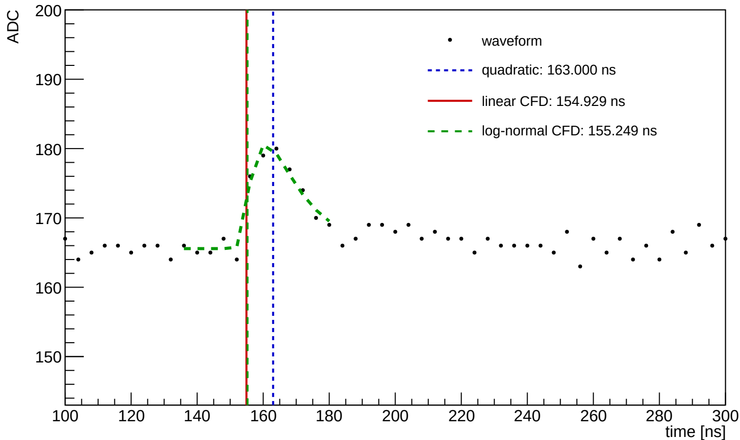
Waveform Time Demo (entry=495, ch=2, module=1115, trigger=SUM)
