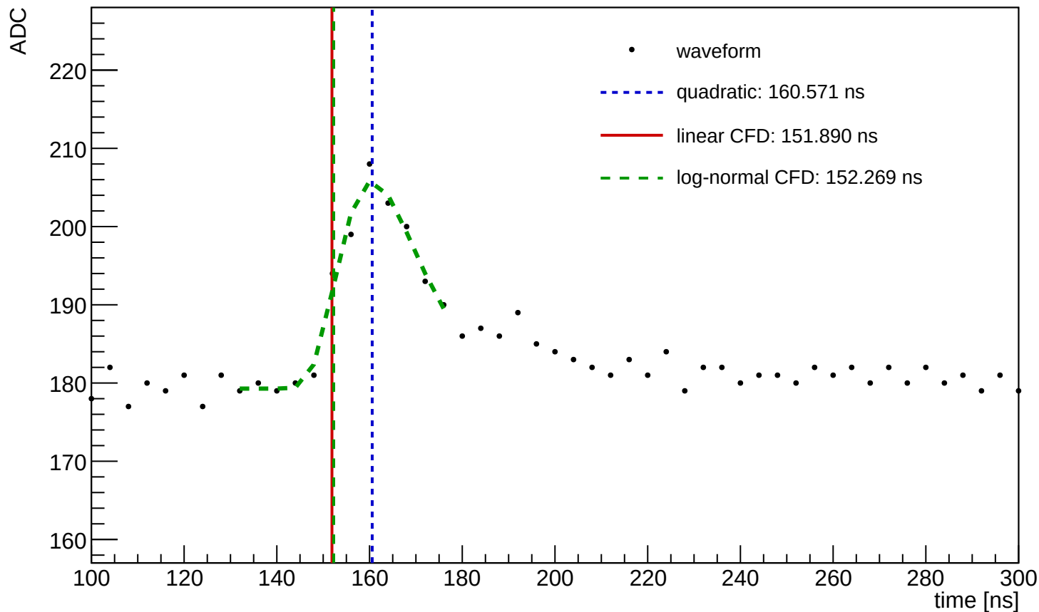
Waveform Time Demo (entry=1127, ch=0, module=1082, trigger=SUM)
