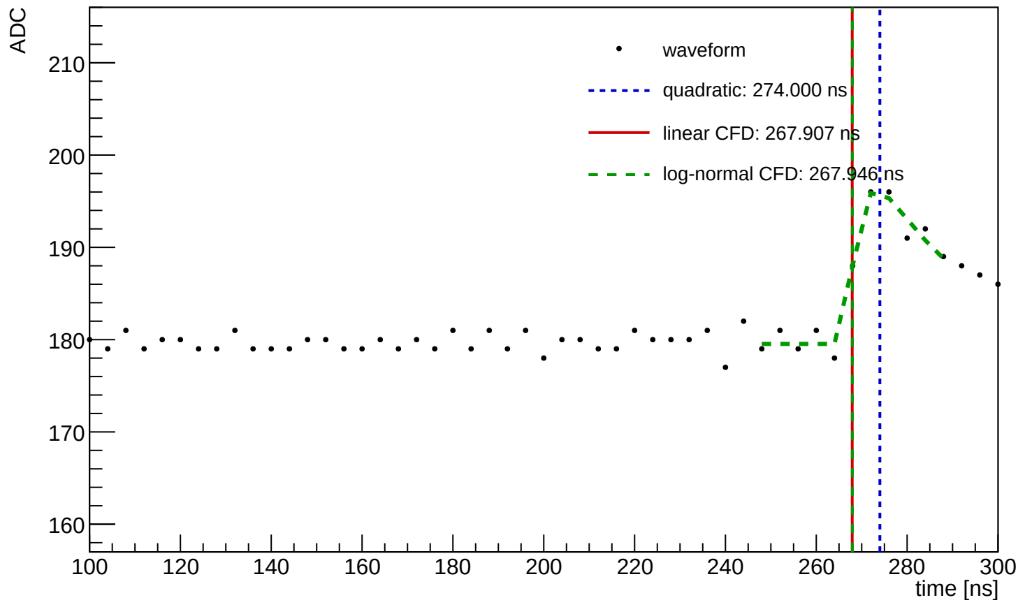
Waveform Time Demo (entry=319, ch=27, module=1025, trigger=SUM)
