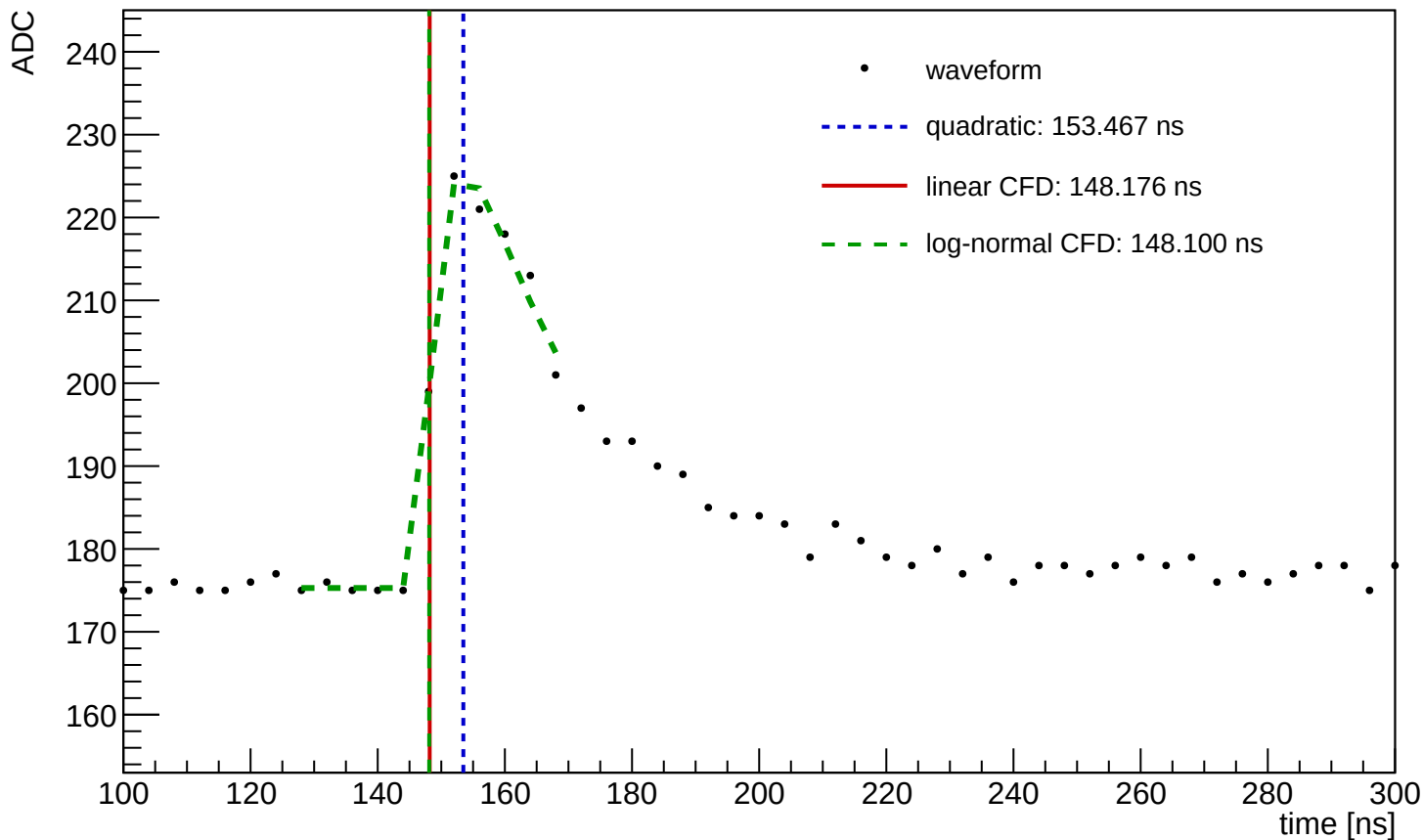
Waveform Time Demo (entry=1474, ch=13, module=1146, trigger=SUM)
