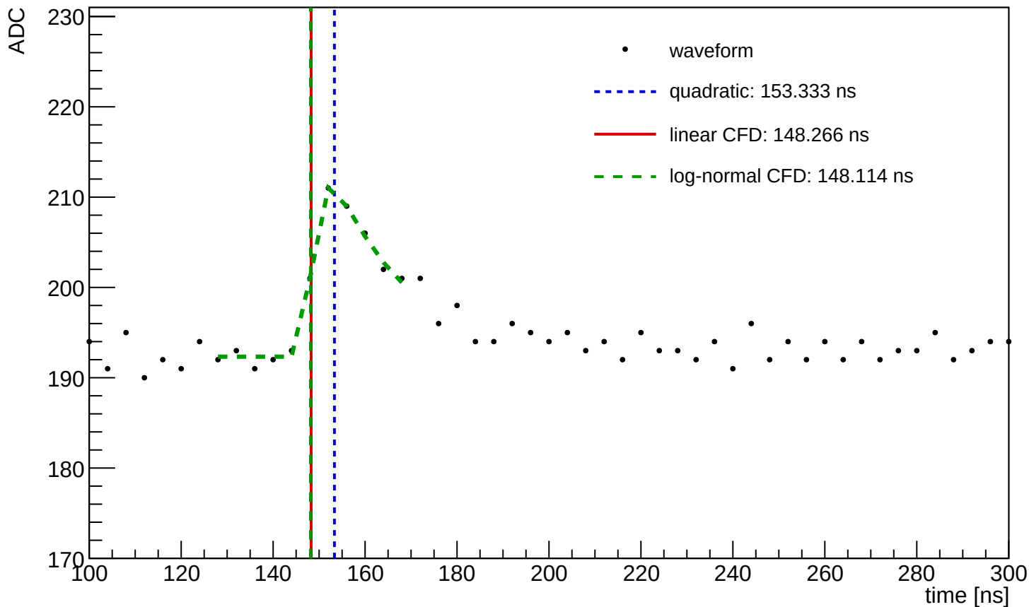
Waveform Time Demo (entry=463, ch=7, module=1018, trigger=SUM)
