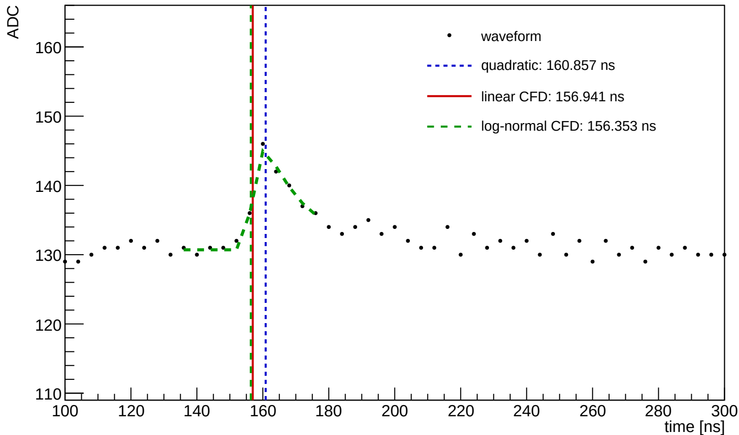
Waveform Time Demo (entry=32, ch=3, module=1093, trigger=SUM)
