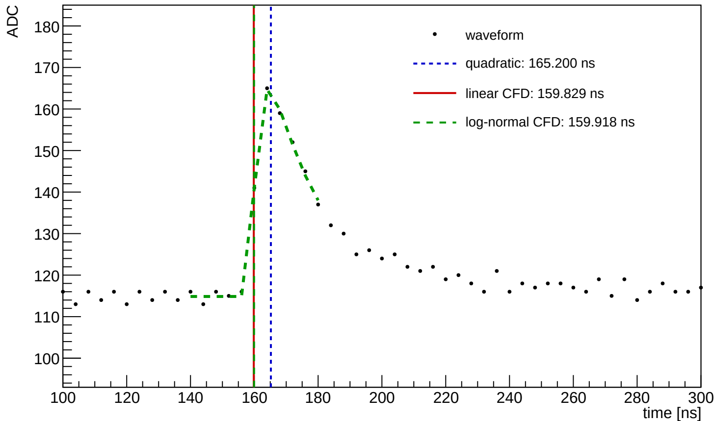
Waveform Time Demo (entry=1013, ch=3, module=1079, trigger=SUM)
