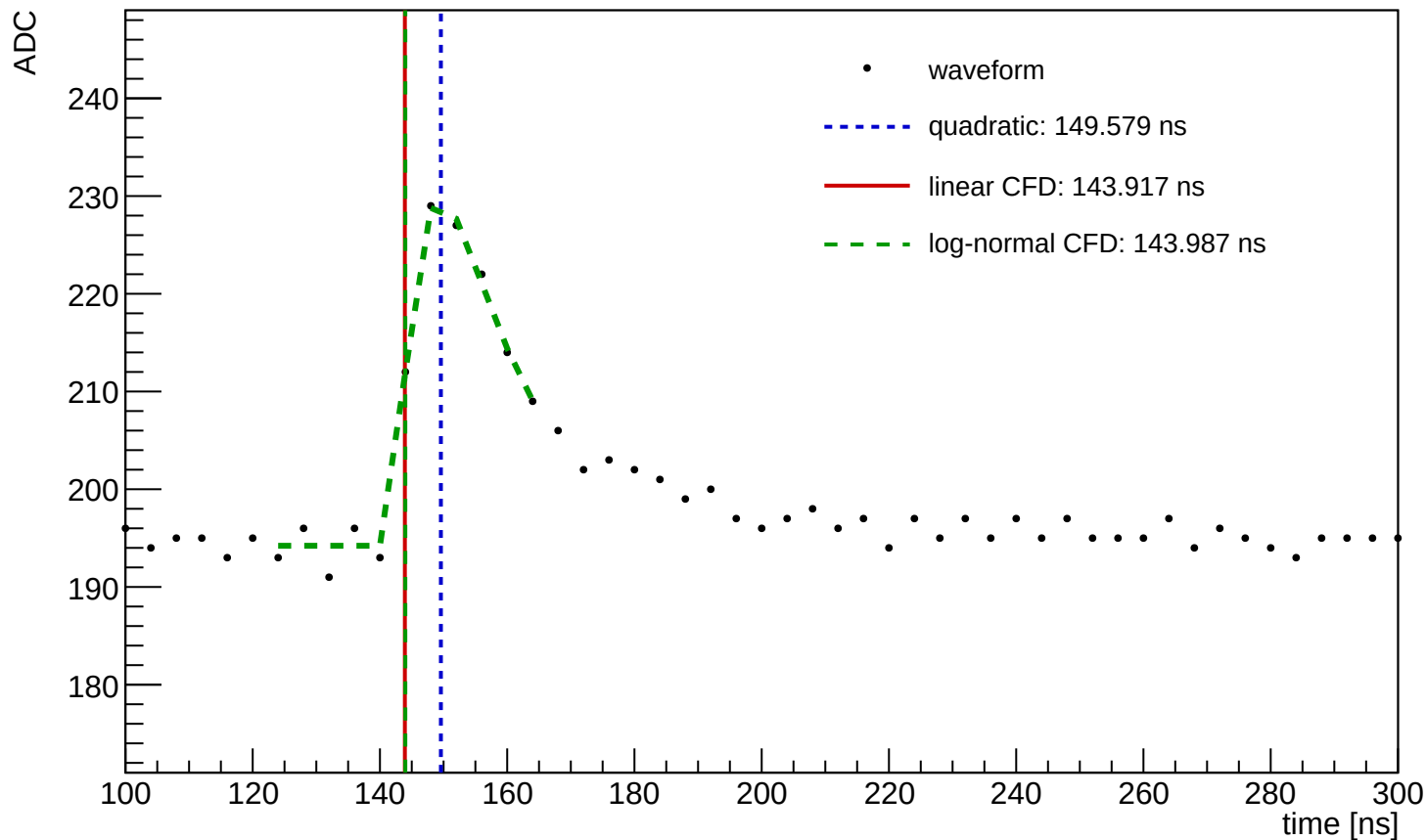
Waveform Time Demo (entry=58, ch=6, module=1052, trigger=SUM)
