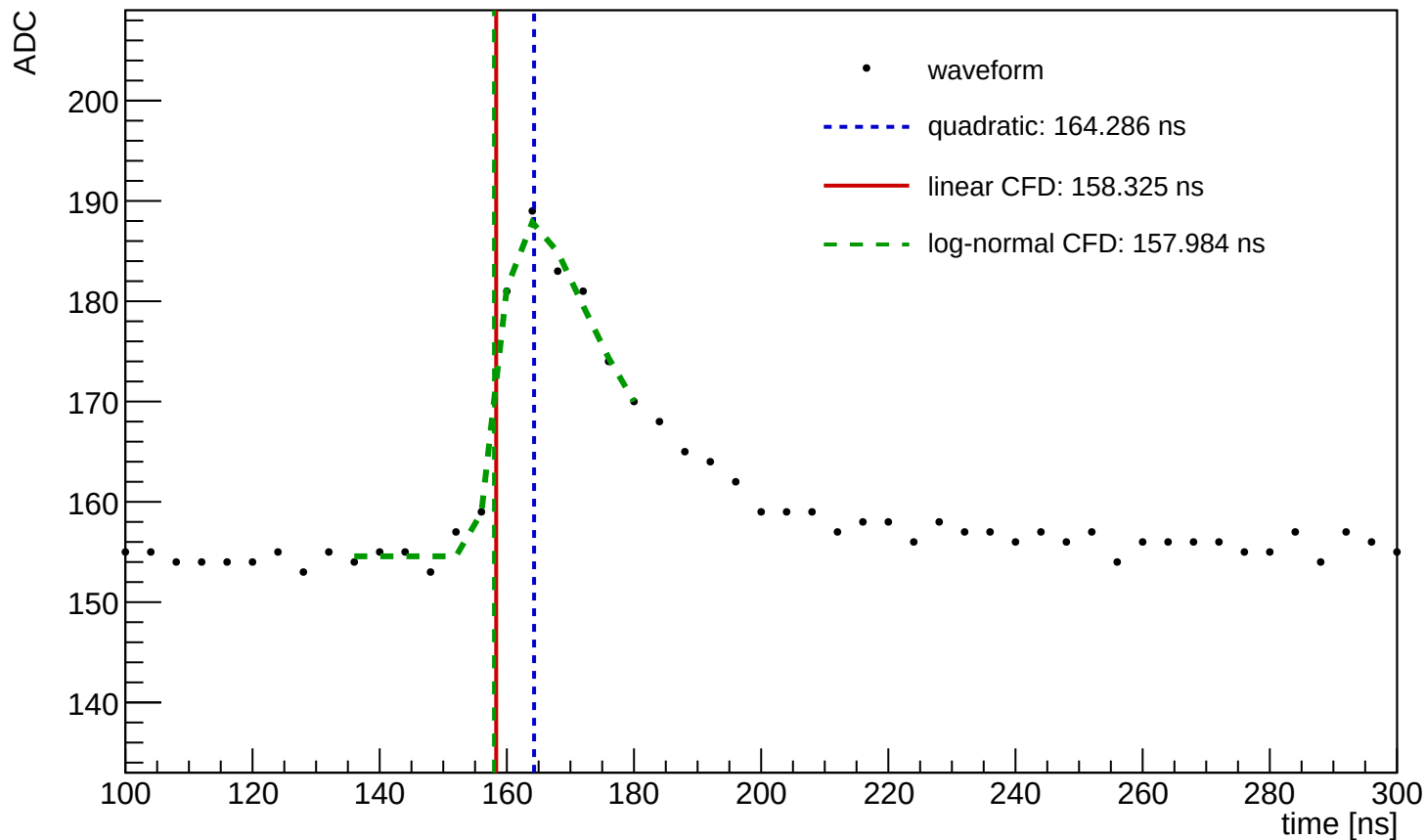
Waveform Time Demo (entry=691, ch=1, module=1113, trigger=SUM)
