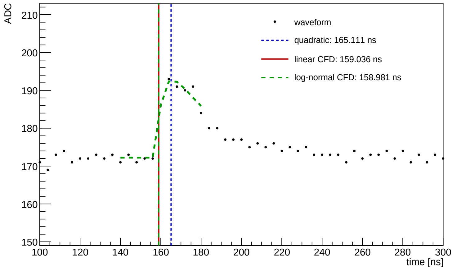
Waveform Time Demo (entry=32, ch=5, module=1092, trigger=SUM)
