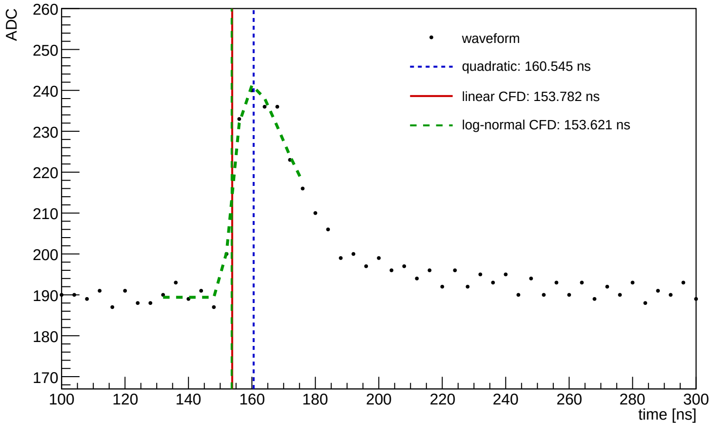
Waveform Time Demo (entry=1353, ch=9, module=1015, trigger=SUM)
