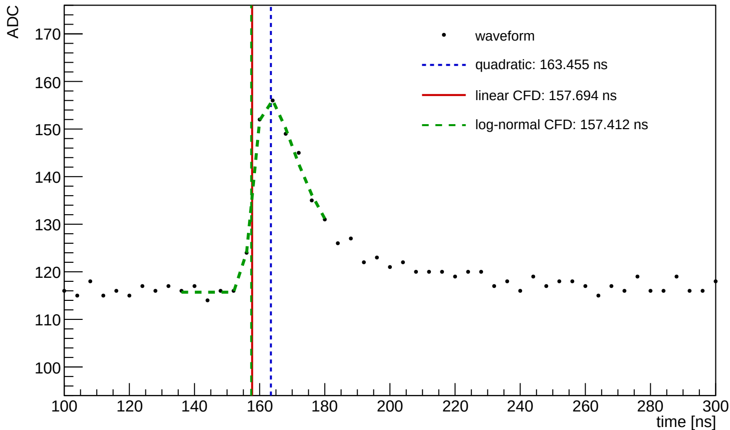
Waveform Time Demo (entry=1013, ch=2, module=1080, trigger=SUM)
