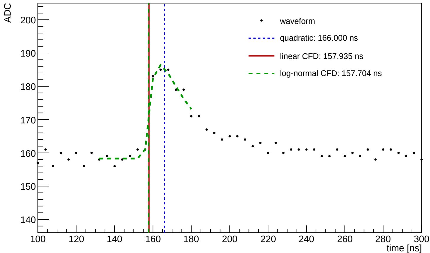
Waveform Time Demo (entry=1127, ch=1, module=1048, trigger=SUM)
