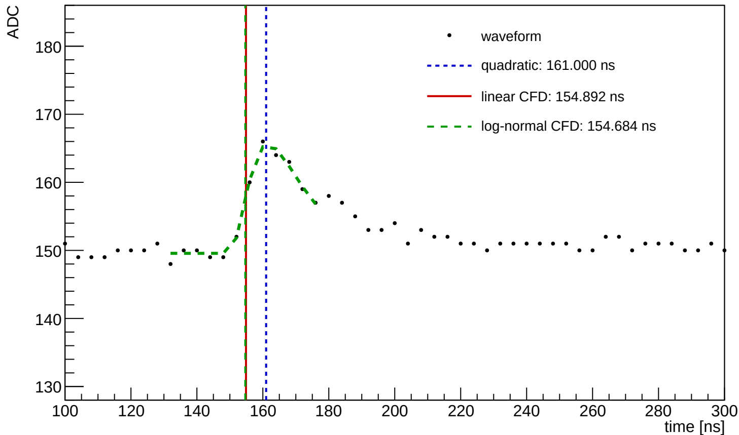
Waveform Time Demo (entry=627, ch=11, module=1153, trigger=SUM)
