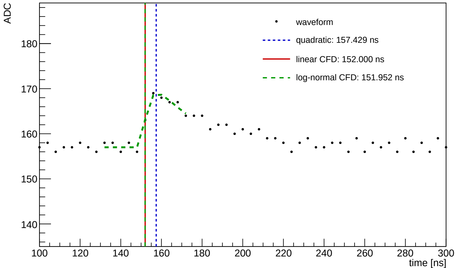
Waveform Time Demo (entry=1135, ch=13, module=1118, trigger=SUM)
