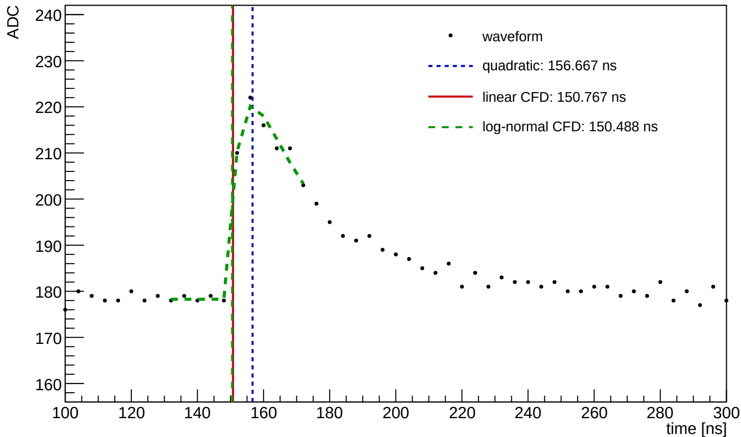
Waveform Time Demo (entry=644, ch=11, module=1152, trigger=SUM)
