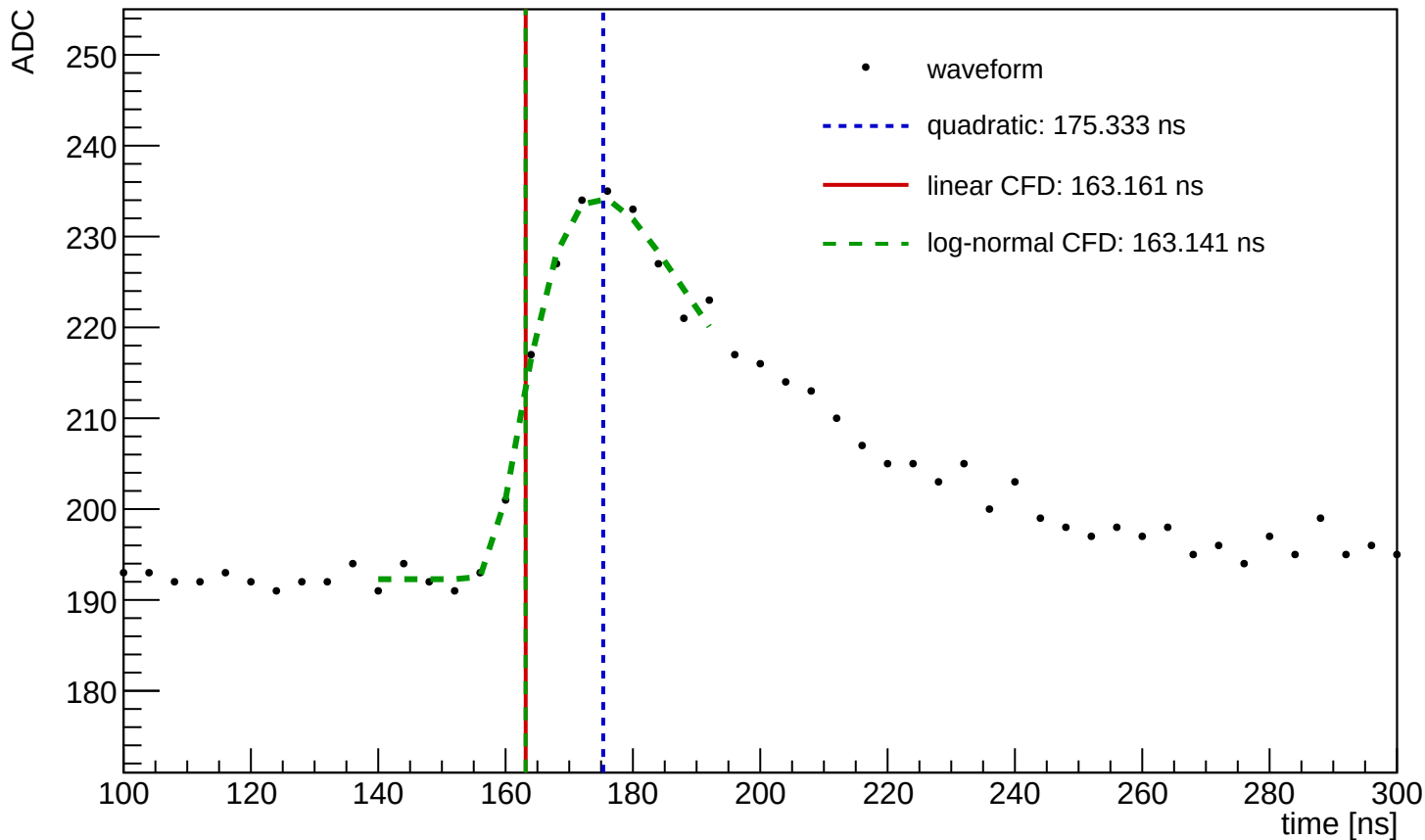
Waveform Time Demo (entry=1186, ch=675, module=1018, trigger=LMS)
