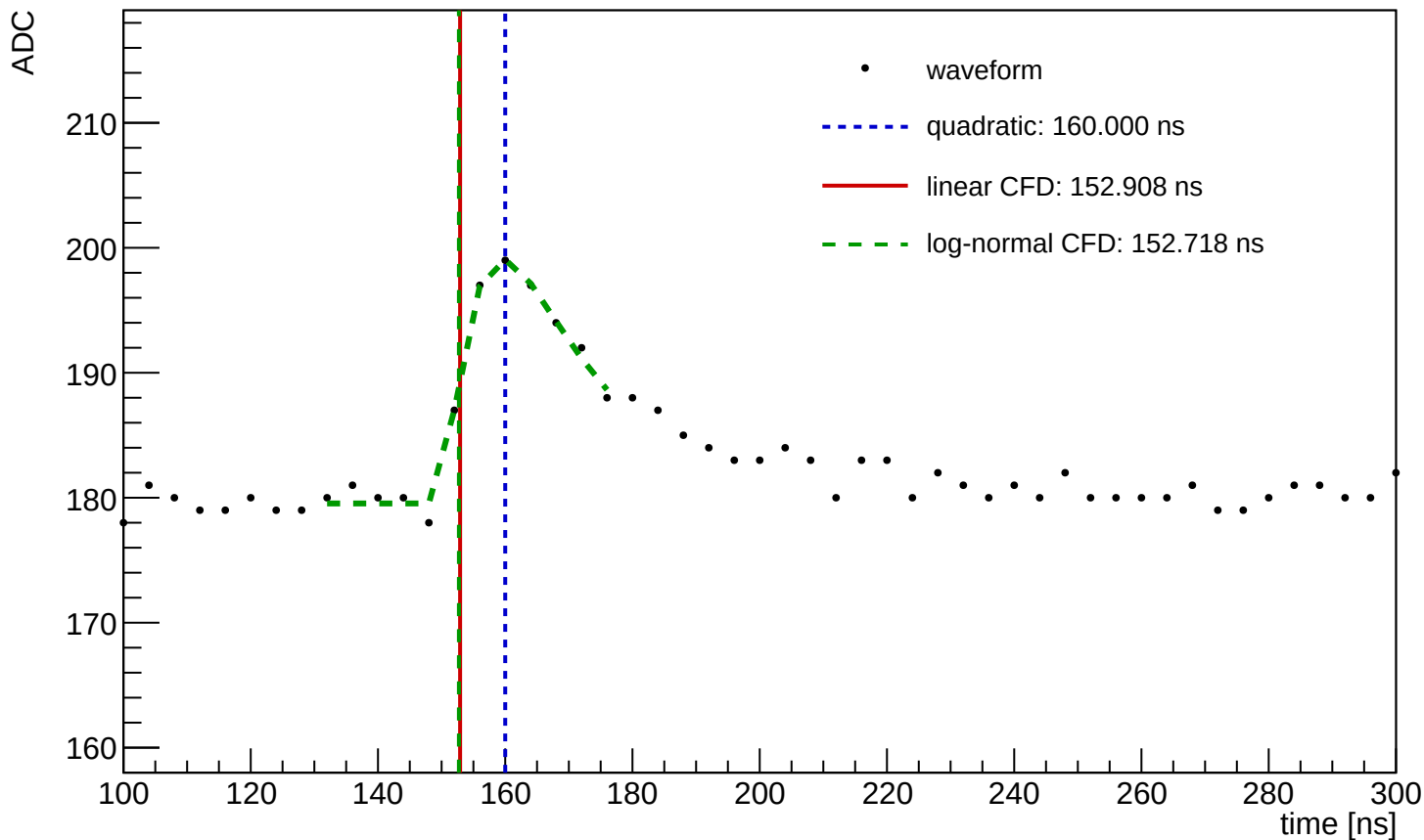
Waveform Time Demo (entry=43, ch=25, module=1089, trigger=SUM)
