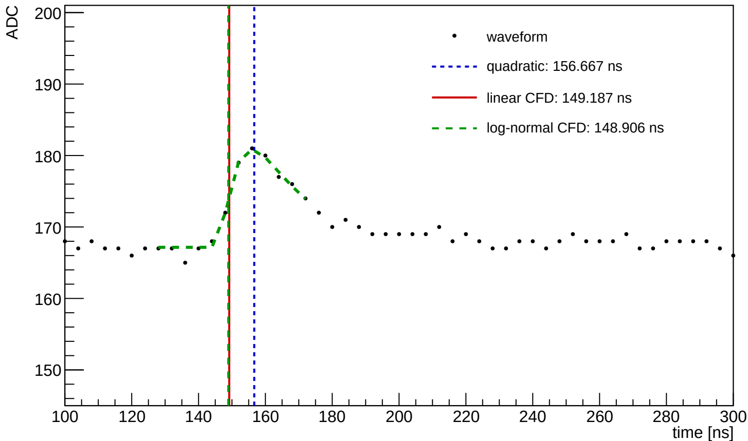
Waveform Time Demo (entry=230, ch=18, module=1126, trigger=SUM)
