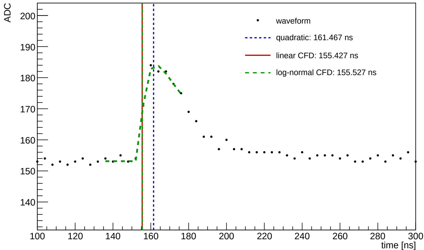
Waveform Time Demo (entry=15, ch=1, module=1114, trigger=SUM)
