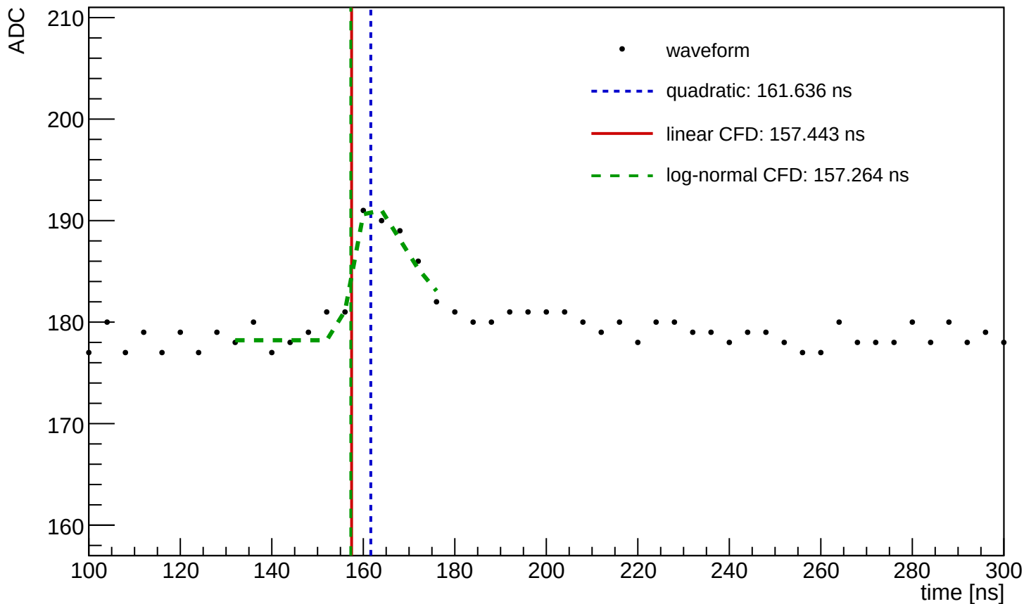
Waveform Time Demo (entry=1127, ch=4, module=1152, trigger=SUM)
