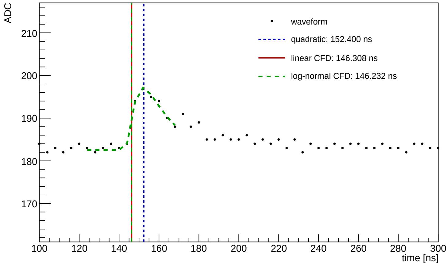
Waveform Time Demo (entry=1438, ch=18, module=1095, trigger=SUM)
