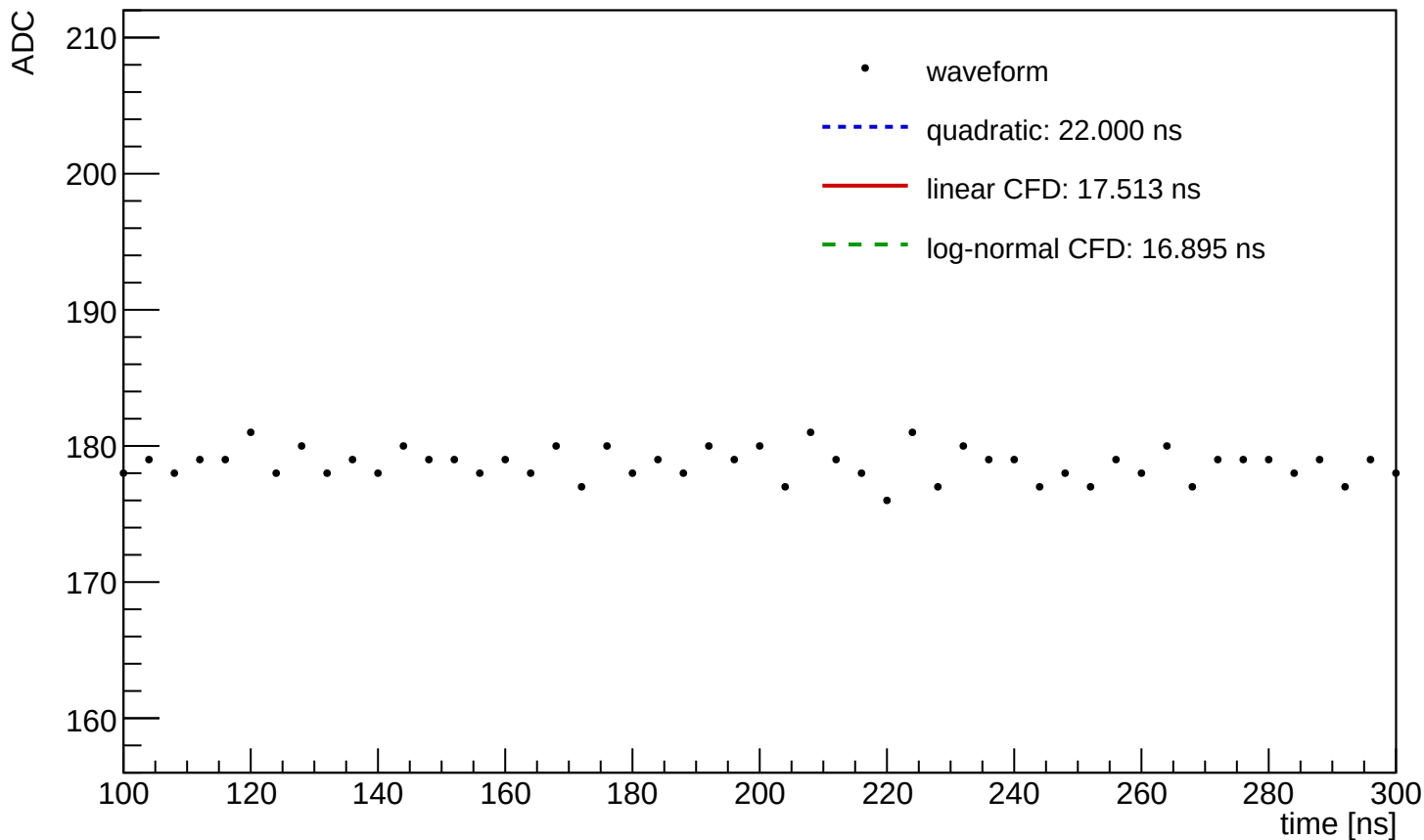
Waveform Time Demo (entry=574, ch=17, module=1152, trigger=SUM)
