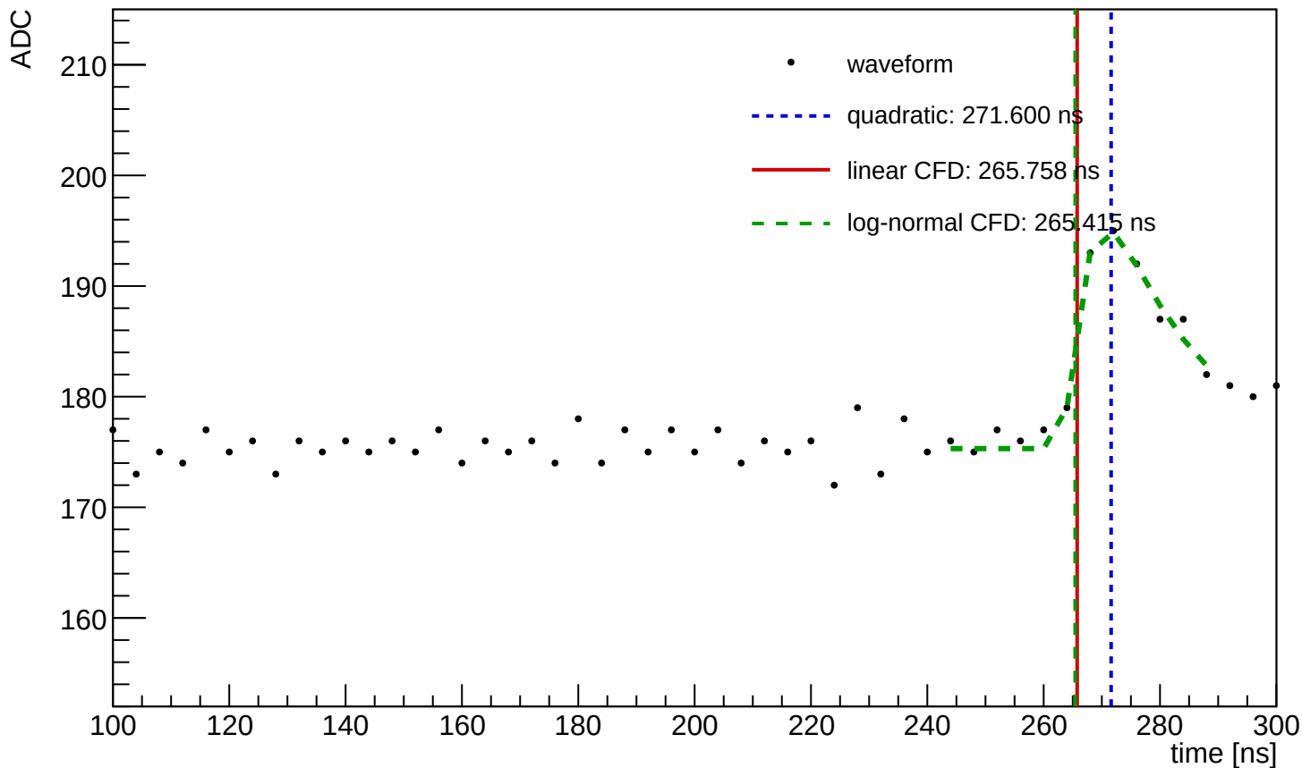
Waveform Time Demo (entry=319, ch=5, module=1146, trigger=SUM)
