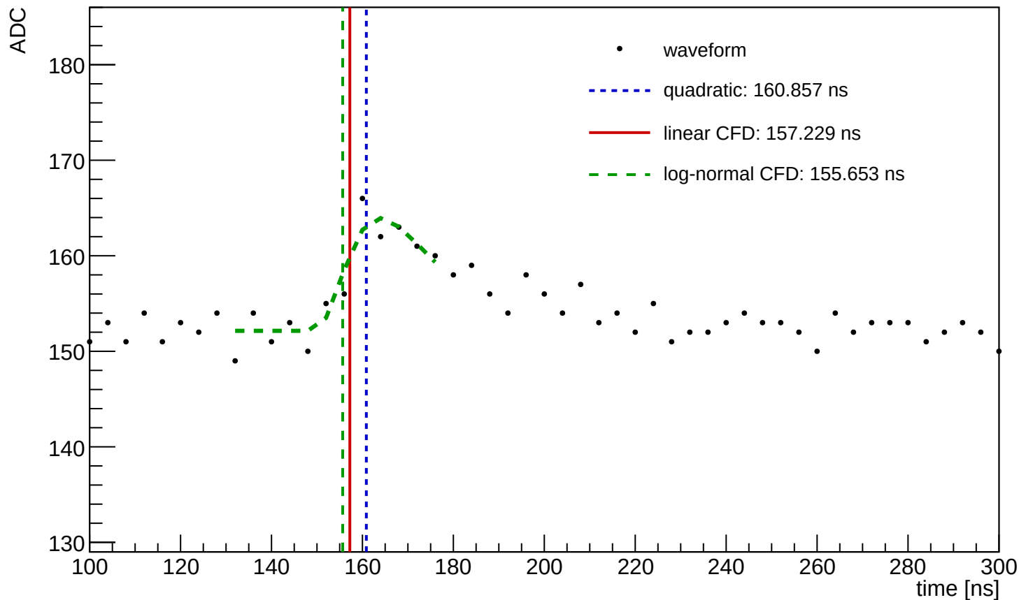
Waveform Time Demo (entry=105, ch=8, module=1119, trigger=SUM)
