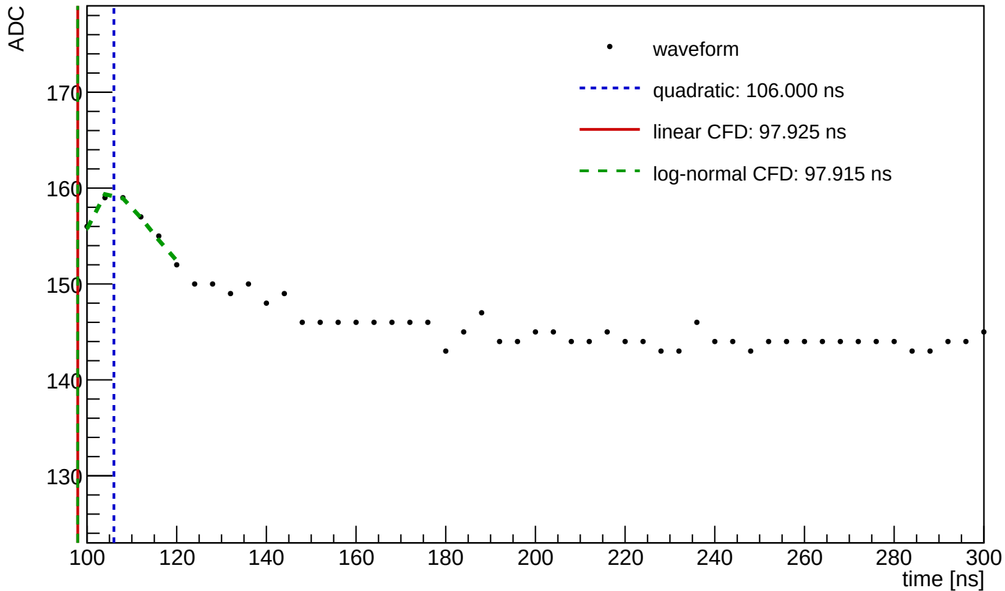
Waveform Time Demo (entry=344, ch=23, module=1122, trigger=SUM)
