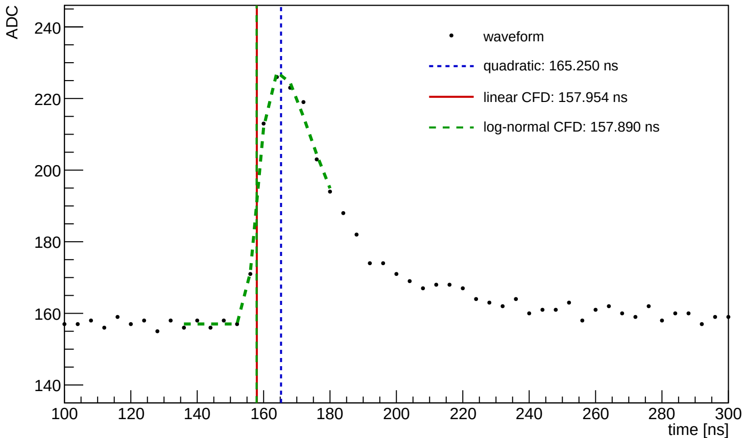
Waveform Time Demo (entry=317, ch=13, module=1118, trigger=SUM)
