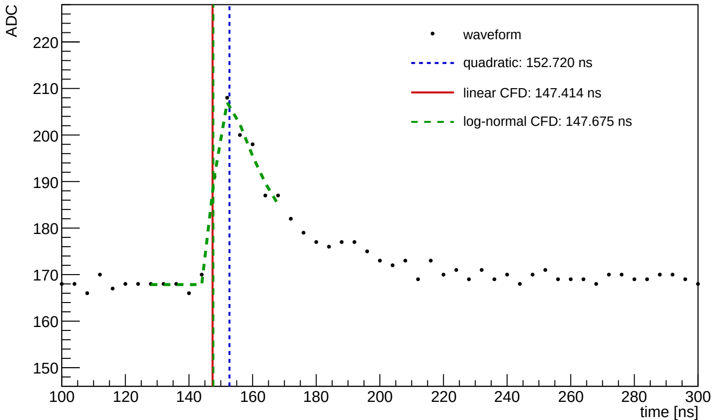
Waveform Time Demo (entry=1331, ch=13, module=1120, trigger=SUM)
