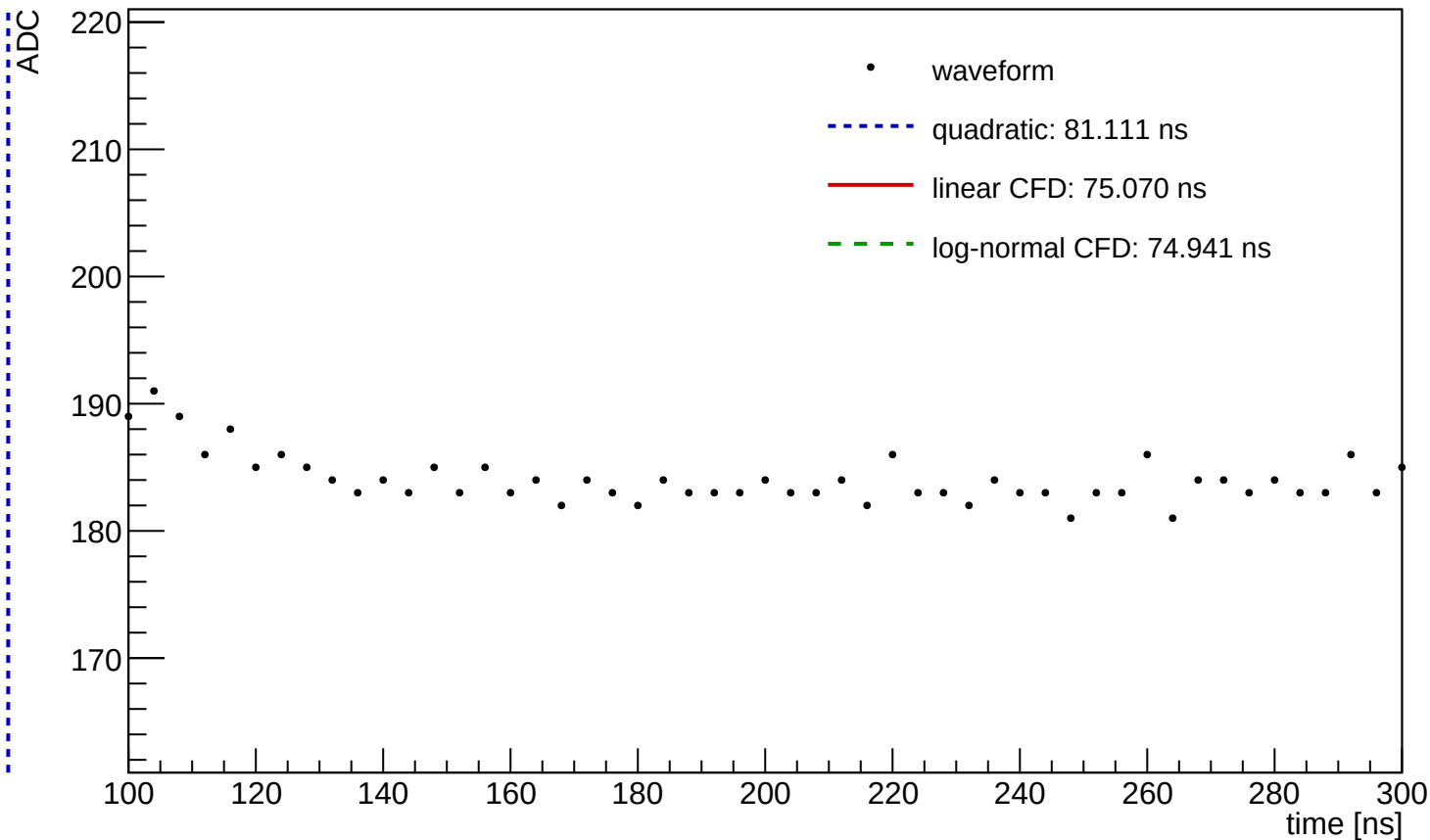
Waveform Time Demo (entry=866, ch=0, module=1076, trigger=SUM)
