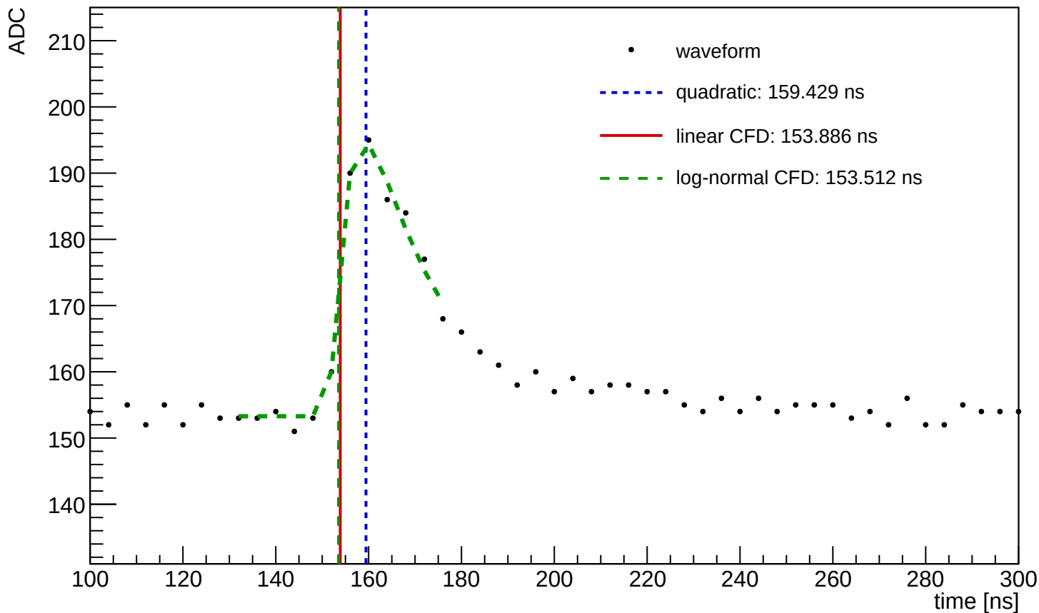
Waveform Time Demo (entry=1013, ch=0, module=1114, trigger=SUM)
