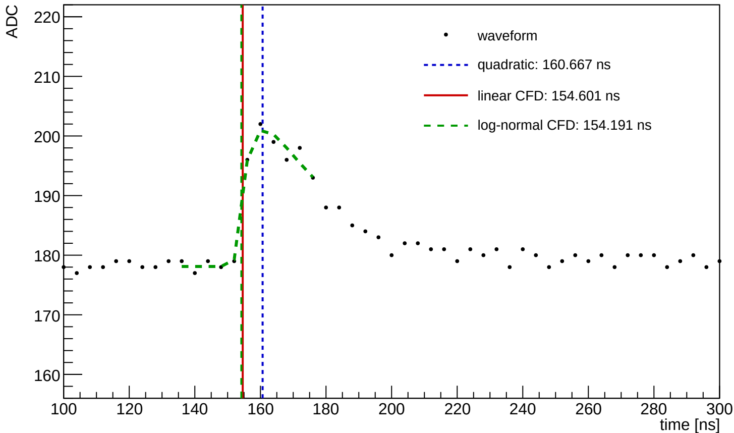
Waveform Time Demo (entry=1198, ch=11, module=1152, trigger=SUM)
