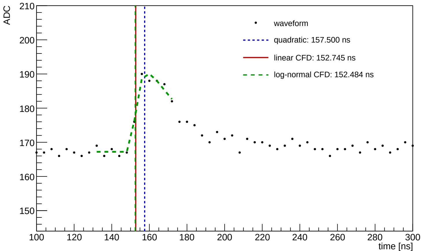
Waveform Time Demo (entry=317, ch=15, module=1151, trigger=SUM)
