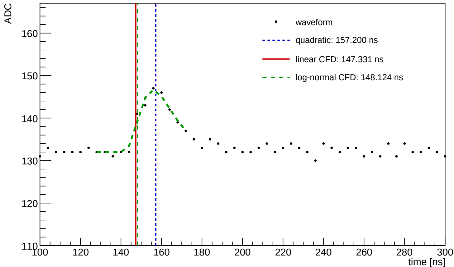
Waveform Time Demo (entry=59, ch=3, module=1071, trigger=SUM)
