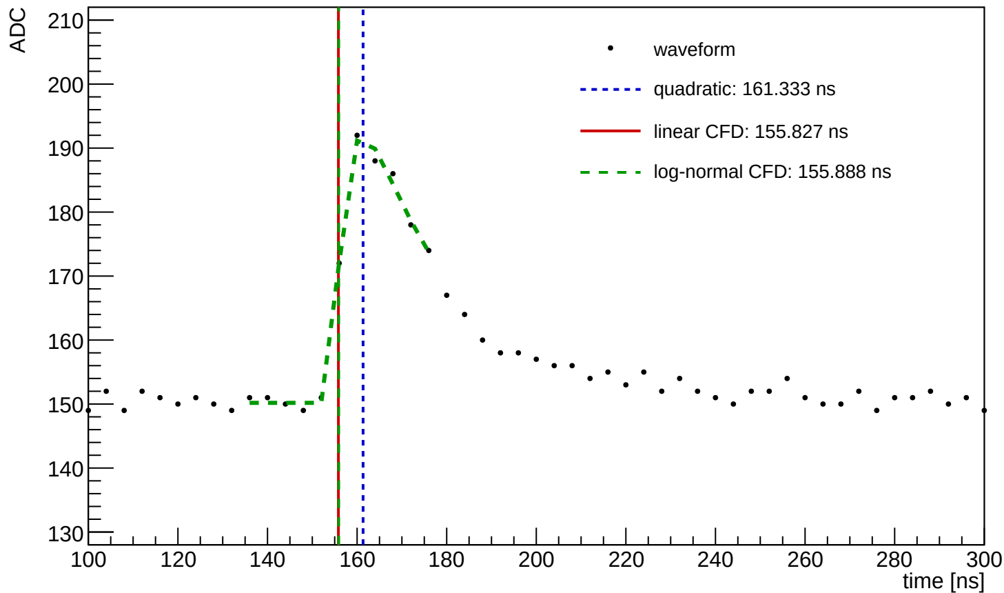
Waveform Time Demo (entry=1487, ch=9, module=1153, trigger=SUM)
