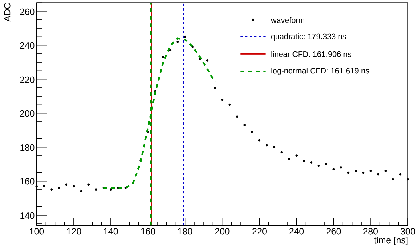
Waveform Time Demo (entry=1186, ch=669, module=1086, trigger=LMS)
