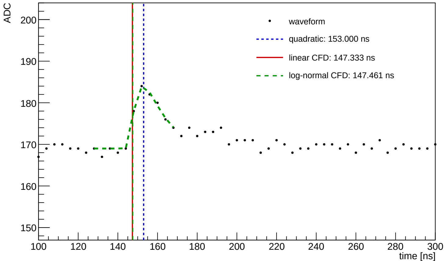
Waveform Time Demo (entry=1163, ch=28, module=1090, trigger=SUM)
