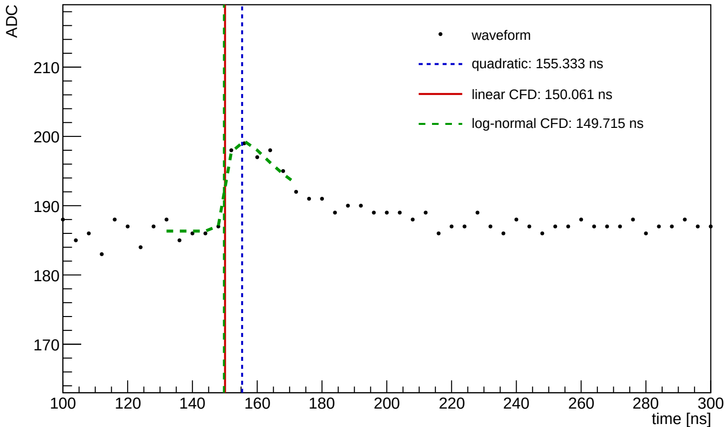
Waveform Time Demo (entry=540, ch=24, module=1024, trigger=SUM)
