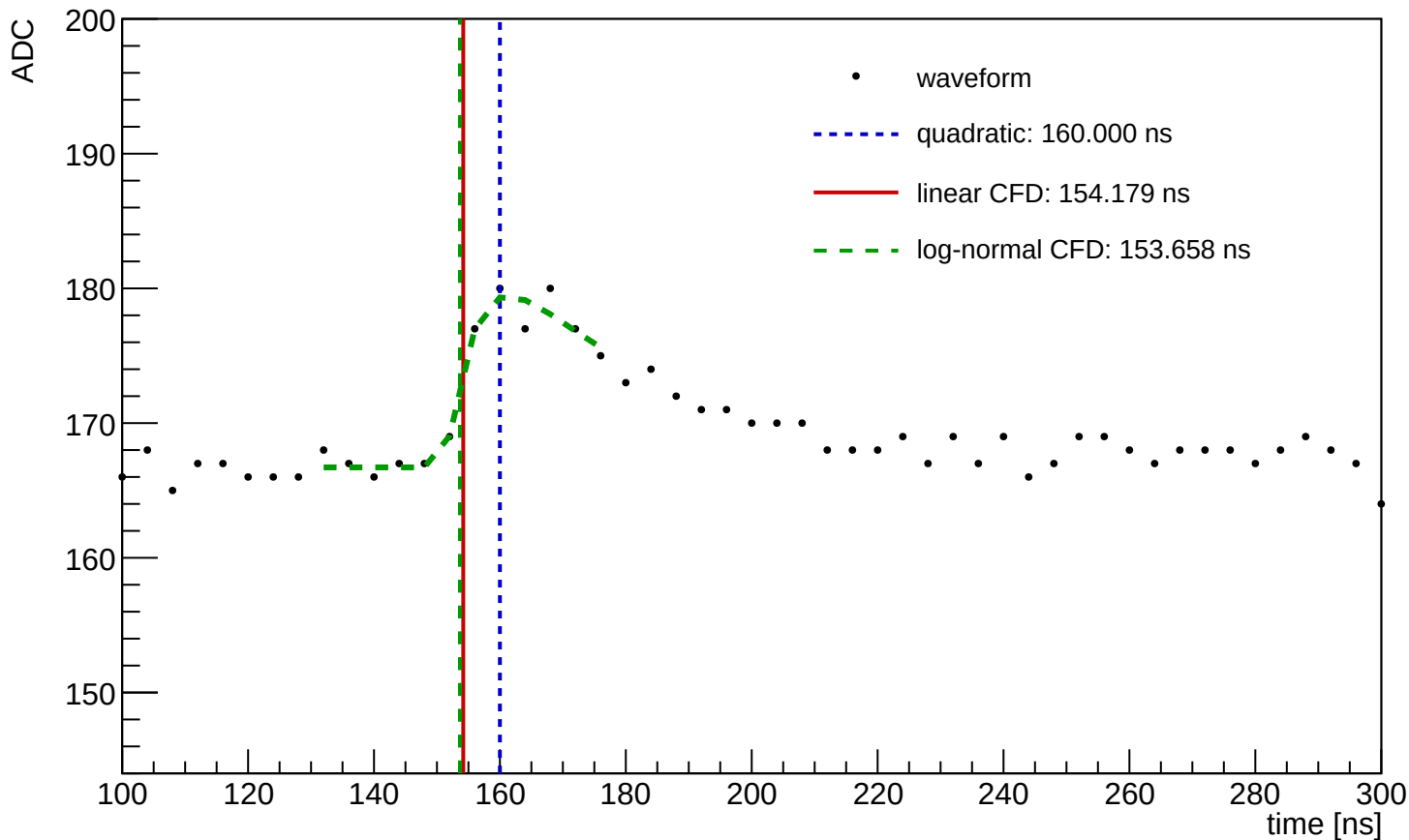
Waveform Time Demo (entry=410, ch=29, module=1098, trigger=SUM)
