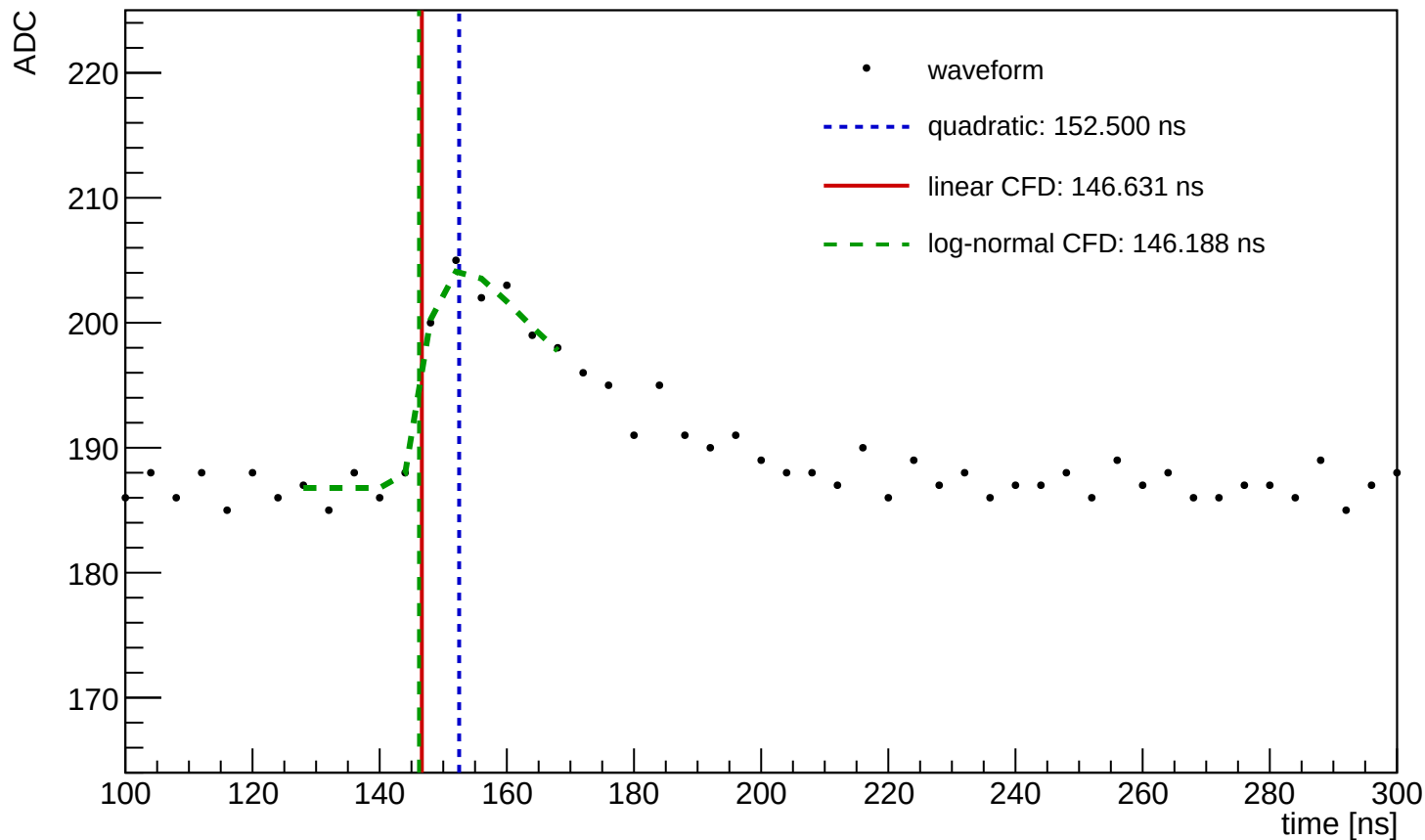
Waveform Time Demo (entry=1294, ch=0, module=1035, trigger=SUM)
