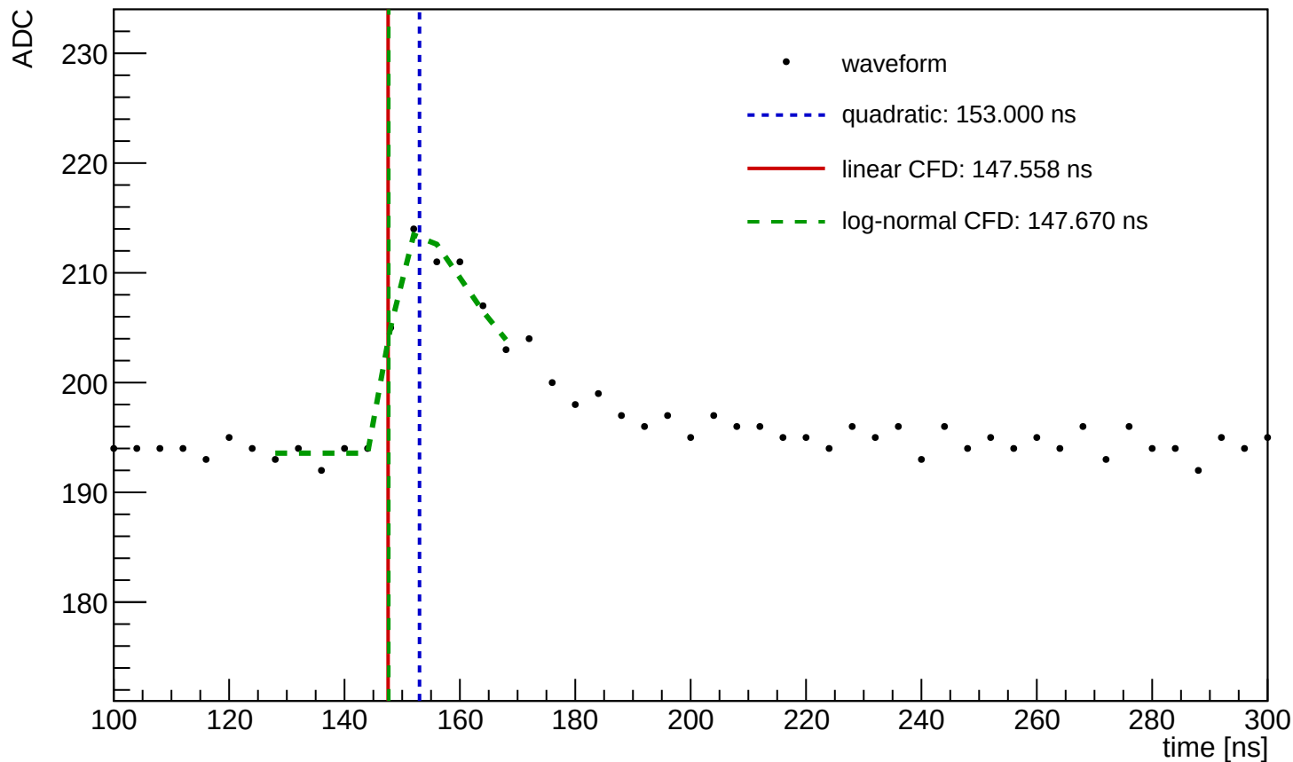
Waveform Time Demo (entry=1474, ch=27, module=1034, trigger=SUM)
