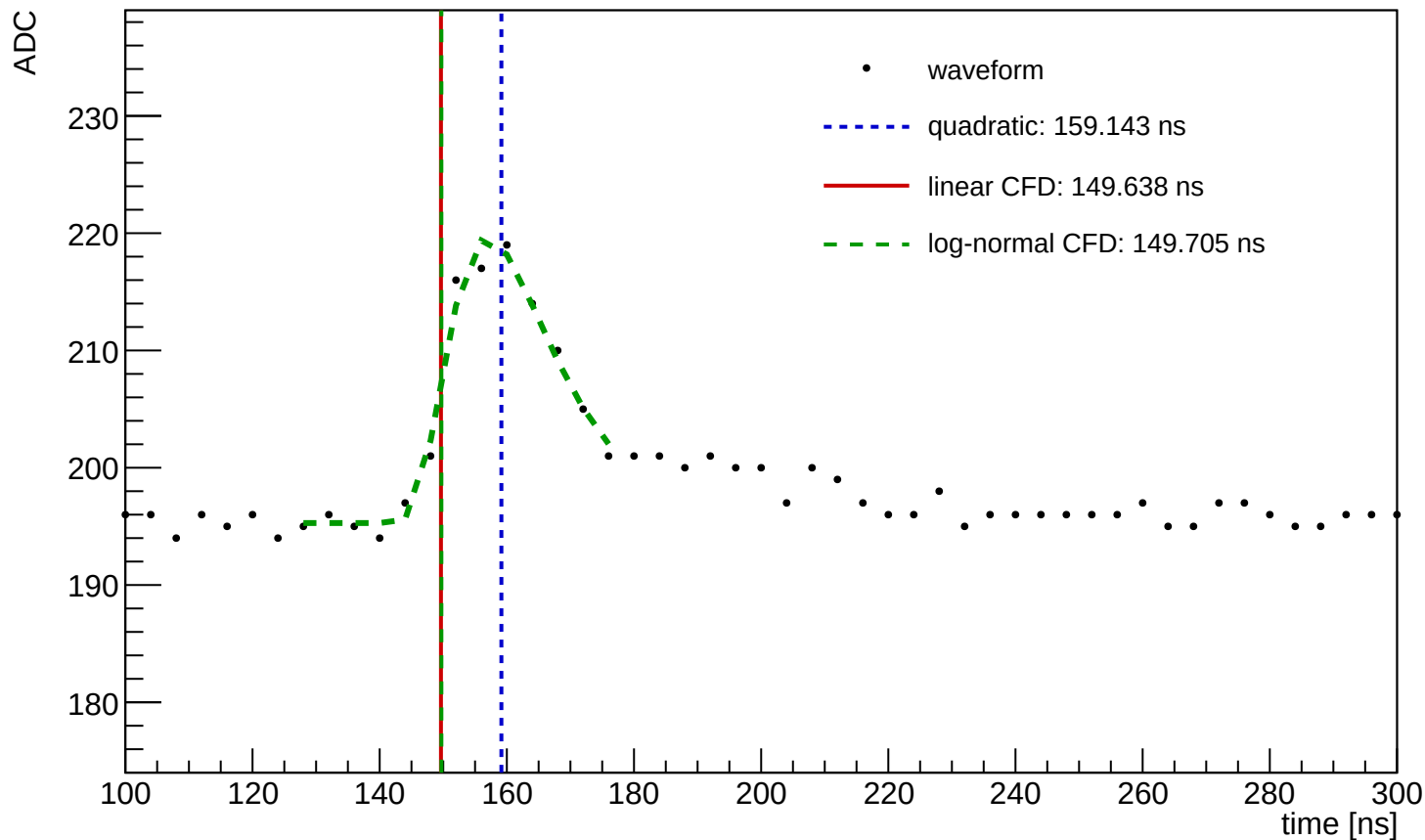
Waveform Time Demo (entry=16, ch=1, module=1150, trigger=SUM)
