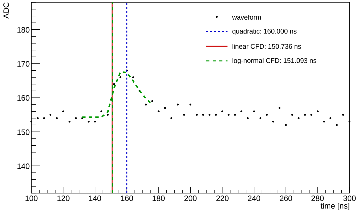
Waveform Time Demo (entry=1135, ch=5, module=1113, trigger=SUM)
