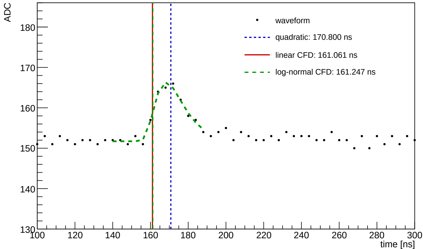
Waveform Time Demo (entry=1487, ch=10, module=1119, trigger=SUM)
