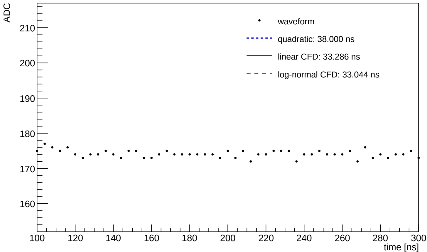
Waveform Time Demo (entry=671, ch=23, module=1026, trigger=SUM)
