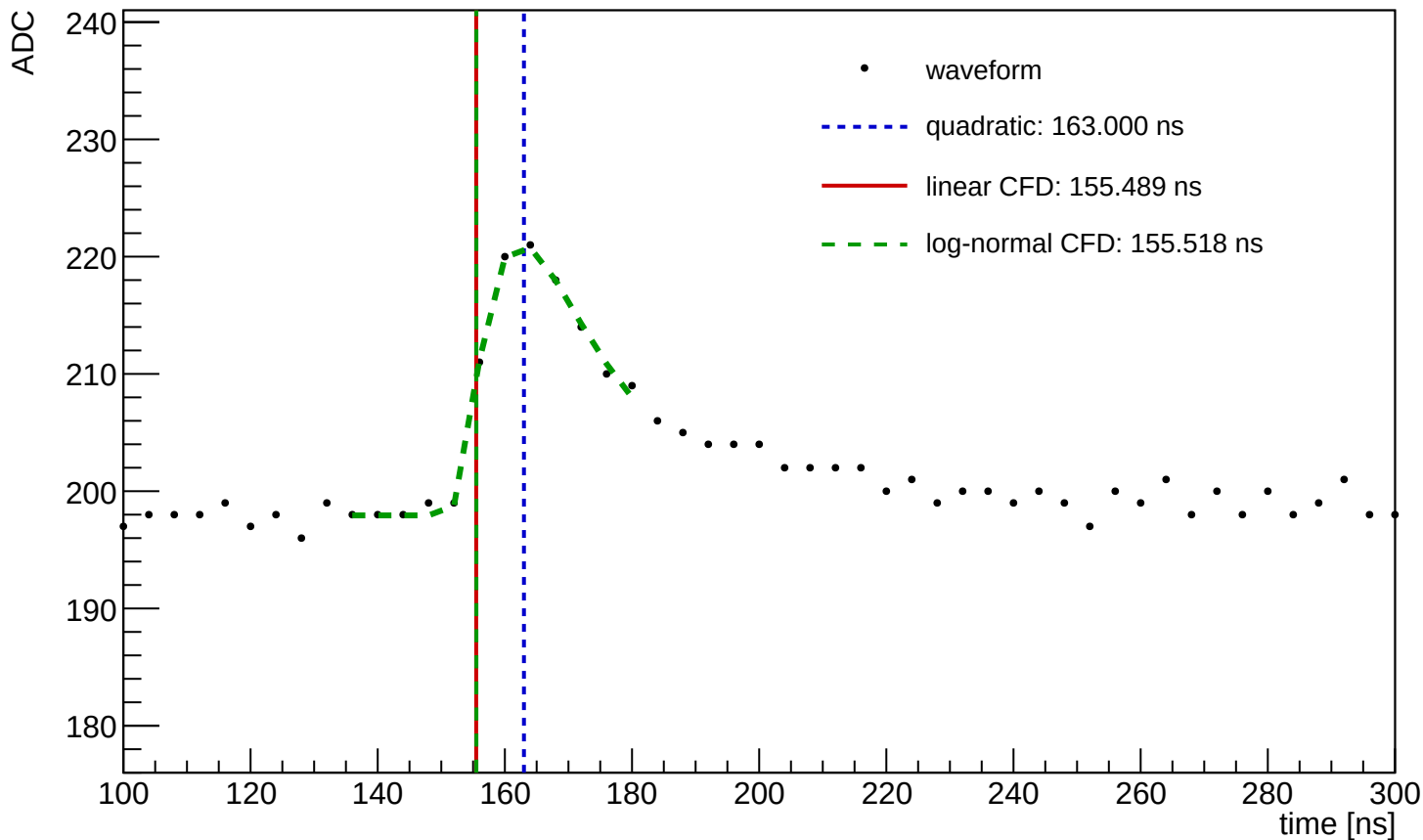
Waveform Time Demo (entry=200, ch=16, module=1055, trigger=SUM)
