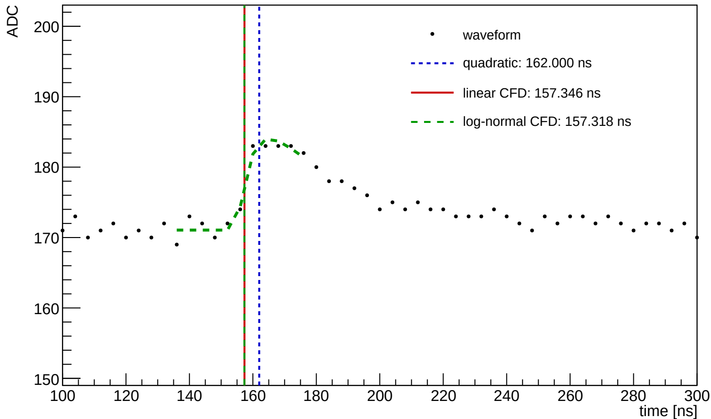
Waveform Time Demo (entry=192, ch=5, module=1017, trigger=SUM)
