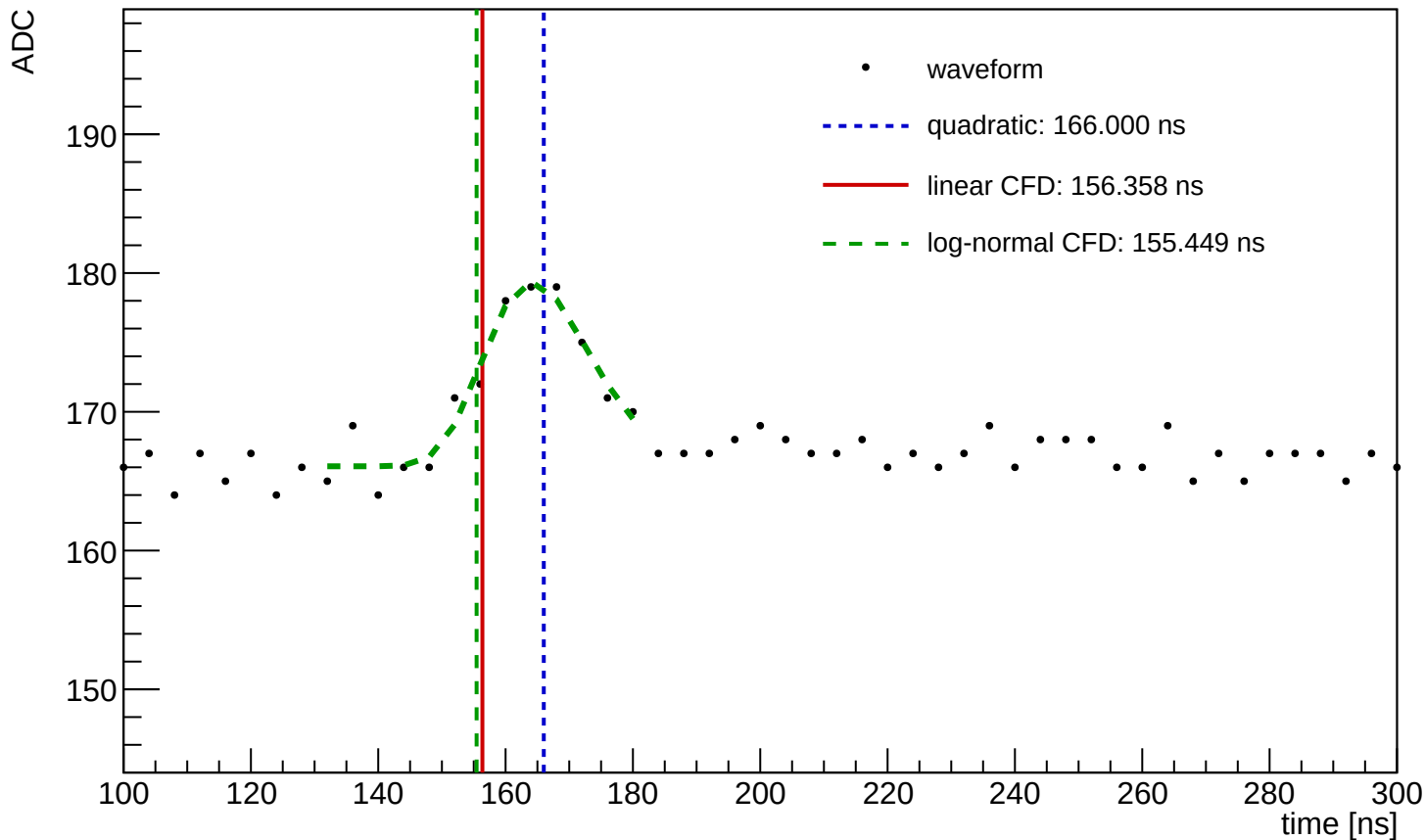
Waveform Time Demo (entry=1127, ch=10, module=1051, trigger=SUM)
