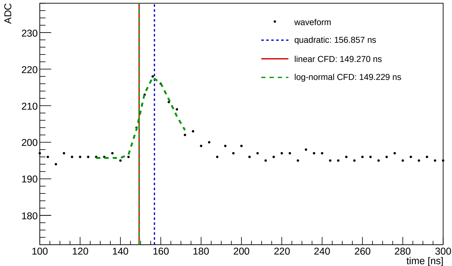
Waveform Time Demo (entry=37, ch=1, module=1150, trigger=SUM)
