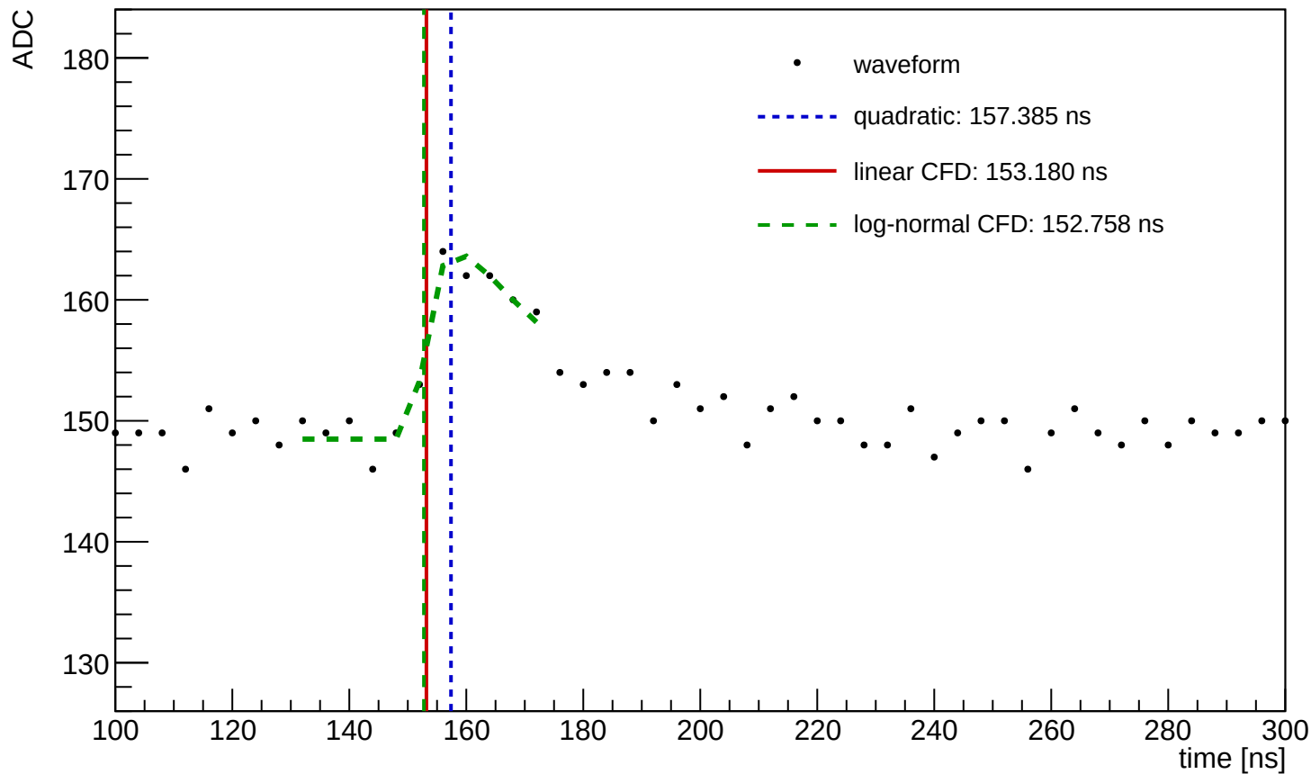
Waveform Time Demo (entry=317, ch=14, module=1117, trigger=SUM)
