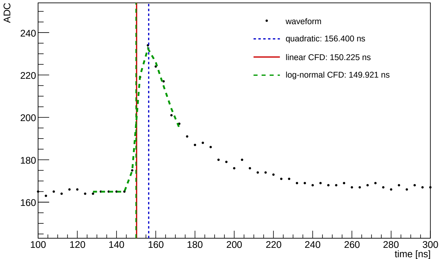
Waveform Time Demo (entry=200, ch=2, module=1088, trigger=SUM)
