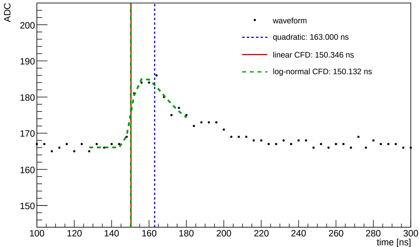
Waveform Time Demo (entry=59, ch=0, module=1141, trigger=SUM)
