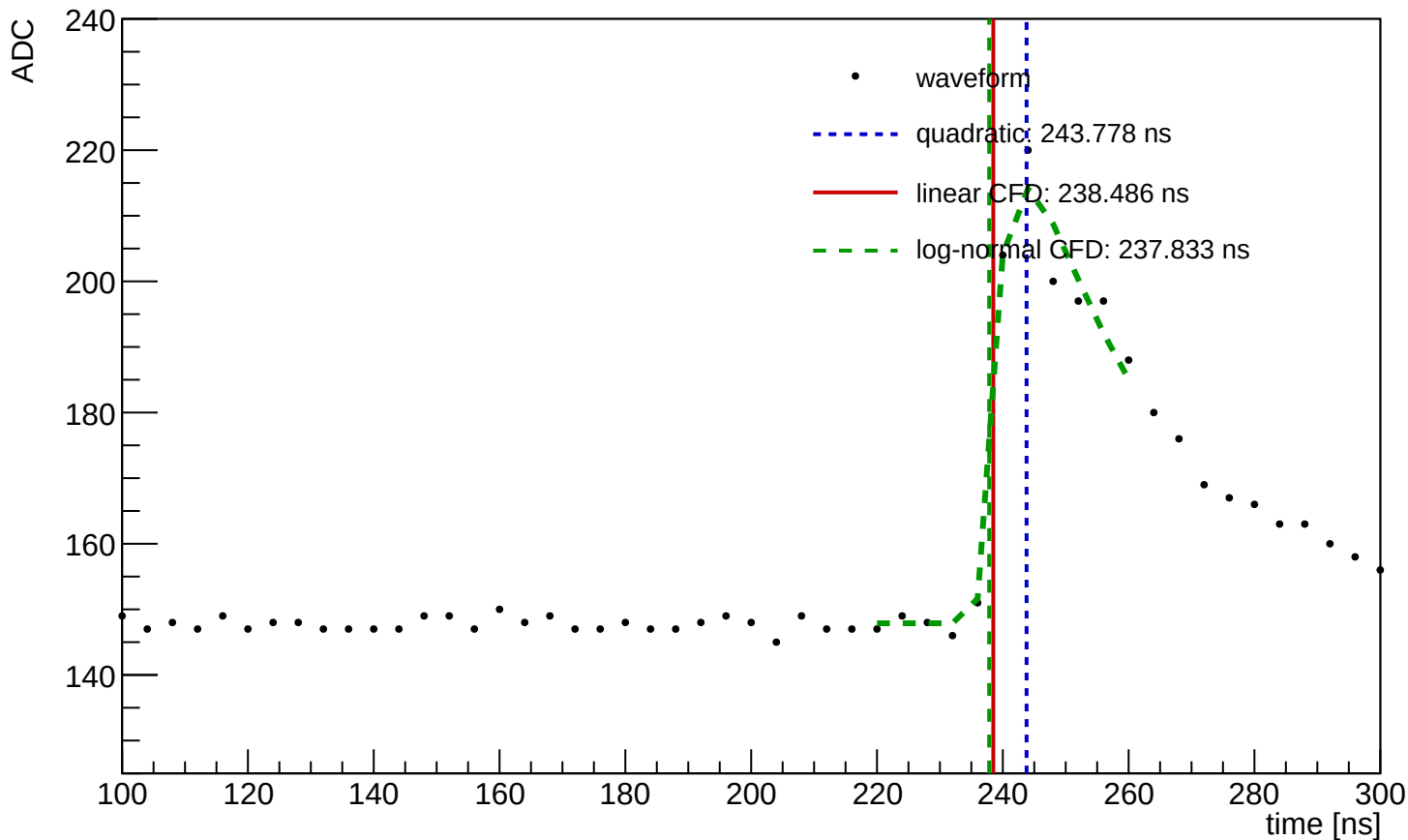
Waveform Time Demo (entry=465, ch=52, module=1124, trigger=SUM)
