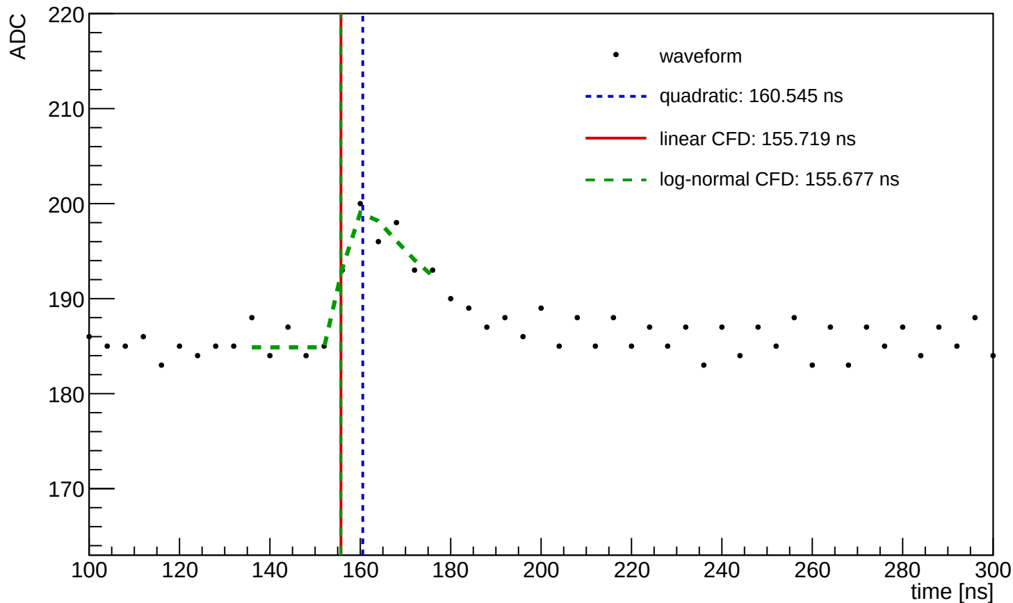
Waveform Time Demo (entry=1353, ch=10, module=1016, trigger=SUM)
