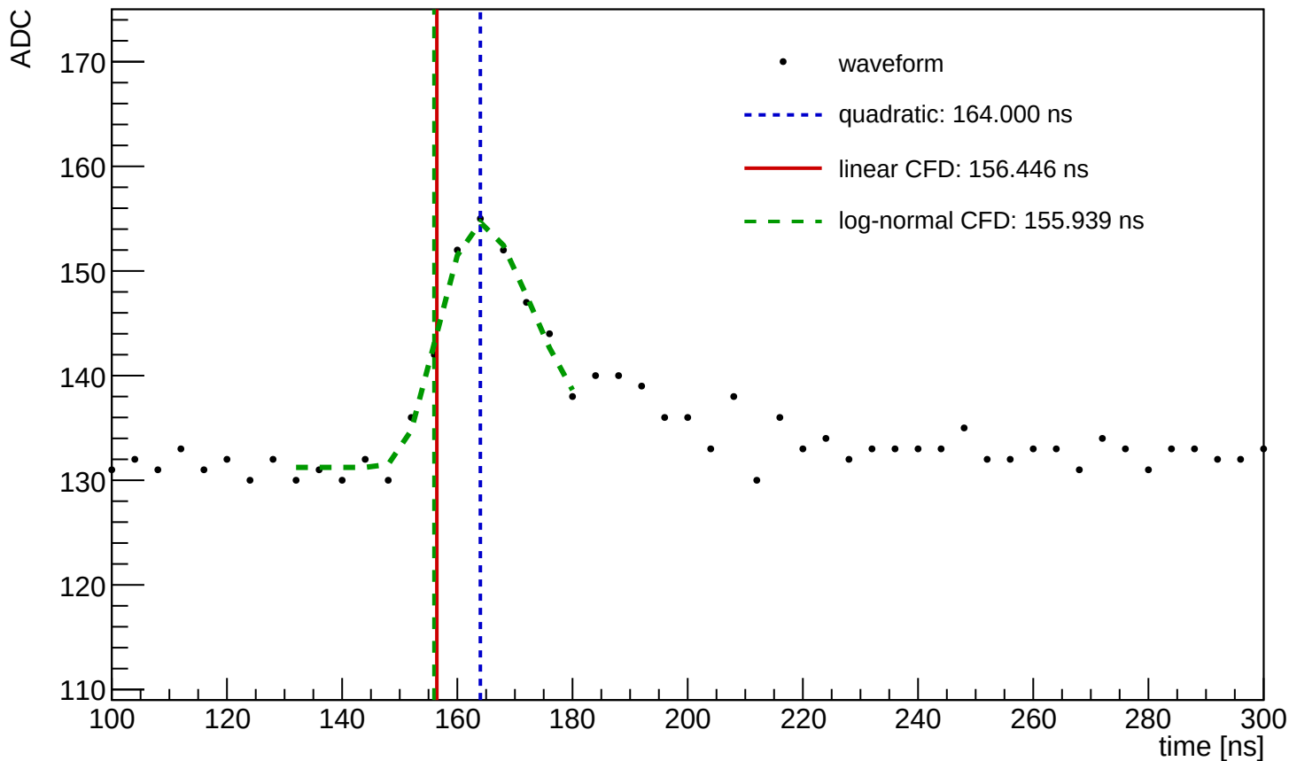
Waveform Time Demo (entry=889, ch=1, module=1010, trigger=SUM)
