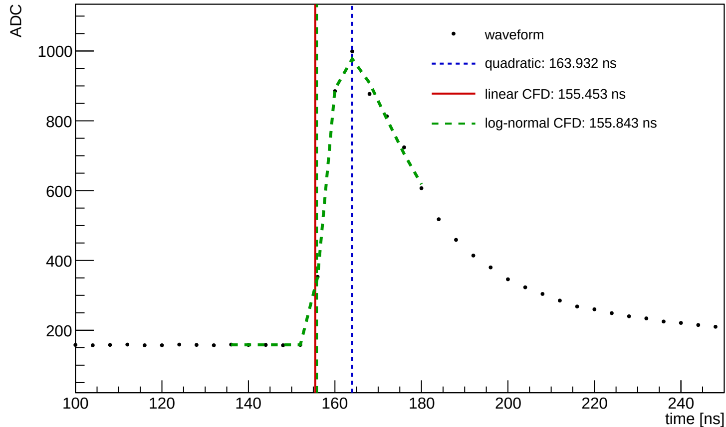
Waveform Time Demo (entry=30055, ch=15, module=1458, trigger=SUM)
