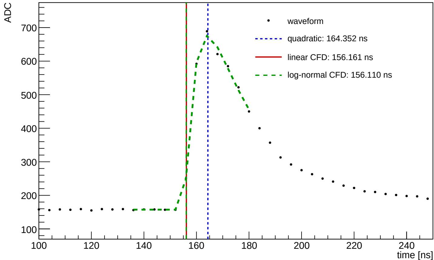
Waveform Time Demo (entry=65987, ch=11, module=1458, trigger=SUM)
