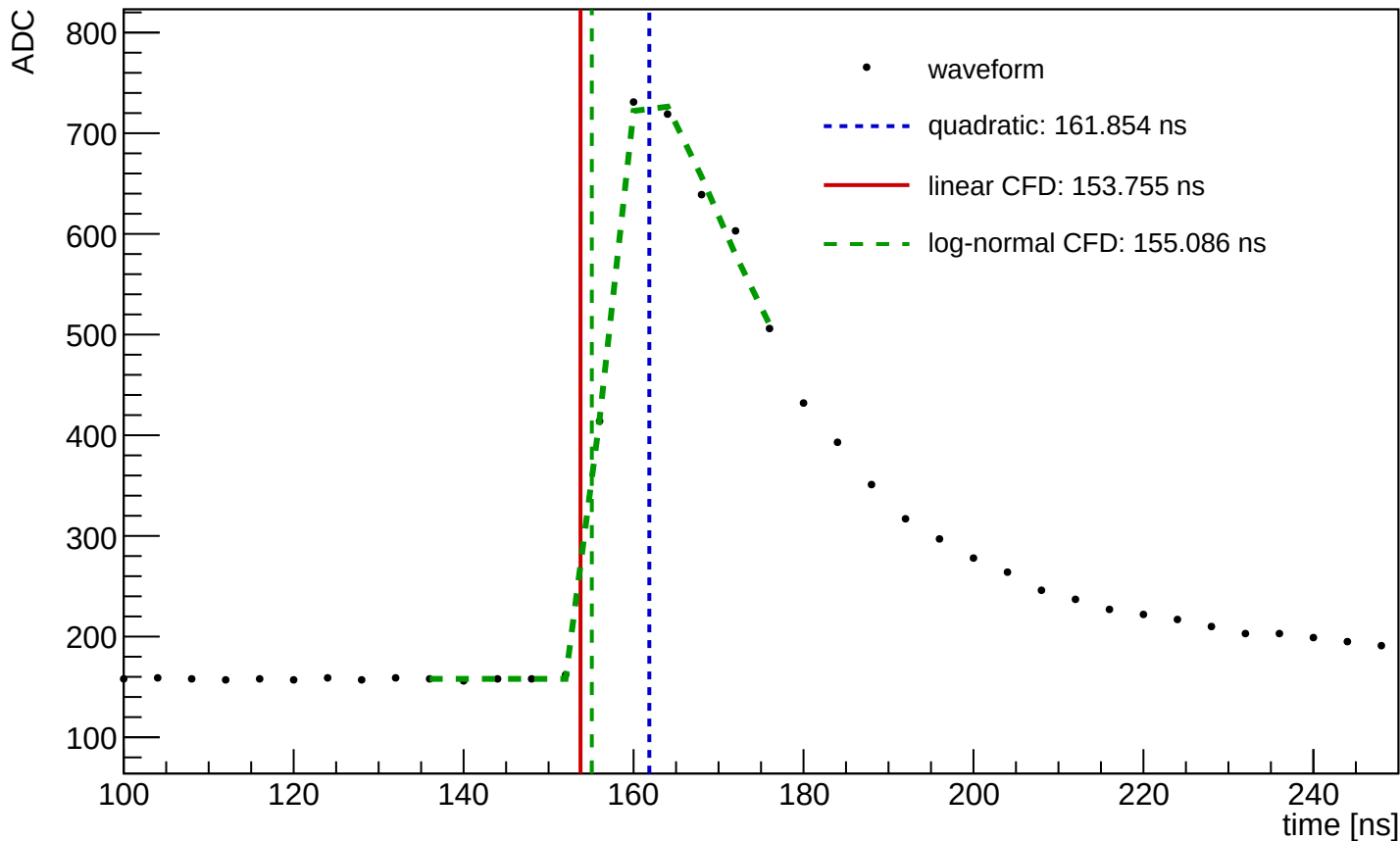
Waveform Time Demo (entry=16460, ch=7, module=1458, trigger=SUM)
