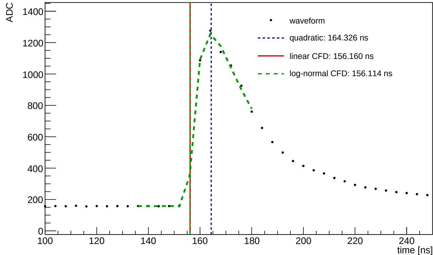
Waveform Time Demo (entry=36389, ch=13, module=1458, trigger=SUM)
