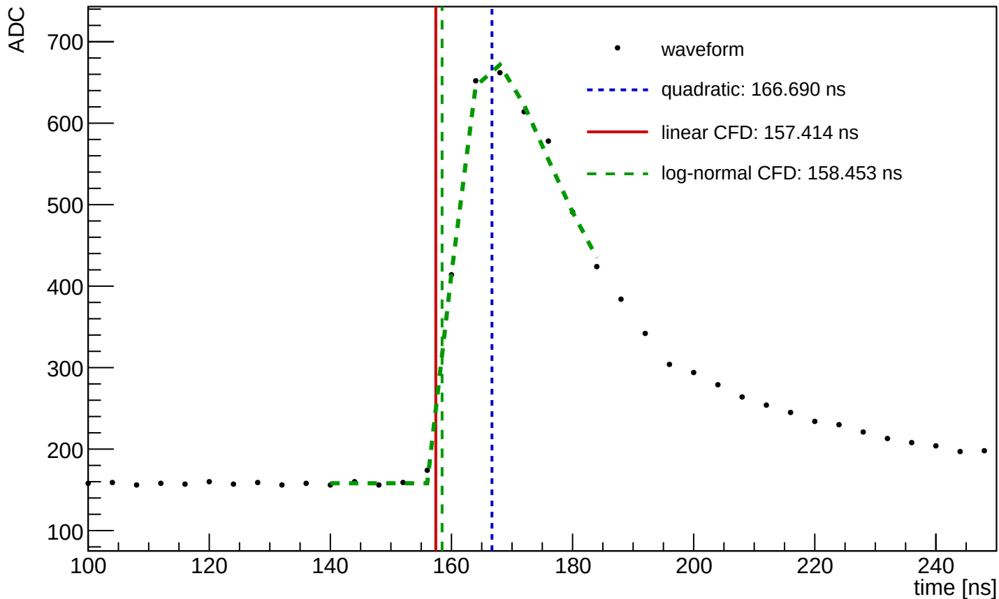
Waveform Time Demo (entry=33511, ch=7, module=1458, trigger=SUM)
