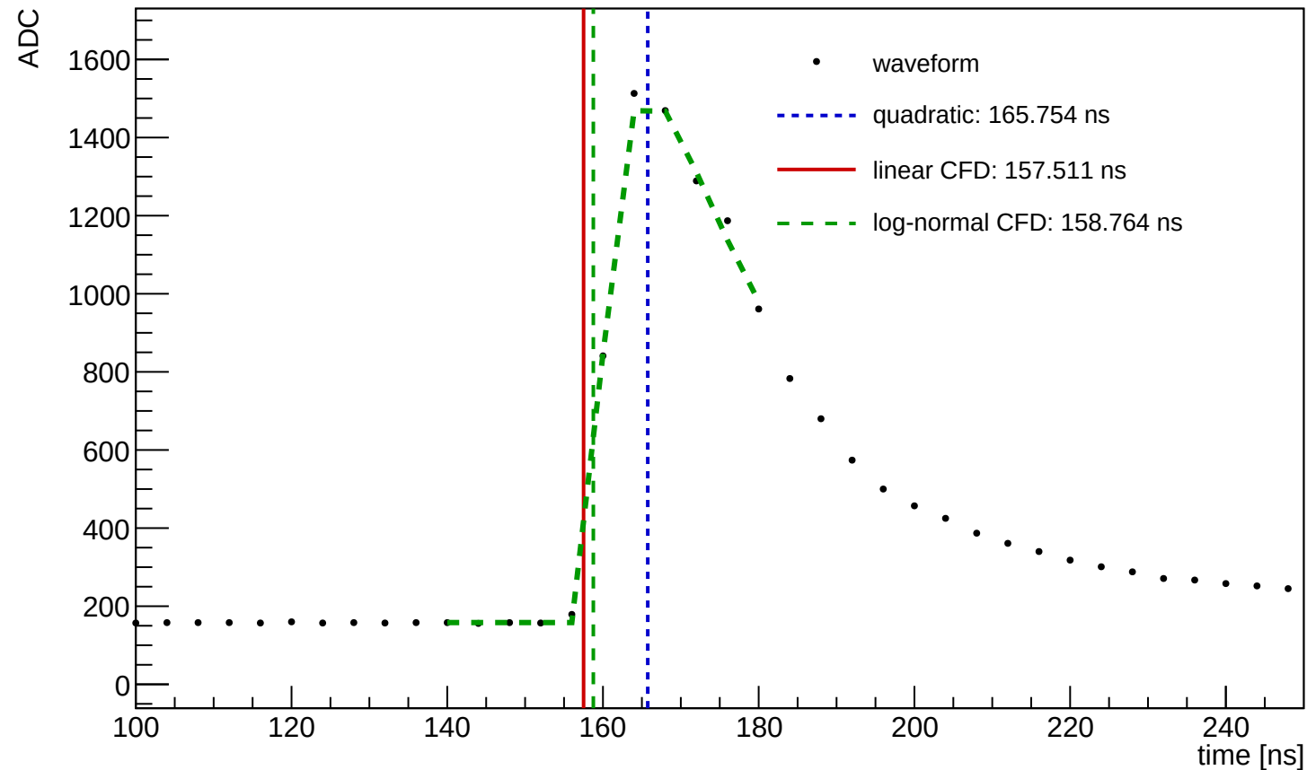
Waveform Time Demo (entry=17277, ch=12, module=1458, trigger=SUM)
