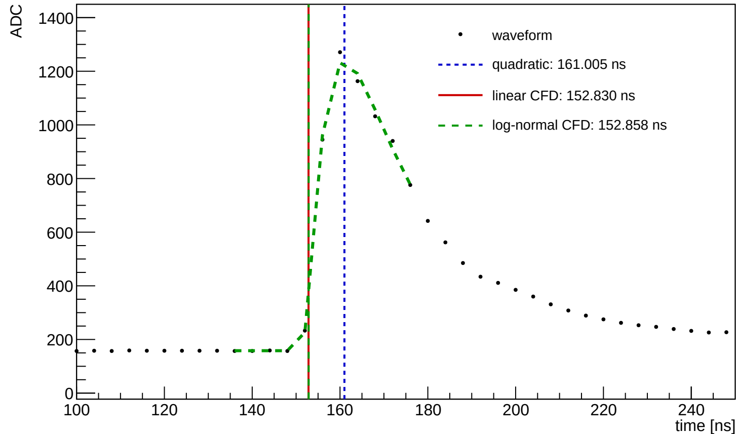
Waveform Time Demo (entry=50300, ch=9, module=1458, trigger=SUM)
