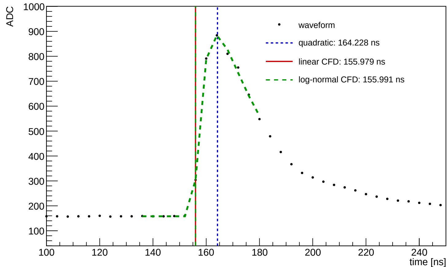
Waveform Time Demo (entry=42040, ch=11, module=1458, trigger=SUM)
