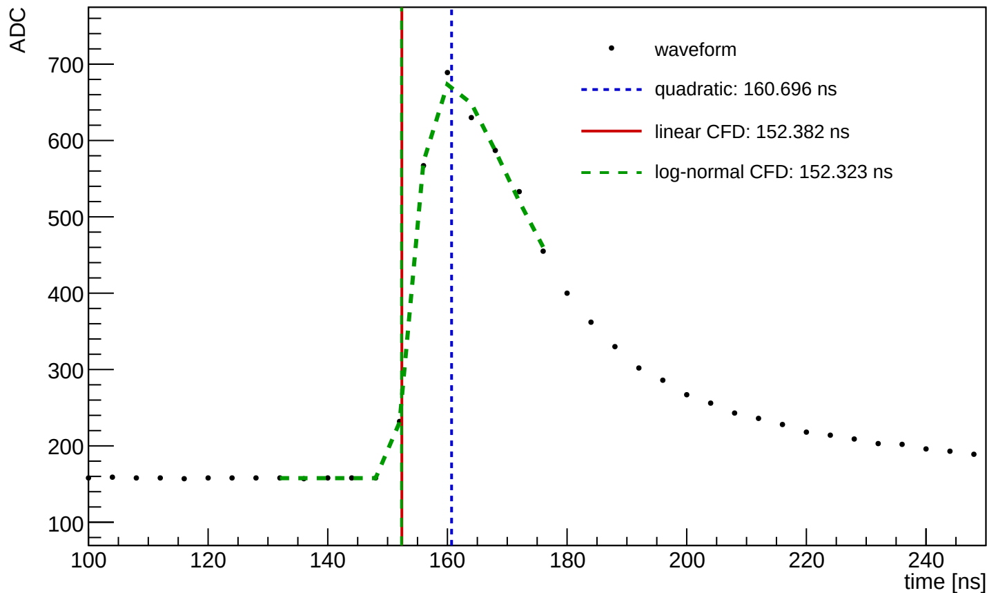
Waveform Time Demo (entry=26542, ch=11, module=1458, trigger=SUM)
