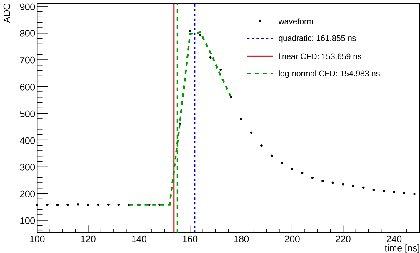
Waveform Time Demo (entry=55468, ch=13, module=1458, trigger=SUM)
