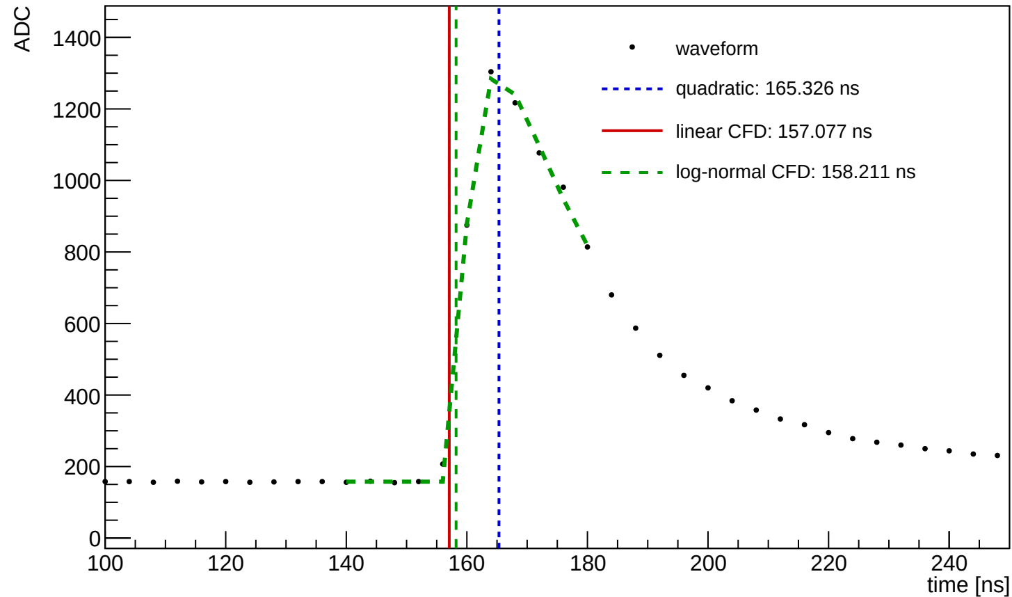
Waveform Time Demo (entry=35431, ch=13, module=1458, trigger=SUM)
