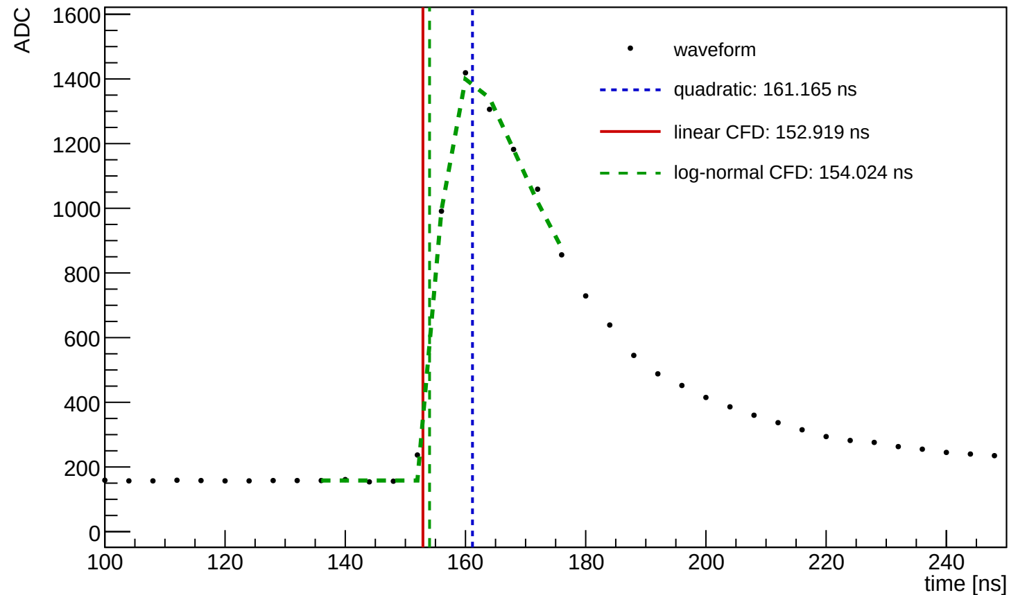
Waveform Time Demo (entry=37559, ch=13, module=1458, trigger=SUM)
