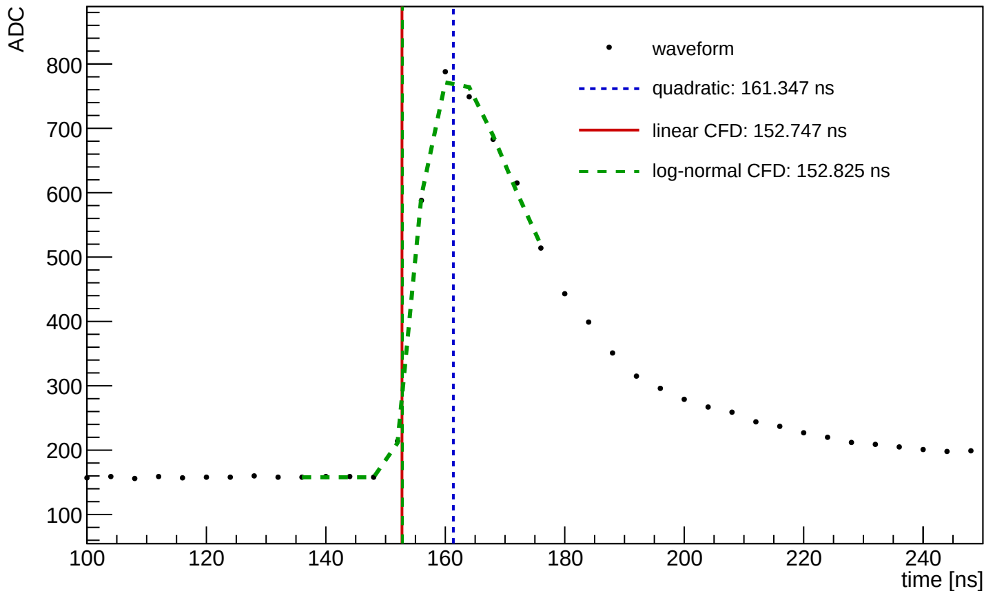
Waveform Time Demo (entry=5786, ch=11, module=1458, trigger=SUM)
