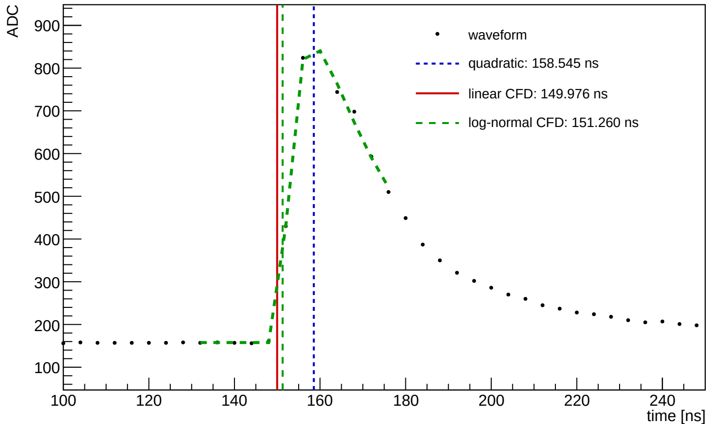
Waveform Time Demo (entry=7206, ch=11, module=1458, trigger=SUM)
