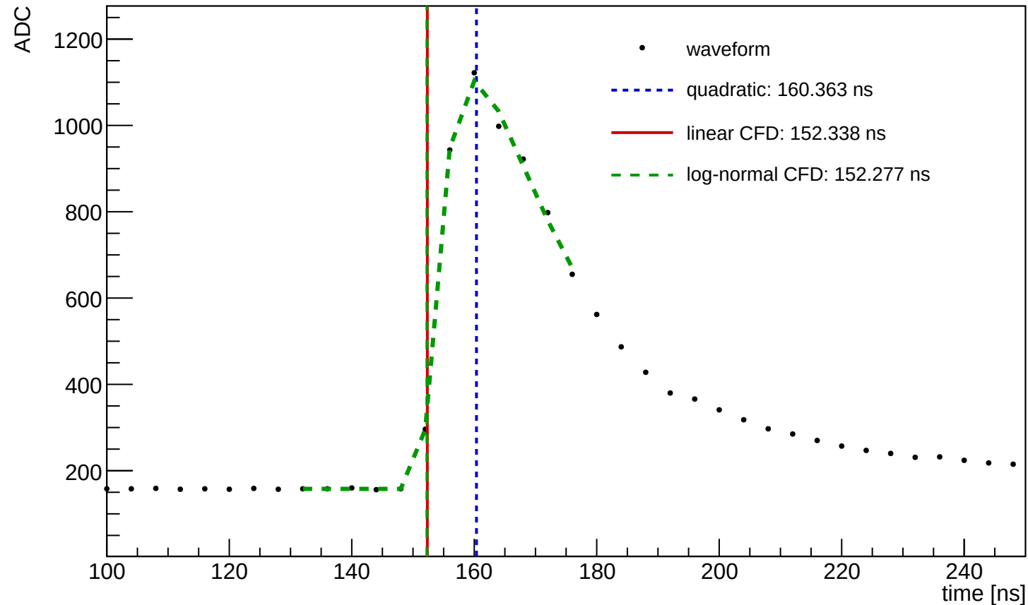
Waveform Time Demo (entry=36584, ch=10, module=1458, trigger=SUM)
