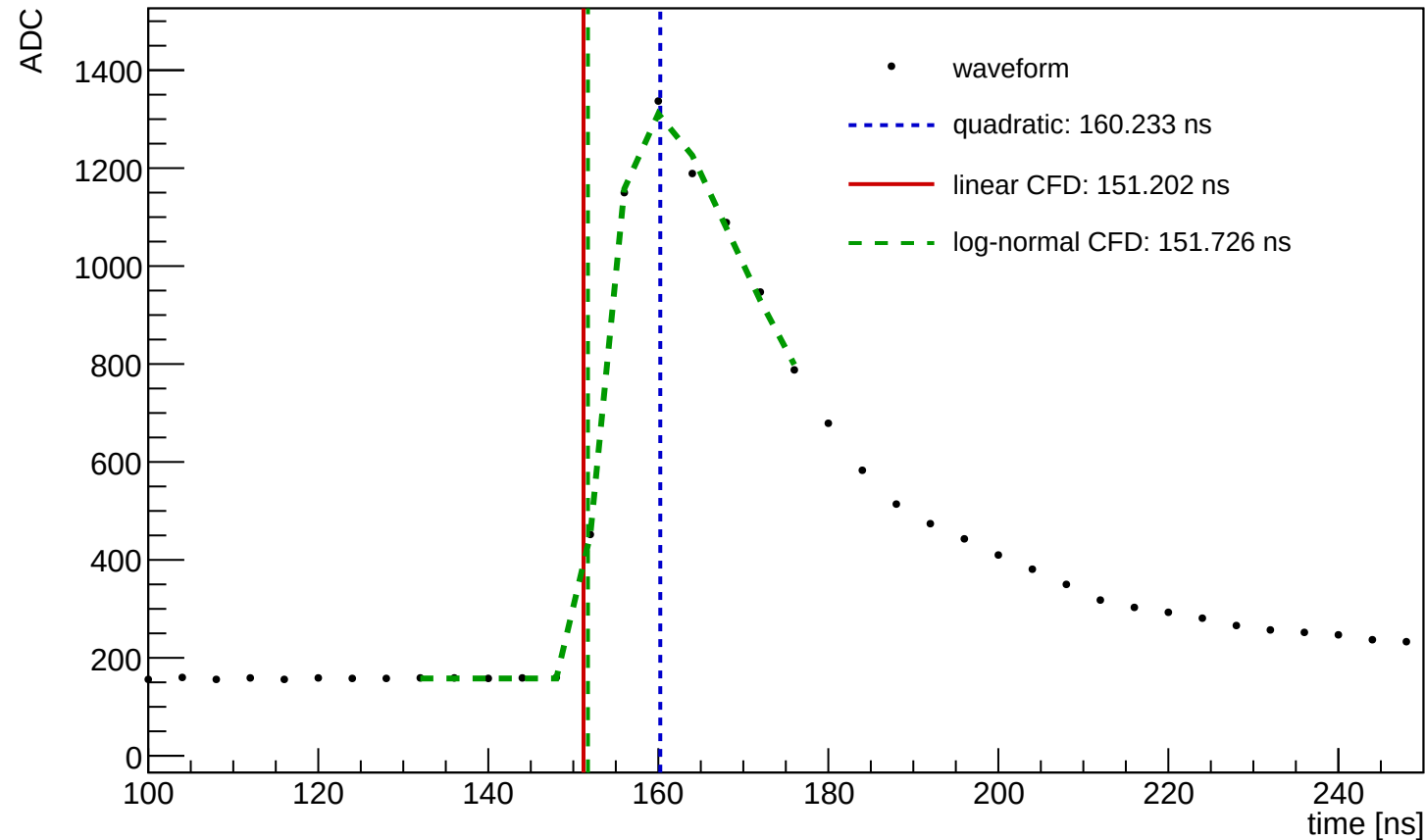
Waveform Time Demo (entry=10124, ch=9, module=1458, trigger=SUM)
