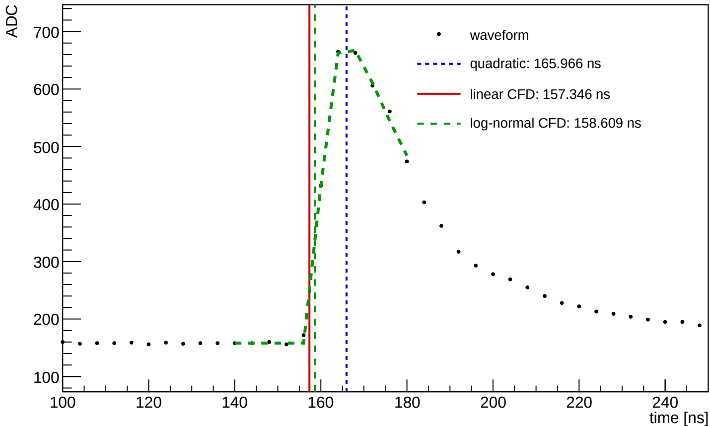
Waveform Time Demo (entry=50934, ch=10, module=1458, trigger=SUM)
