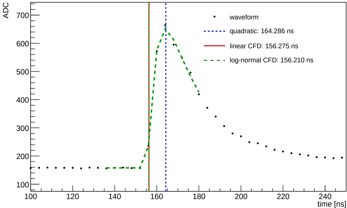
Waveform Time Demo (entry=34048, ch=10, module=1458, trigger=SUM)
