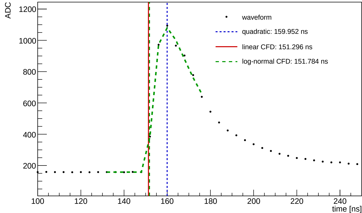
Waveform Time Demo (entry=20413, ch=7, module=1458, trigger=SUM)
