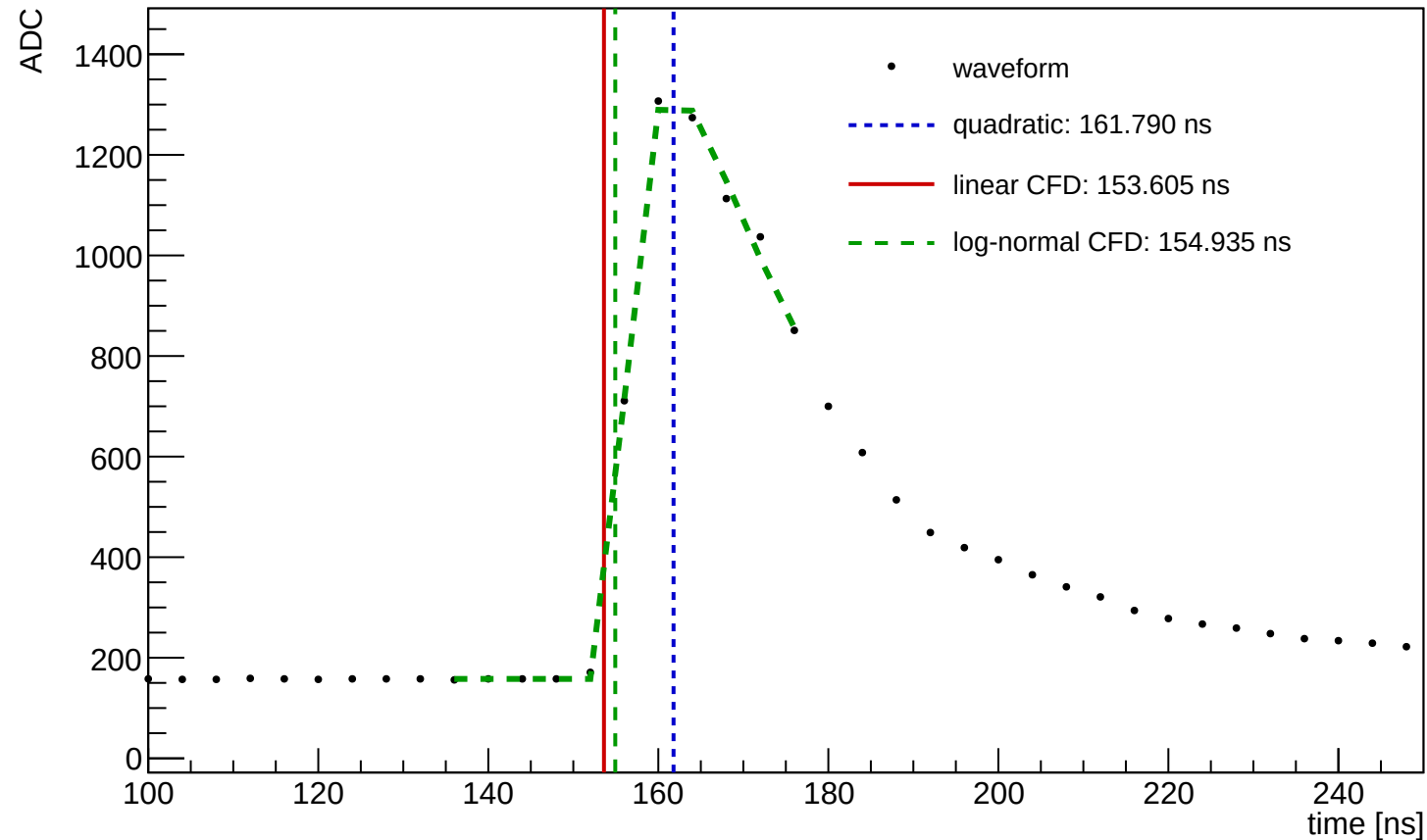
Waveform Time Demo (entry=50200, ch=16, module=1458, trigger=SUM)
