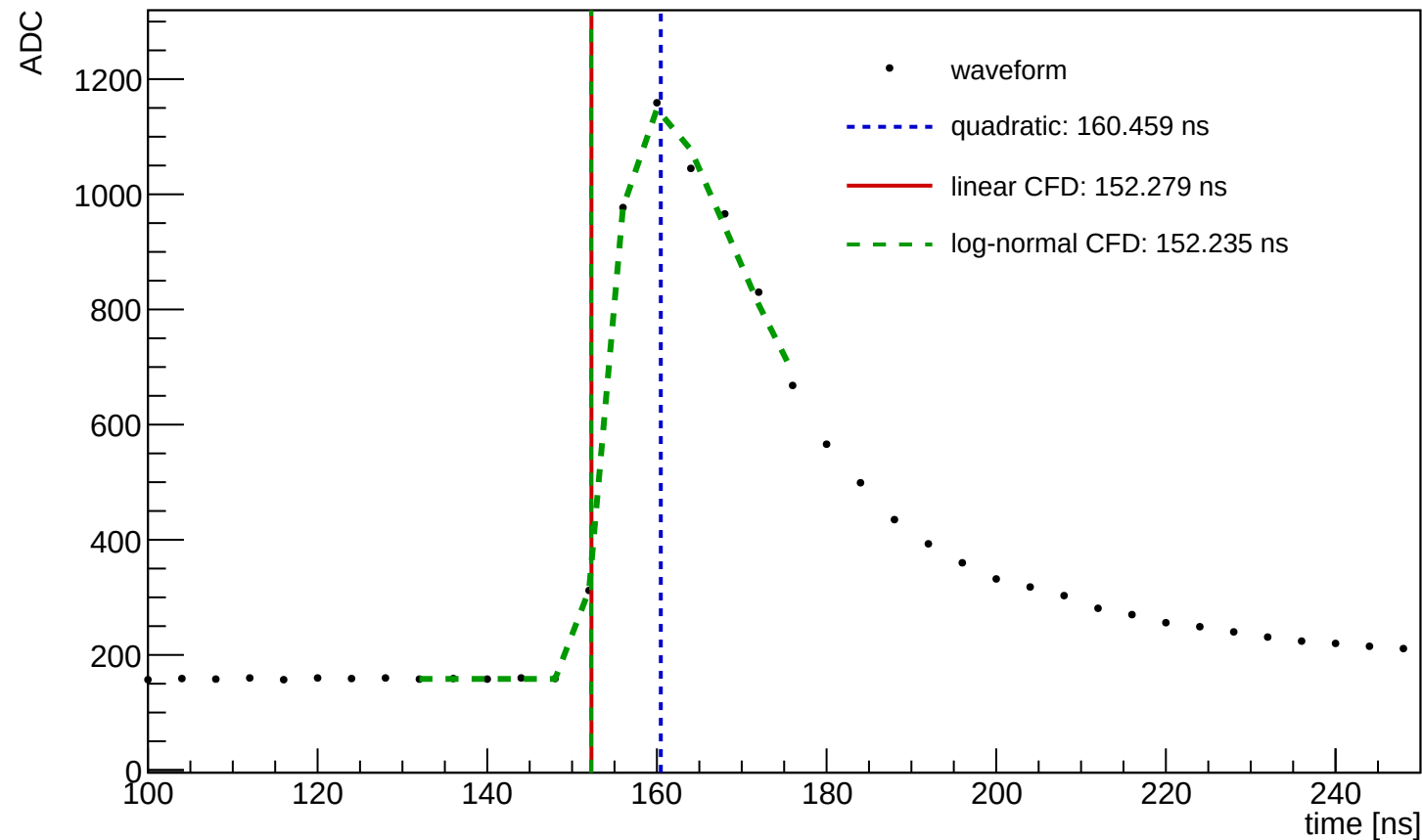
Waveform Time Demo (entry=44017, ch=8, module=1458, trigger=SUM)
