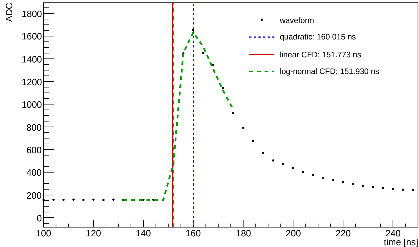
Waveform Time Demo (entry=22051, ch=10, module=1458, trigger=SUM)
