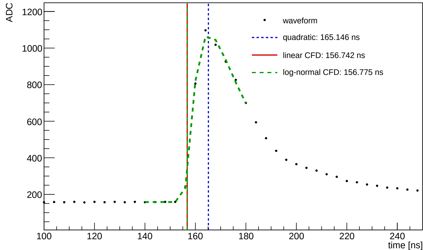
Waveform Time Demo (entry=51717, ch=12, module=1458, trigger=SUM)
