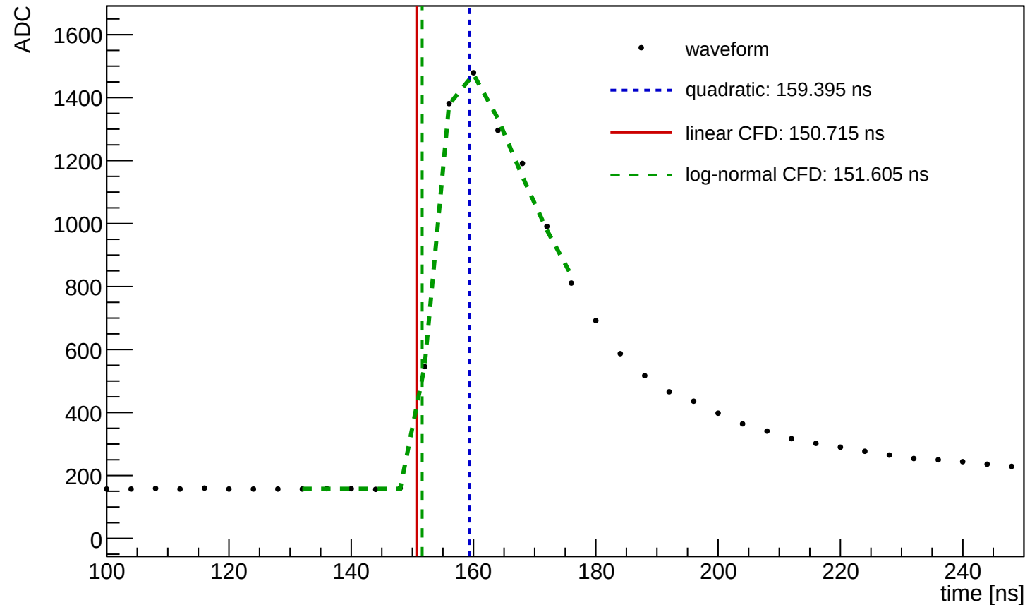
Waveform Time Demo (entry=5444, ch=10, module=1458, trigger=SUM)
