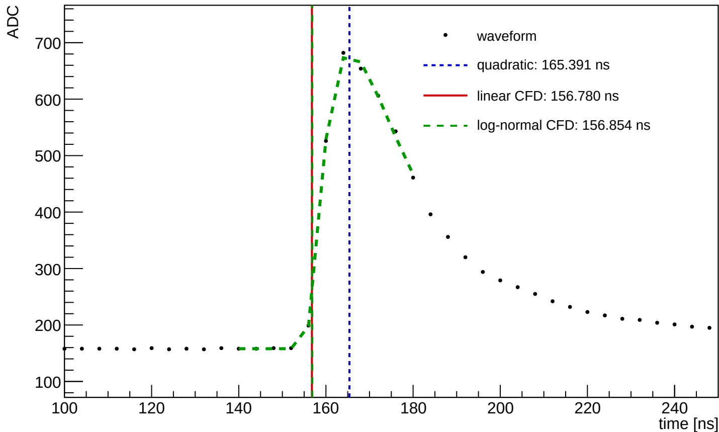
Waveform Time Demo (entry=66255, ch=12, module=1458, trigger=SUM)
