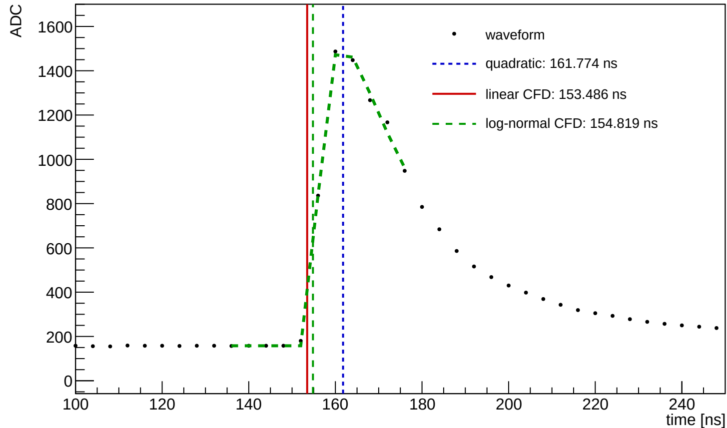
Waveform Time Demo (entry=11716, ch=11, module=1458, trigger=SUM)
