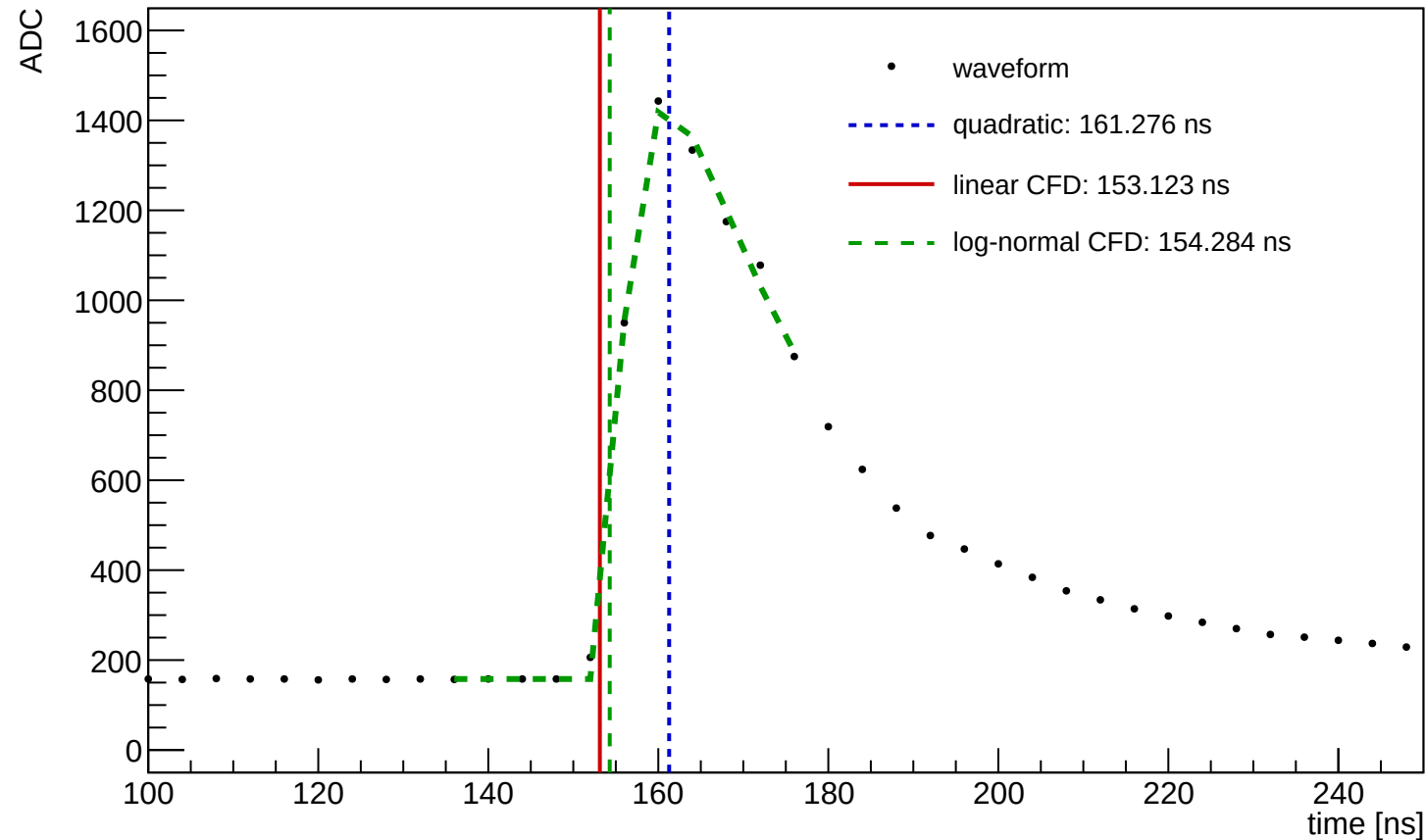
Waveform Time Demo (entry=3919, ch=13, module=1458, trigger=SUM)
