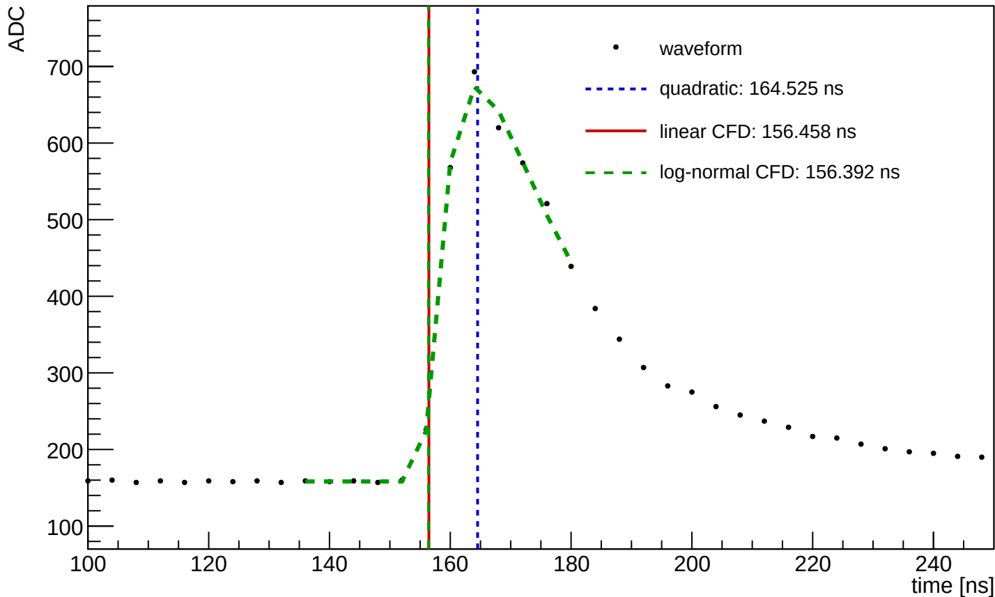
Waveform Time Demo (entry=1049, ch=8, module=1458, trigger=SUM)
