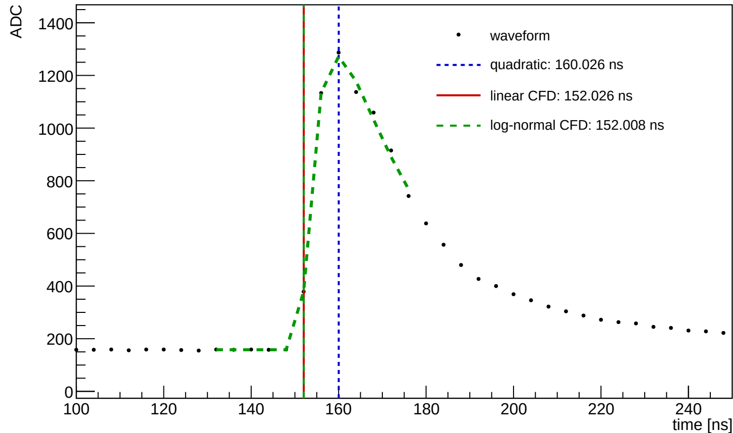
Waveform Time Demo (entry=31506, ch=8, module=1458, trigger=SUM)
