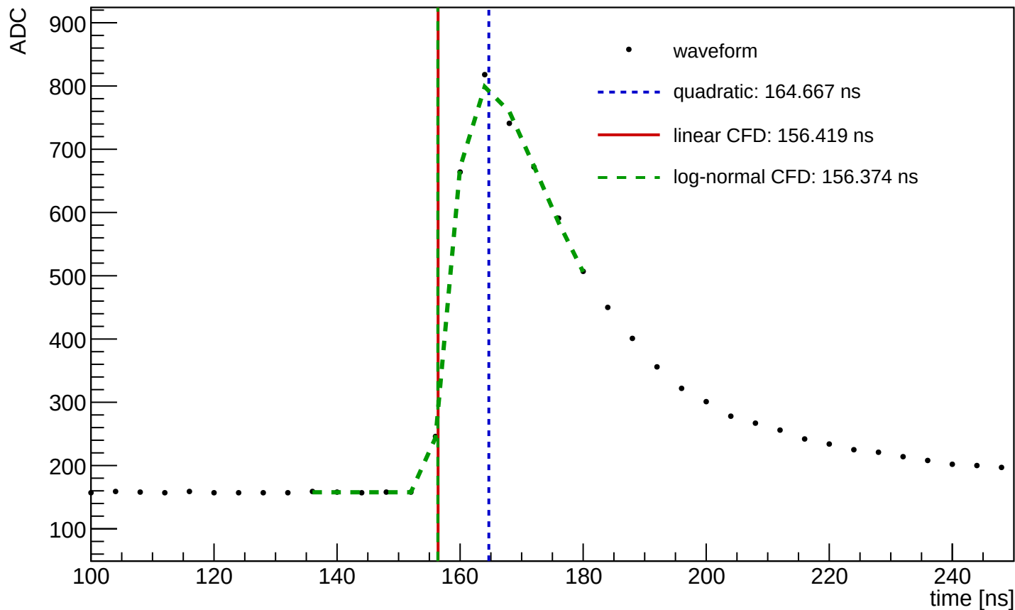
Waveform Time Demo (entry=3195, ch=9, module=1458, trigger=SUM)
