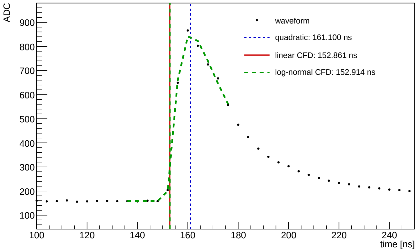
Waveform Time Demo (entry=7583, ch=13, module=1458, trigger=SUM)
