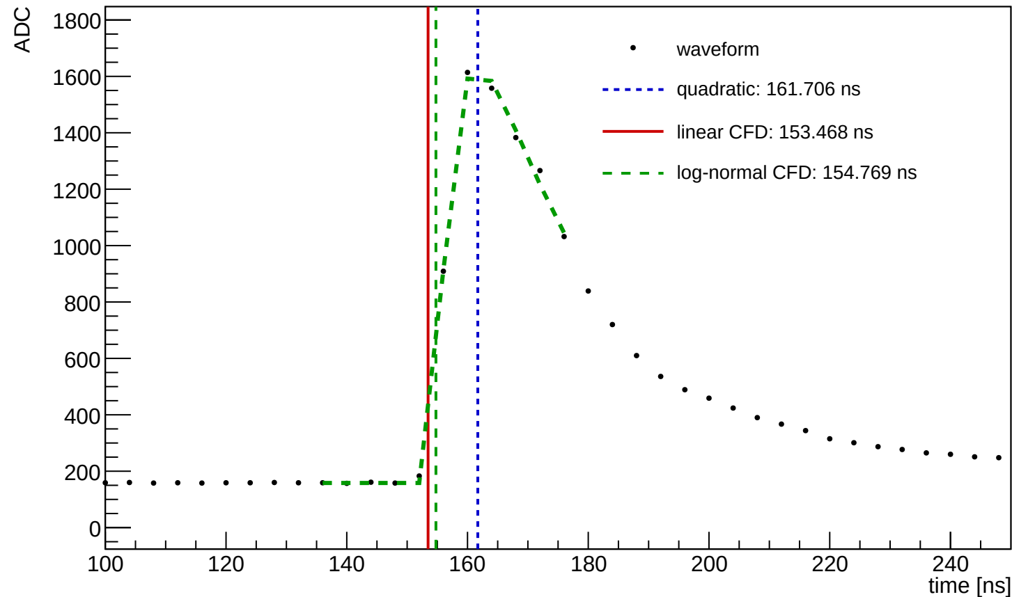
Waveform Time Demo (entry=64651, ch=14, module=1458, trigger=SUM)
