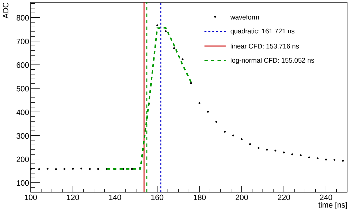
Waveform Time Demo (entry=55958, ch=8, module=1458, trigger=SUM)
