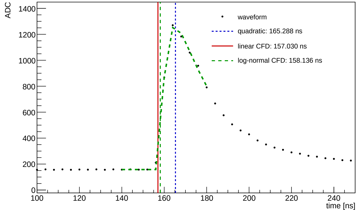
Waveform Time Demo (entry=56354, ch=11, module=1458, trigger=SUM)
