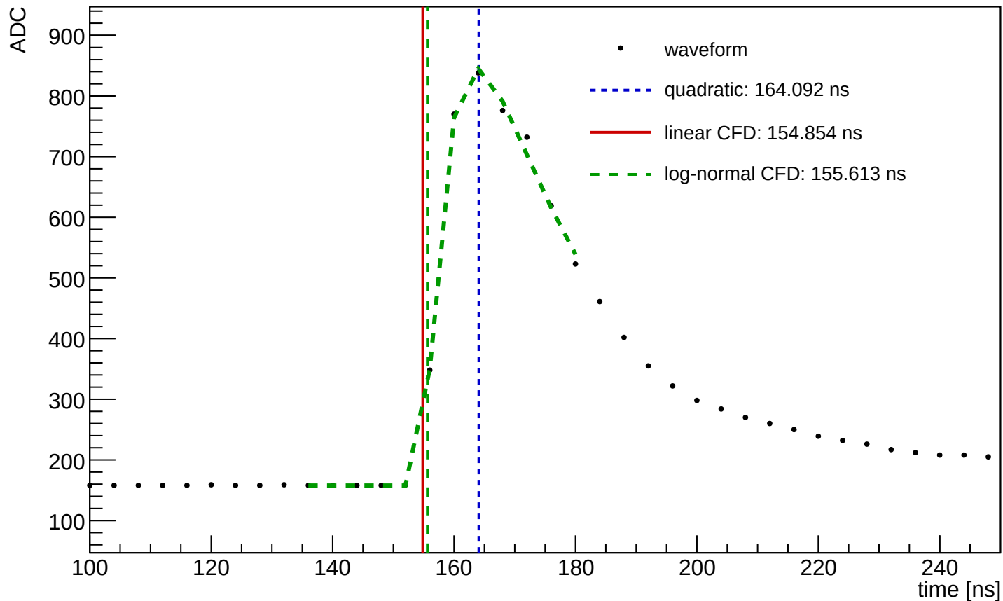
Waveform Time Demo (entry=54892, ch=10, module=1458, trigger=SUM)
