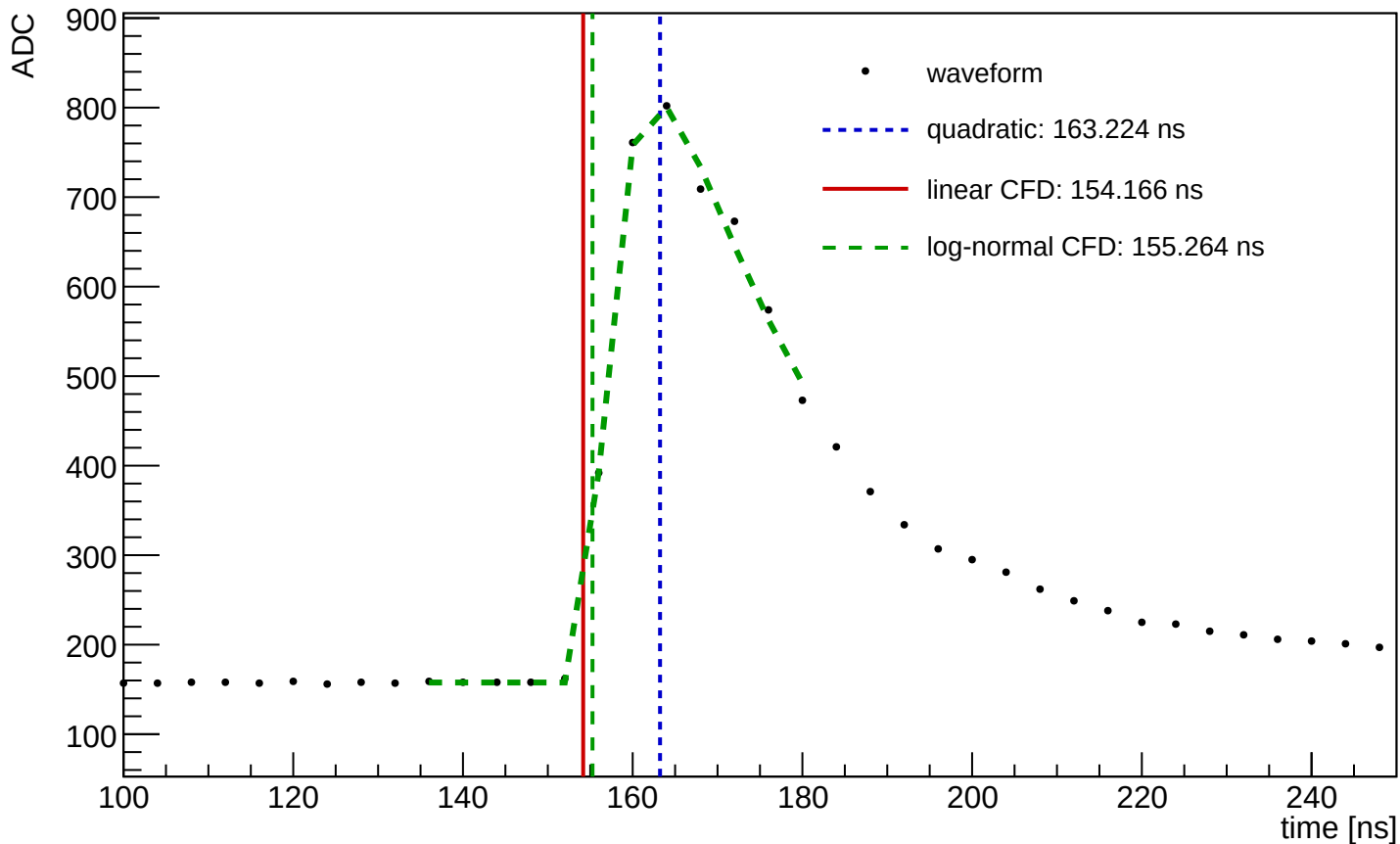
Waveform Time Demo (entry=61901, ch=14, module=1458, trigger=SUM)
