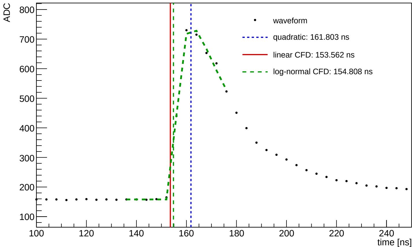
Waveform Time Demo (entry=62516, ch=9, module=1458, trigger=SUM)
