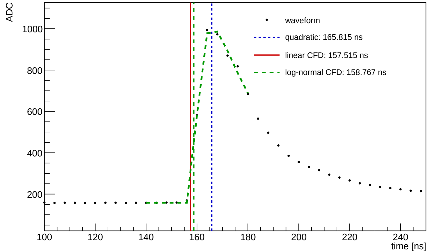
Waveform Time Demo (entry=40211, ch=30, module=1458, trigger=SUM)
