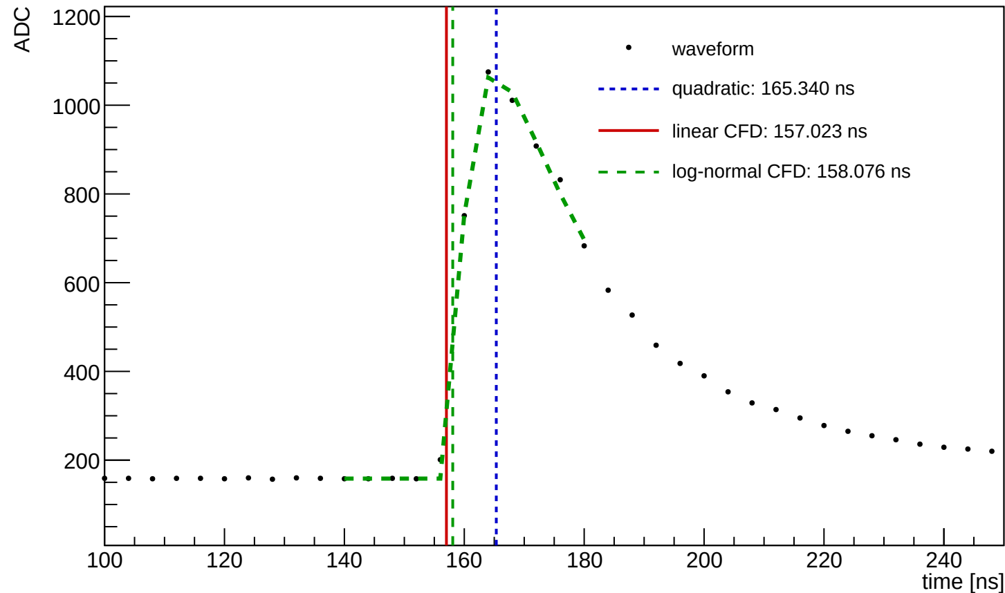
Waveform Time Demo (entry=17639, ch=12, module=1458, trigger=SUM)
