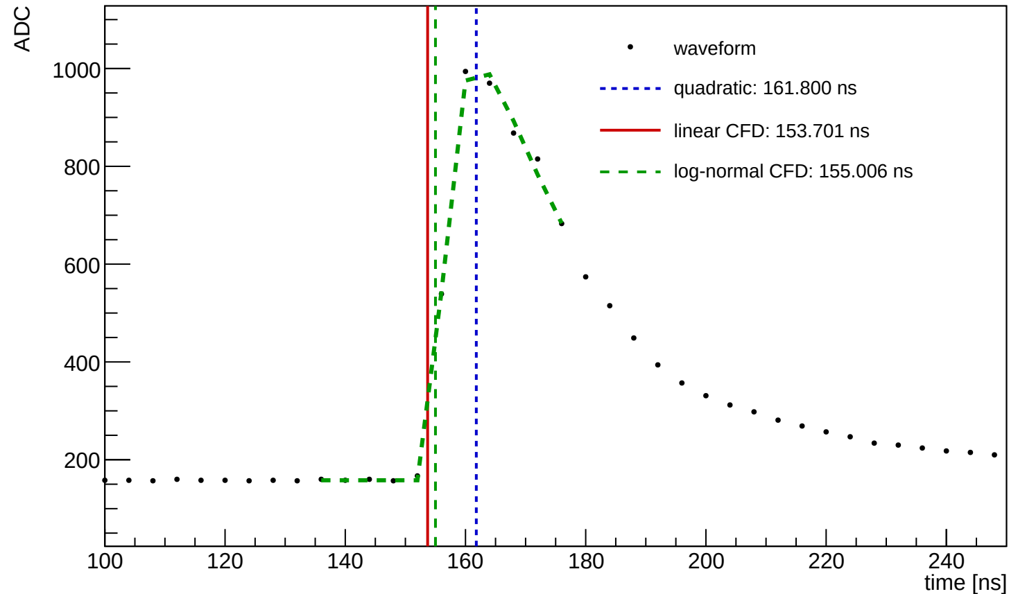
Waveform Time Demo (entry=31648, ch=15, module=1458, trigger=SUM)
