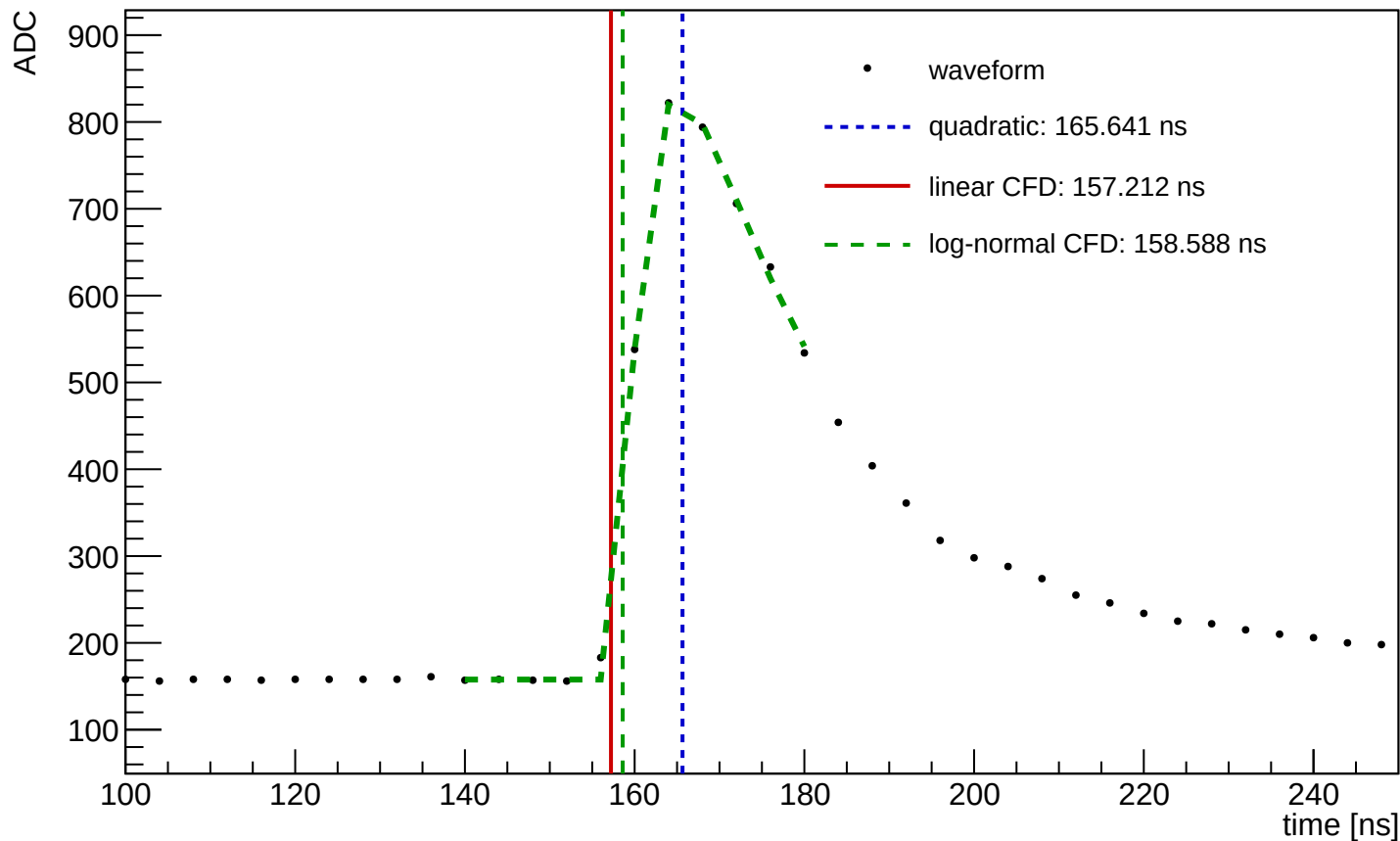
Waveform Time Demo (entry=61849, ch=10, module=1458, trigger=SUM)
