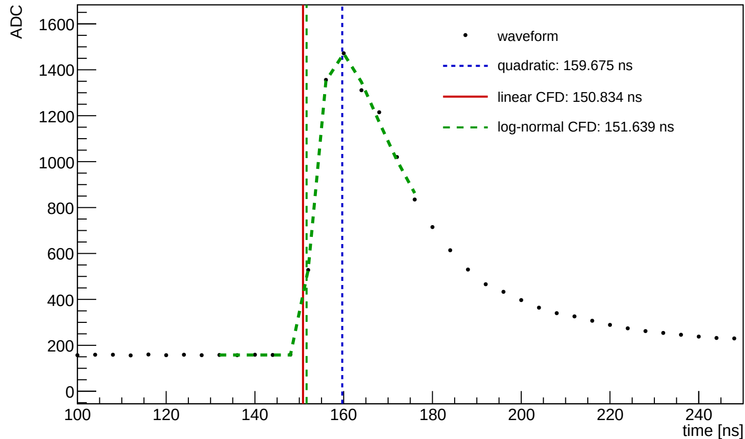
Waveform Time Demo (entry=64135, ch=28, module=1458, trigger=SUM)
