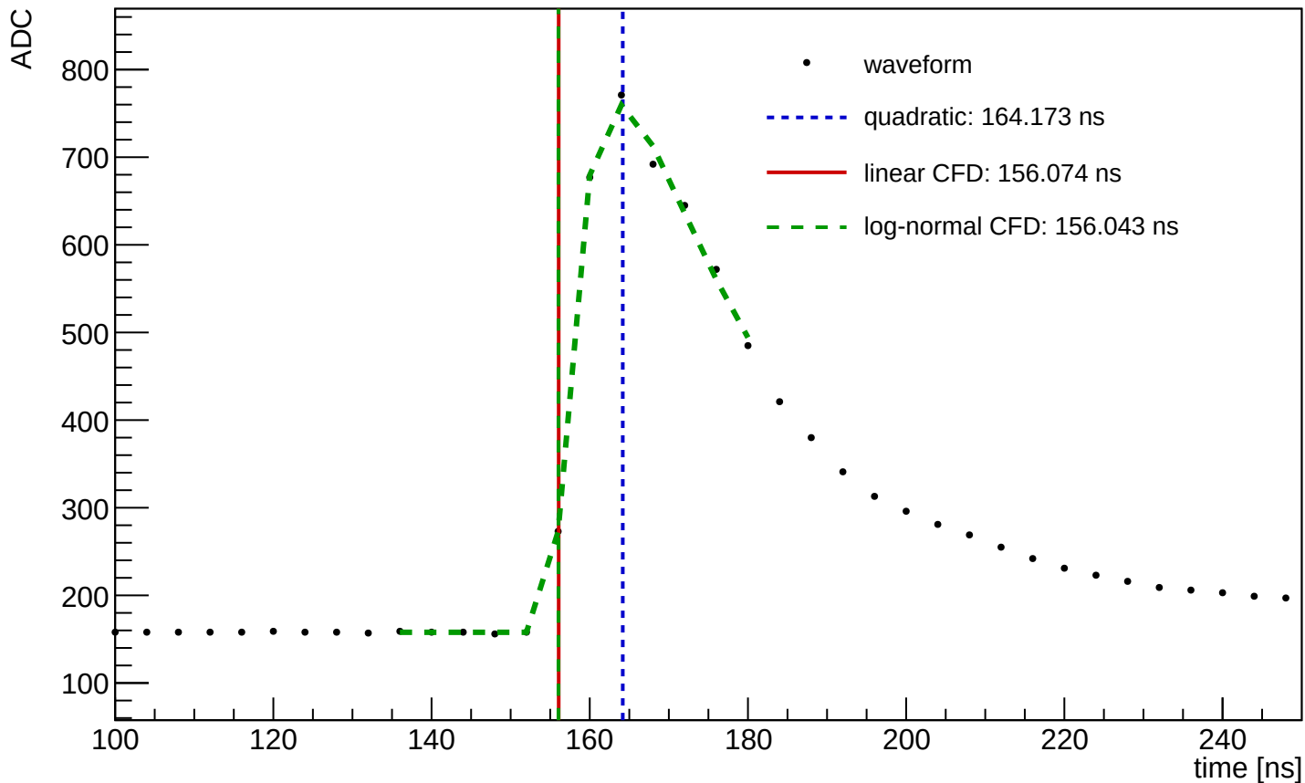
Waveform Time Demo (entry=54431, ch=7, module=1458, trigger=SUM)
