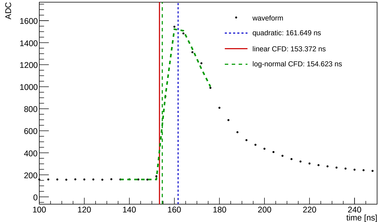
Waveform Time Demo (entry=40470, ch=12, module=1458, trigger=SUM)
