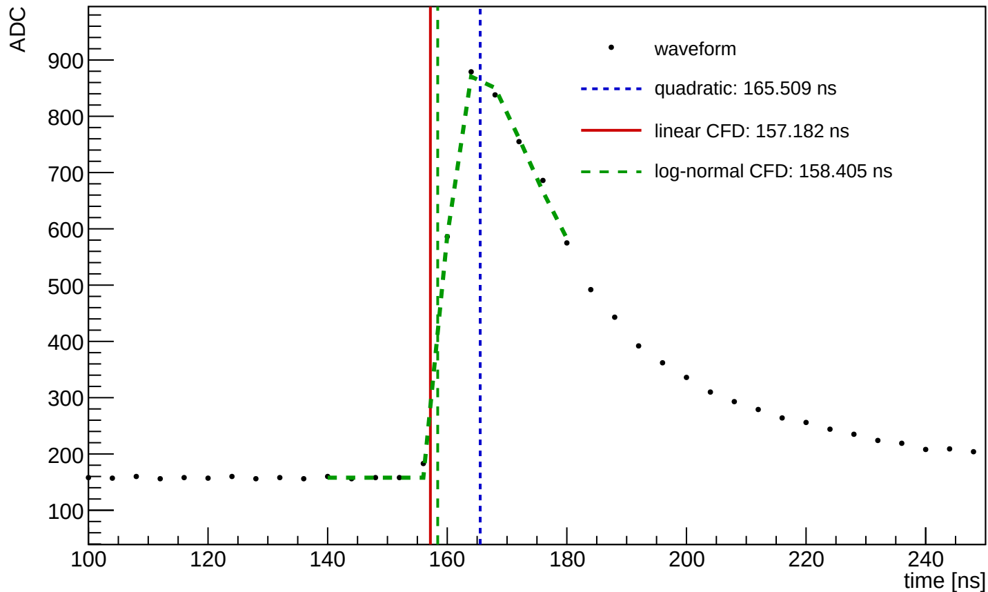
Waveform Time Demo (entry=26272, ch=11, module=1458, trigger=SUM)
