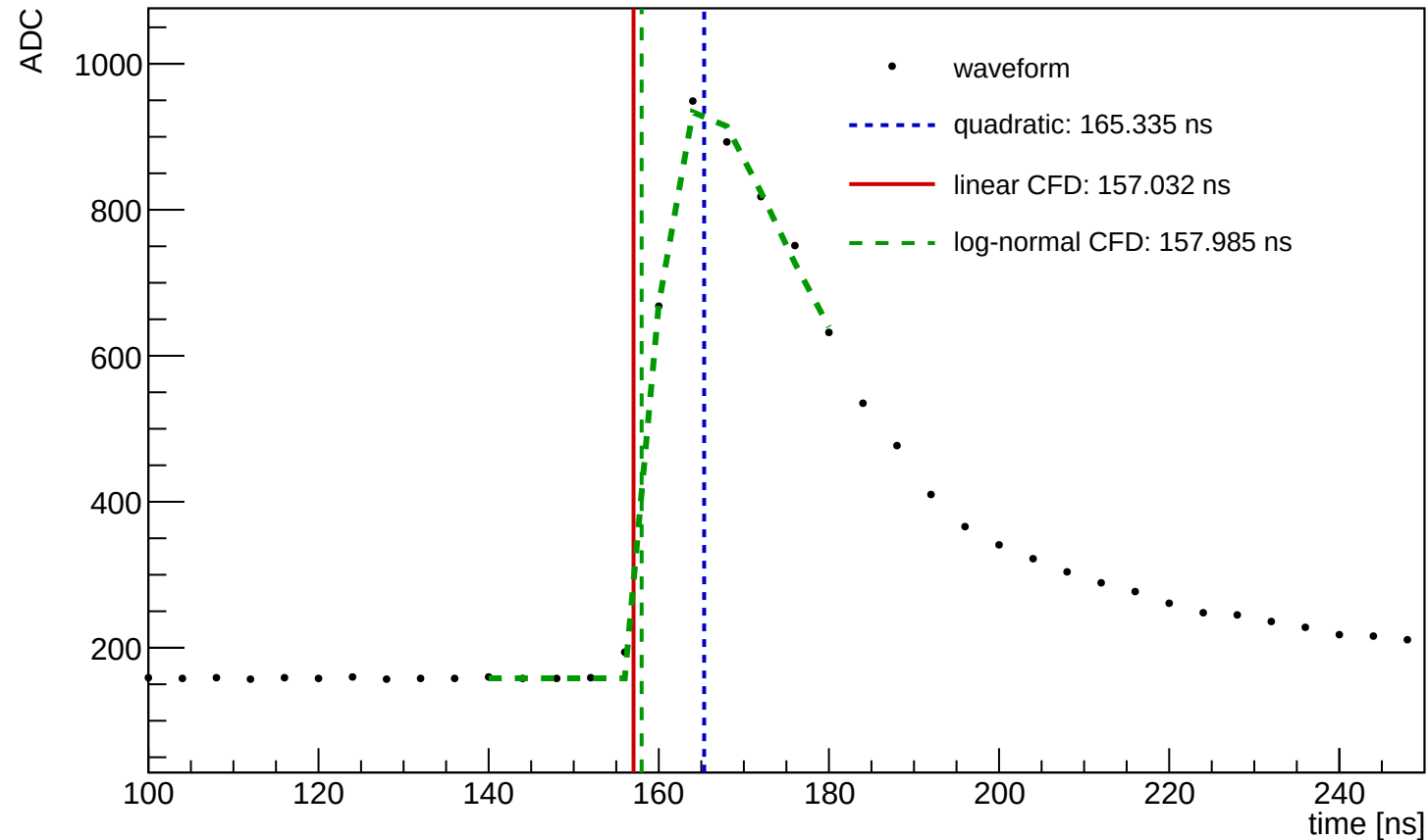
Waveform Time Demo (entry=61275, ch=12, module=1458, trigger=SUM)
