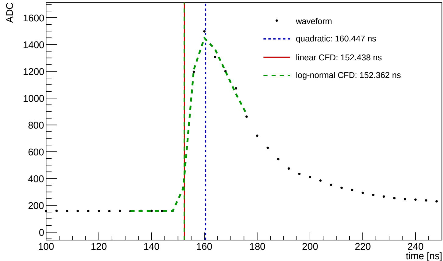
Waveform Time Demo (entry=49011, ch=11, module=1458, trigger=SUM)
