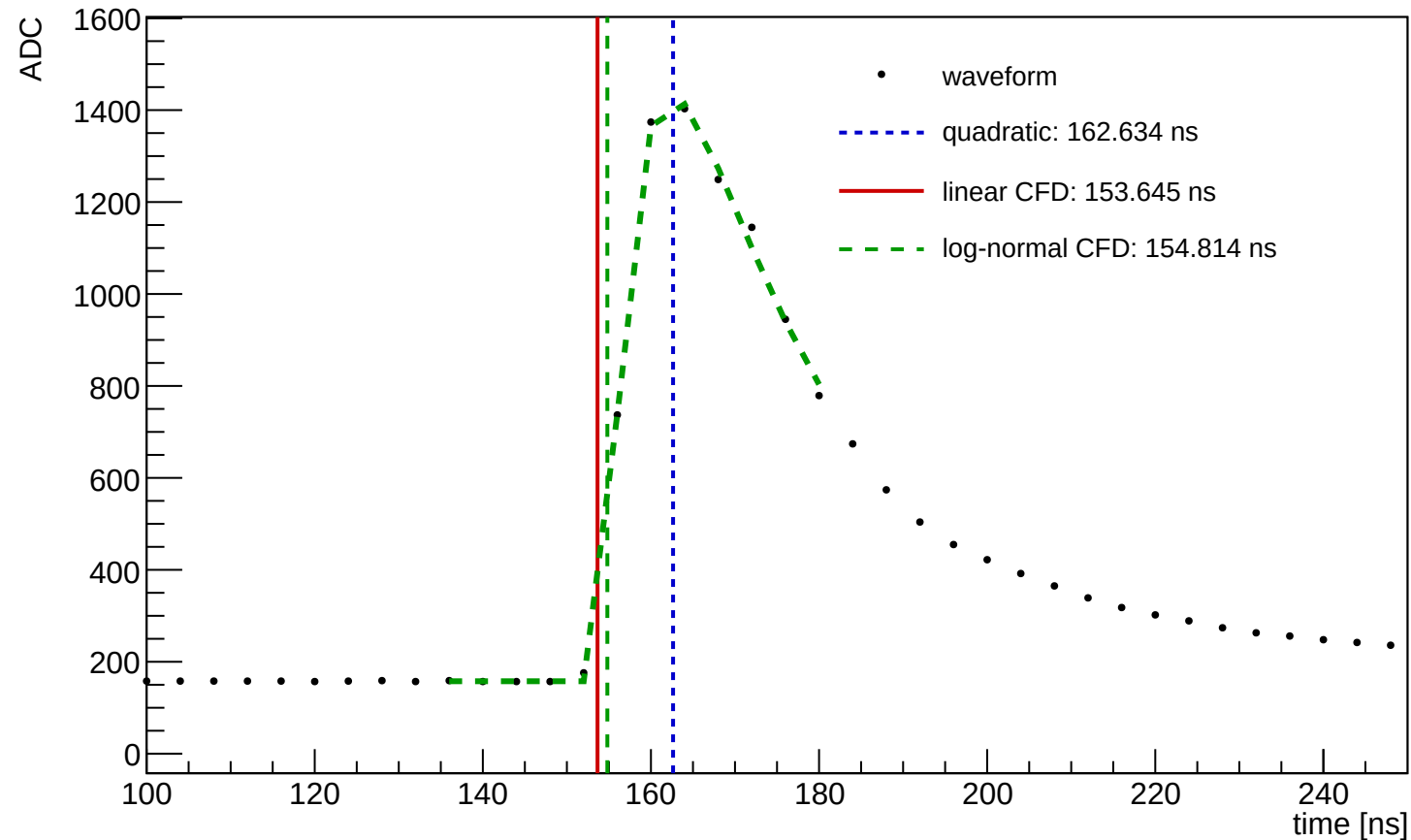
Waveform Time Demo (entry=33699, ch=11, module=1458, trigger=SUM)
