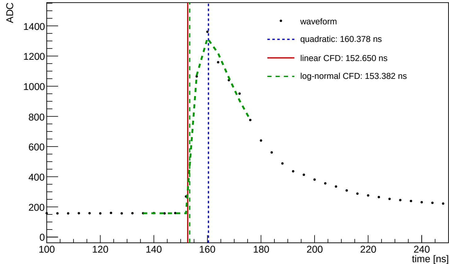
Waveform Time Demo (entry=37312, ch=9, module=1458, trigger=SUM)
