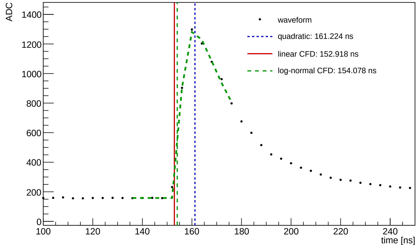
Waveform Time Demo (entry=42356, ch=9, module=1458, trigger=SUM)
