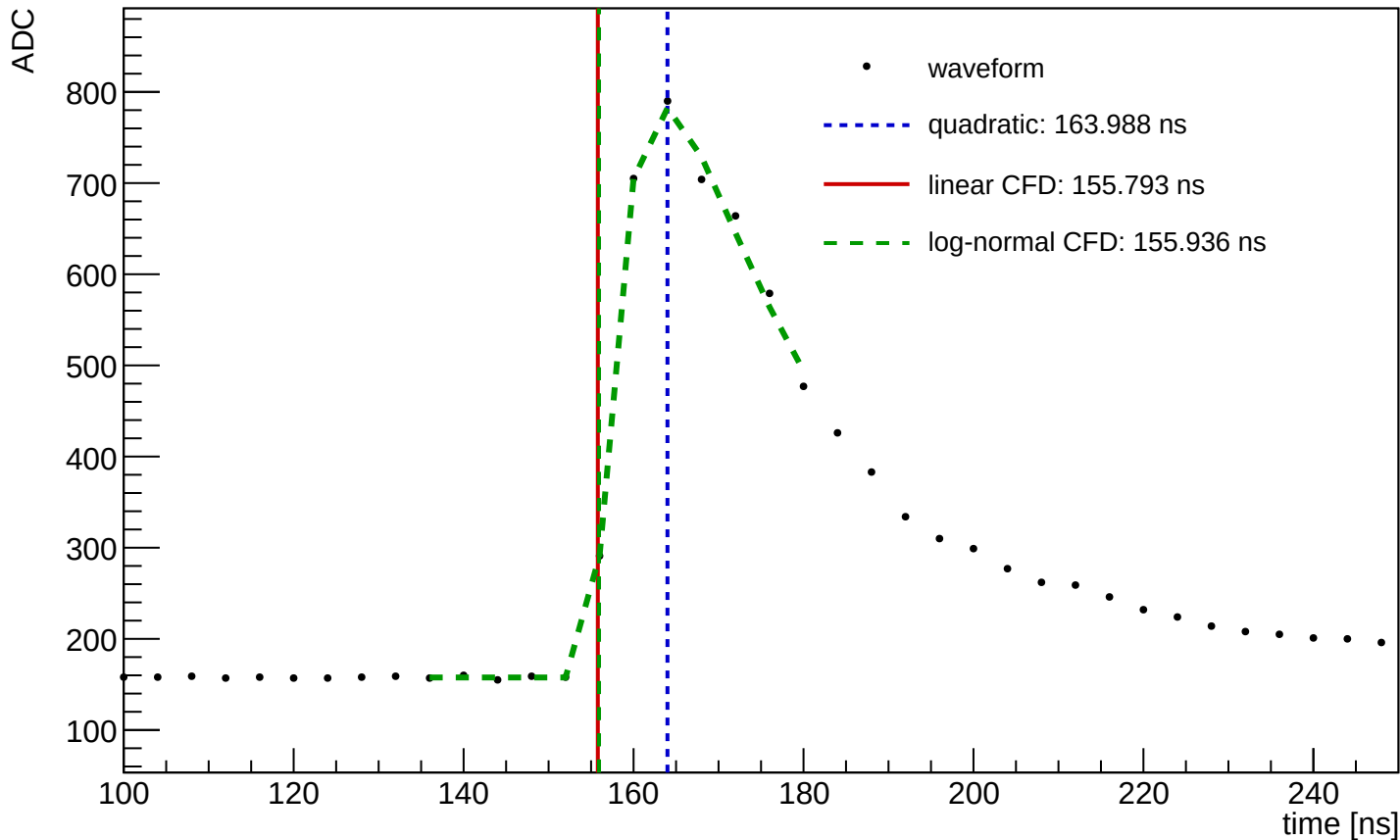
Waveform Time Demo (entry=32034, ch=7, module=1458, trigger=SUM)
