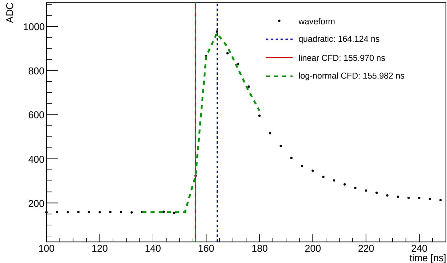
Waveform Time Demo (entry=15548, ch=10, module=1458, trigger=SUM)
