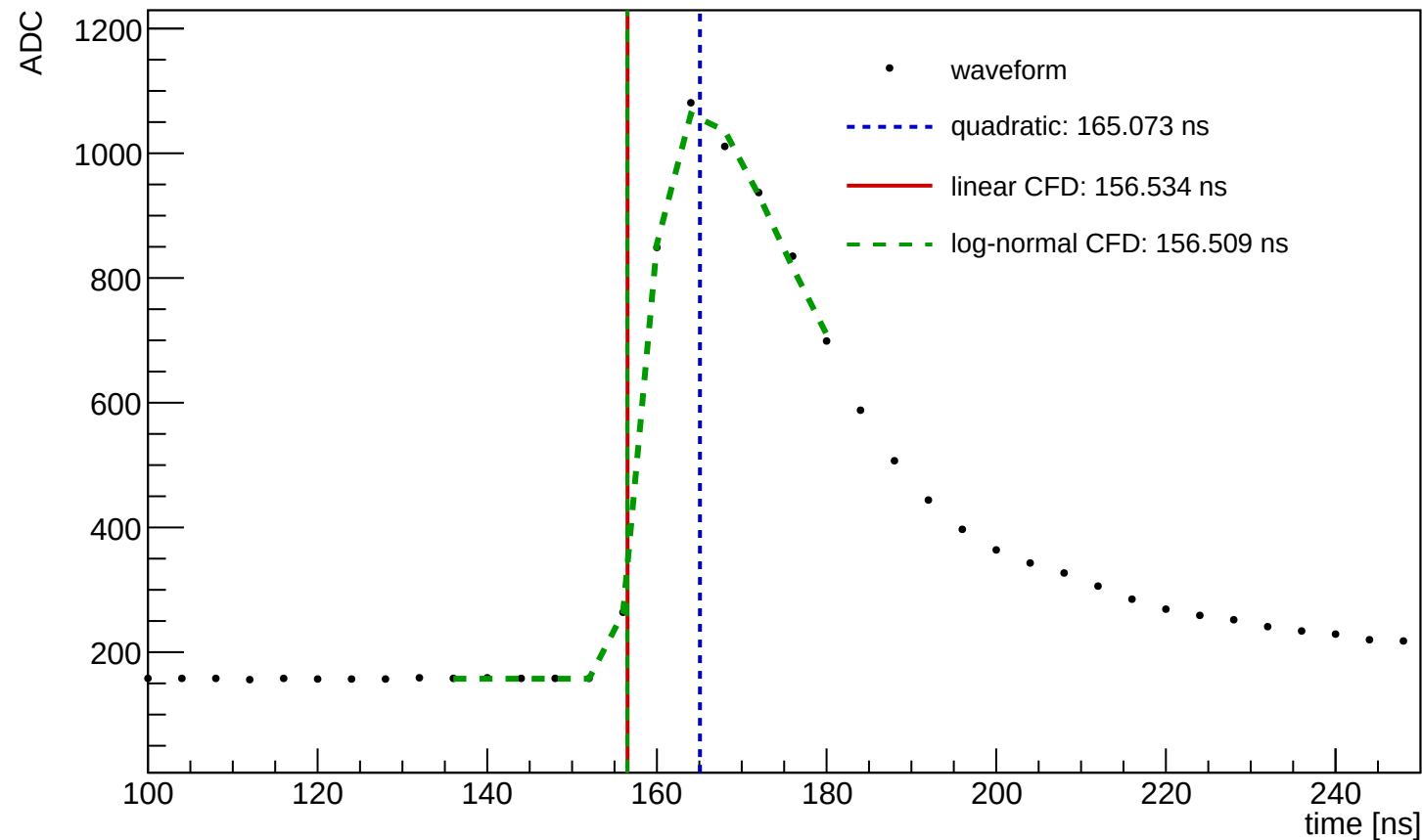
Waveform Time Demo (entry=64223, ch=9, module=1458, trigger=SUM)
