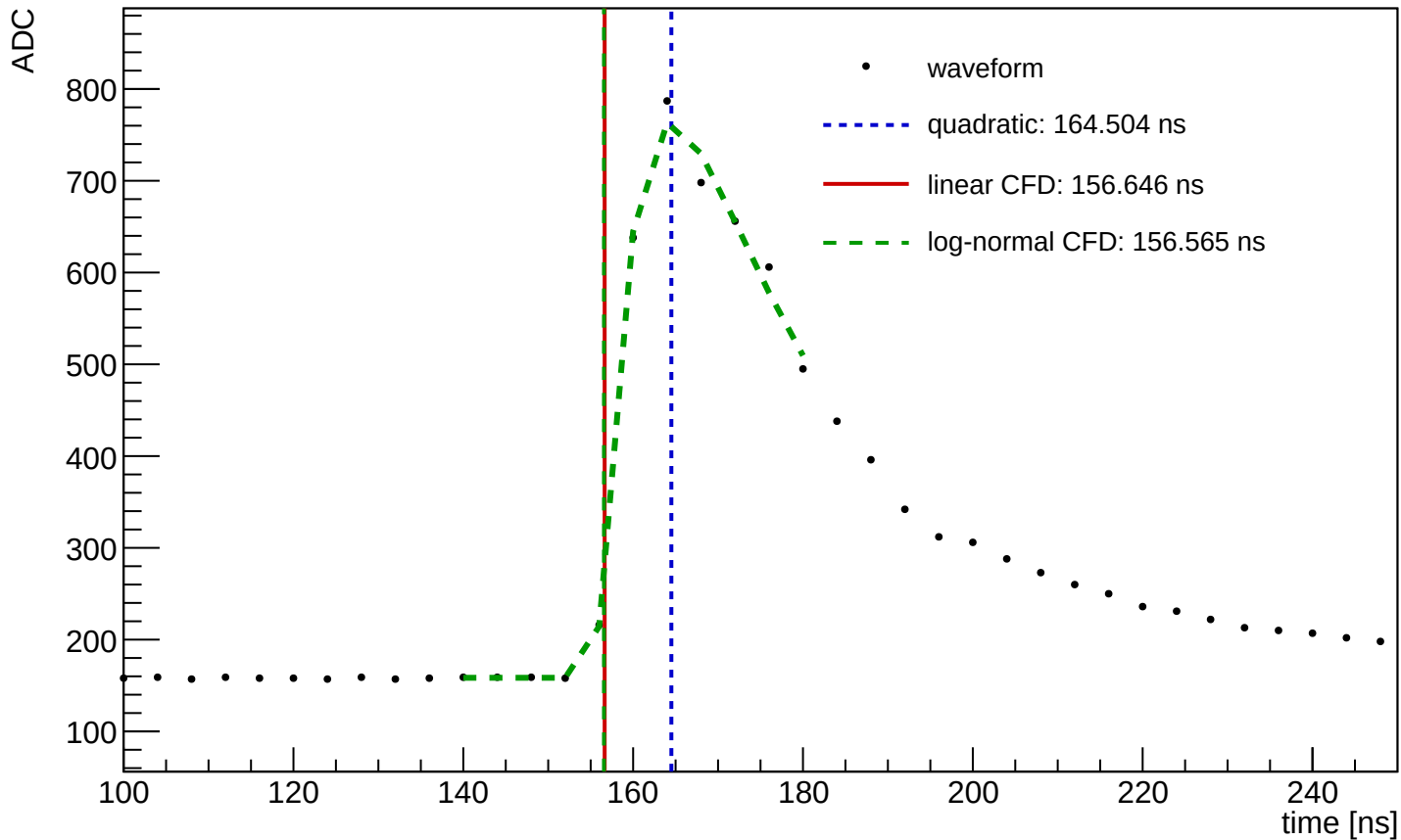
Waveform Time Demo (entry=9298, ch=8, module=1458, trigger=SUM)
