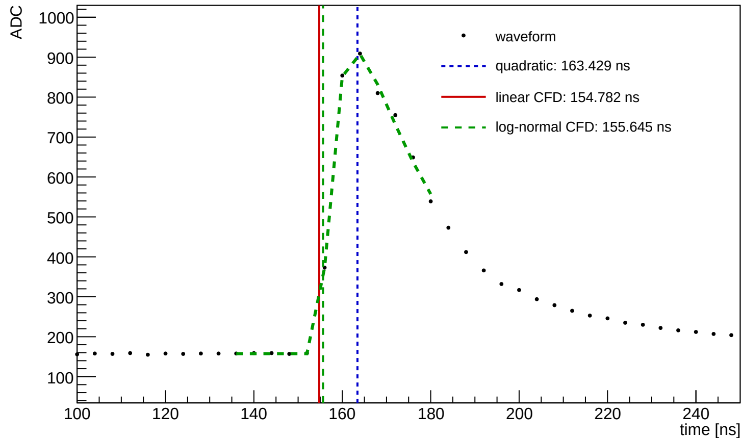
Waveform Time Demo (entry=64257, ch=12, module=1458, trigger=SUM)
