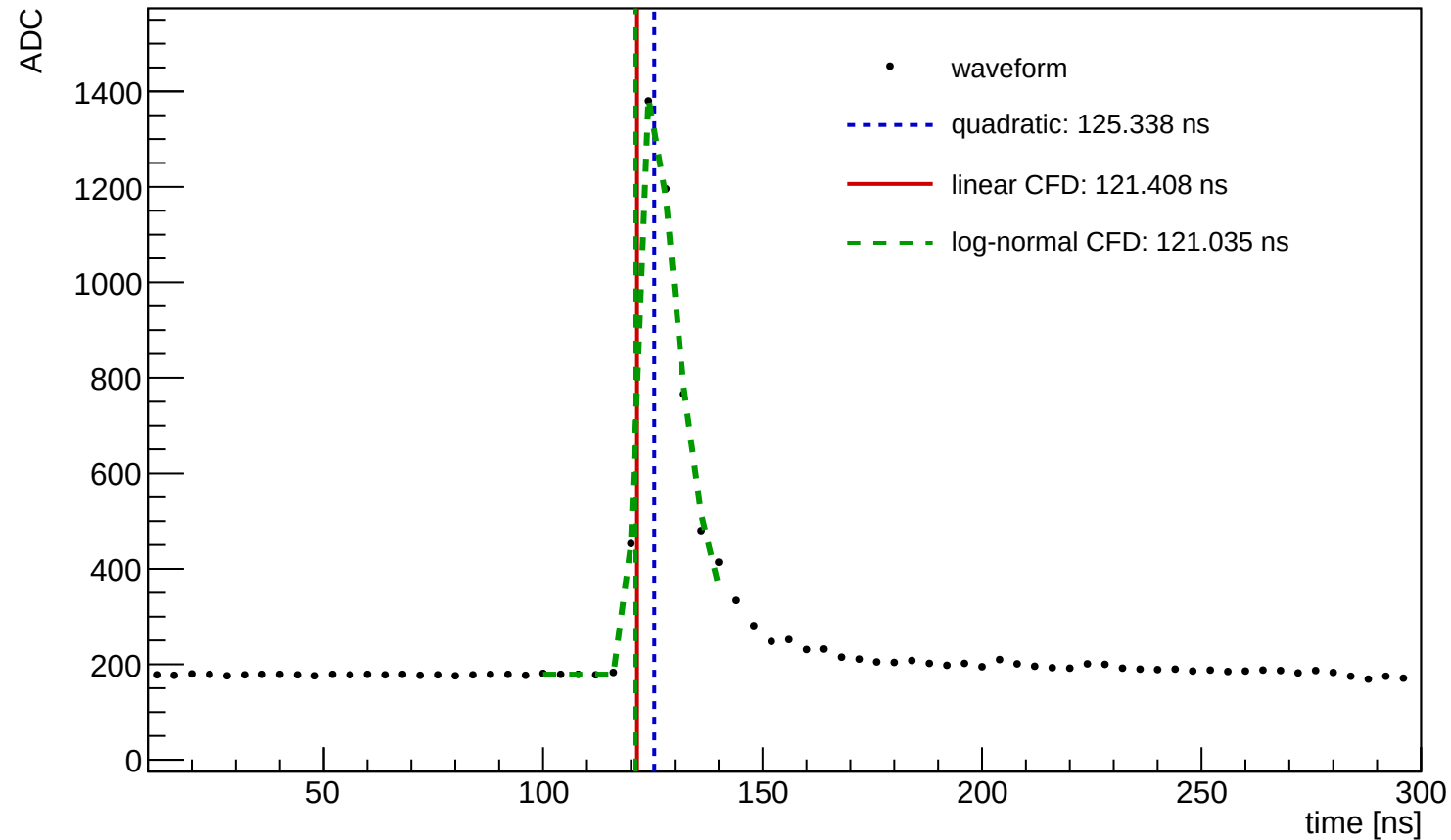
Waveform Time Demo (entry=347, ch=0, module=3003, trigger=SUM)
