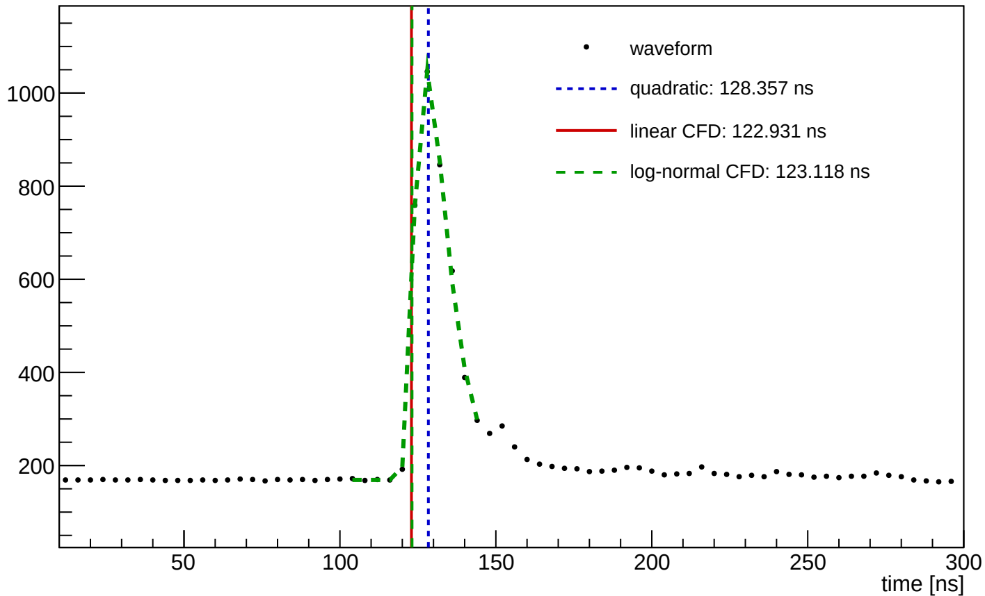
Waveform Time Demo (entry=1401, ch=3, module=3004, trigger=SUM)
