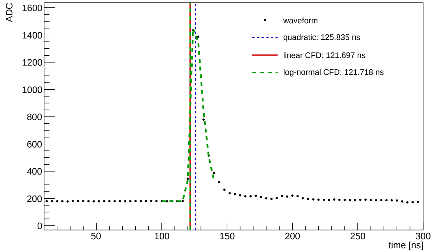
Waveform Time Demo (entry=1249, ch=1, module=3003, trigger=SUM)
