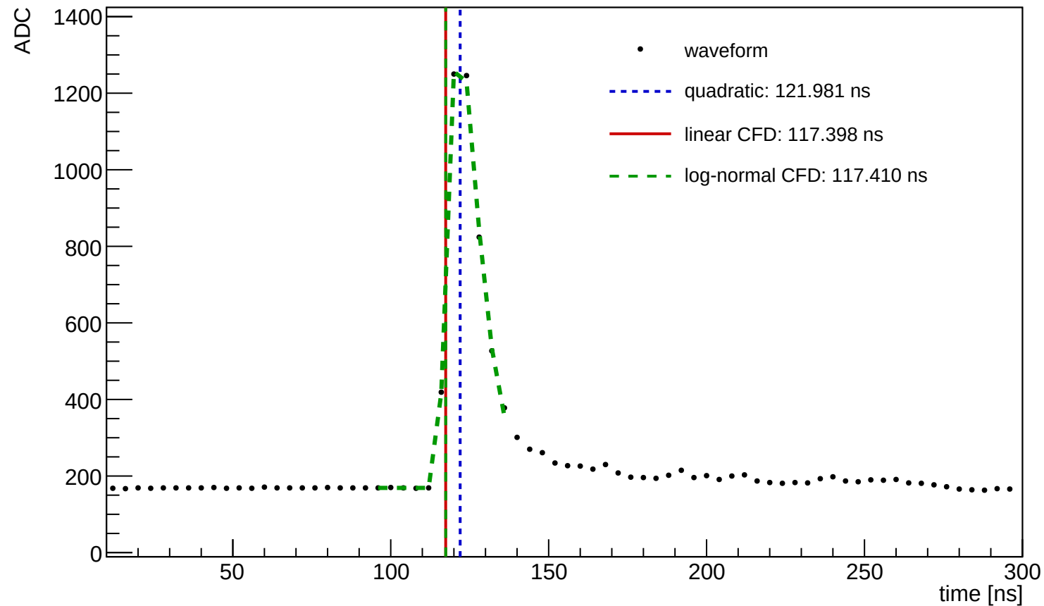
Waveform Time Demo (entry=329, ch=2, module=3004, trigger=SUM)
