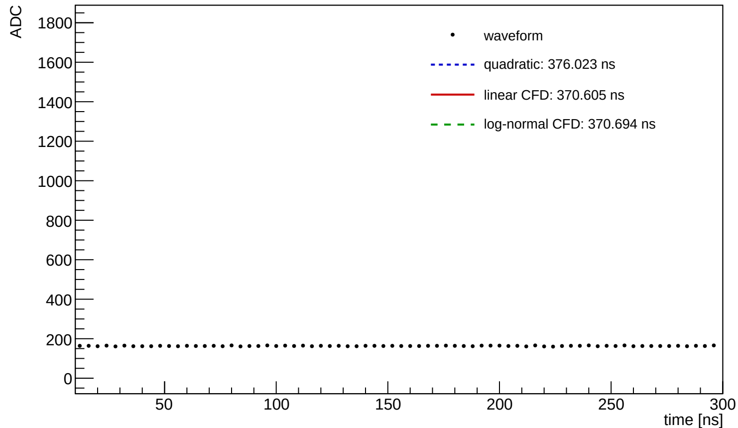
Waveform Time Demo (entry=1616, ch=1, module=3002, trigger=SUM)
