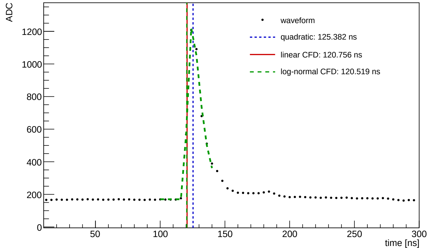
Waveform Time Demo (entry=1207, ch=2, module=3004, trigger=SUM)
