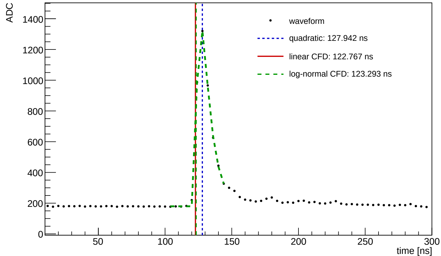
Waveform Time Demo (entry=1573, ch=6, module=3003, trigger=SUM)
