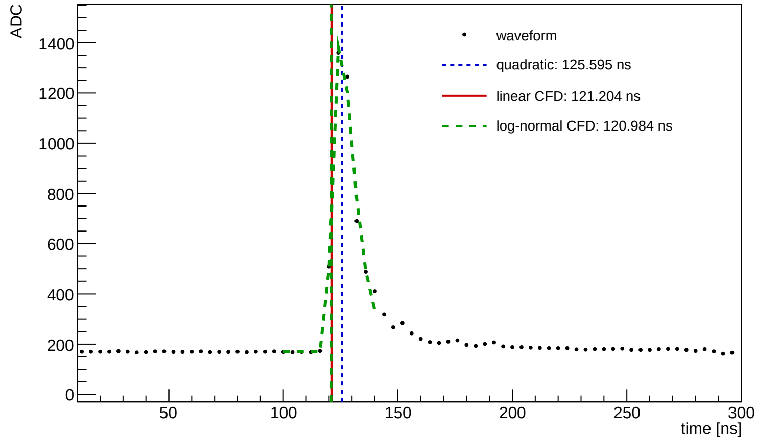
Waveform Time Demo (entry=1098, ch=17, module=3004, trigger=SUM)
