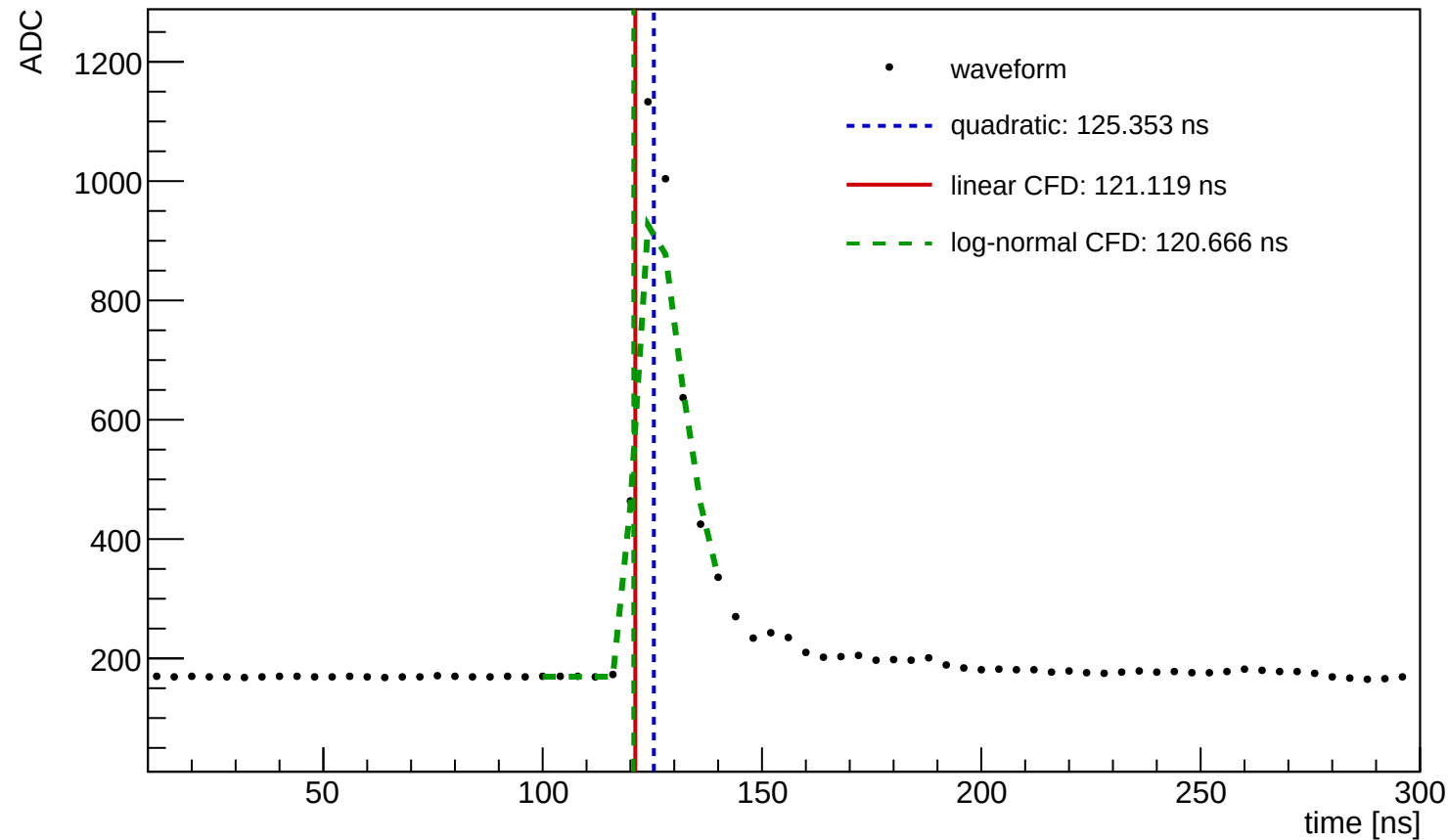
Waveform Time Demo (entry=618, ch=3, module=3004, trigger=SUM)
