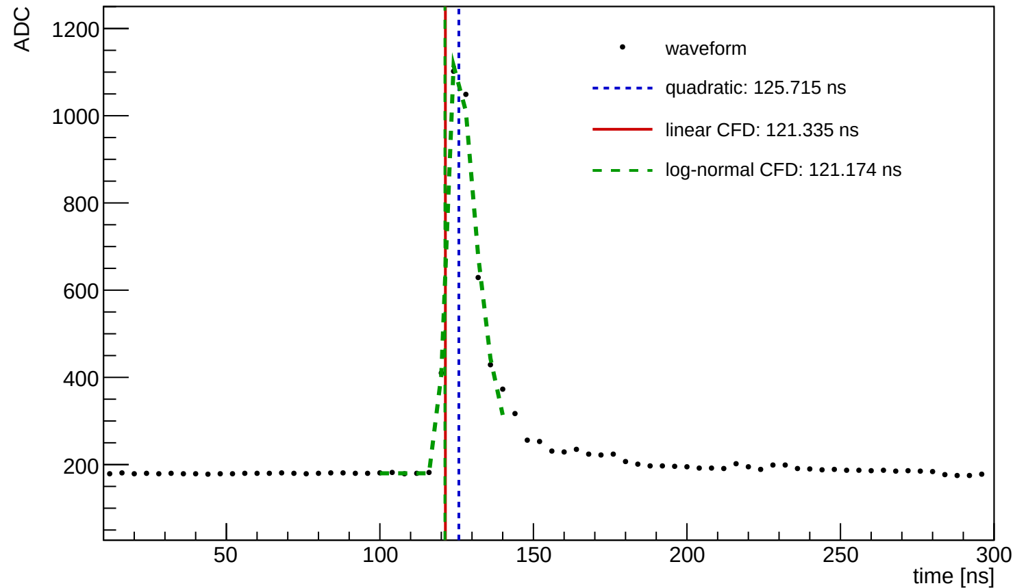
Waveform Time Demo (entry=331, ch=3, module=3003, trigger=SUM)
