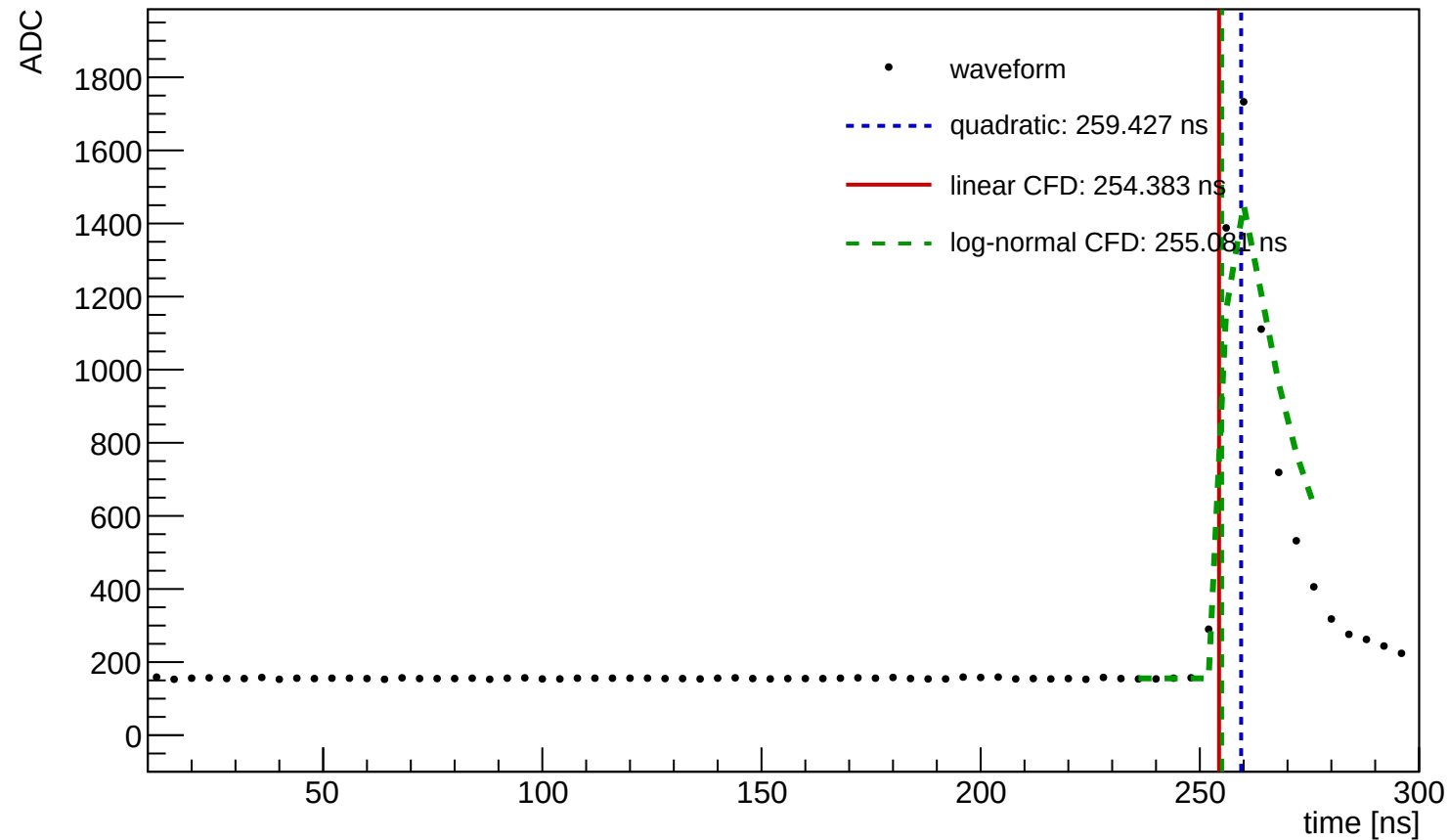
Waveform Time Demo (entry=361, ch=0, module=3001, trigger=SUM)
