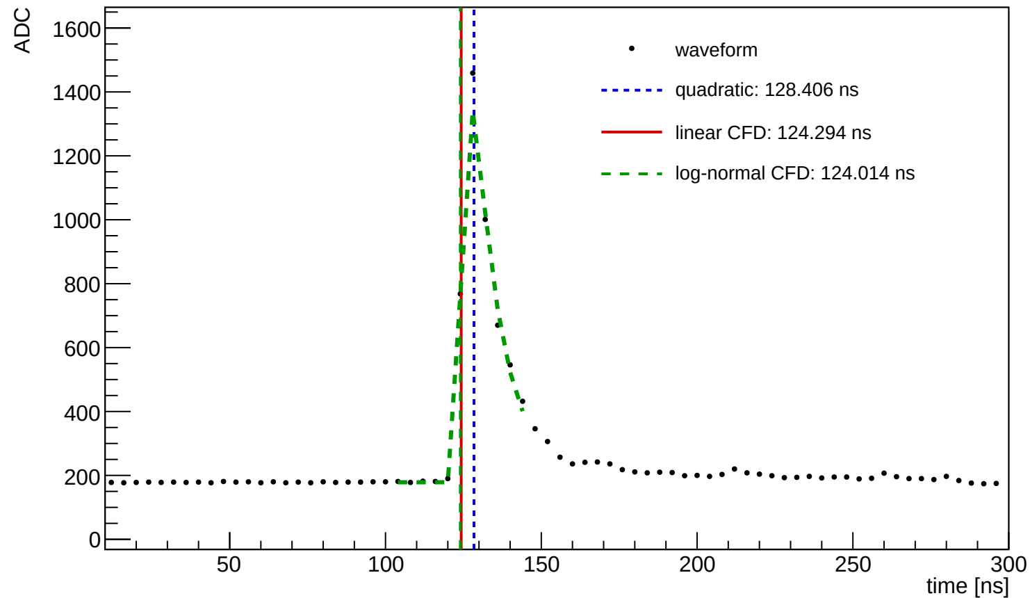
Waveform Time Demo (entry=1113, ch=3, module=3003, trigger=SUM)
