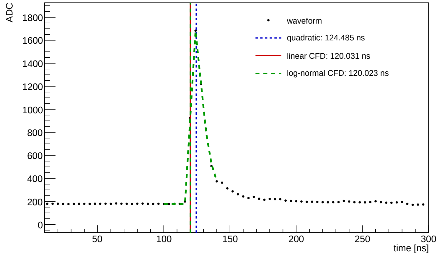
Waveform Time Demo (entry=1114, ch=10, module=3003, trigger=SUM)
