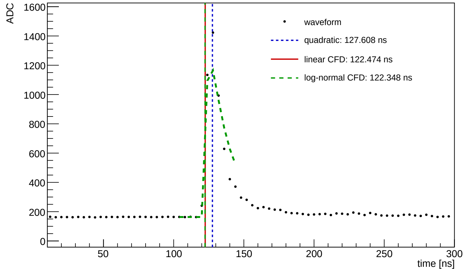
Waveform Time Demo (entry=393, ch=3, module=3002, trigger=SUM)
