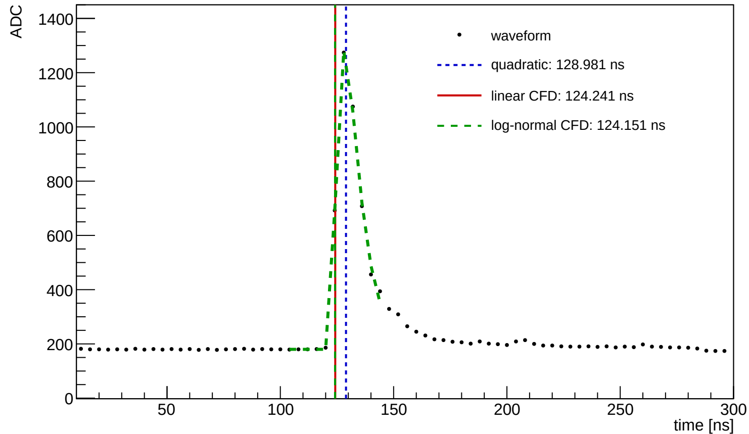
Waveform Time Demo (entry=243, ch=12, module=3003, trigger=SUM)
