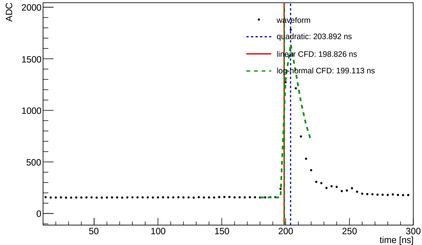
Waveform Time Demo (entry=1312, ch=2, module=3001, trigger=SUM)
