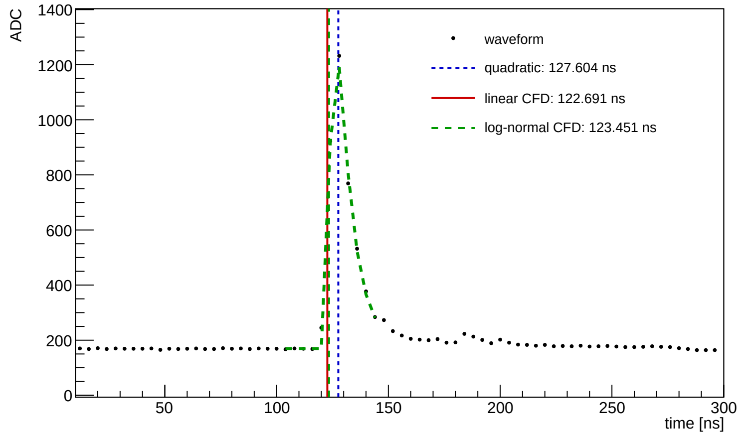
Waveform Time Demo (entry=1345, ch=1, module=3004, trigger=SUM)
