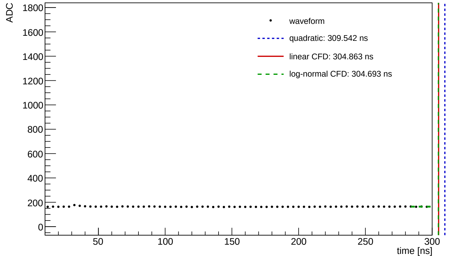
Waveform Time Demo (entry=814, ch=1, module=3002, trigger=SUM)
