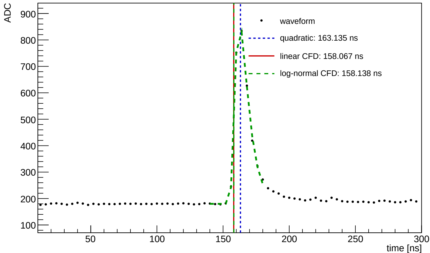
Waveform Time Demo (entry=367, ch=5, module=3003, trigger=SUM)
