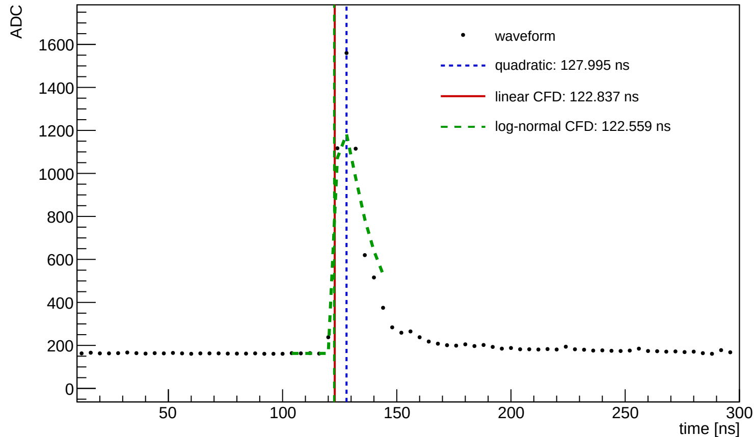
Waveform Time Demo (entry=1487, ch=0, module=3002, trigger=SUM)
