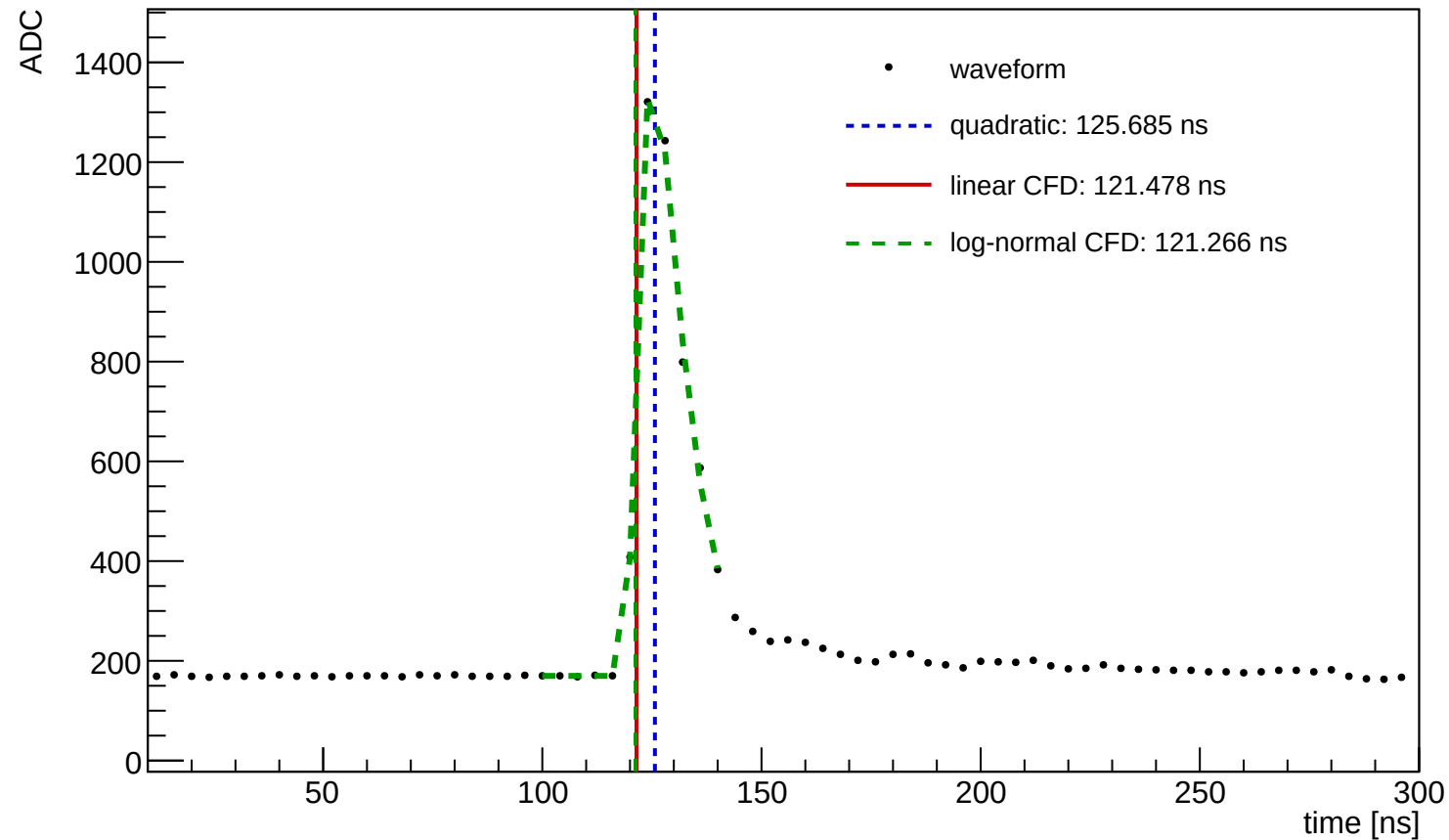
Waveform Time Demo (entry=1136, ch=4, module=3004, trigger=SUM)
