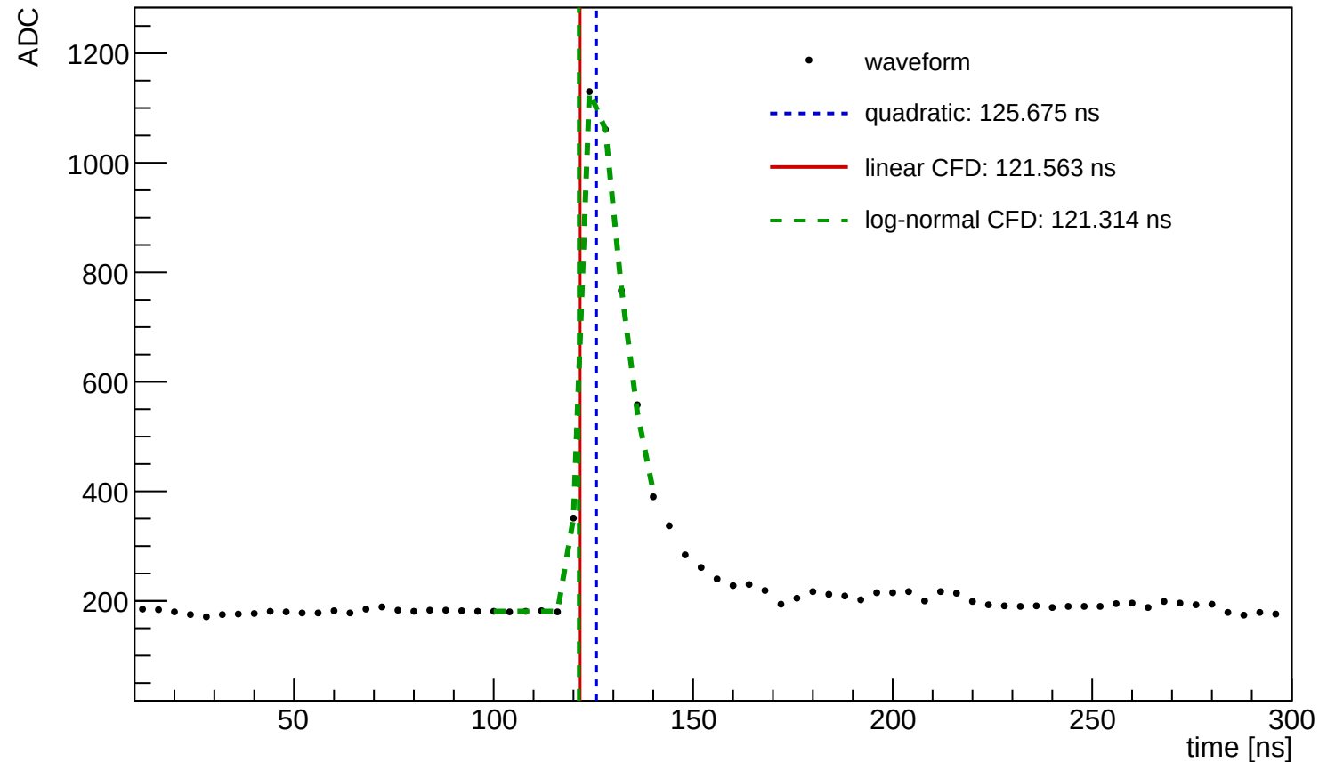
Waveform Time Demo (entry=1563, ch=11, module=3003, trigger=SUM)
