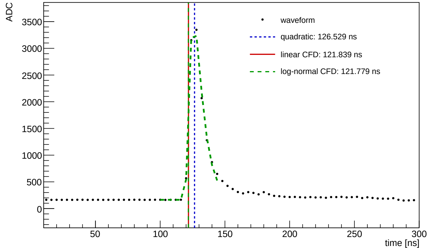
Waveform Time Demo (entry=133, ch=2, module=3002, trigger=SUM)
