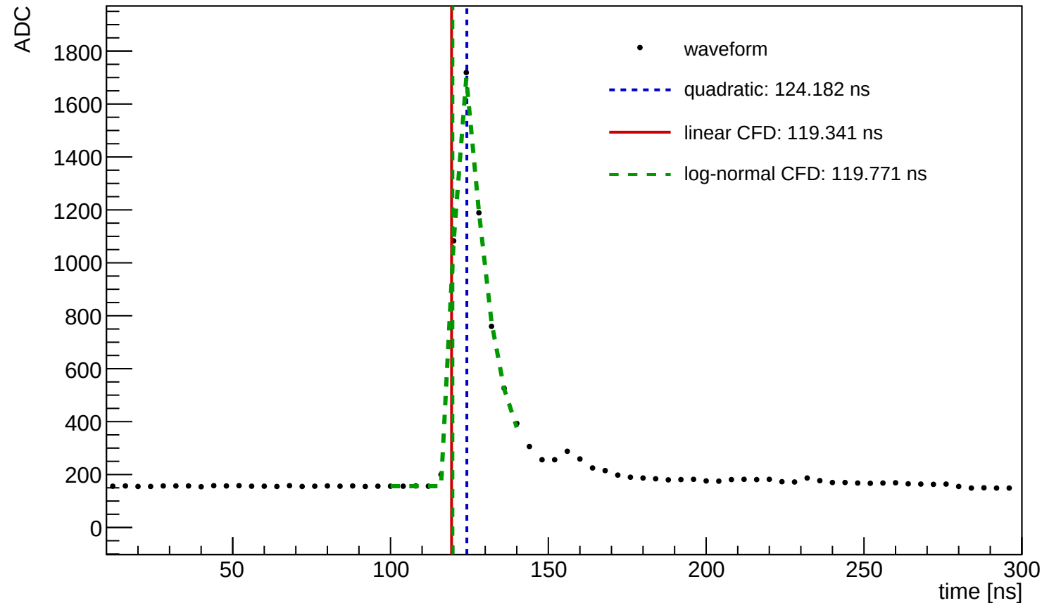
Waveform Time Demo (entry=338, ch=4, module=3001, trigger=SUM)
