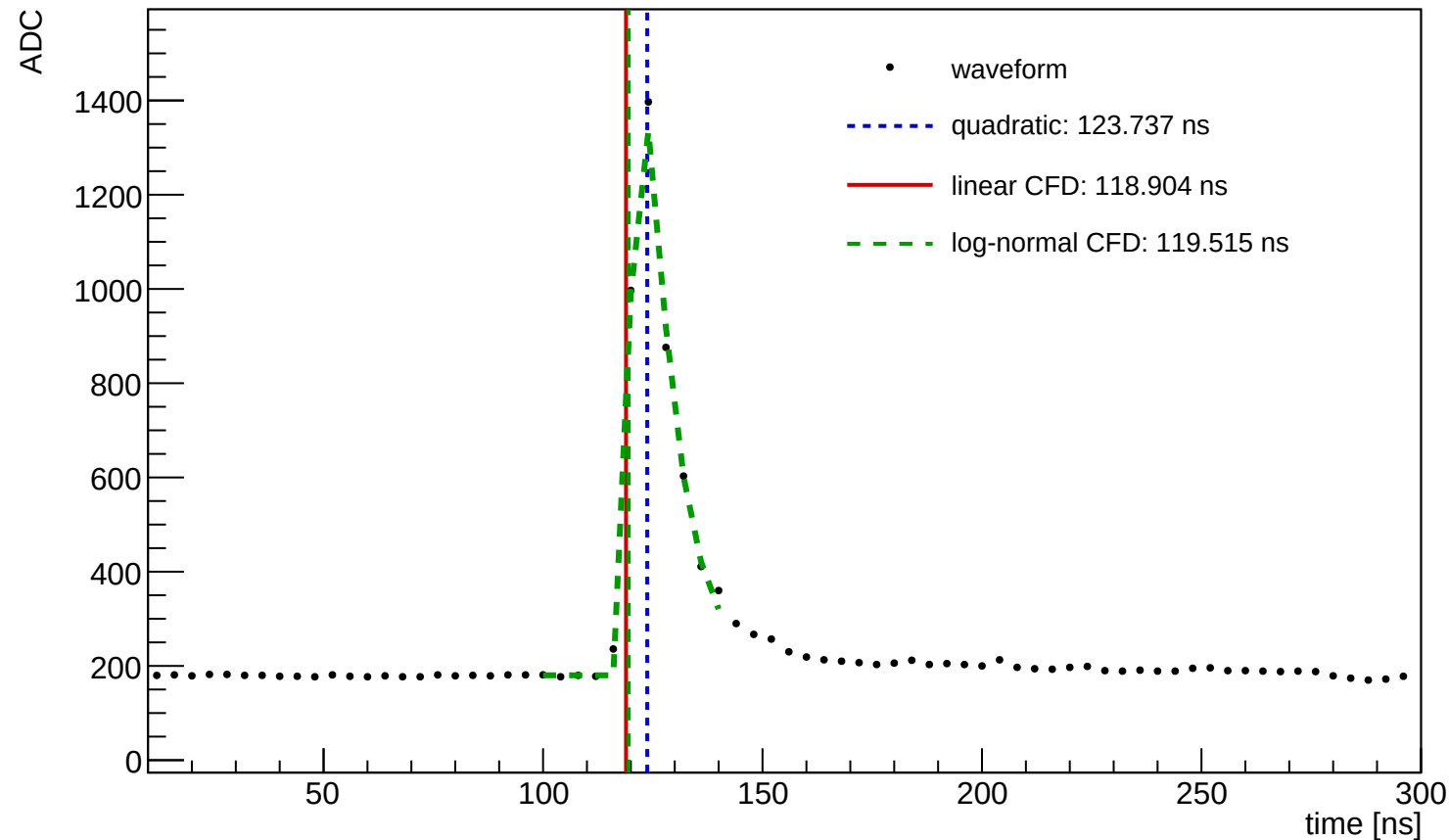
Waveform Time Demo (entry=40, ch=3, module=3003, trigger=SUM)
