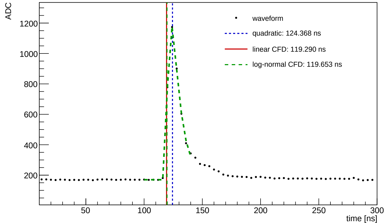
Waveform Time Demo (entry=265, ch=3, module=3004, trigger=SUM)
