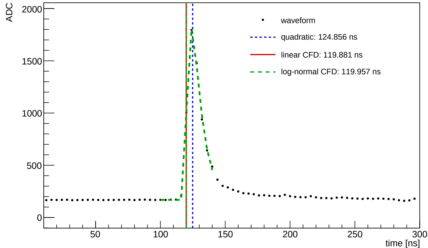
Waveform Time Demo (entry=850, ch=2, module=3004, trigger=SUM)
