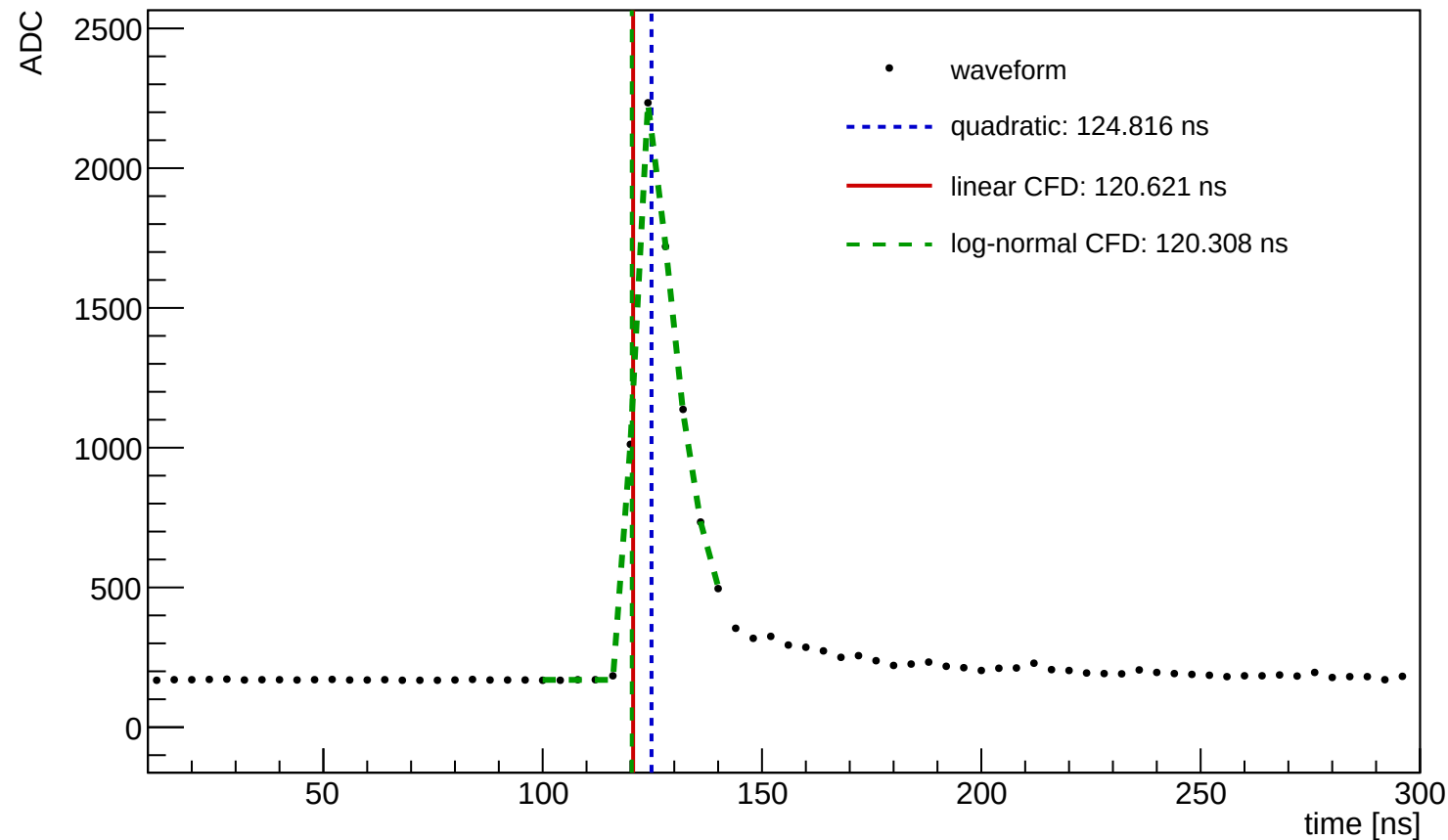
Waveform Time Demo (entry=83, ch=5, module=3004, trigger=SUM)
