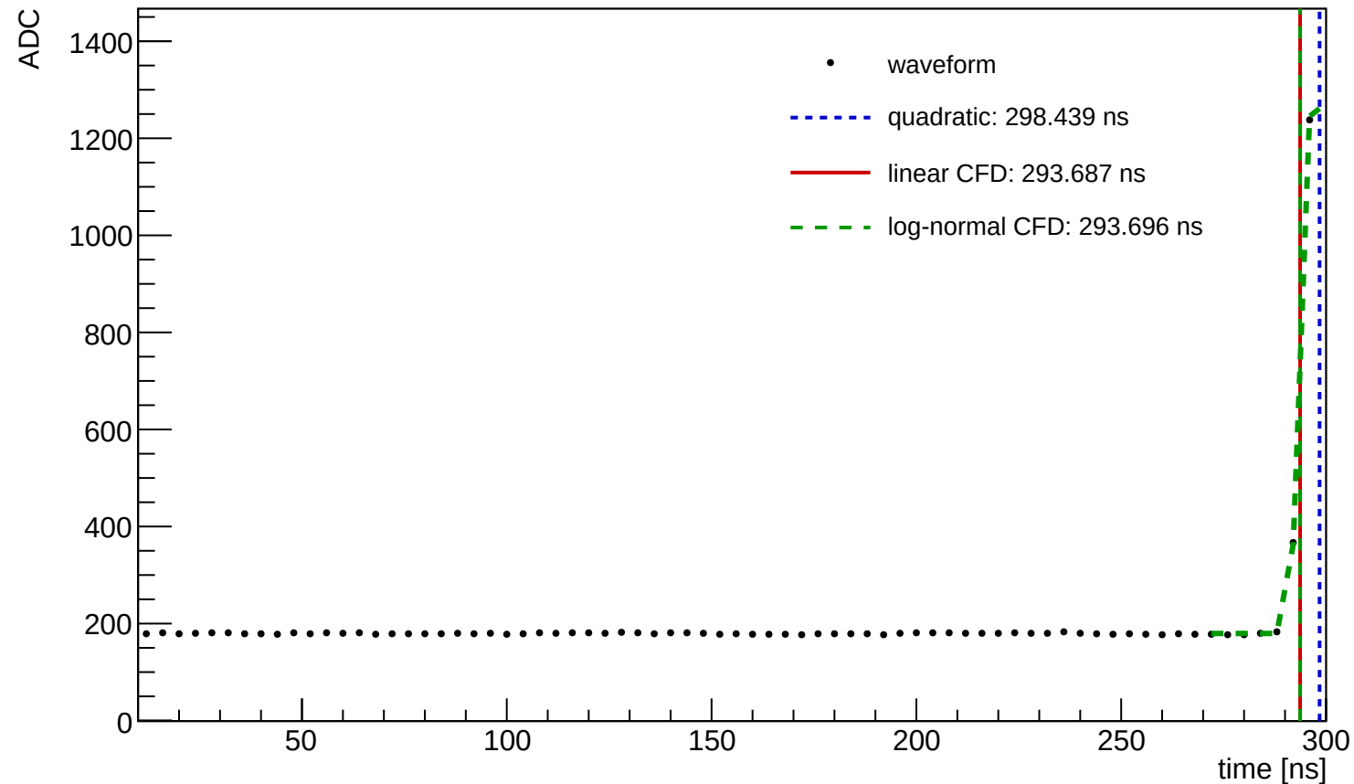
Waveform Time Demo (entry=1144, ch=0, module=3003, trigger=SUM)
