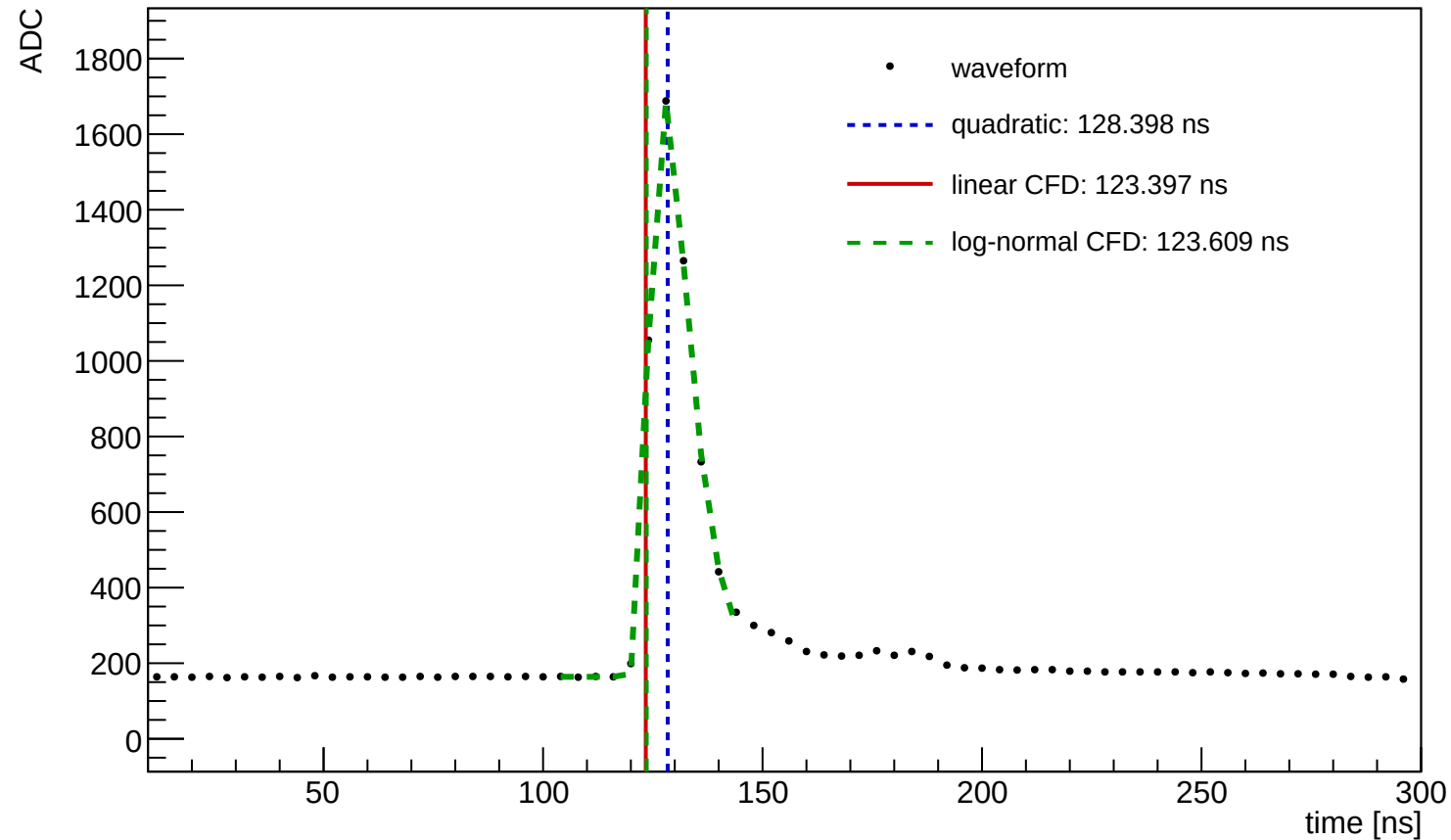
Waveform Time Demo (entry=429, ch=0, module=3002, trigger=SUM)
