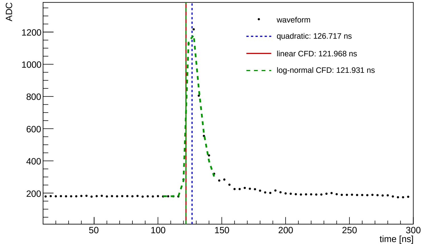
Waveform Time Demo (entry=197, ch=1, module=3003, trigger=SUM)
