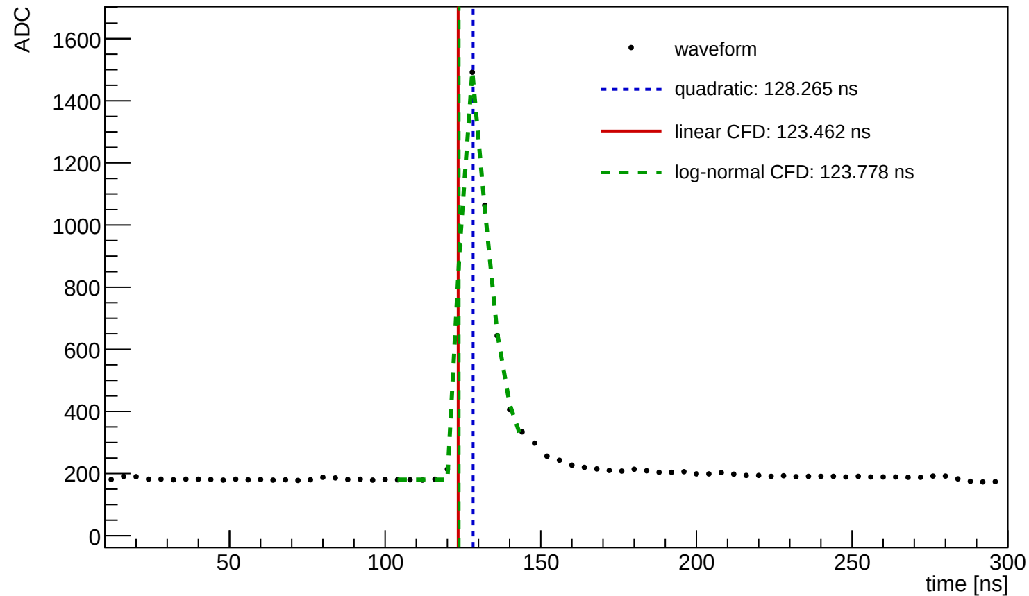
Waveform Time Demo (entry=420, ch=8, module=3003, trigger=SUM)
