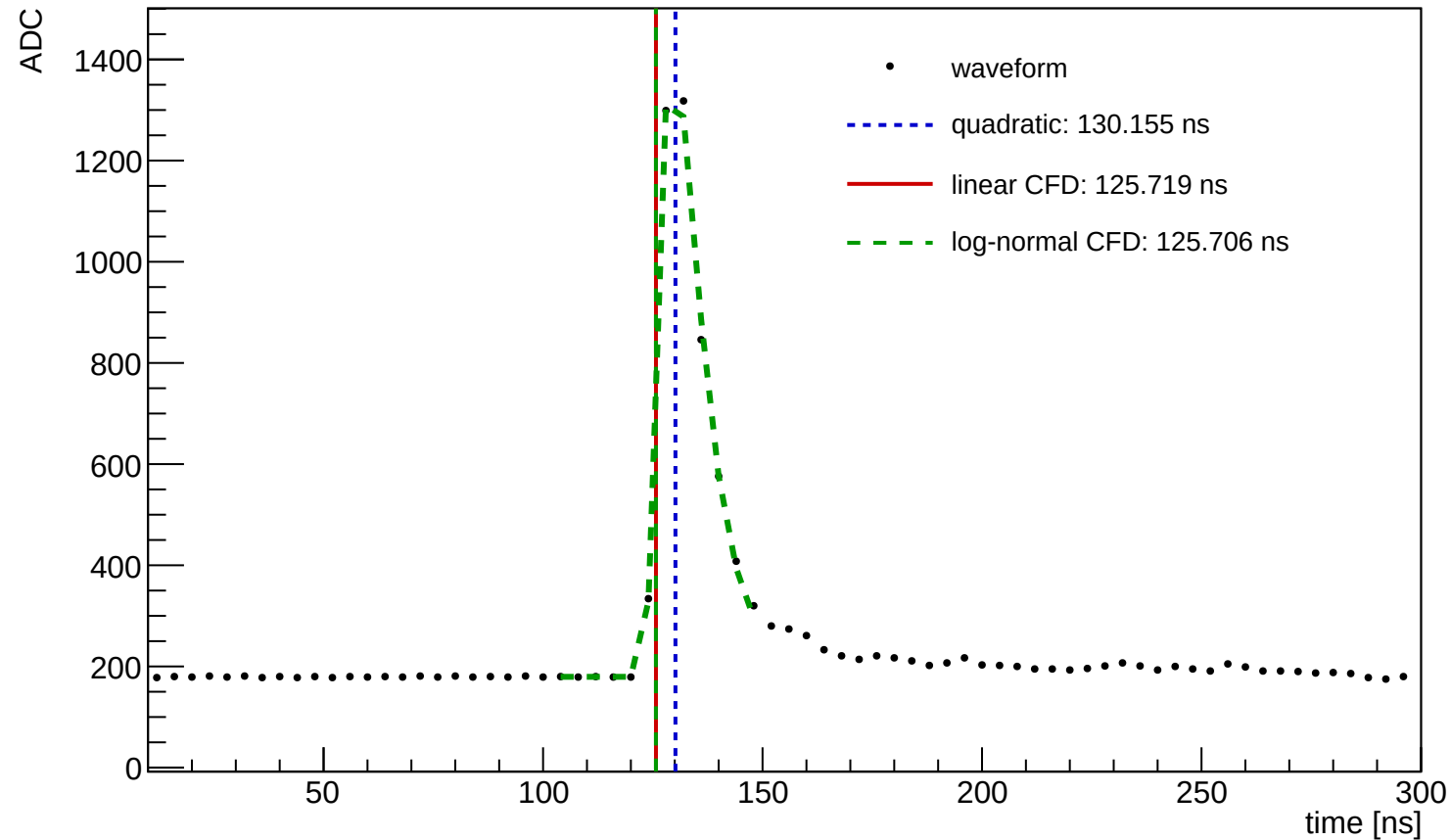
Waveform Time Demo (entry=1356, ch=7, module=3003, trigger=SUM)
