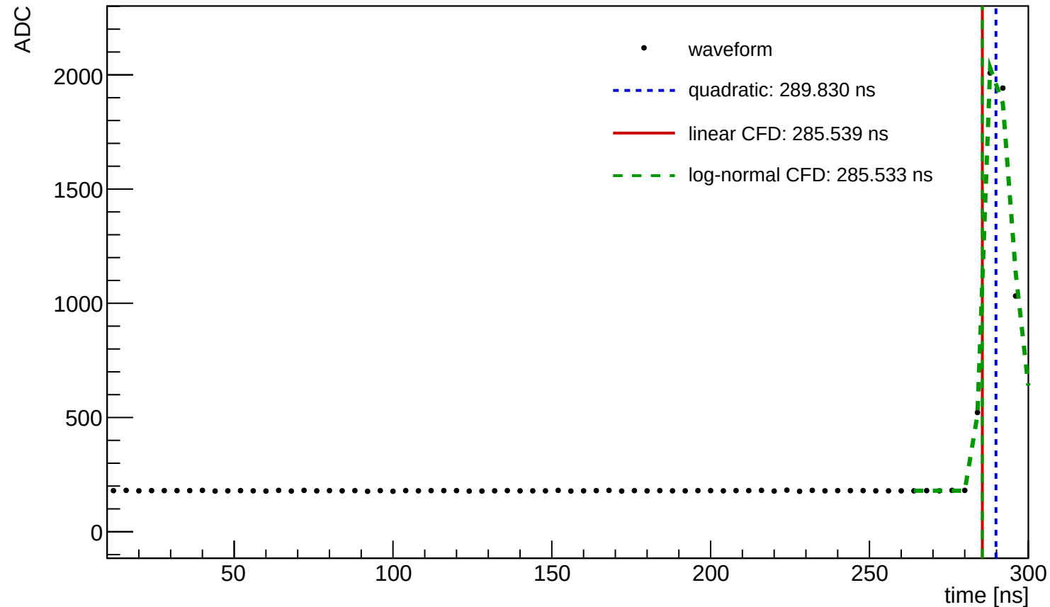
Waveform Time Demo (entry=632, ch=4, module=3003, trigger=SUM)
