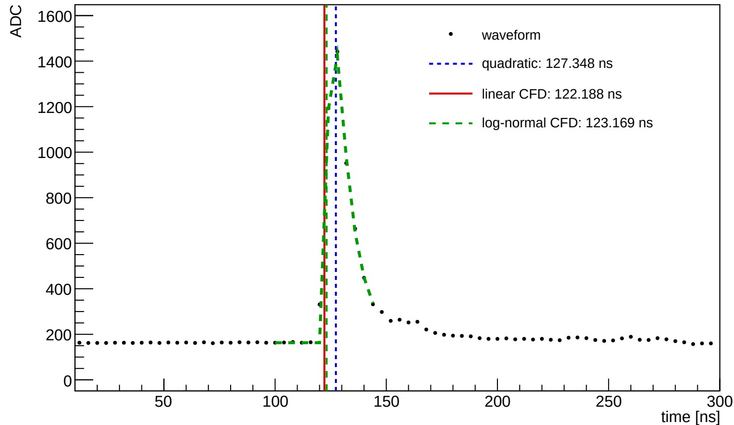
Waveform Time Demo (entry=1068, ch=0, module=3002, trigger=SUM)
