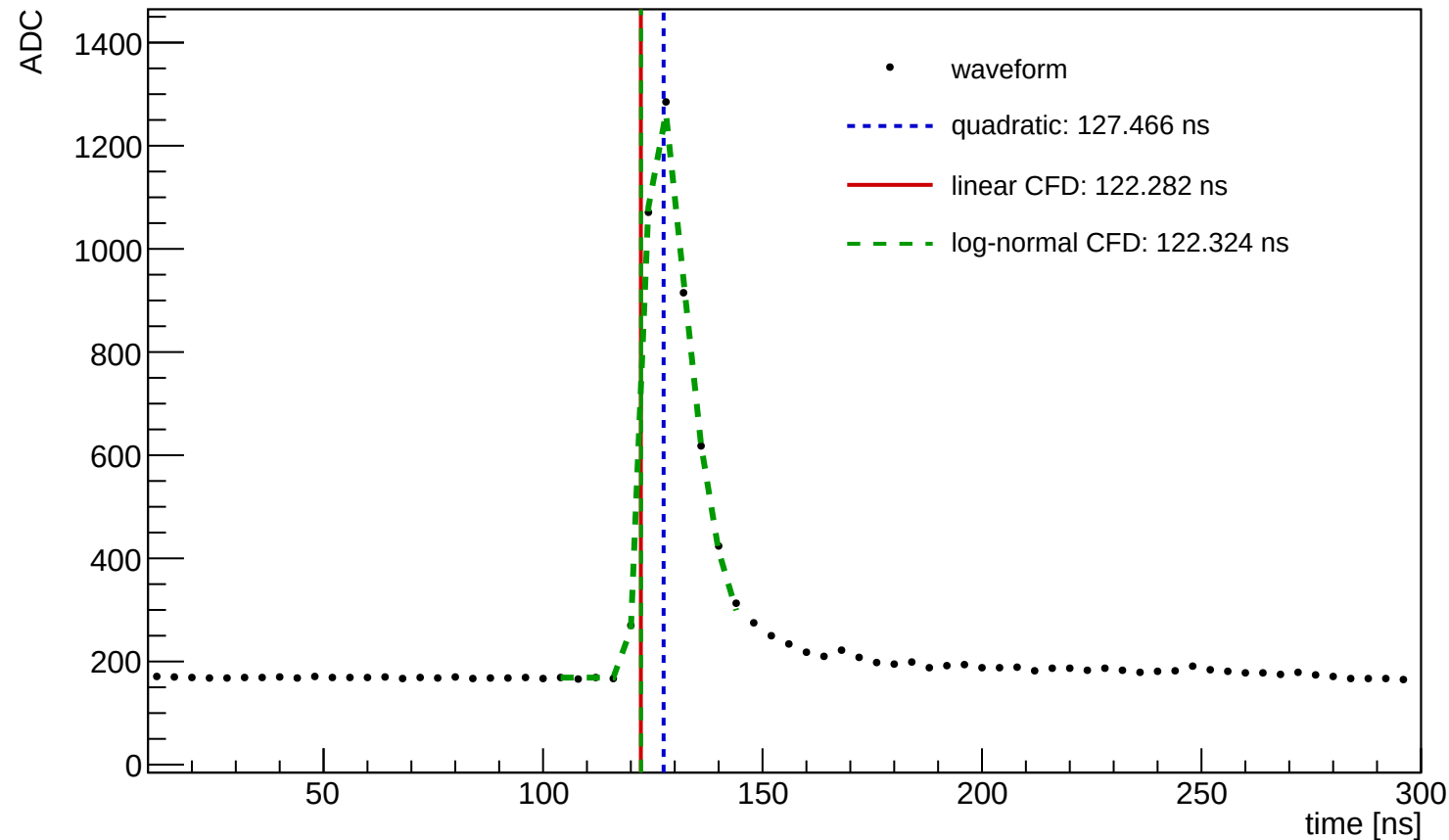
Waveform Time Demo (entry=262, ch=1, module=3004, trigger=SUM)
