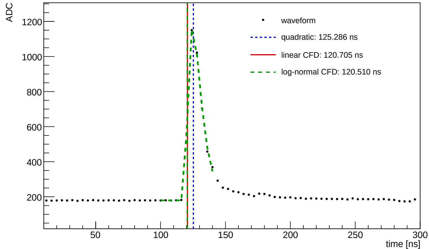
Waveform Time Demo (entry=11, ch=0, module=3003, trigger=SUM)
