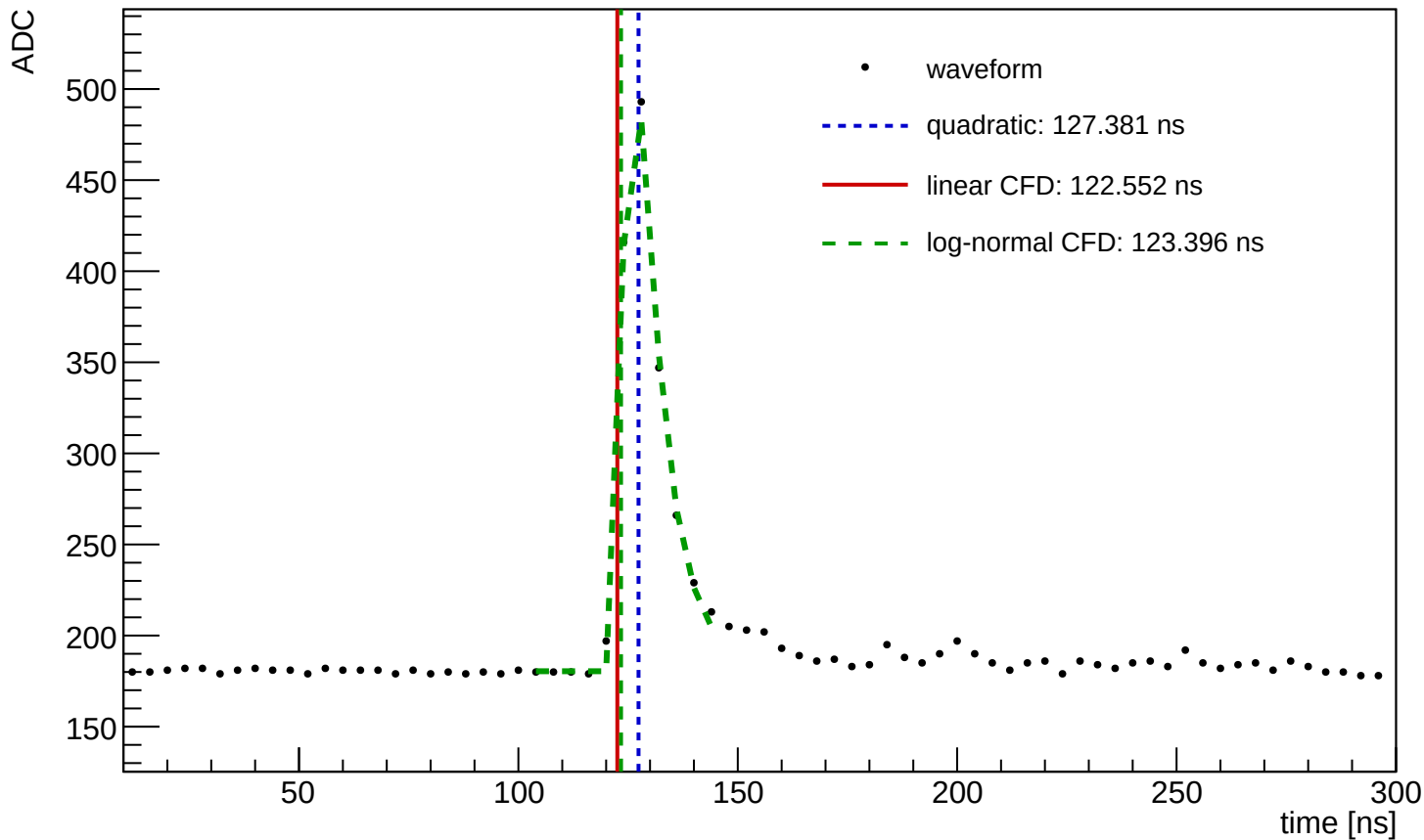
Waveform Time Demo (entry=1532, ch=4, module=3003, trigger=SUM)
