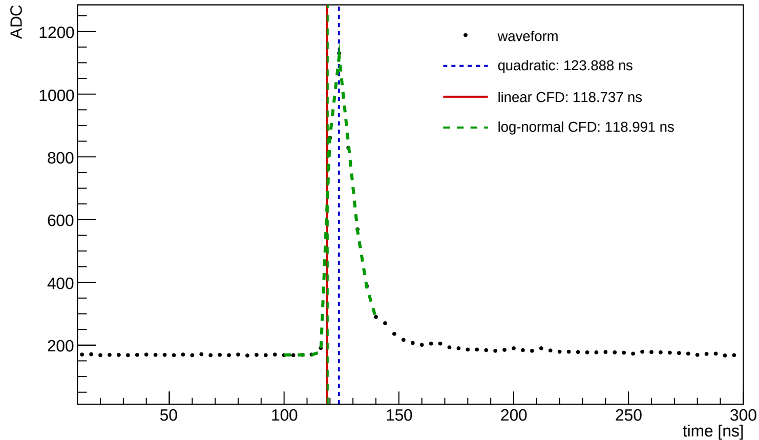
Waveform Time Demo (entry=678, ch=2, module=3004, trigger=SUM)
