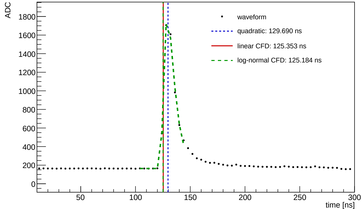
Waveform Time Demo (entry=1016, ch=5, module=3002, trigger=SUM)
