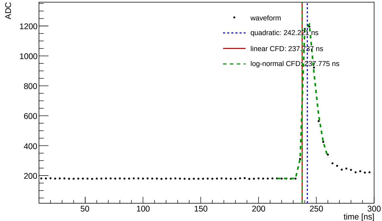
Waveform Time Demo (entry=1156, ch=5, module=3003, trigger=SUM)
