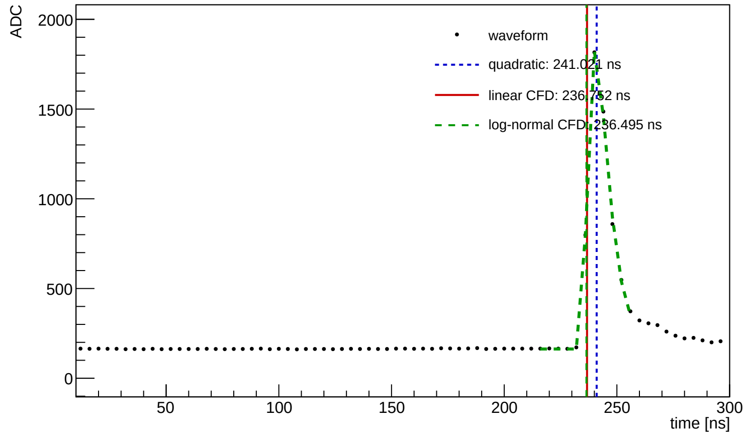
Waveform Time Demo (entry=1156, ch=4, module=3002, trigger=SUM)
