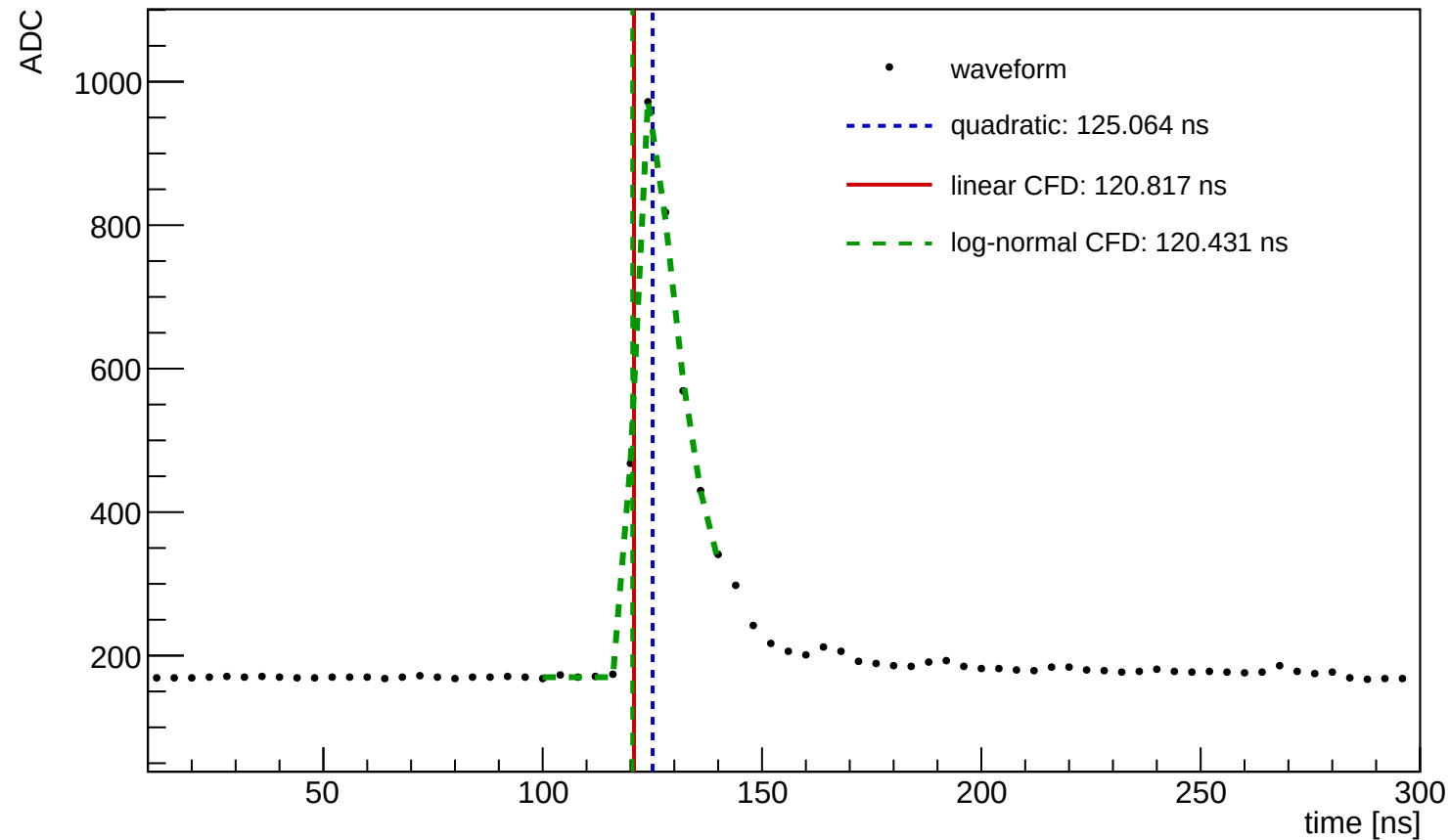
Waveform Time Demo (entry=933, ch=13, module=3004, trigger=SUM)
