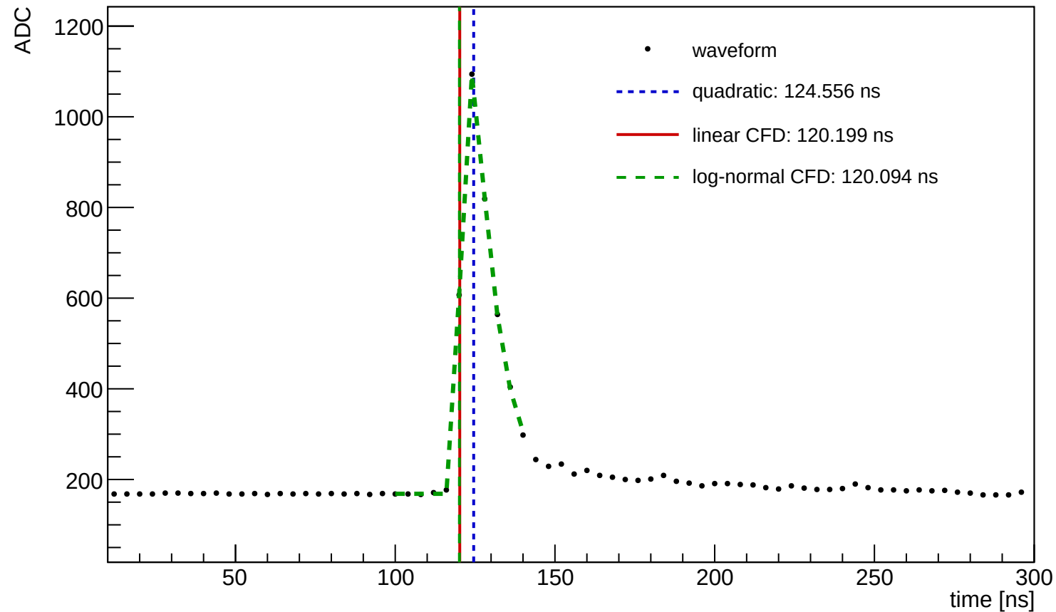
Waveform Time Demo (entry=1319, ch=0, module=3004, trigger=SUM)
