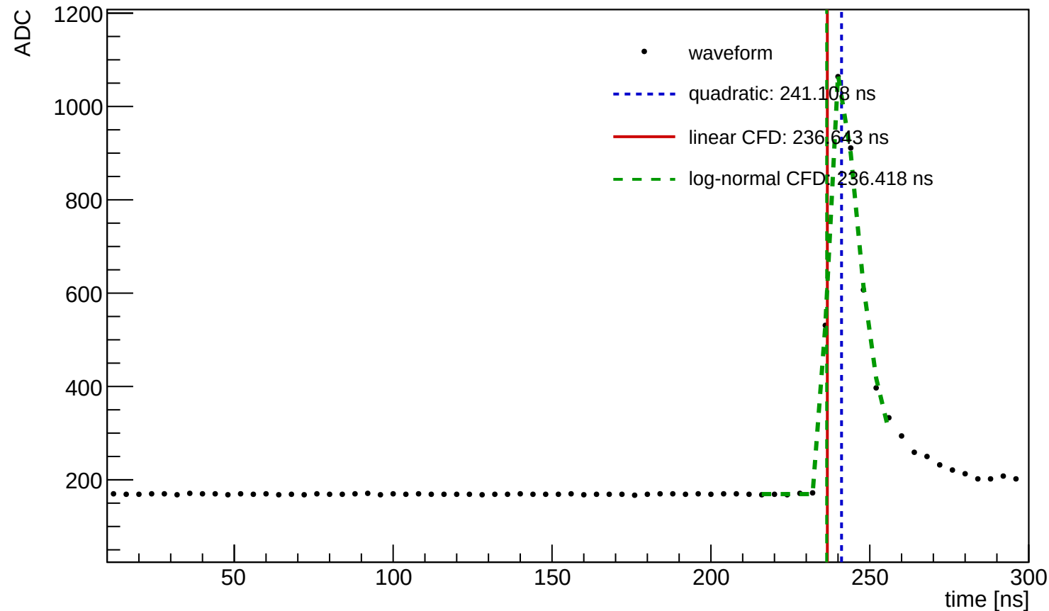
Waveform Time Demo (entry=319, ch=8, module=3004, trigger=SUM)
