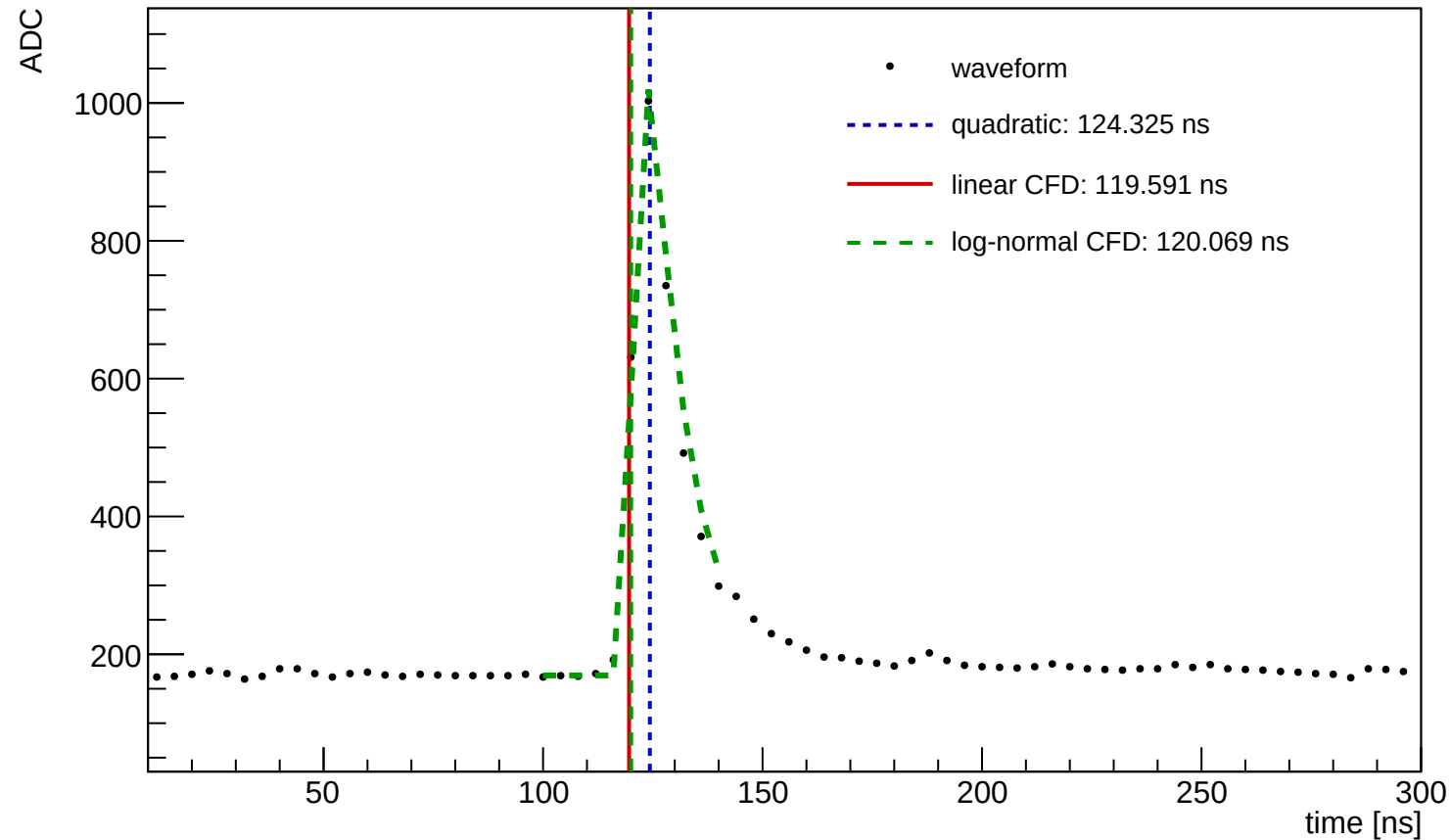
Waveform Time Demo (entry=1304, ch=1, module=3004, trigger=SUM)
