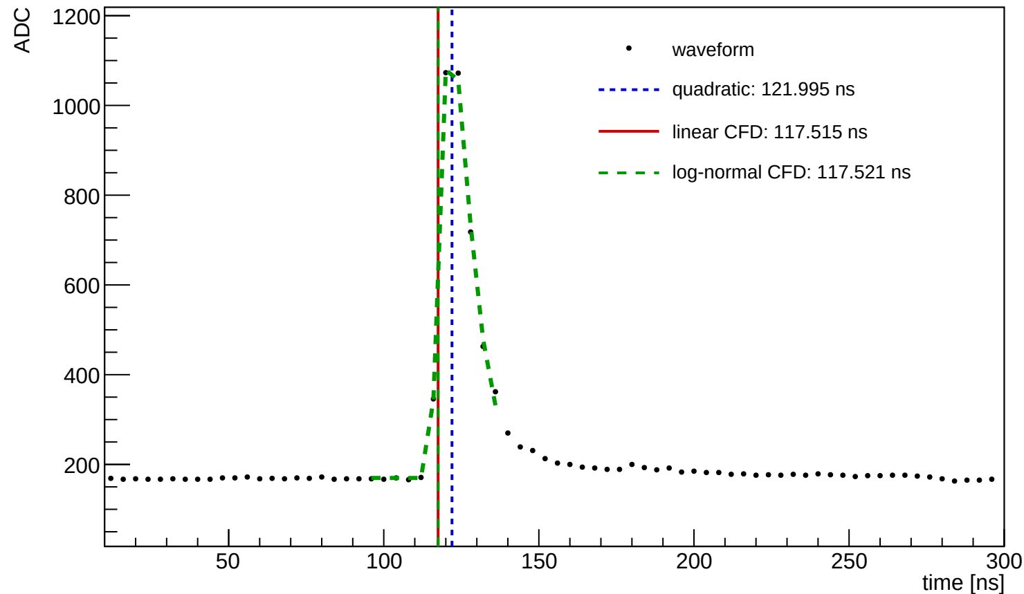
Waveform Time Demo (entry=28, ch=16, module=3004, trigger=SUM)
