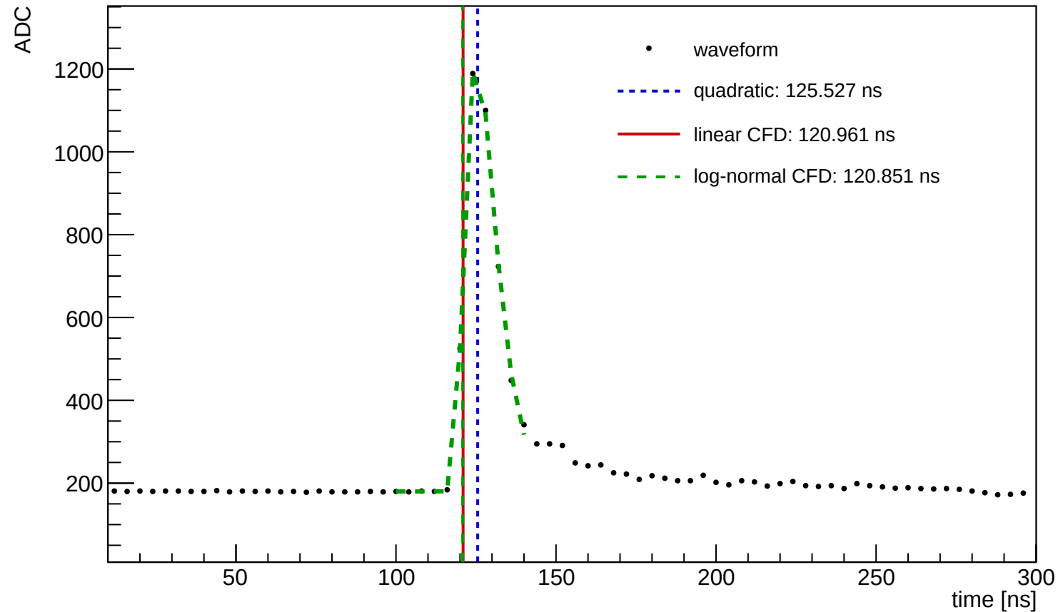
Waveform Time Demo (entry=1514, ch=0, module=3003, trigger=SUM)
