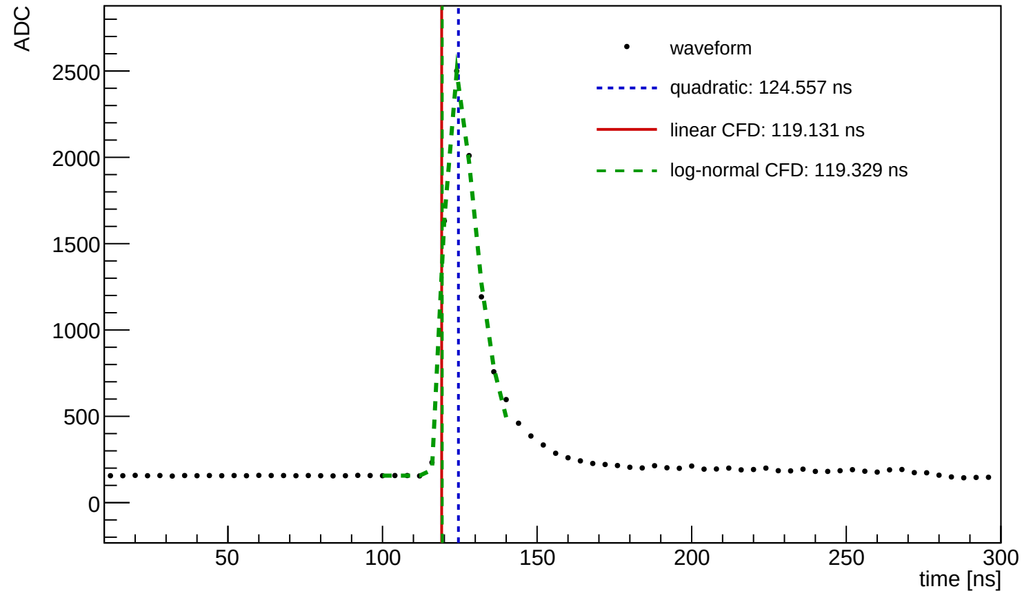
Waveform Time Demo (entry=1510, ch=5, module=3001, trigger=SUM)
