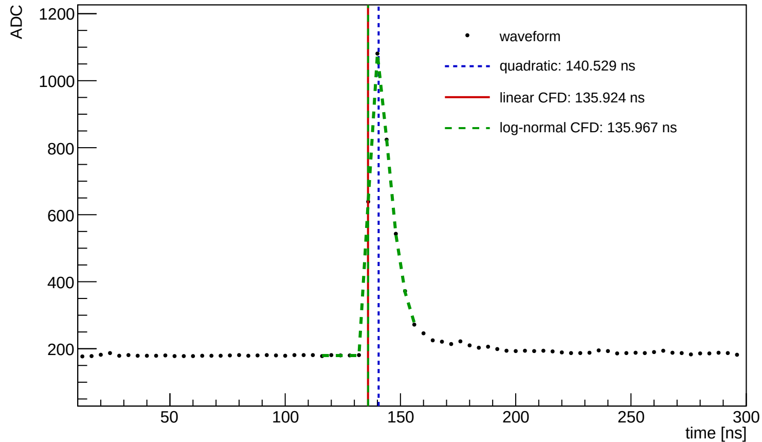
Waveform Time Demo (entry=729, ch=8, module=3003, trigger=SUM)
