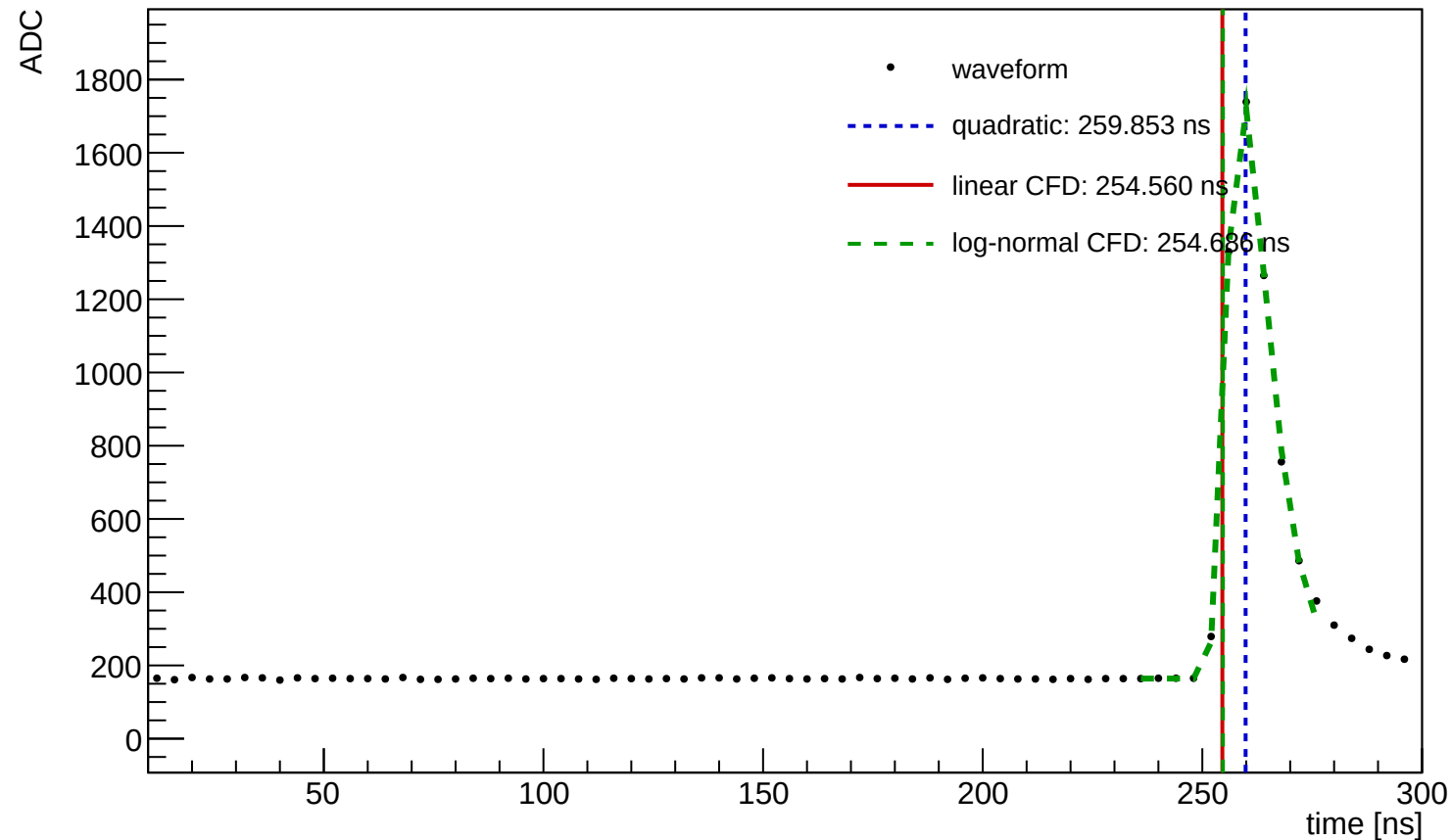
Waveform Time Demo (entry=361, ch=1, module=3002, trigger=SUM)
