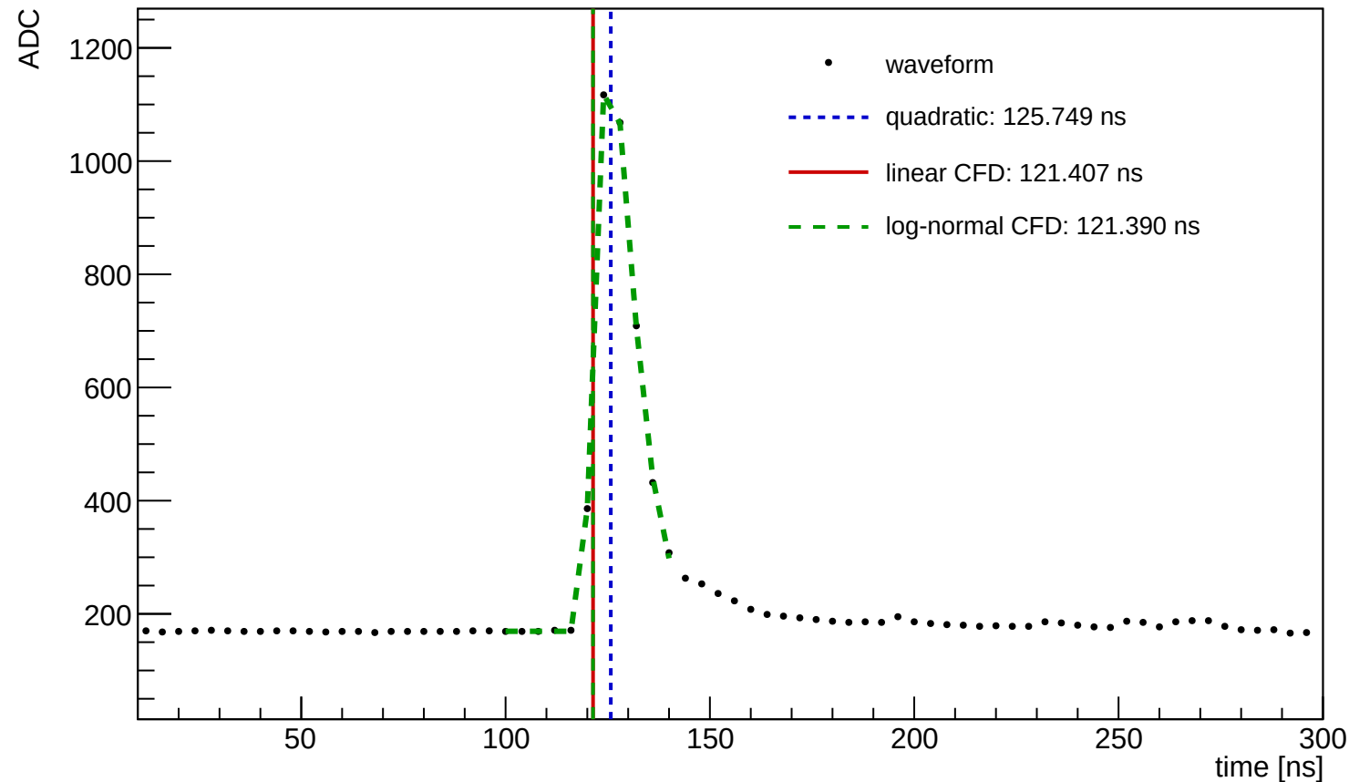
Waveform Time Demo (entry=151, ch=1, module=3004, trigger=SUM)
