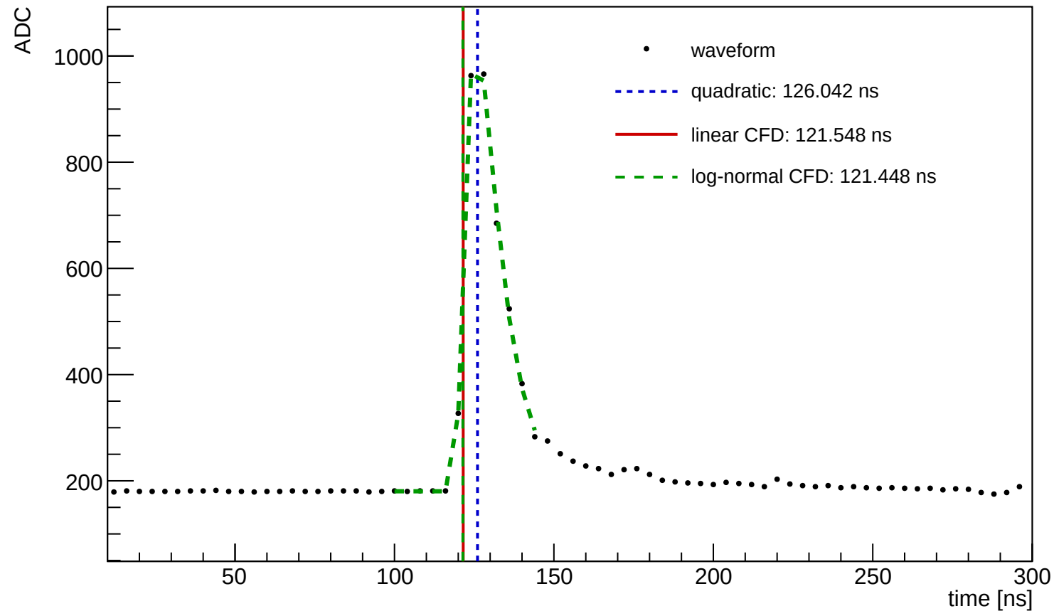
Waveform Time Demo (entry=949, ch=16, module=3003, trigger=SUM)
