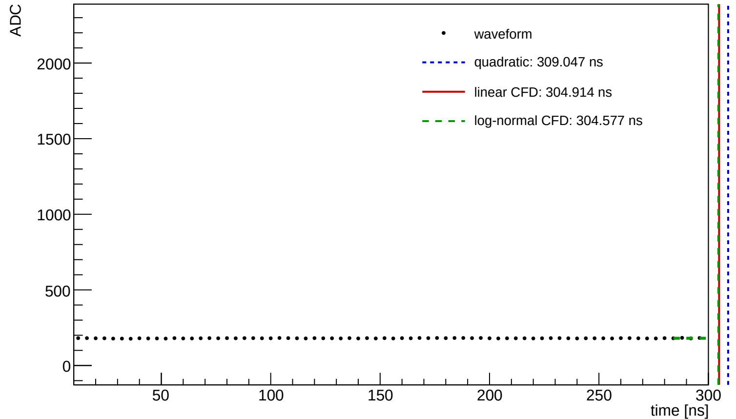
Waveform Time Demo (entry=835, ch=0, module=3003, trigger=SUM)
