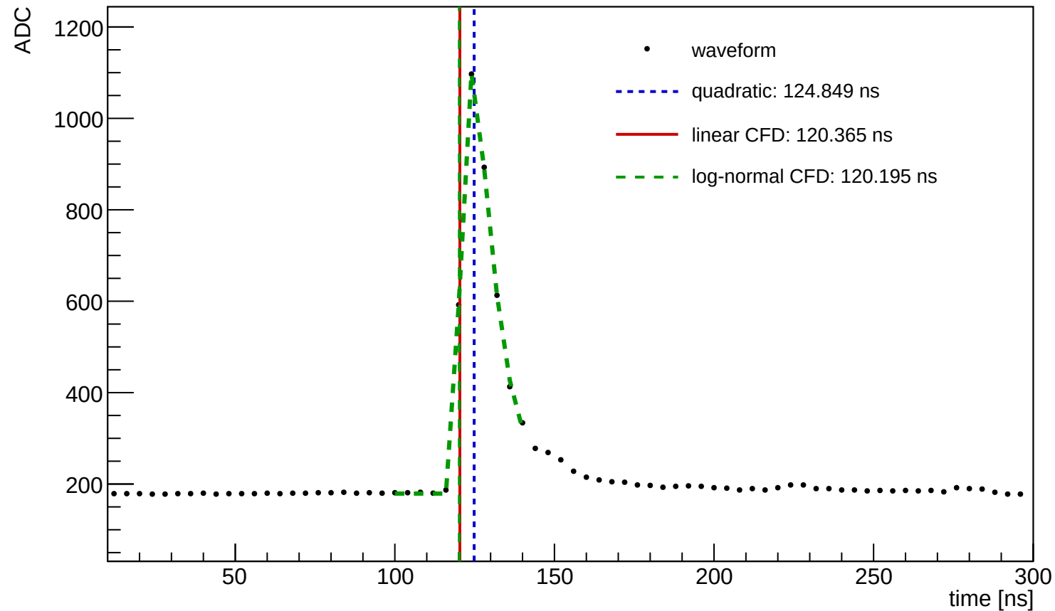
Waveform Time Demo (entry=1320, ch=2, module=3003, trigger=SUM)
