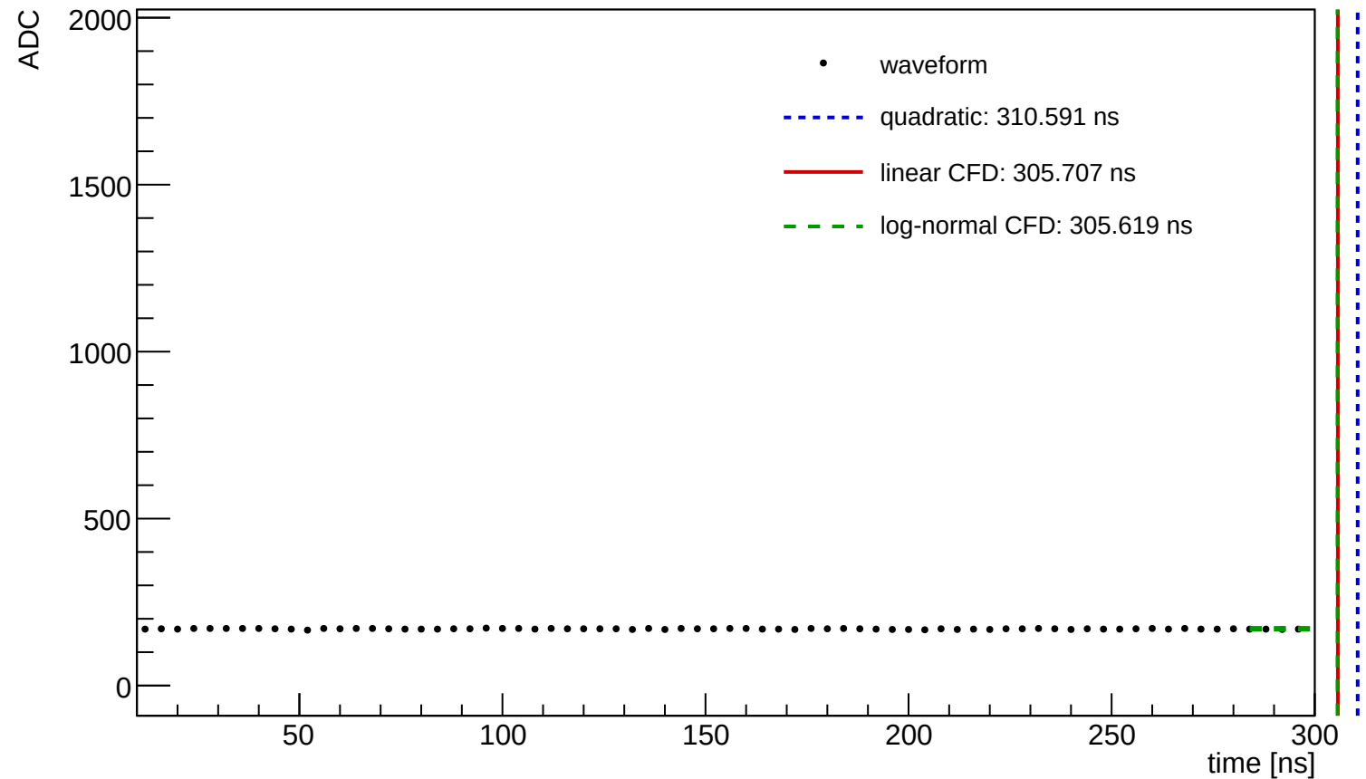
Waveform Time Demo (entry=835, ch=1, module=3004, trigger=SUM)
