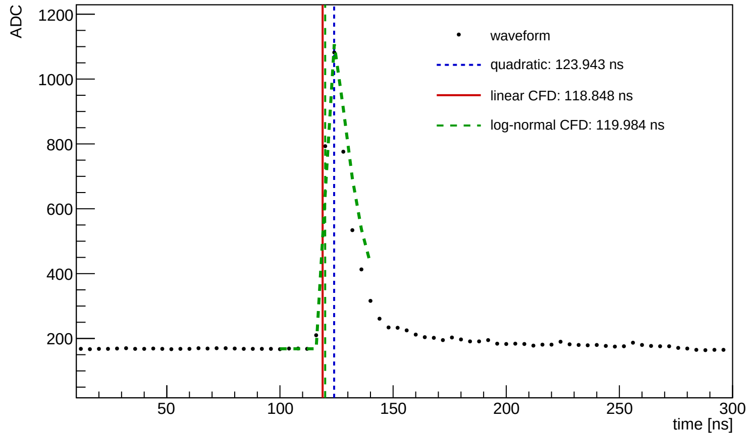
Waveform Time Demo (entry=1533, ch=1, module=3004, trigger=SUM)
