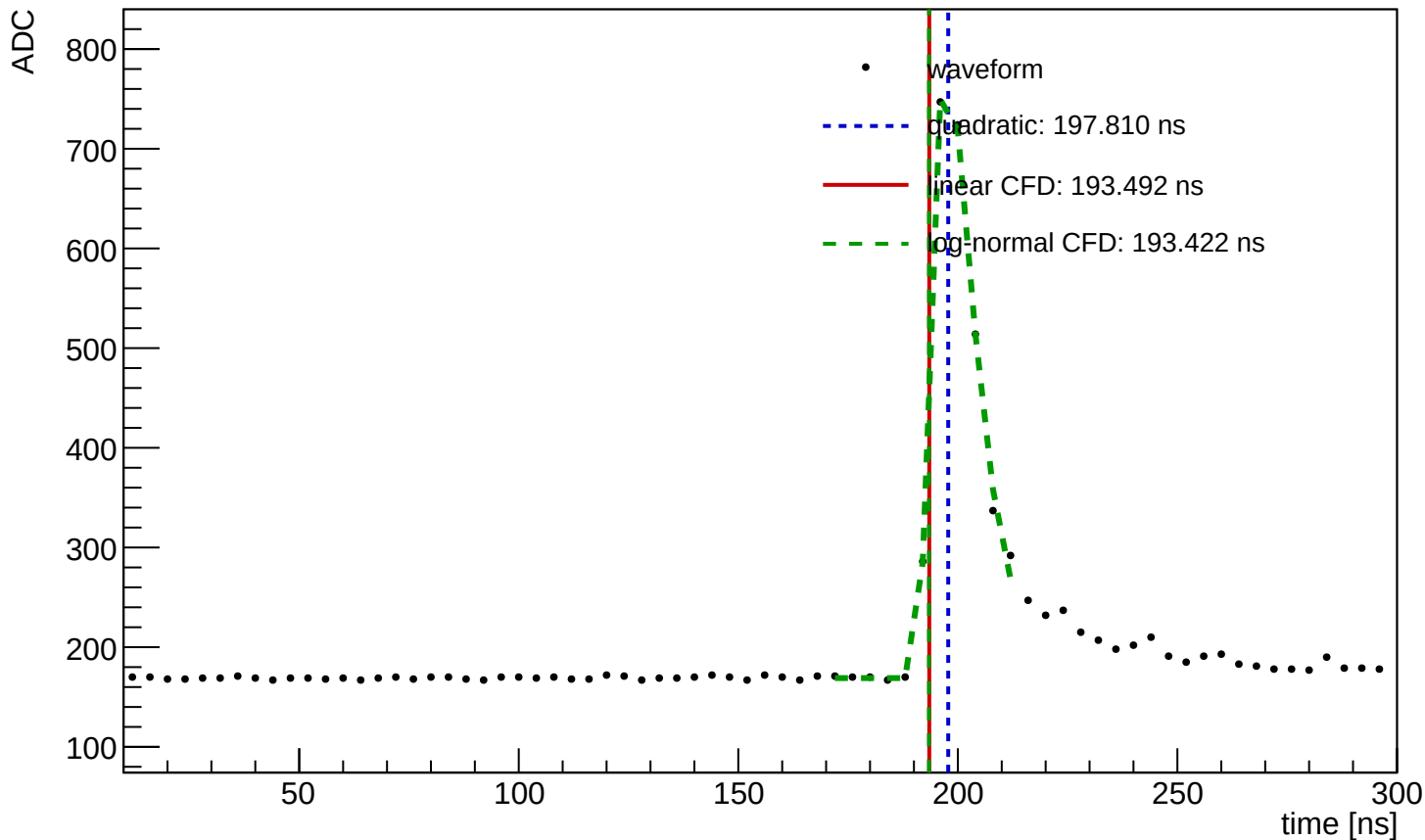
Waveform Time Demo (entry=1639, ch=2, module=3004, trigger=SUM)
