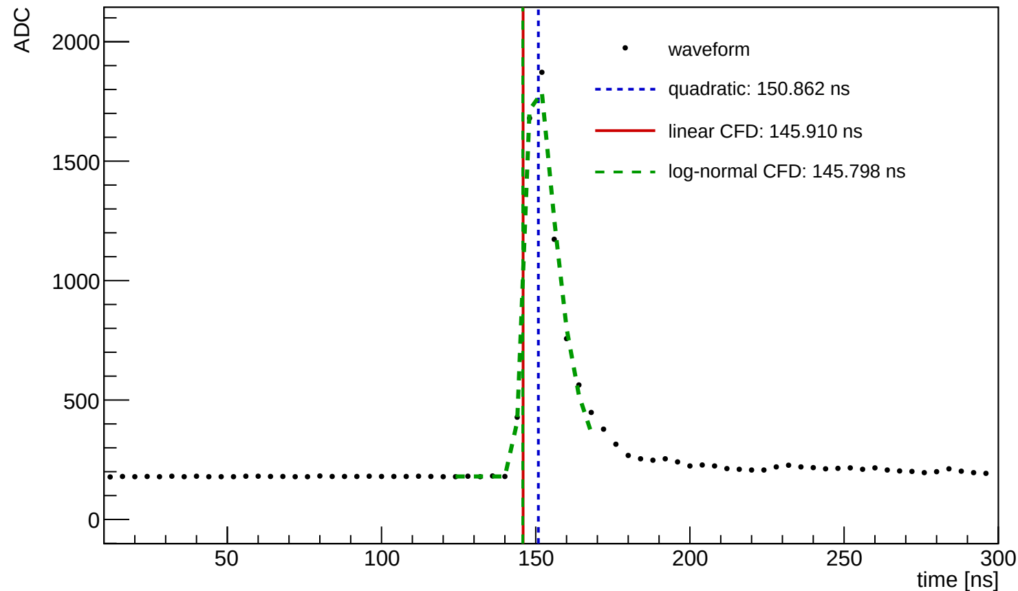
Waveform Time Demo (entry=153, ch=14, module=3003, trigger=SUM)
