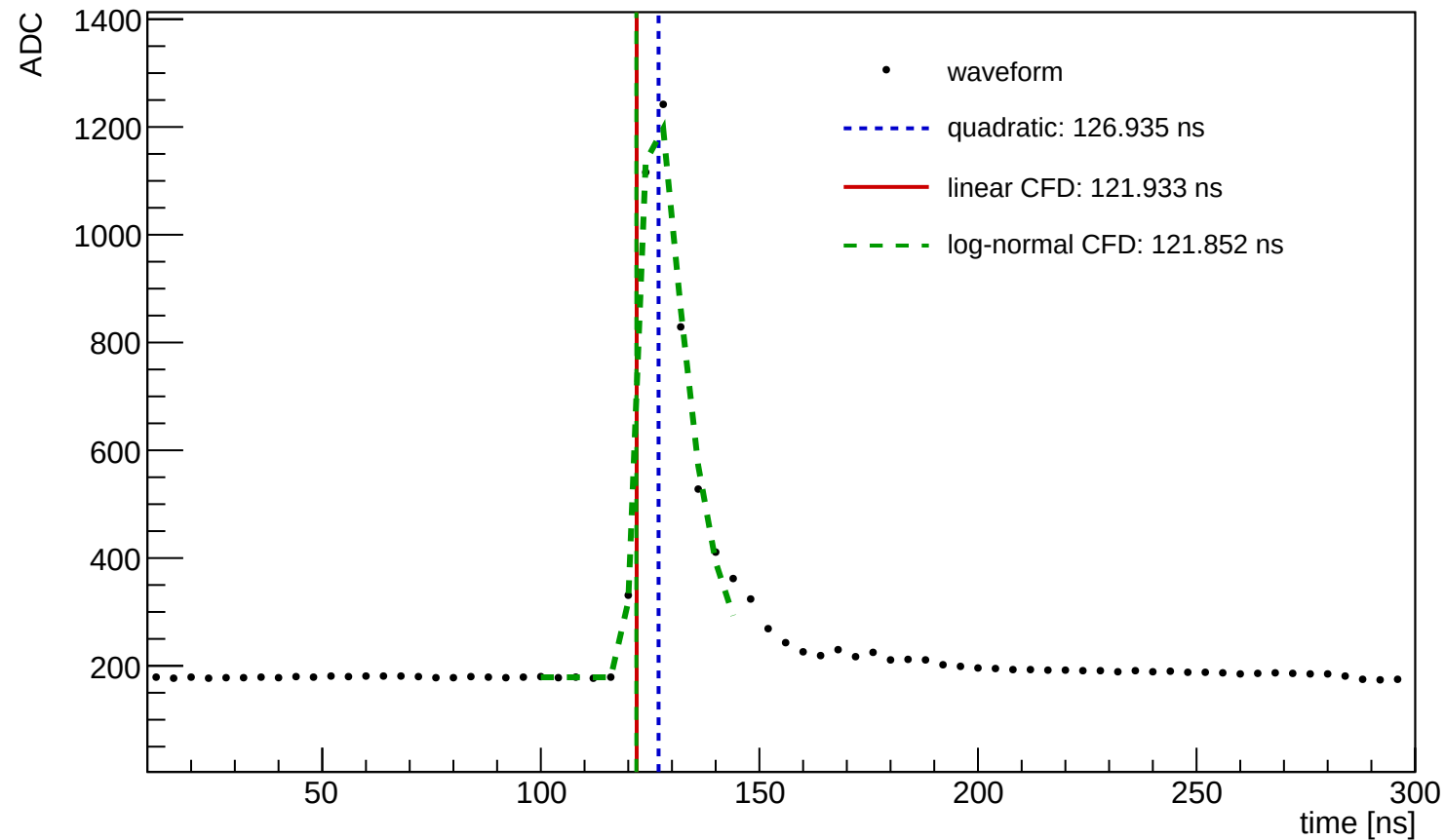
Waveform Time Demo (entry=1308, ch=0, module=3003, trigger=SUM)
