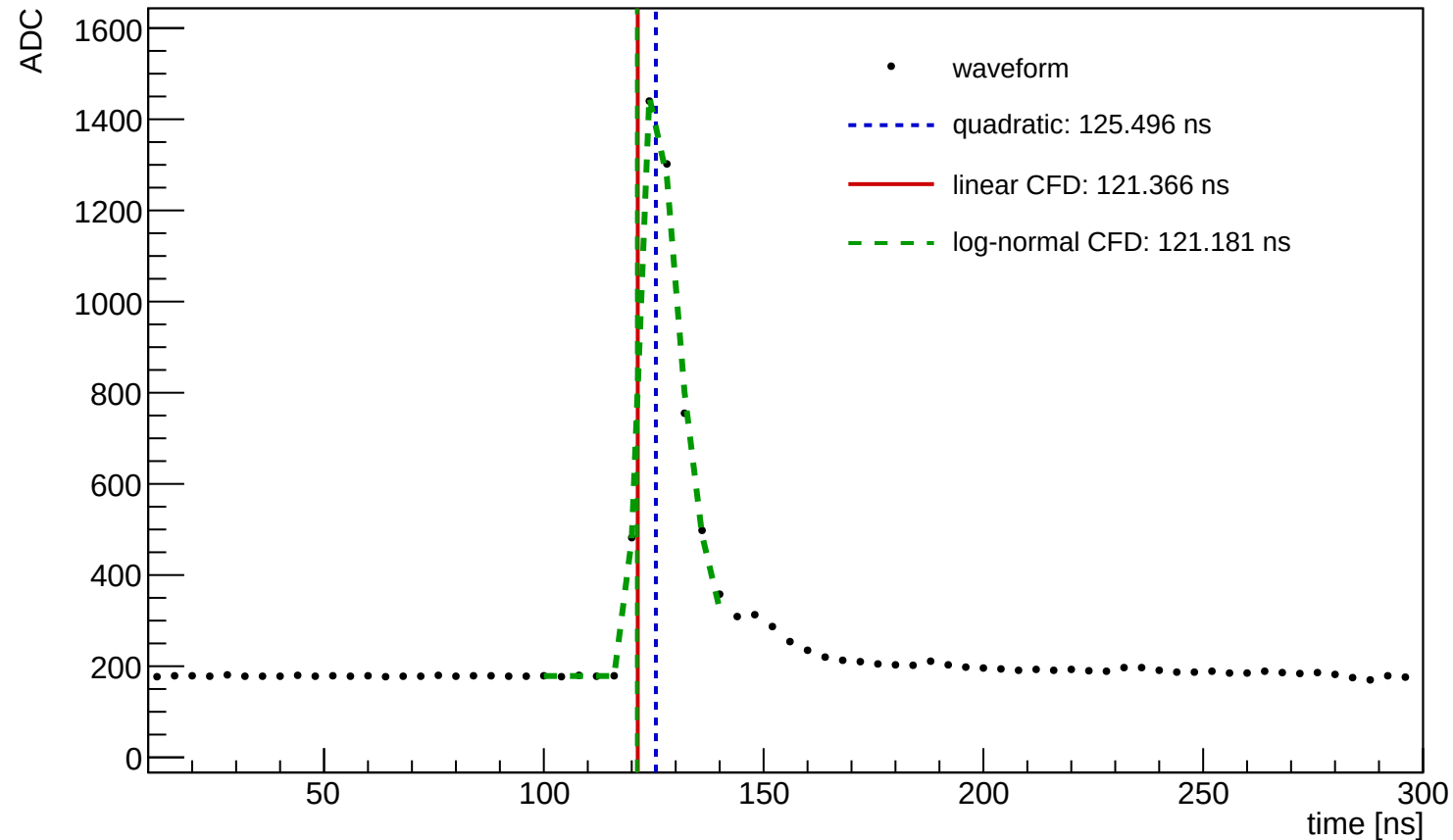
Waveform Time Demo (entry=910, ch=1, module=3003, trigger=SUM)
