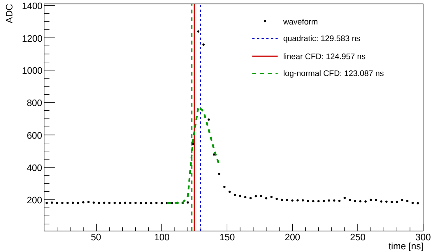
Waveform Time Demo (entry=937, ch=6, module=3003, trigger=SUM)
