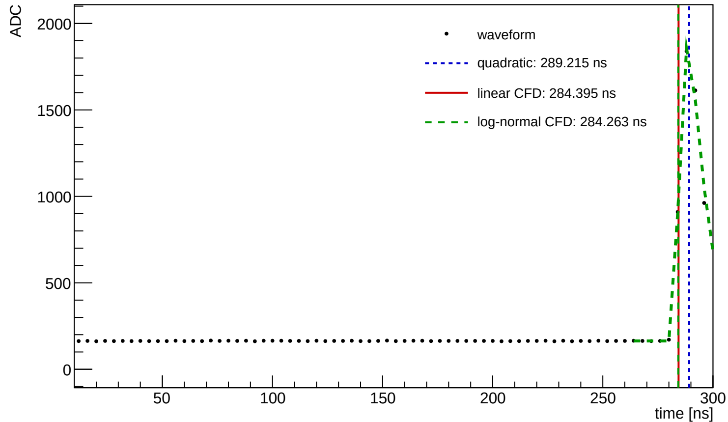
Waveform Time Demo (entry=632, ch=3, module=3002, trigger=SUM)
