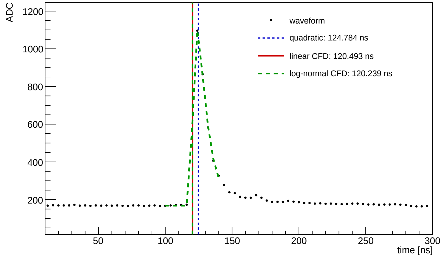
Waveform Time Demo (entry=1331, ch=12, module=3004, trigger=SUM)
