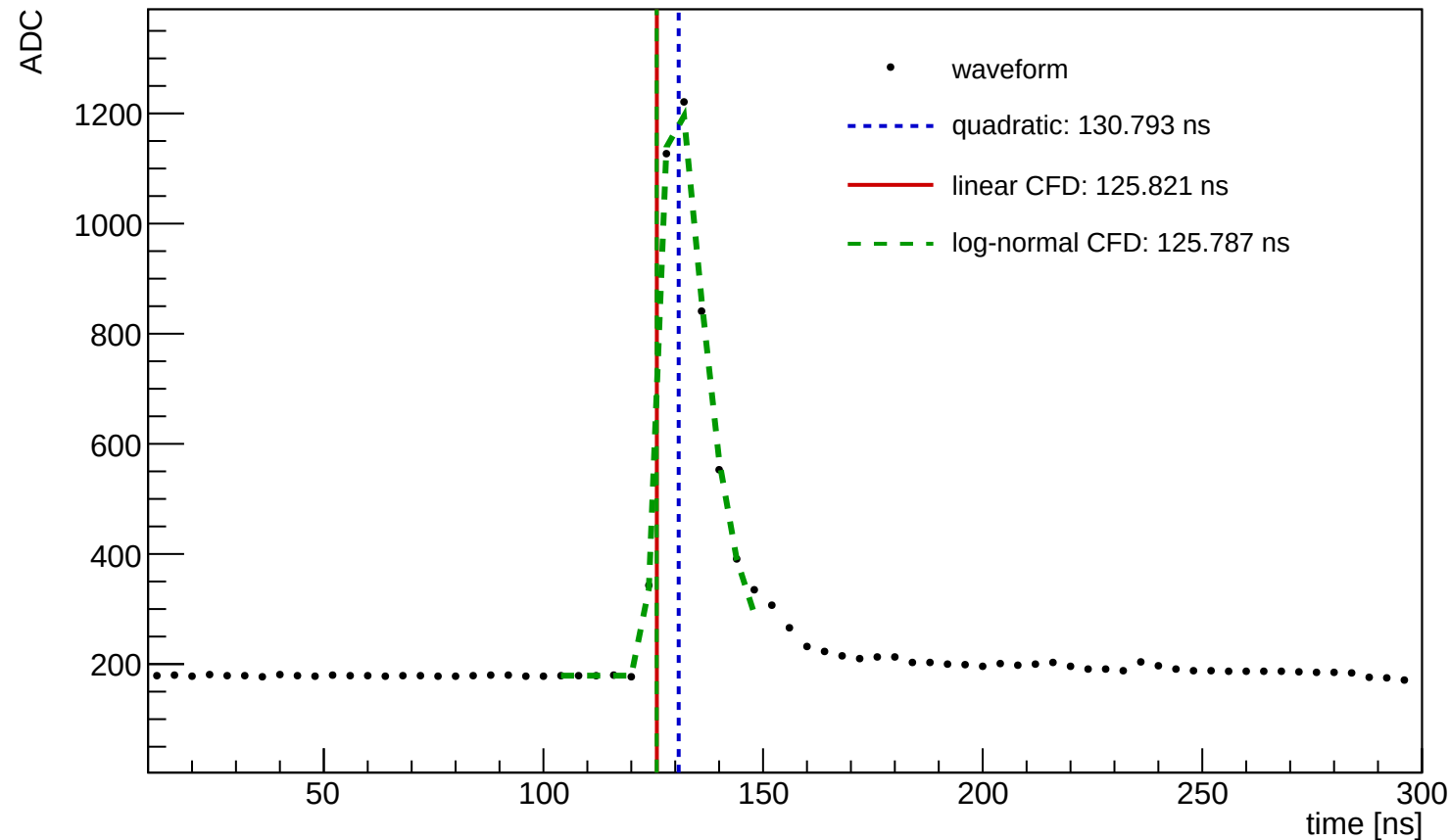
Waveform Time Demo (entry=814, ch=2, module=3003, trigger=SUM)
