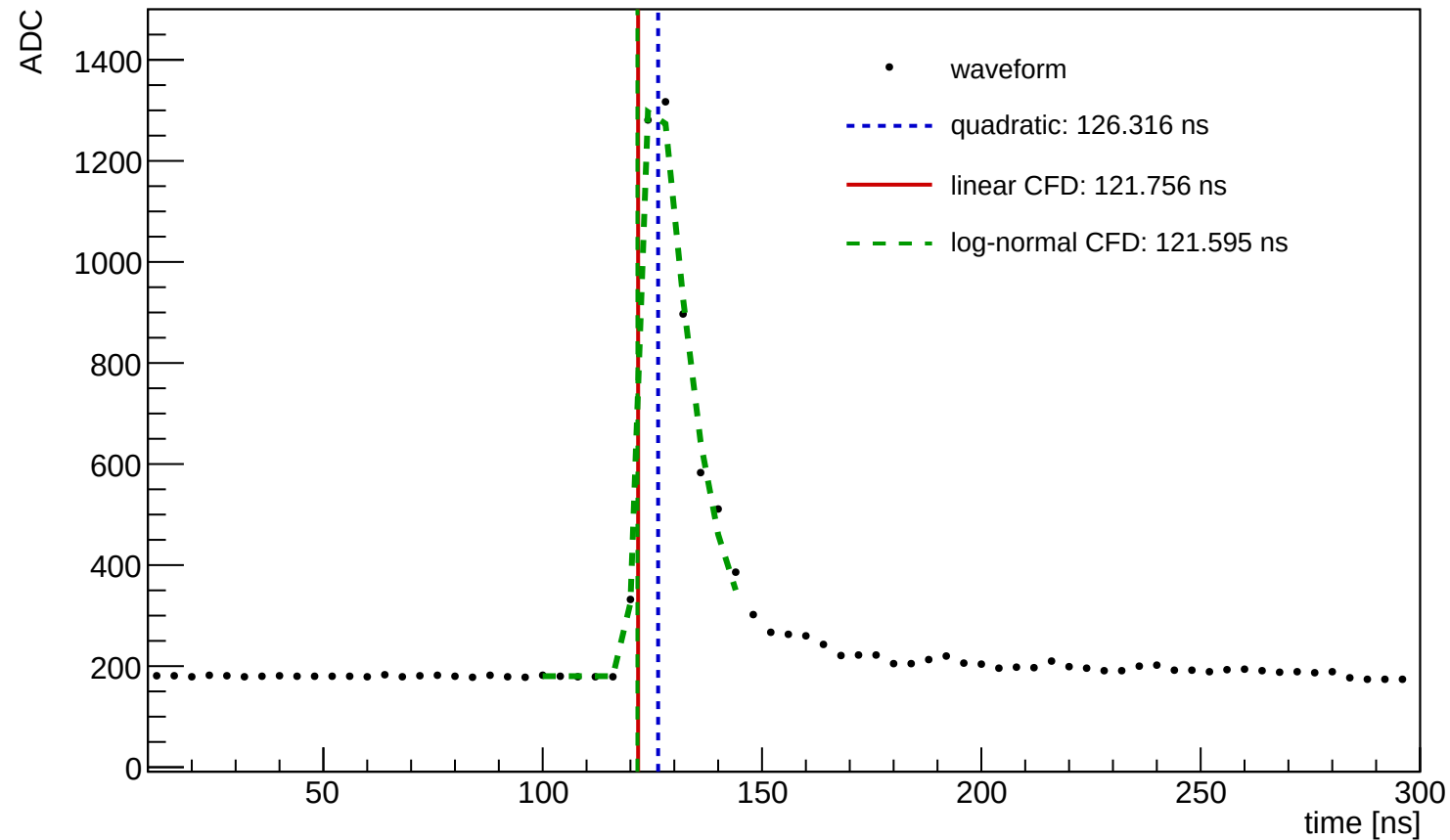
Waveform Time Demo (entry=419, ch=5, module=3003, trigger=SUM)
