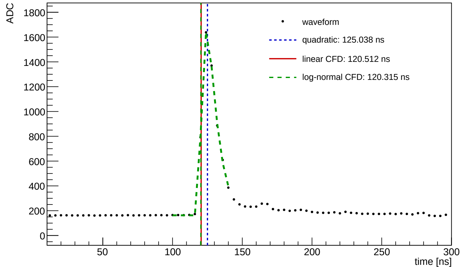
Waveform Time Demo (entry=409, ch=6, module=3002, trigger=SUM)
