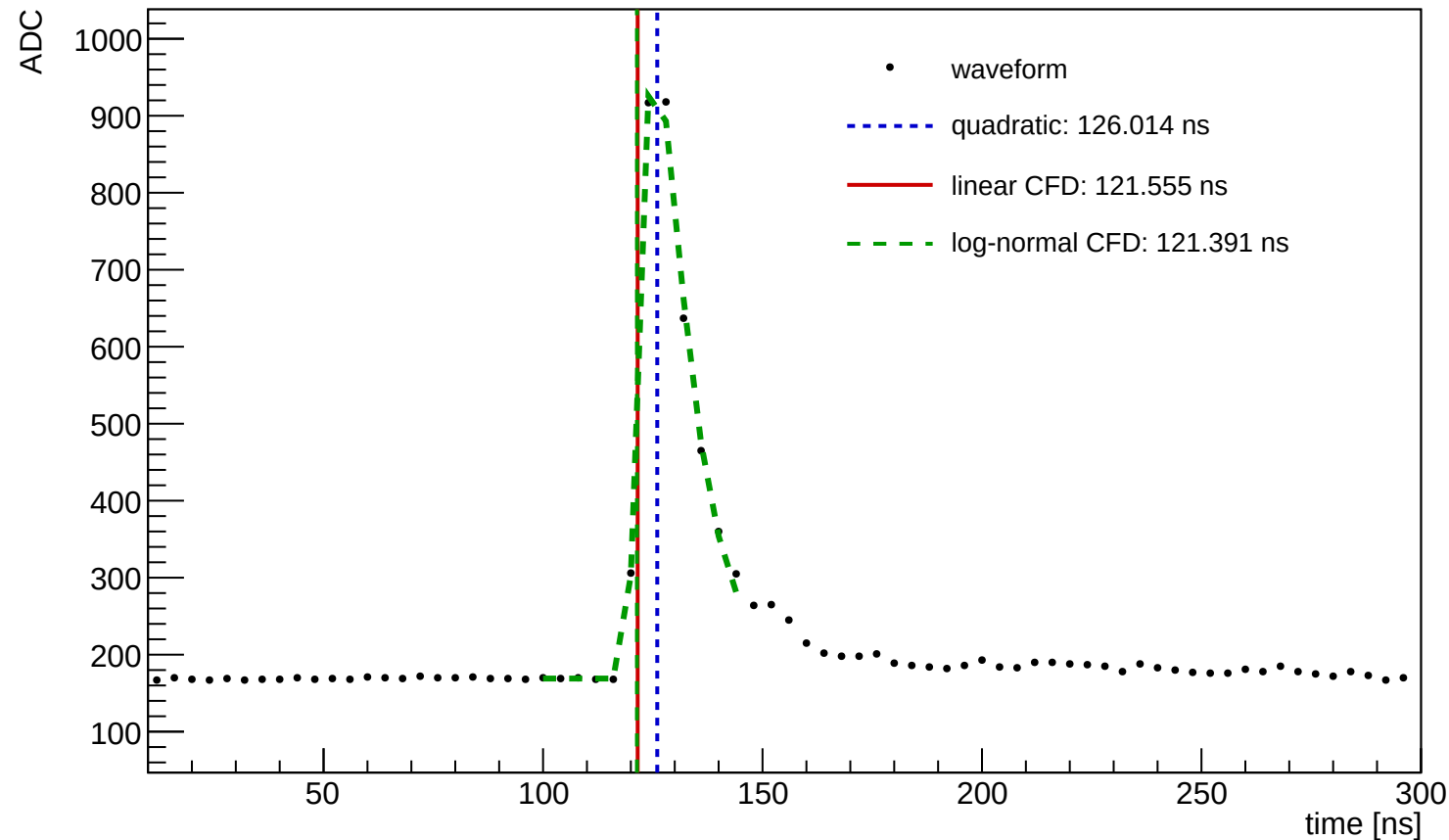
Waveform Time Demo (entry=263, ch=1, module=3004, trigger=SUM)
