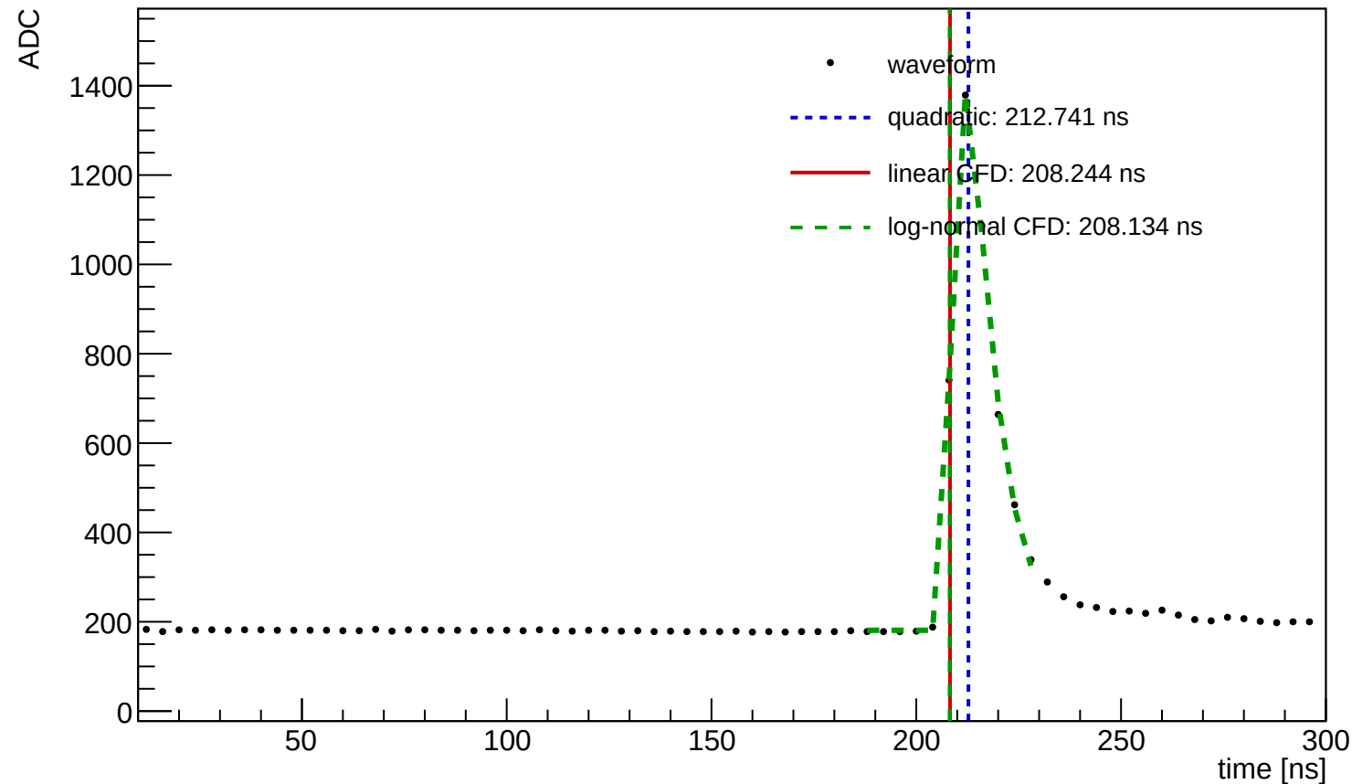
Waveform Time Demo (entry=465, ch=13, module=3003, trigger=SUM)
