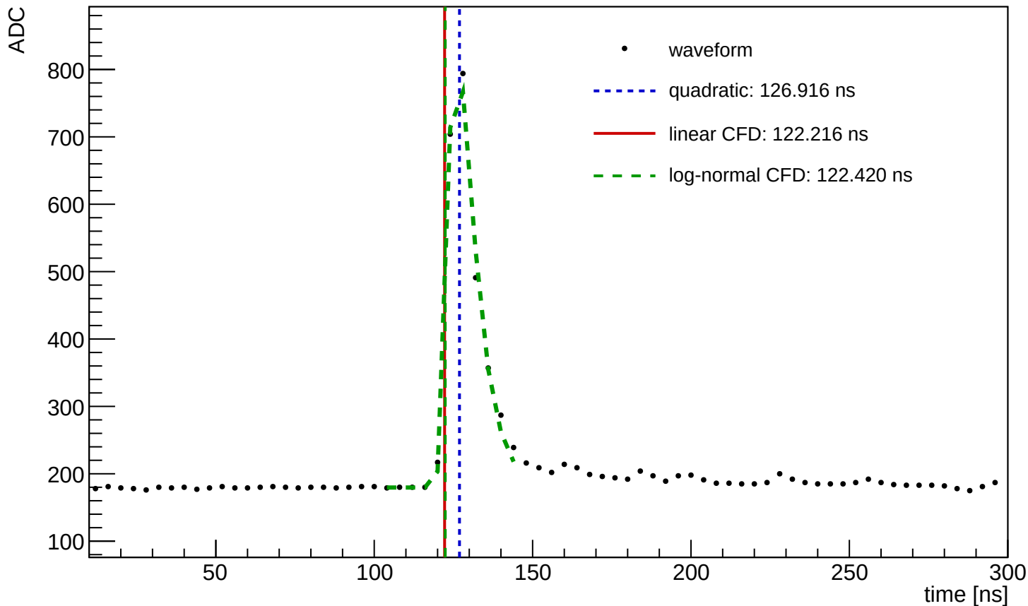
Waveform Time Demo (entry=849, ch=12, module=3003, trigger=SUM)
