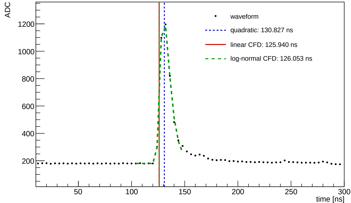
Waveform Time Demo (entry=1484, ch=4, module=3003, trigger=SUM)
