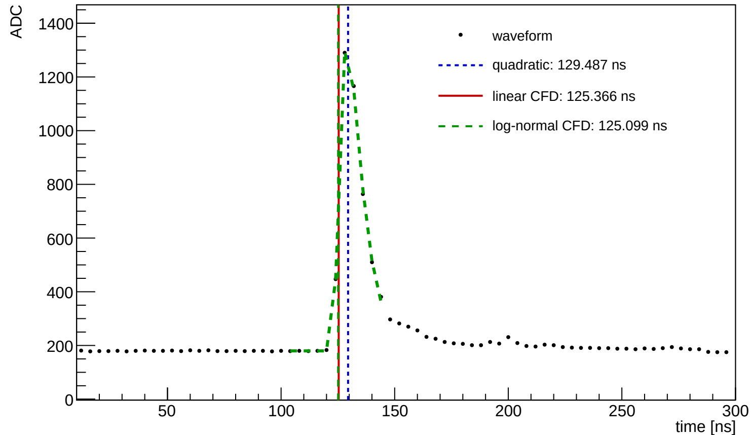
Waveform Time Demo (entry=1466, ch=2, module=3003, trigger=SUM)
