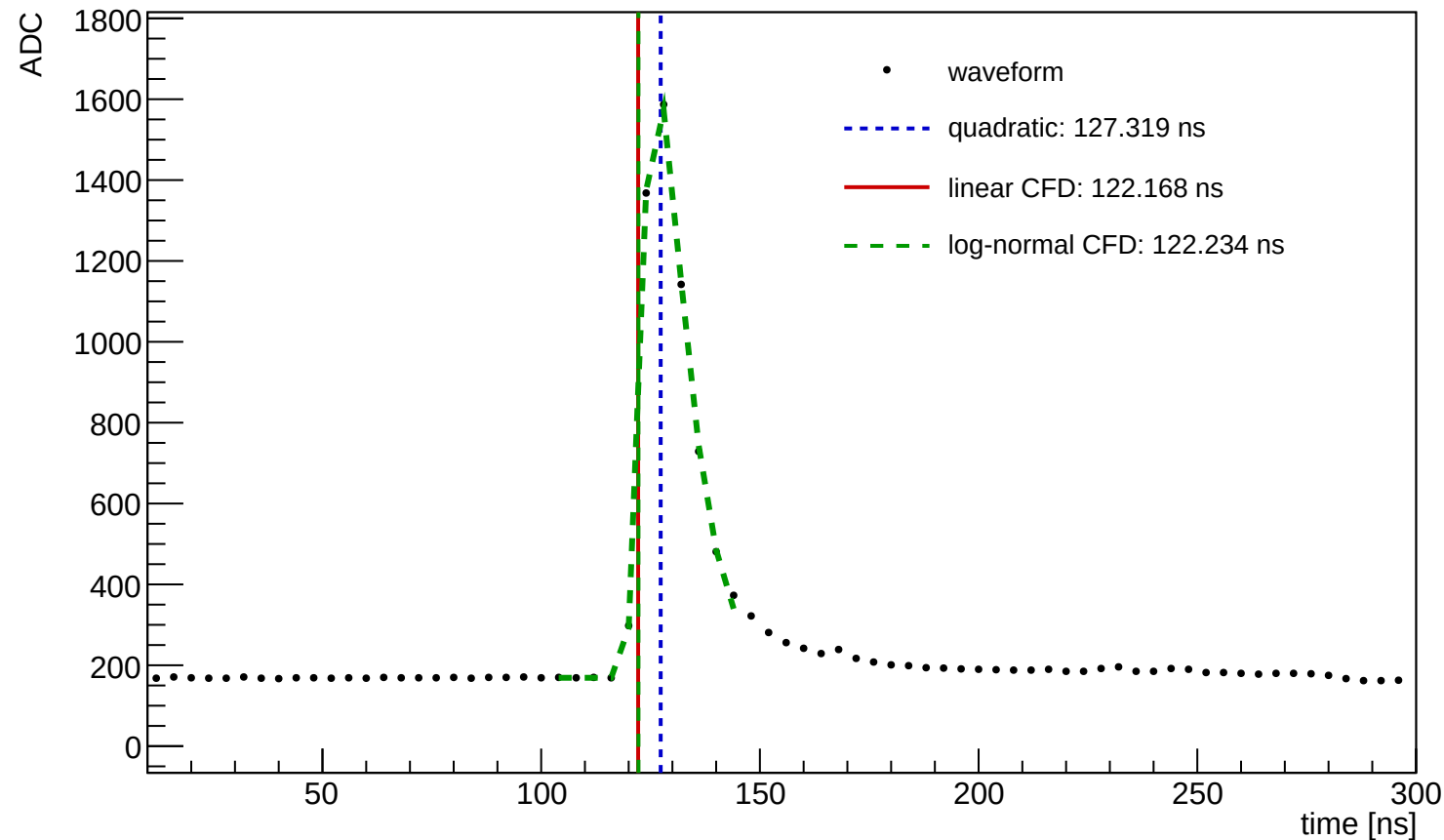
Waveform Time Demo (entry=1469, ch=2, module=3004, trigger=SUM)
