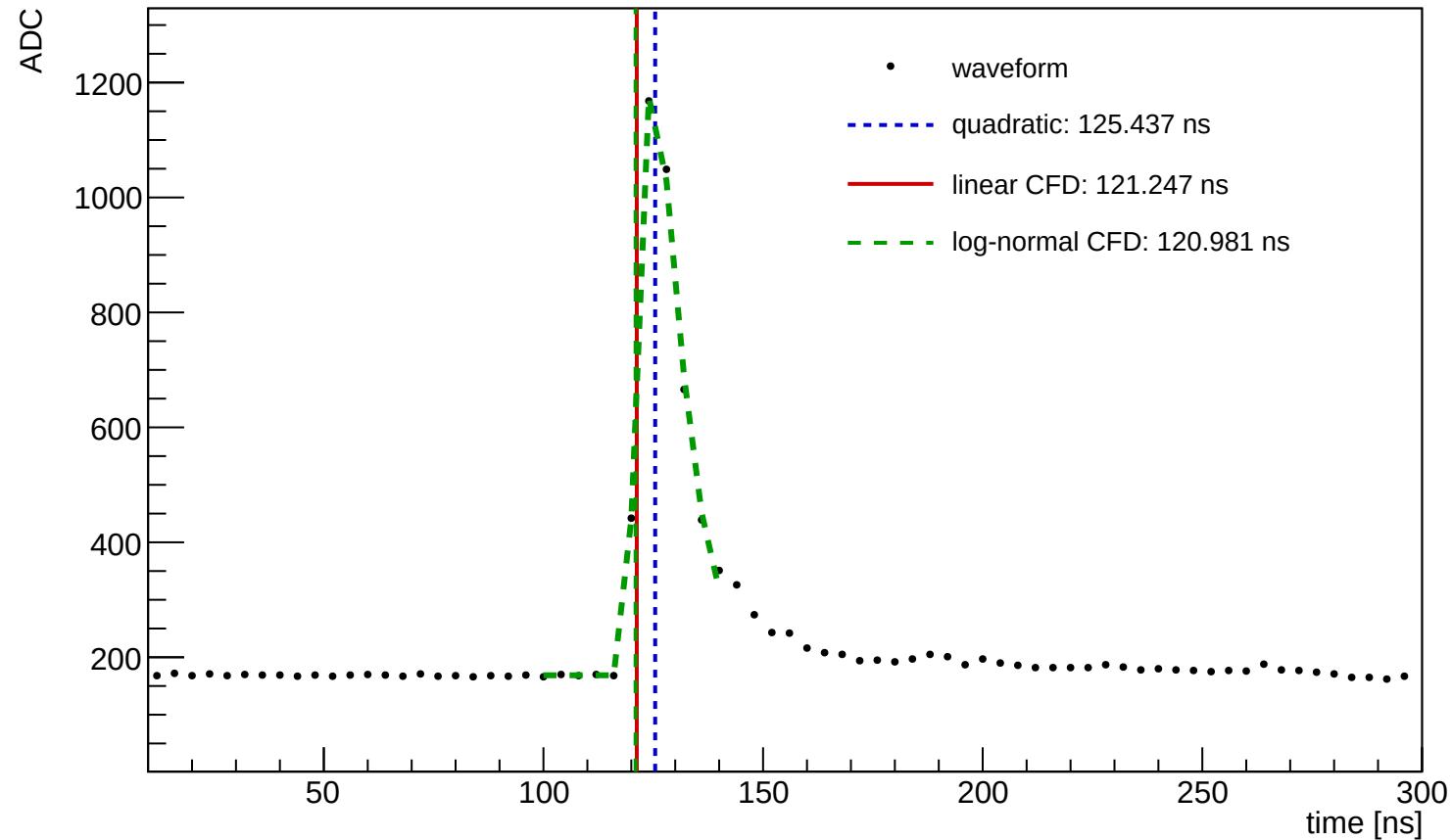
Waveform Time Demo (entry=276, ch=2, module=3004, trigger=SUM)
