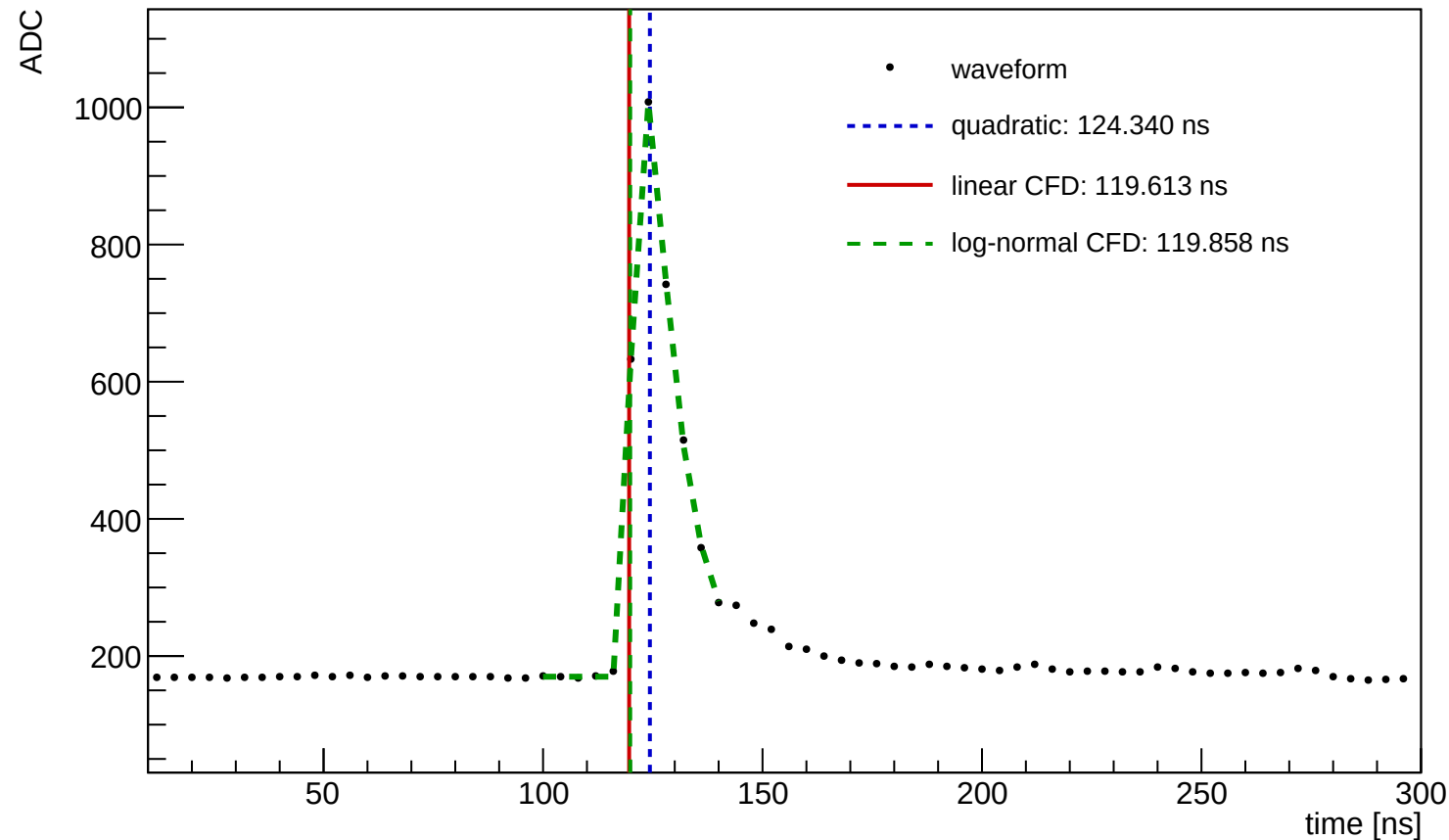
Waveform Time Demo (entry=61, ch=4, module=3004, trigger=SUM)
