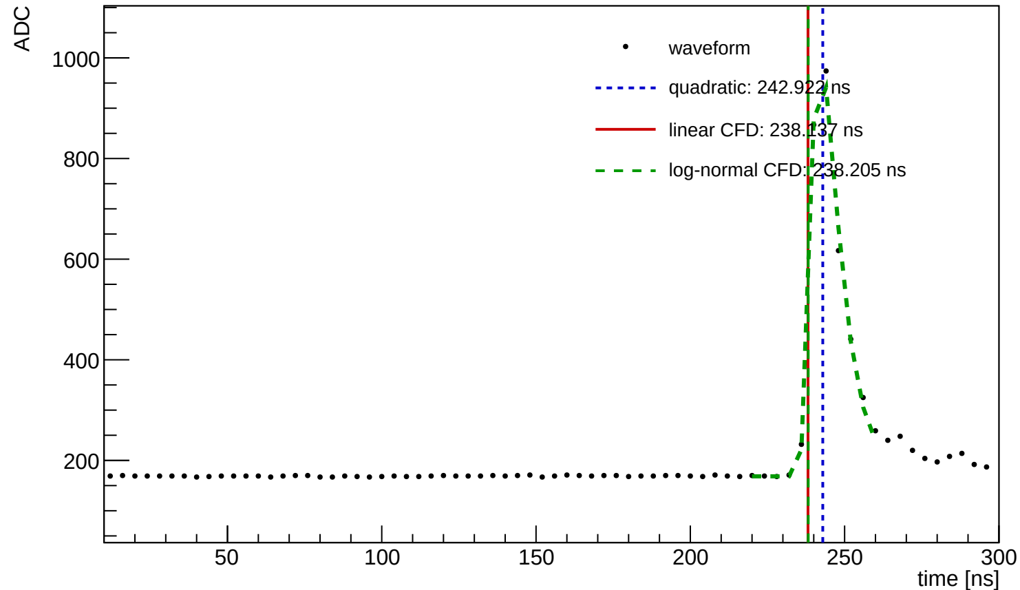
Waveform Time Demo (entry=312, ch=0, module=3004, trigger=SUM)
