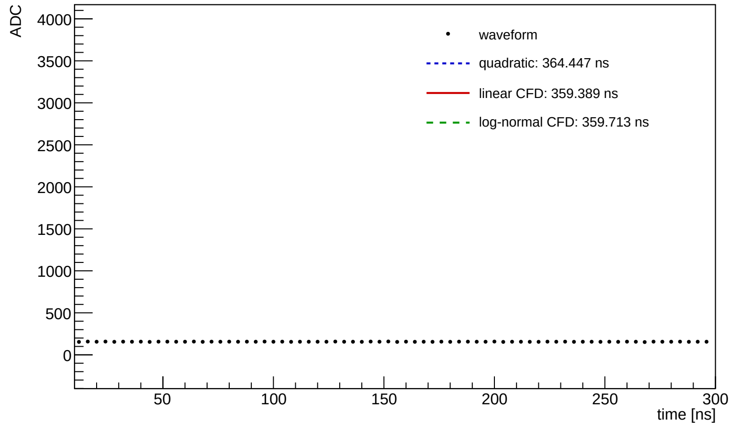
Waveform Time Demo (entry=688, ch=0, module=3001, trigger=SUM)
