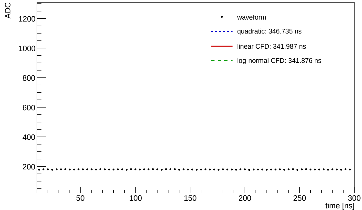
Waveform Time Demo (entry=630, ch=0, module=3003, trigger=SUM)
