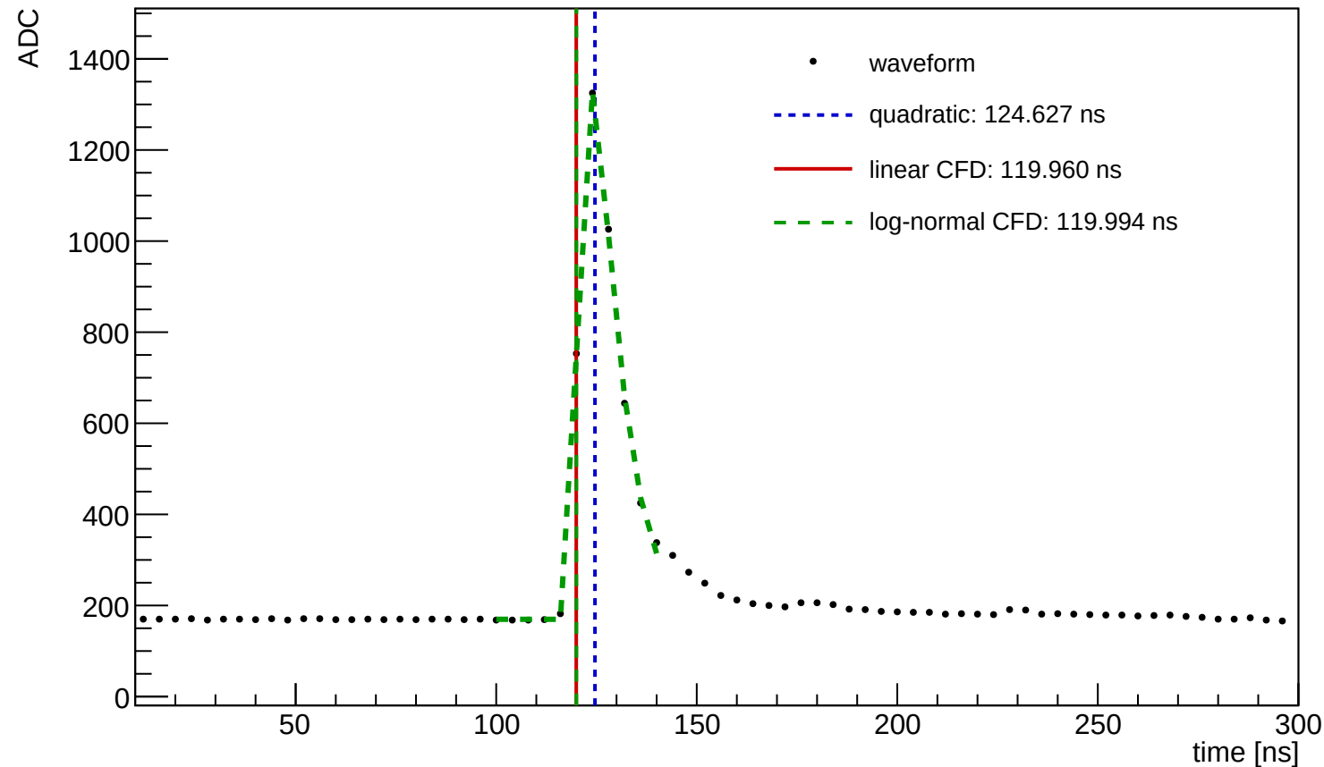
Waveform Time Demo (entry=1318, ch=16, module=3004, trigger=SUM)
