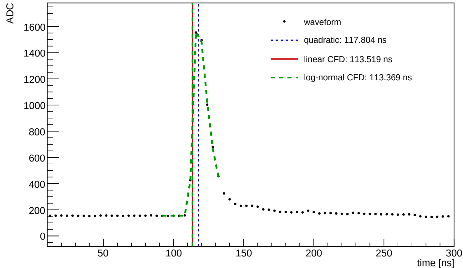
Waveform Time Demo (entry=109, ch=4, module=3001, trigger=SUM)
