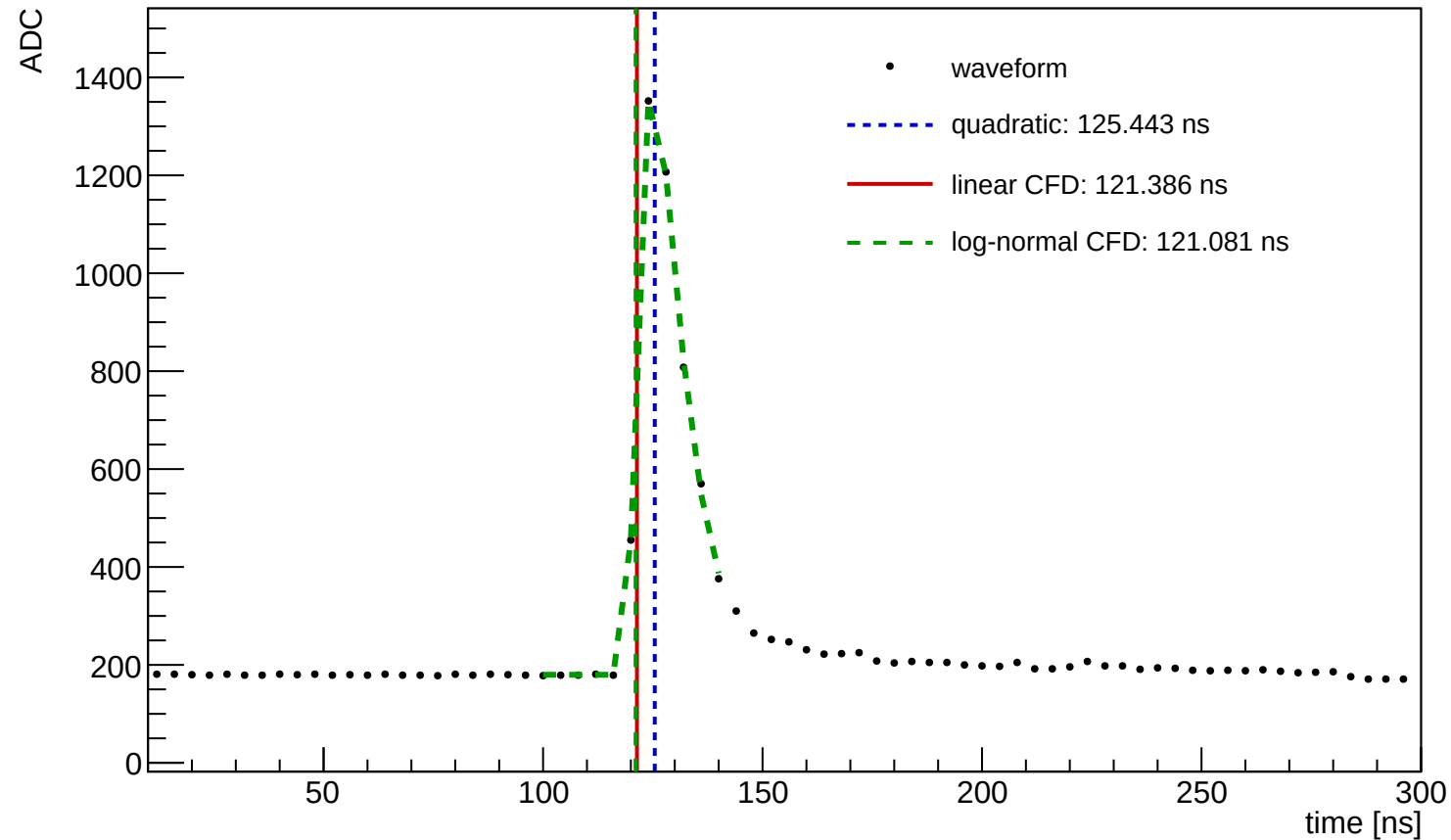
Waveform Time Demo (entry=262, ch=0, module=3003, trigger=SUM)
