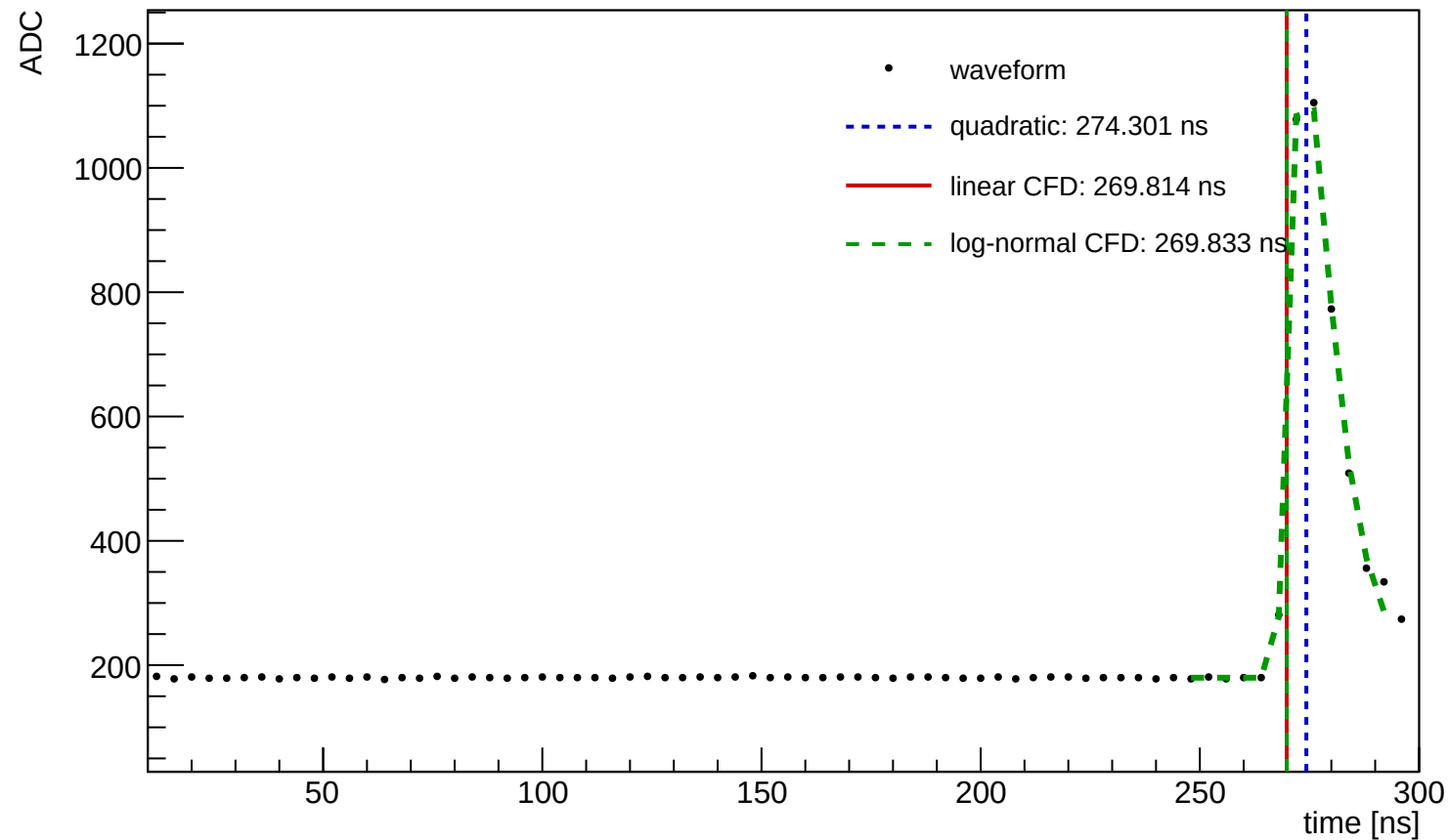
Waveform Time Demo (entry=548, ch=4, module=3003, trigger=SUM)
