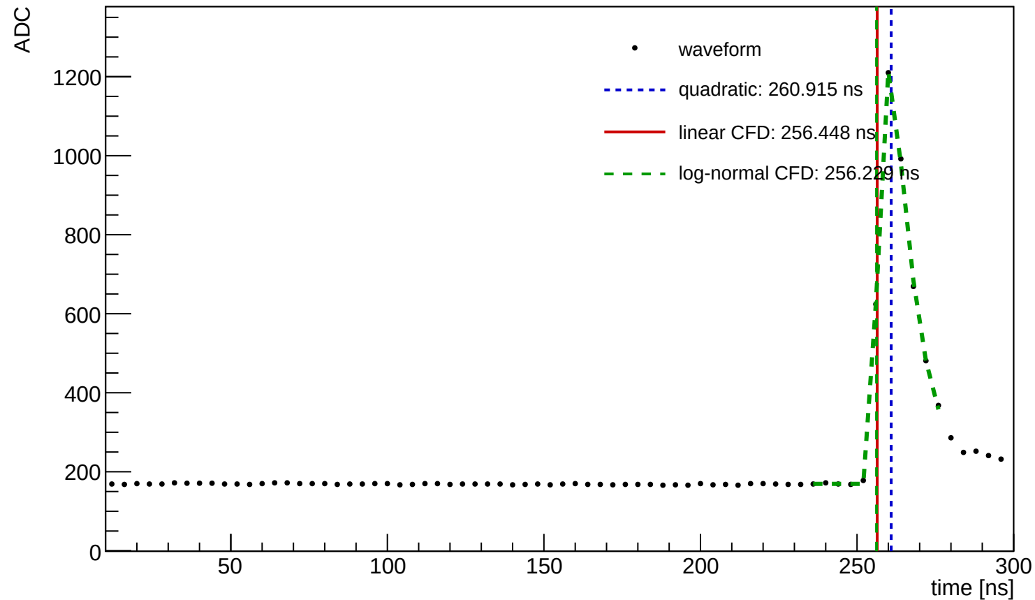
Waveform Time Demo (entry=640, ch=2, module=3004, trigger=SUM)
