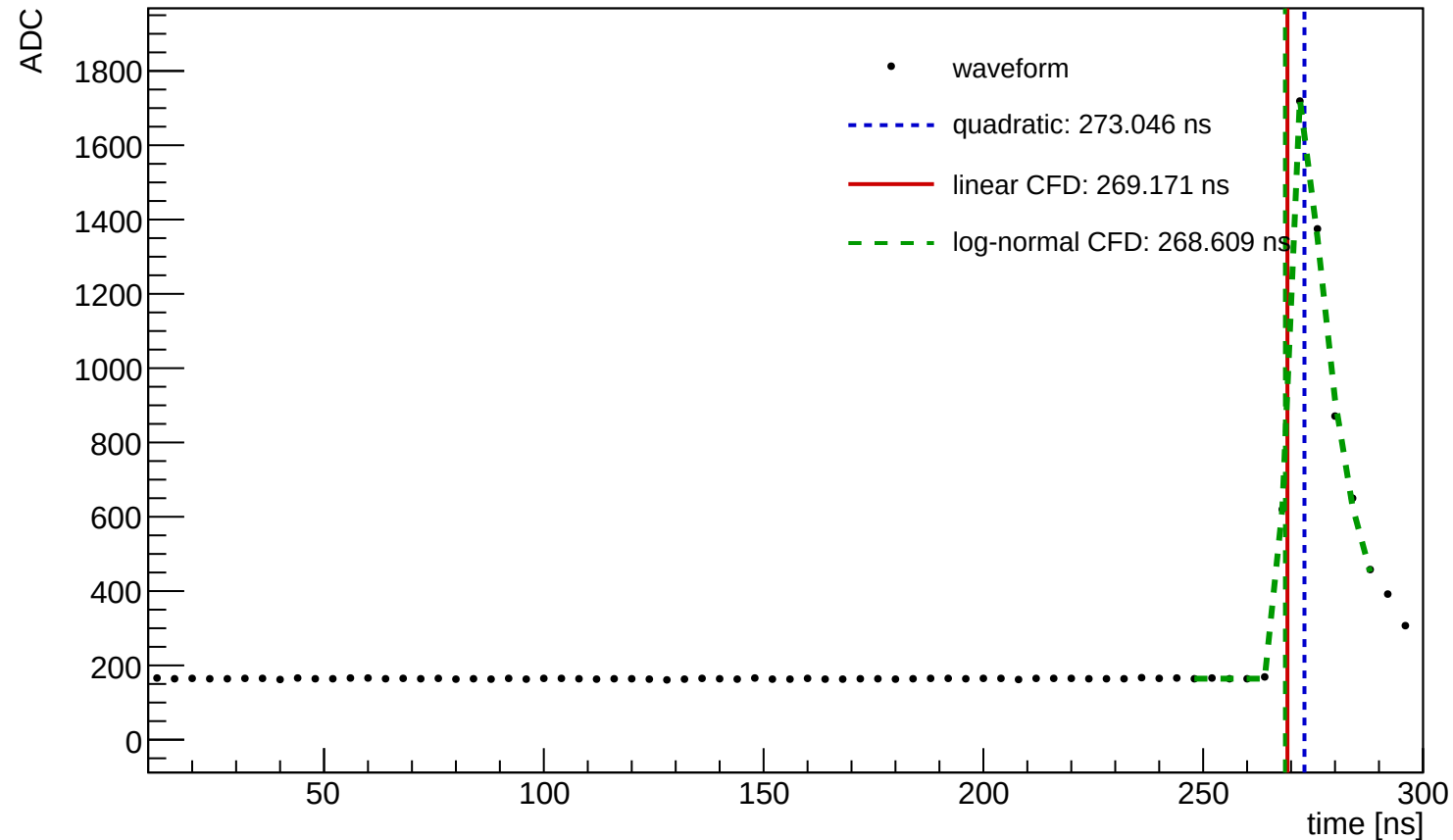
Waveform Time Demo (entry=548, ch=3, module=3002, trigger=SUM)
