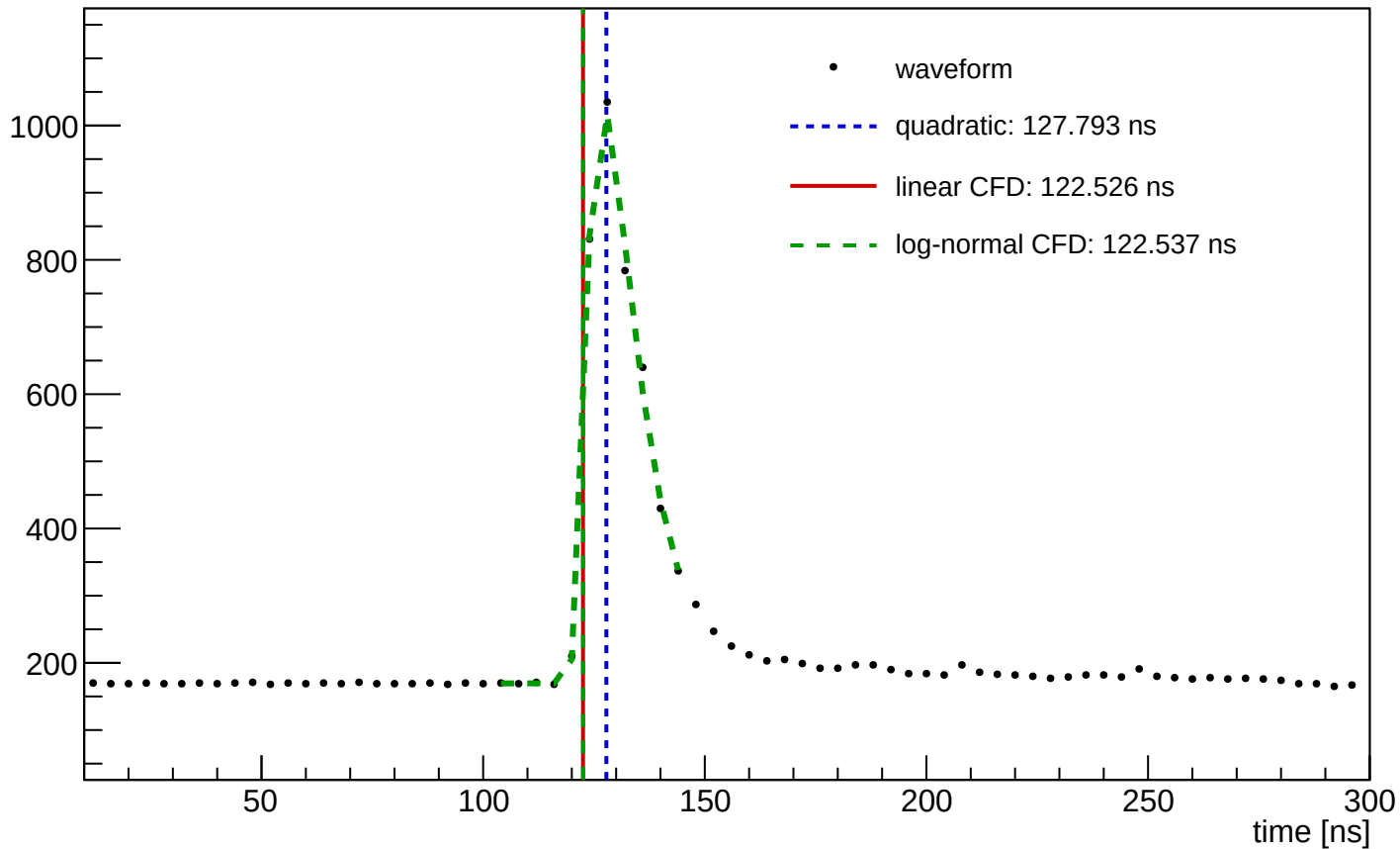
Waveform Time Demo (entry=1649, ch=2, module=3004, trigger=SUM)
