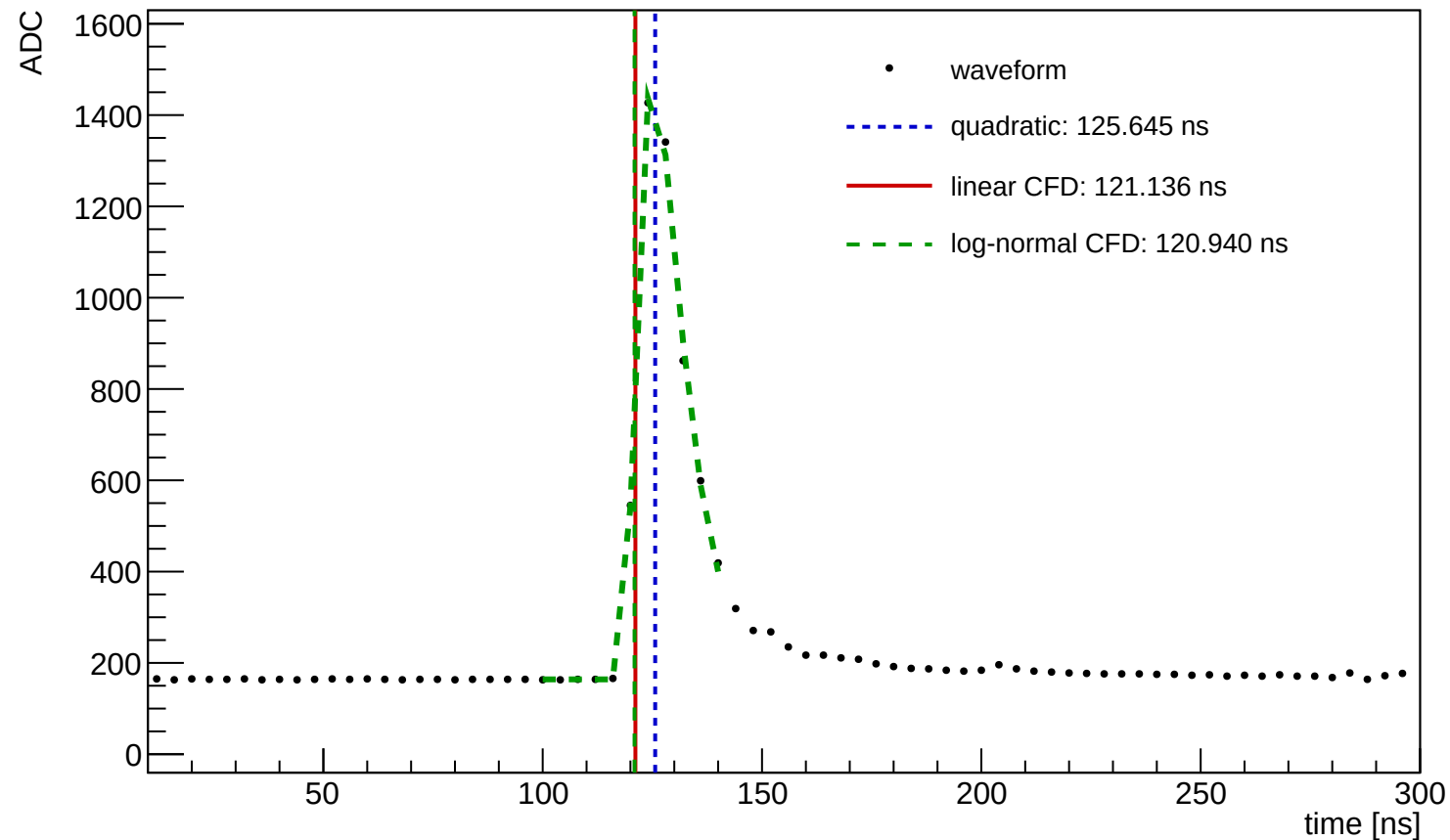
Waveform Time Demo (entry=627, ch=0, module=3002, trigger=SUM)
