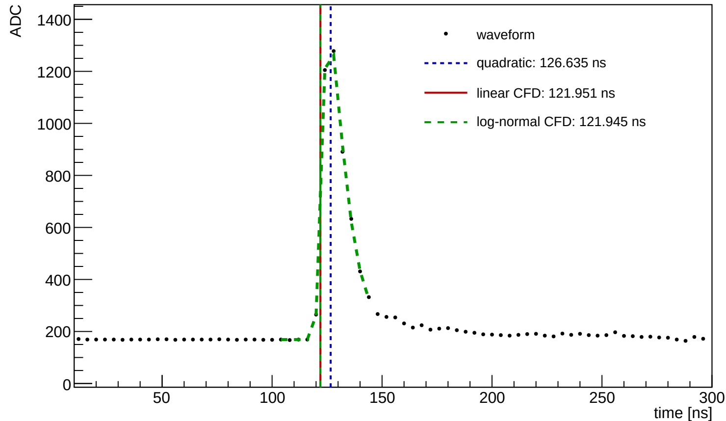
Waveform Time Demo (entry=1078, ch=1, module=3004, trigger=SUM)
