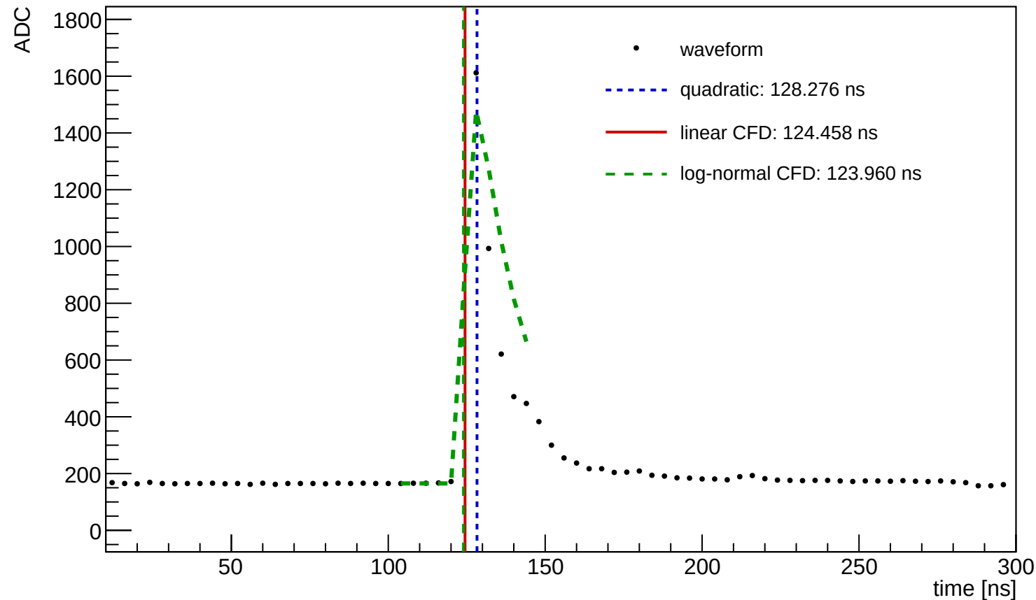
Waveform Time Demo (entry=1642, ch=4, module=3002, trigger=SUM)
