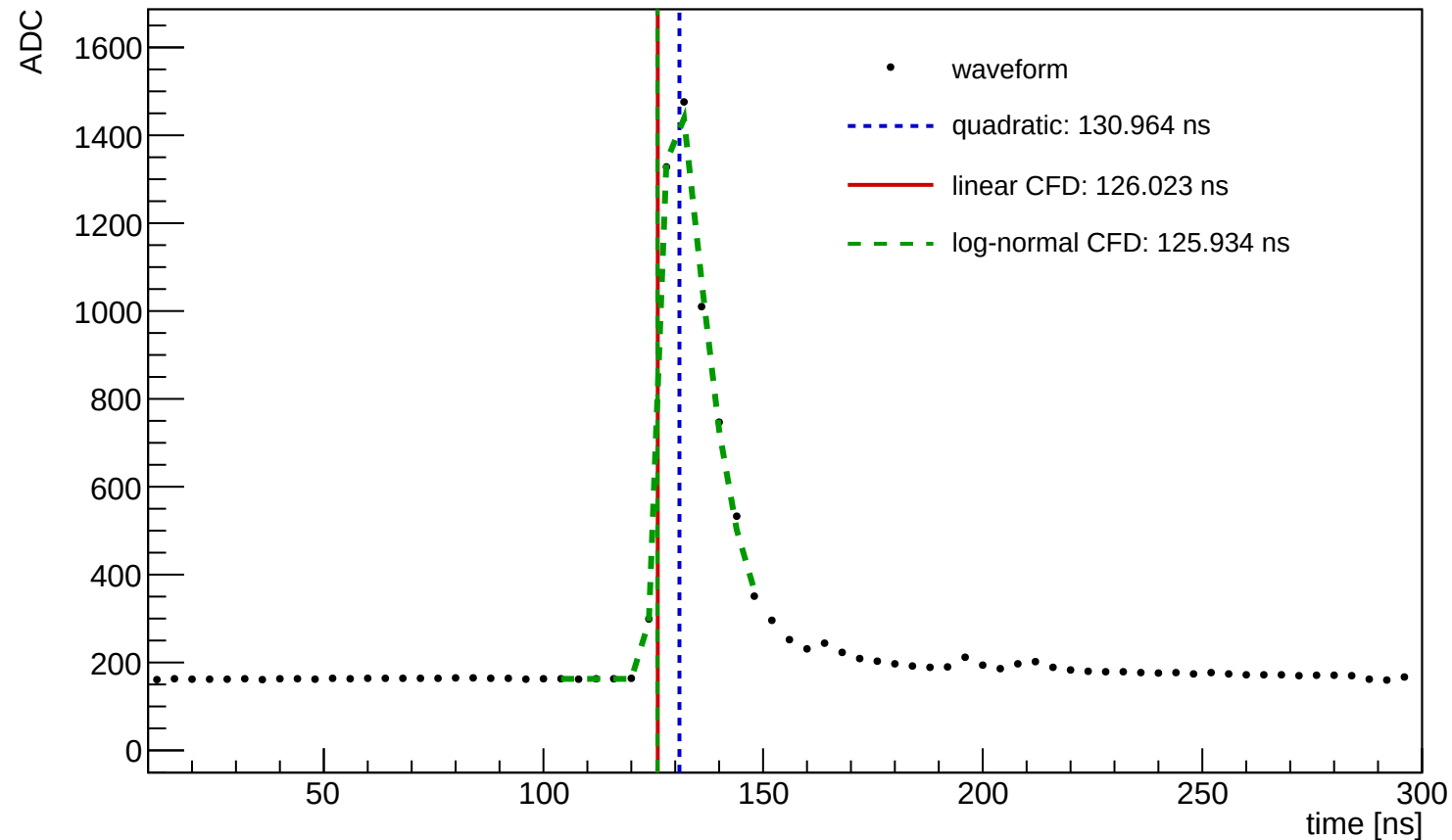
Waveform Time Demo (entry=691, ch=4, module=3002, trigger=SUM)
