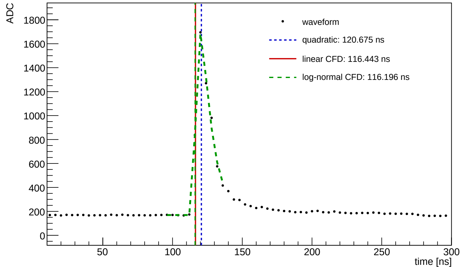
Waveform Time Demo (entry=792, ch=0, module=3004, trigger=SUM)
