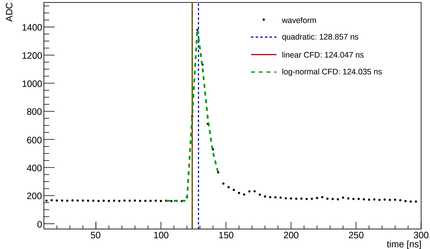
Waveform Time Demo (entry=789, ch=1, module=3002, trigger=SUM)
