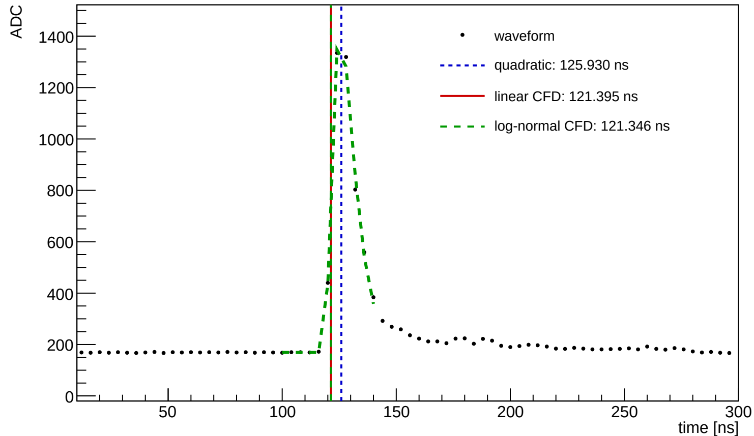
Waveform Time Demo (entry=292, ch=1, module=3004, trigger=SUM)
