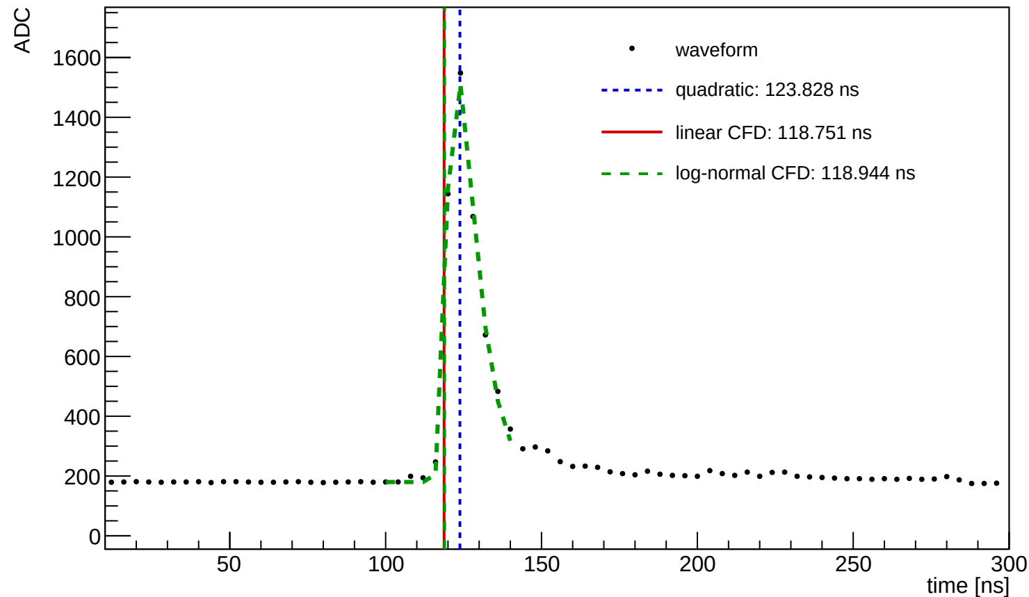
Waveform Time Demo (entry=61, ch=3, module=3003, trigger=SUM)
