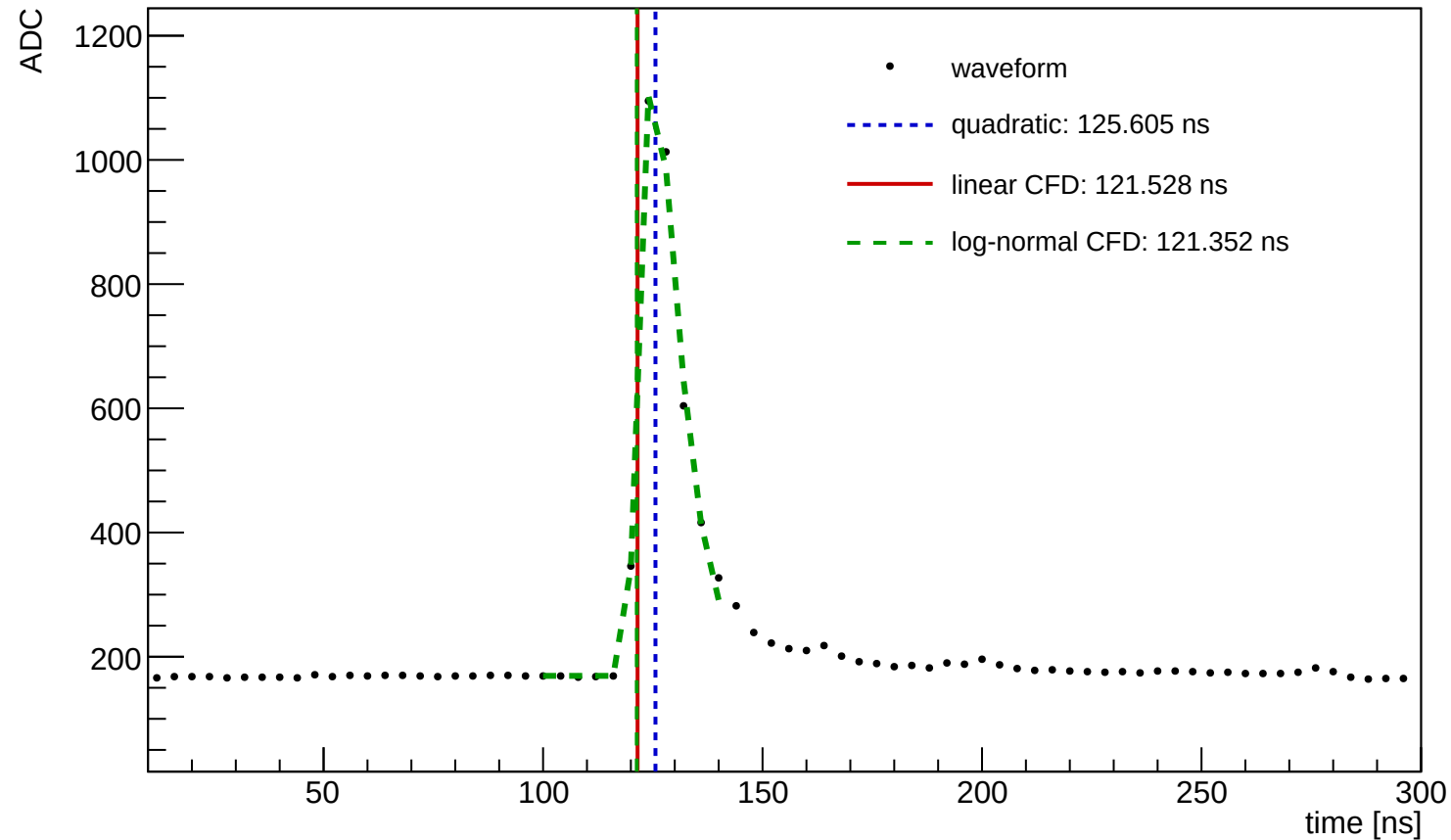
Waveform Time Demo (entry=1560, ch=6, module=3004, trigger=SUM)
