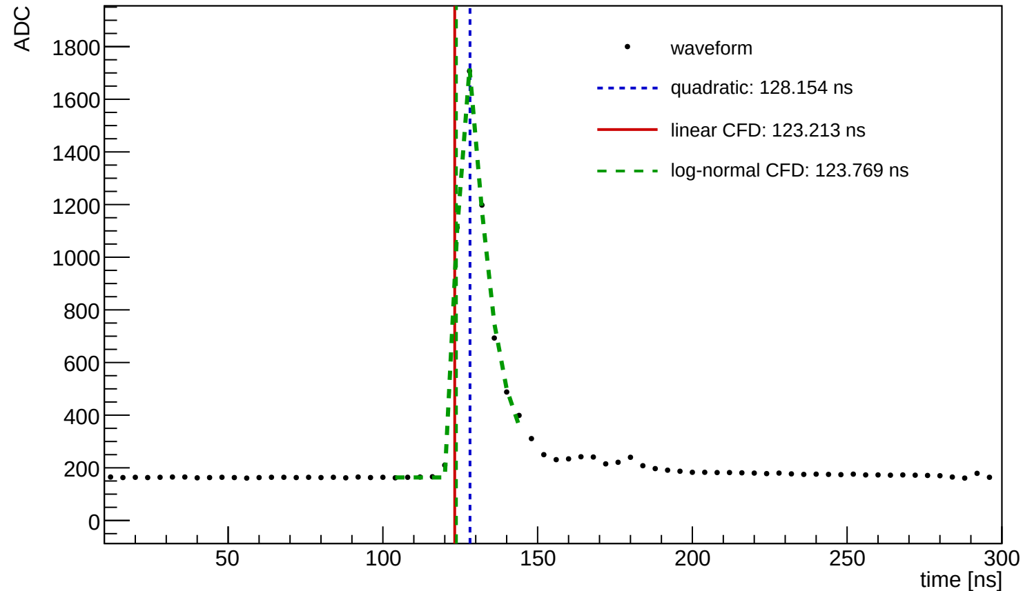
Waveform Time Demo (entry=317, ch=0, module=3002, trigger=SUM)
