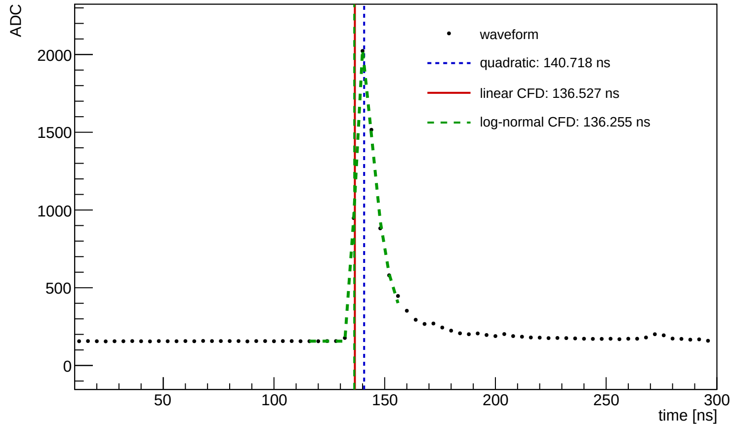
Waveform Time Demo (entry=973, ch=0, module=3001, trigger=SUM)
