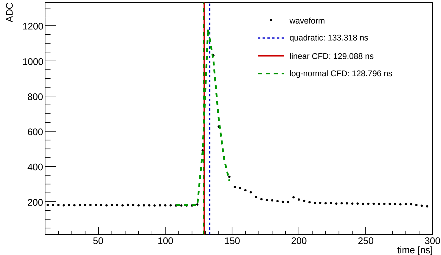
Waveform Time Demo (entry=452, ch=1, module=3003, trigger=SUM)
