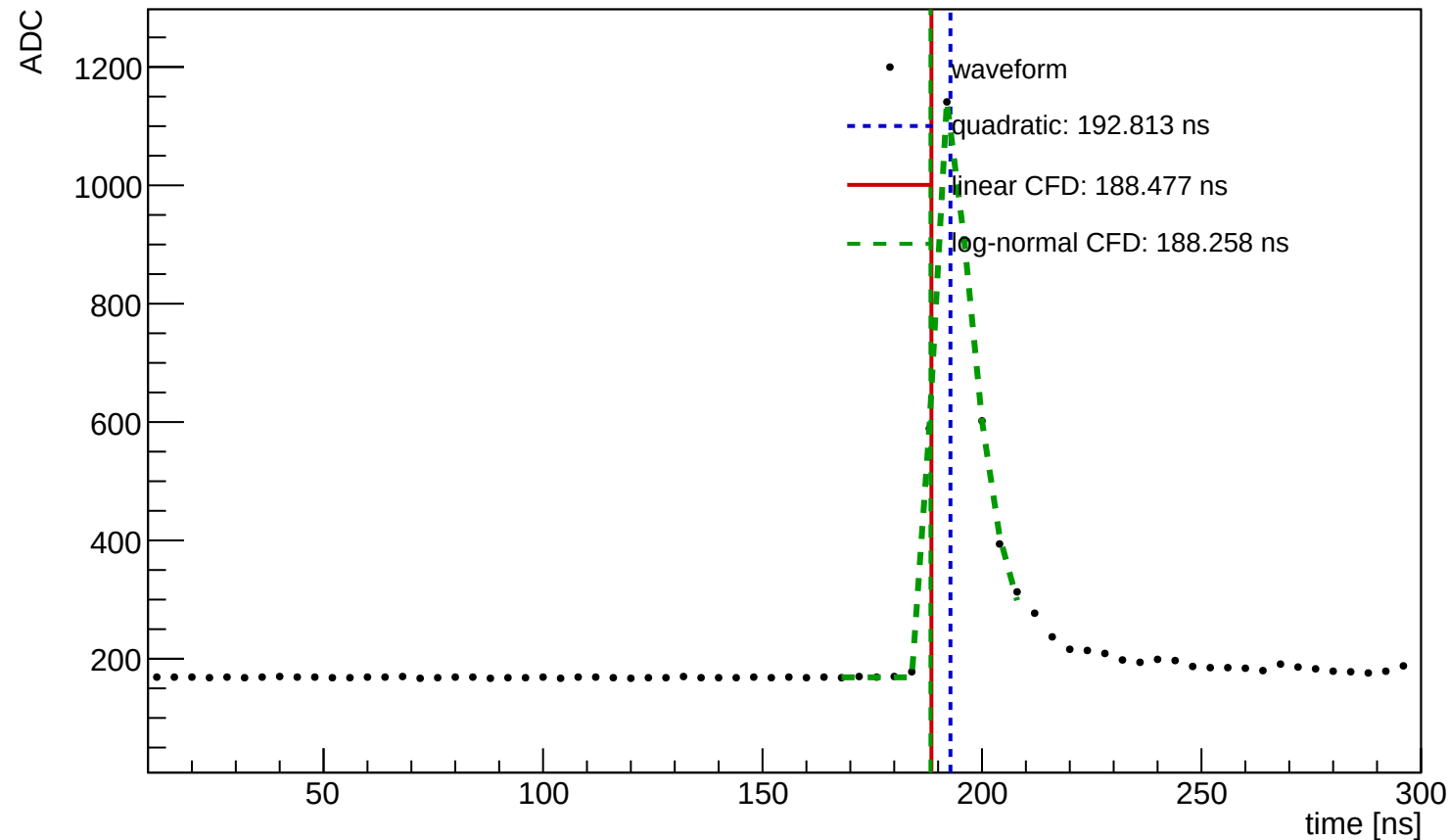
Waveform Time Demo (entry=732, ch=5, module=3004, trigger=SUM)
