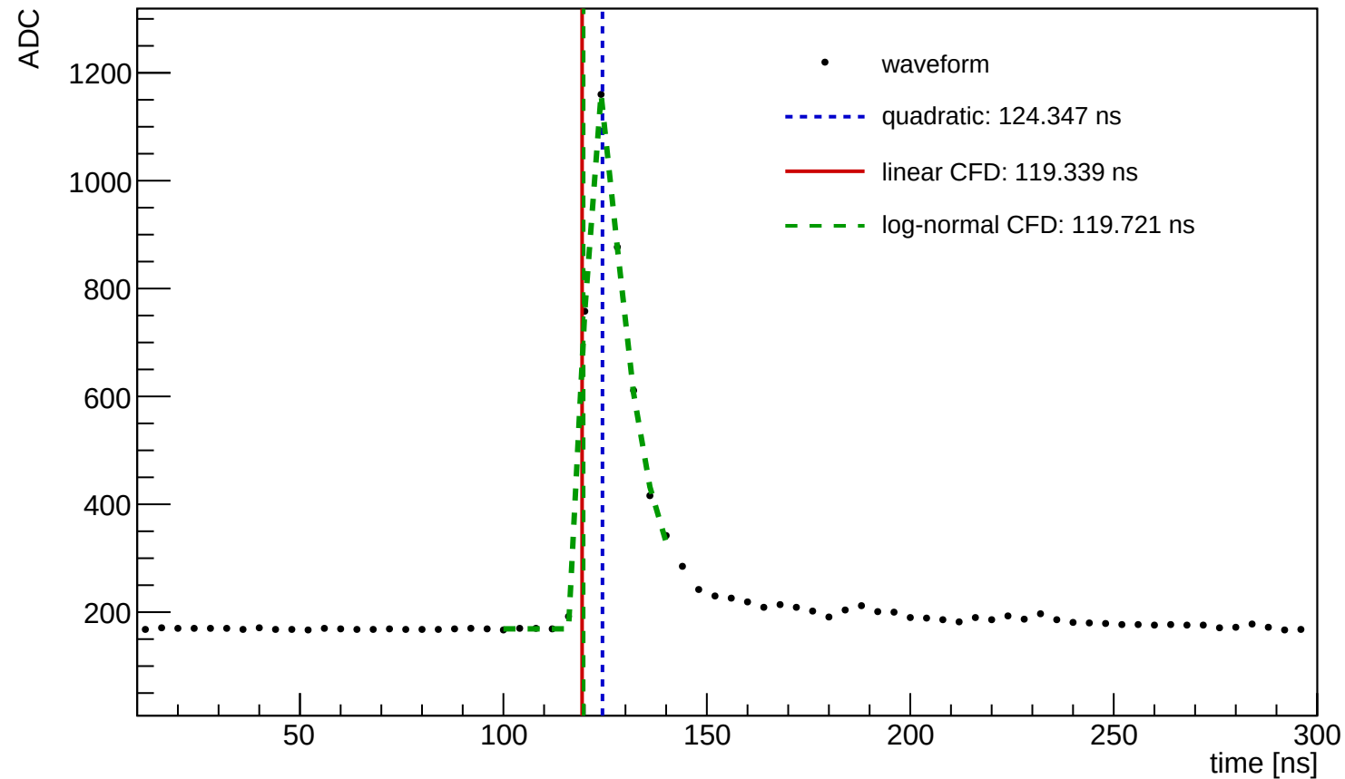
Waveform Time Demo (entry=920, ch=1, module=3004, trigger=SUM)
