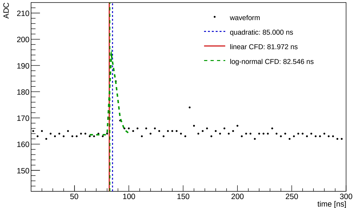
Waveform Time Demo (entry=2236, ch=6, module=3002, trigger=SUM)
