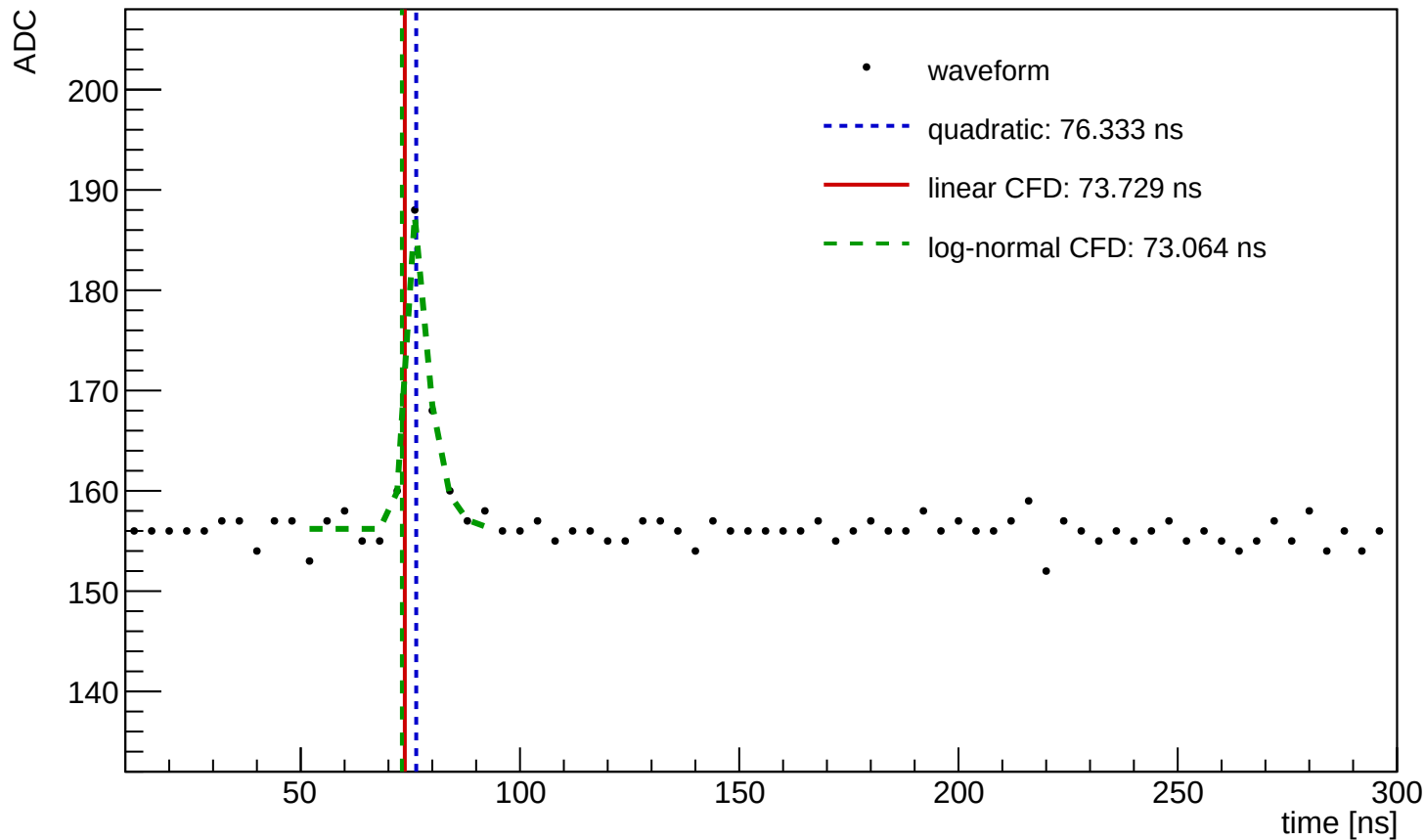
Waveform Time Demo (entry=1797, ch=0, module=3001, trigger=SUM)
