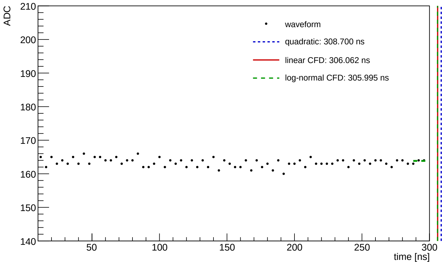
Waveform Time Demo (entry=3025, ch=0, module=3002, trigger=SUM)
