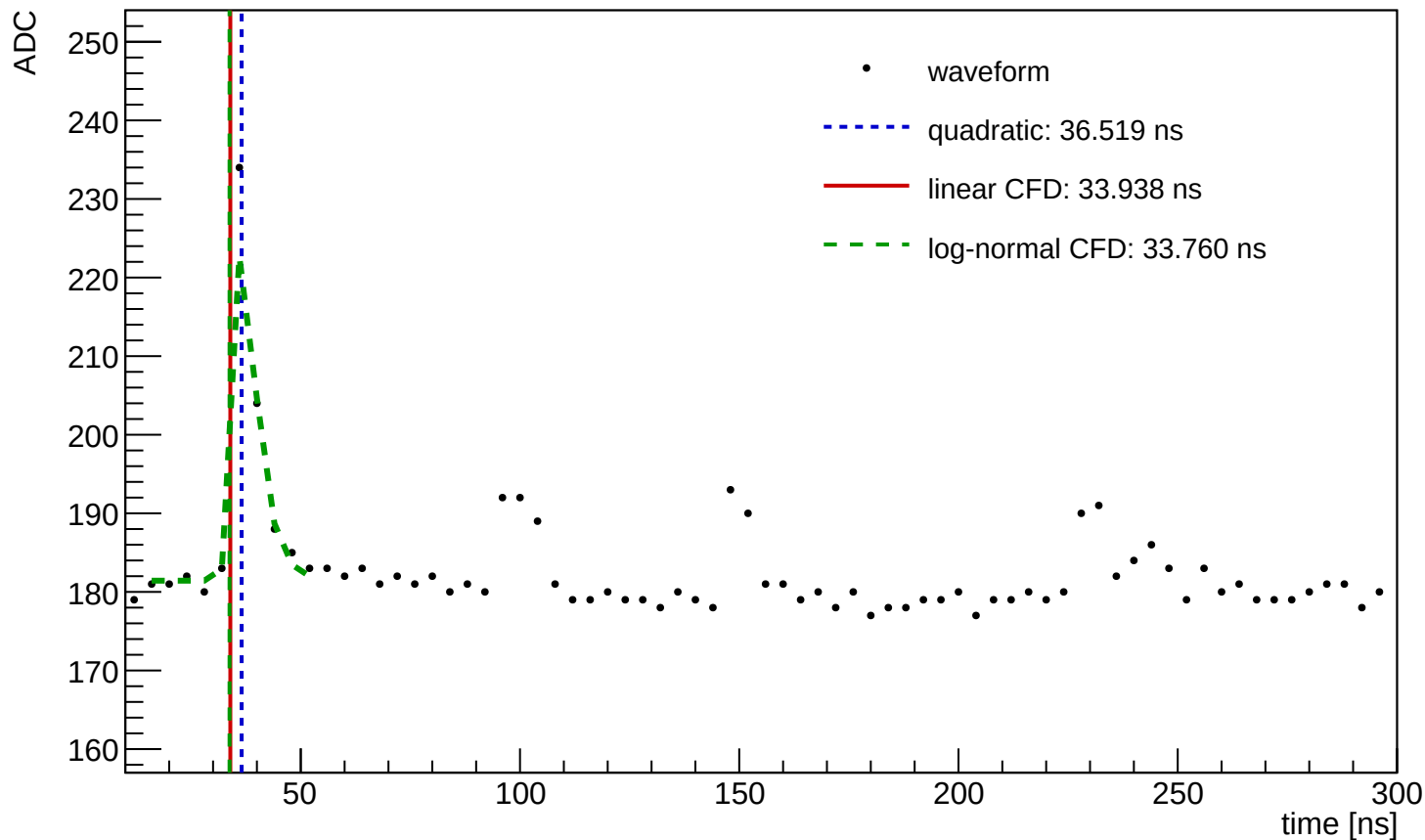
Waveform Time Demo (entry=2504, ch=11, module=3003, trigger=SUM)
