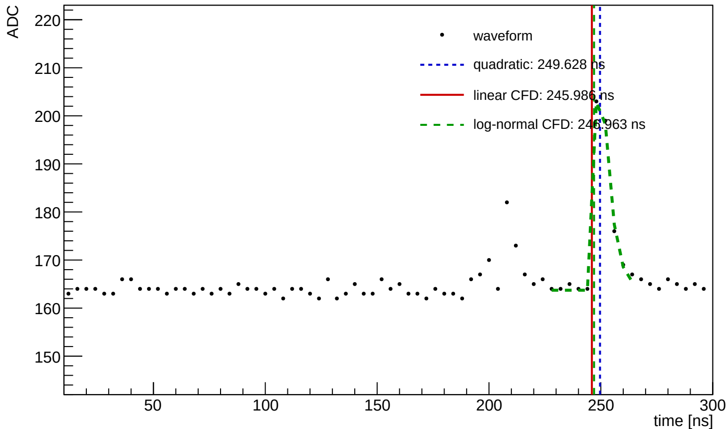
Waveform Time Demo (entry=2949, ch=13, module=3002, trigger=SUM)
