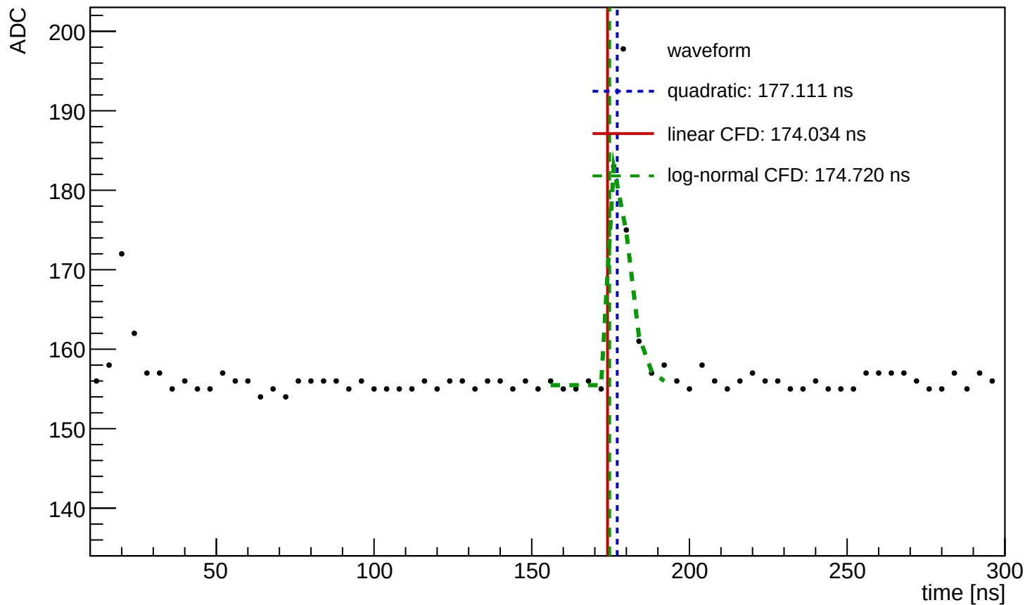
Waveform Time Demo (entry=785, ch=0, module=3001, trigger=SUM)
