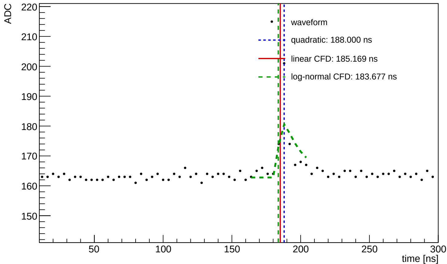
Waveform Time Demo (entry=486, ch=3, module=3002, trigger=SUM)
