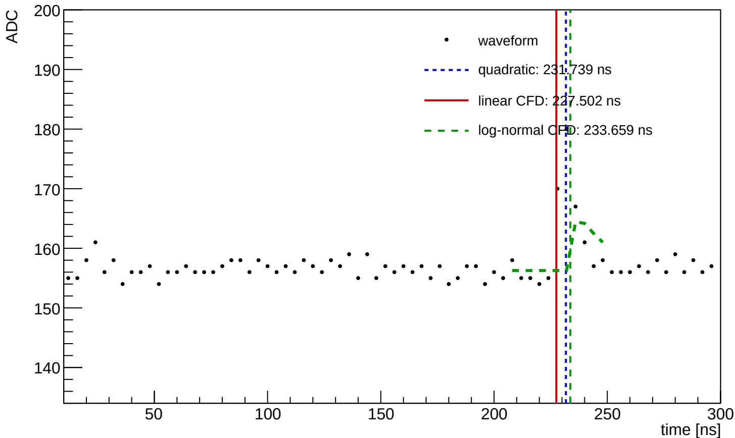
Waveform Time Demo (entry=543, ch=0, module=3001, trigger=SUM)
