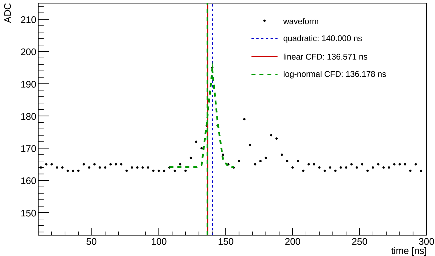
Waveform Time Demo (entry=1114, ch=9, module=3002, trigger=SUM)
