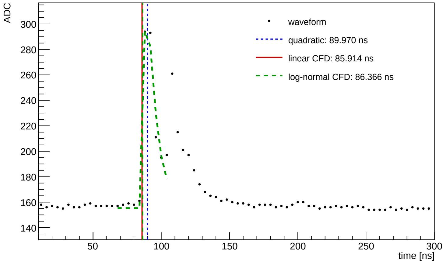
Waveform Time Demo (entry=824, ch=0, module=3001, trigger=SUM)
