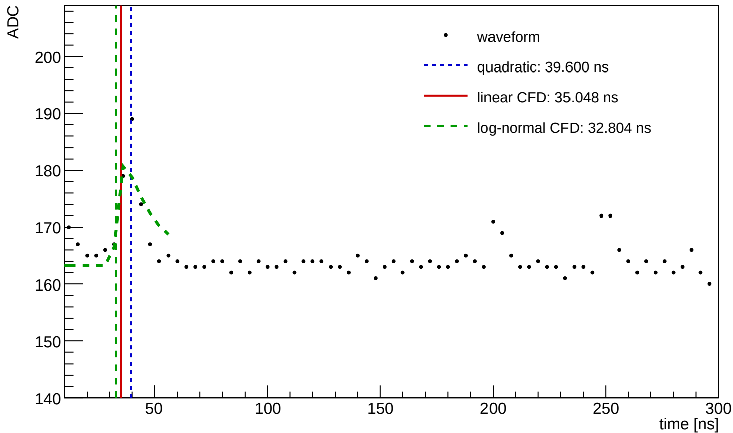
Waveform Time Demo (entry=3026, ch=0, module=3002, trigger=SUM)
