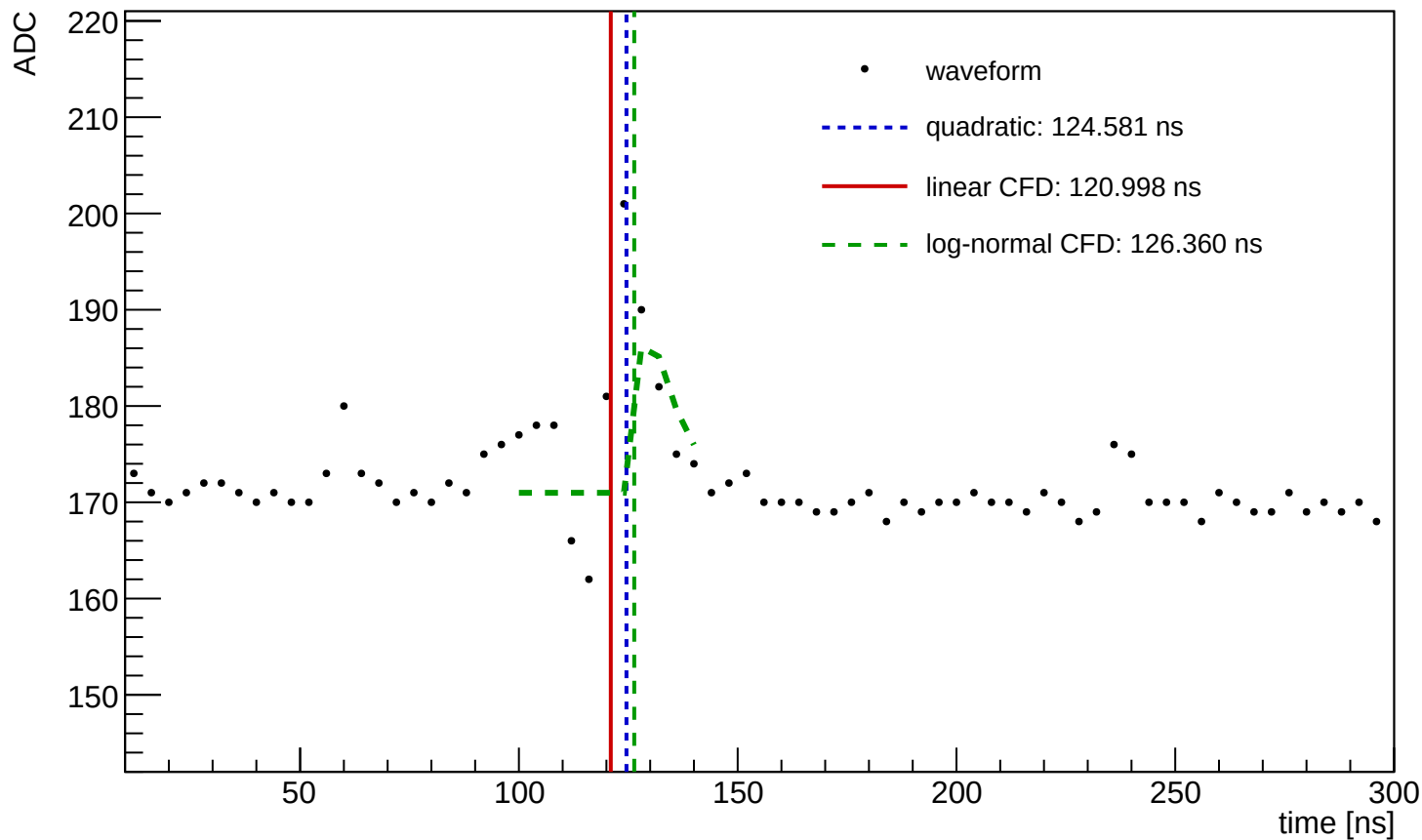
Waveform Time Demo (entry=824, ch=1, module=3004, trigger=SUM)
