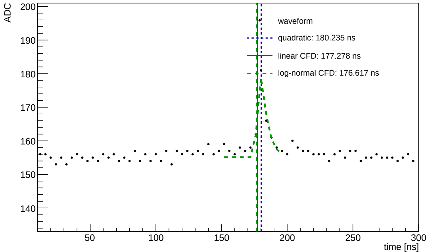
Waveform Time Demo (entry=2576, ch=6, module=3001, trigger=SUM)
