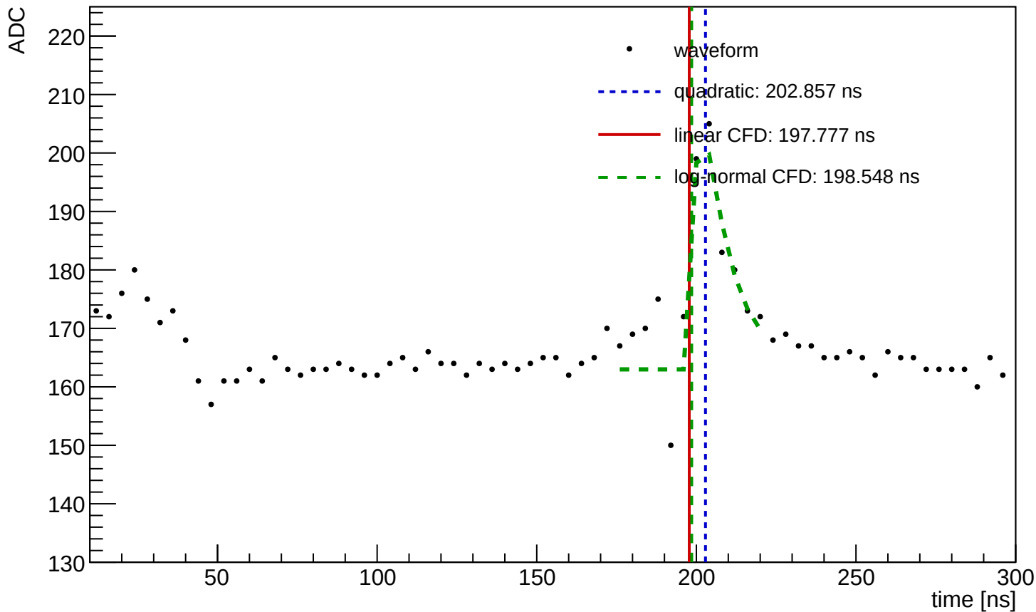
Waveform Time Demo (entry=3096, ch=0, module=3002, trigger=SUM)
