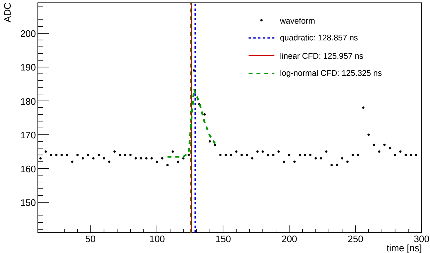
Waveform Time Demo (entry=2165, ch=2, module=3002, trigger=SUM)
