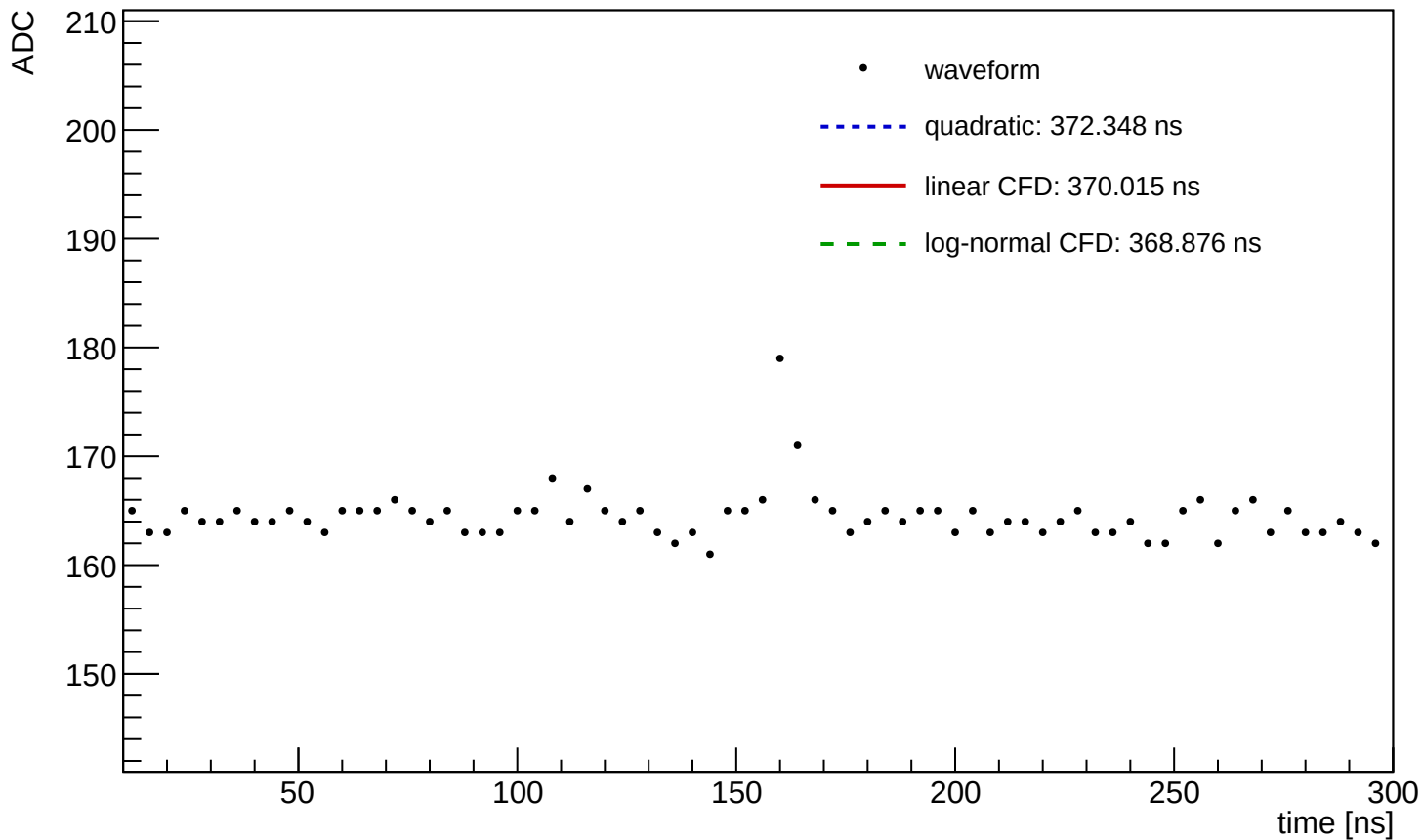
Waveform Time Demo (entry=868, ch=0, module=3002, trigger=SUM)
