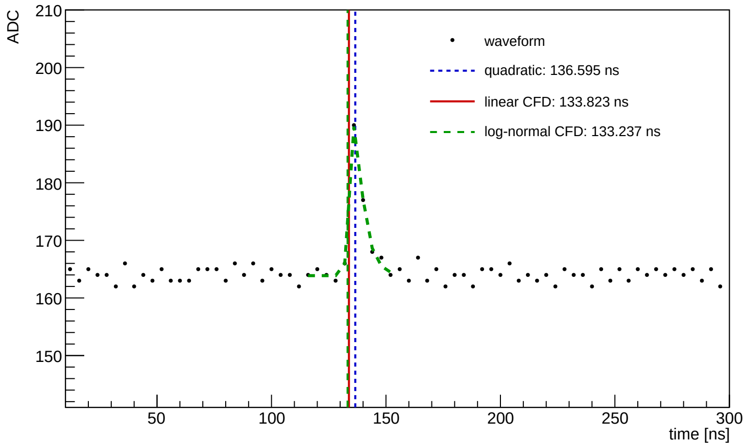
Waveform Time Demo (entry=2527, ch=9, module=3002, trigger=SUM)
