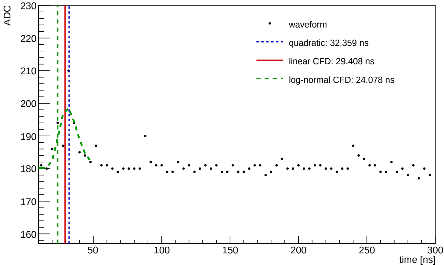
Waveform Time Demo (entry=2845, ch=0, module=3003, trigger=SUM)
