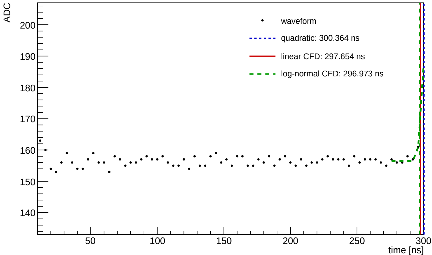
Waveform Time Demo (entry=709, ch=0, module=3001, trigger=SUM)
