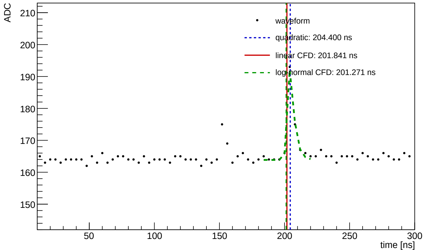
Waveform Time Demo (entry=1883, ch=4, module=3002, trigger=SUM)
