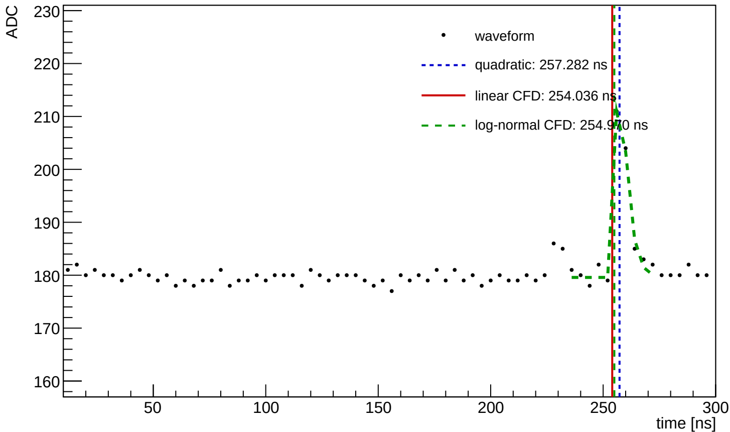
Waveform Time Demo (entry=2550, ch=4, module=3003, trigger=SUM)
