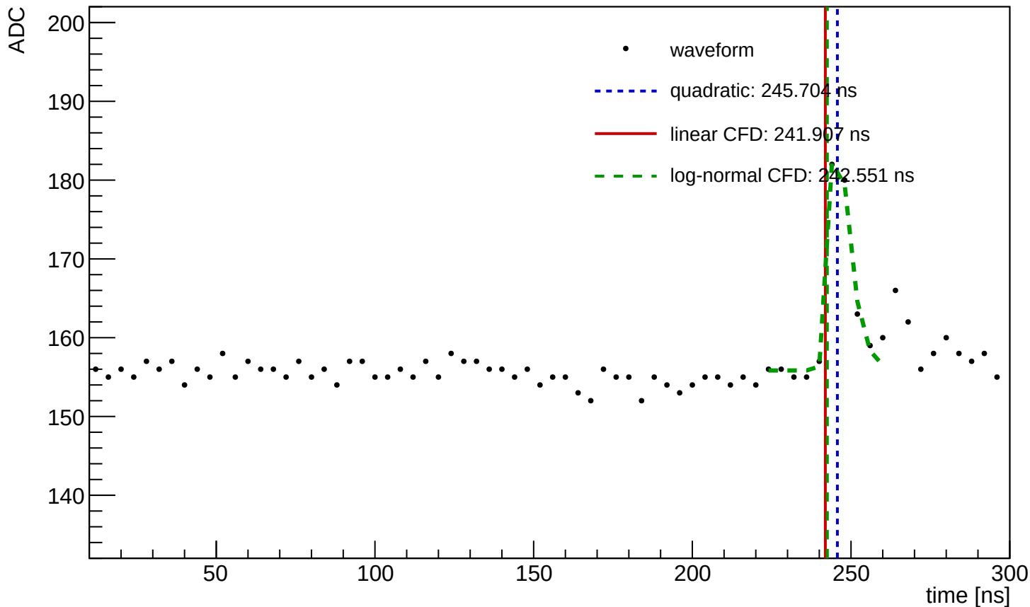
Waveform Time Demo (entry=508, ch=2, module=3001, trigger=SUM)
