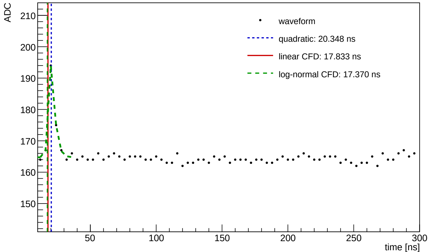
Waveform Time Demo (entry=2654, ch=3, module=3002, trigger=SUM)
