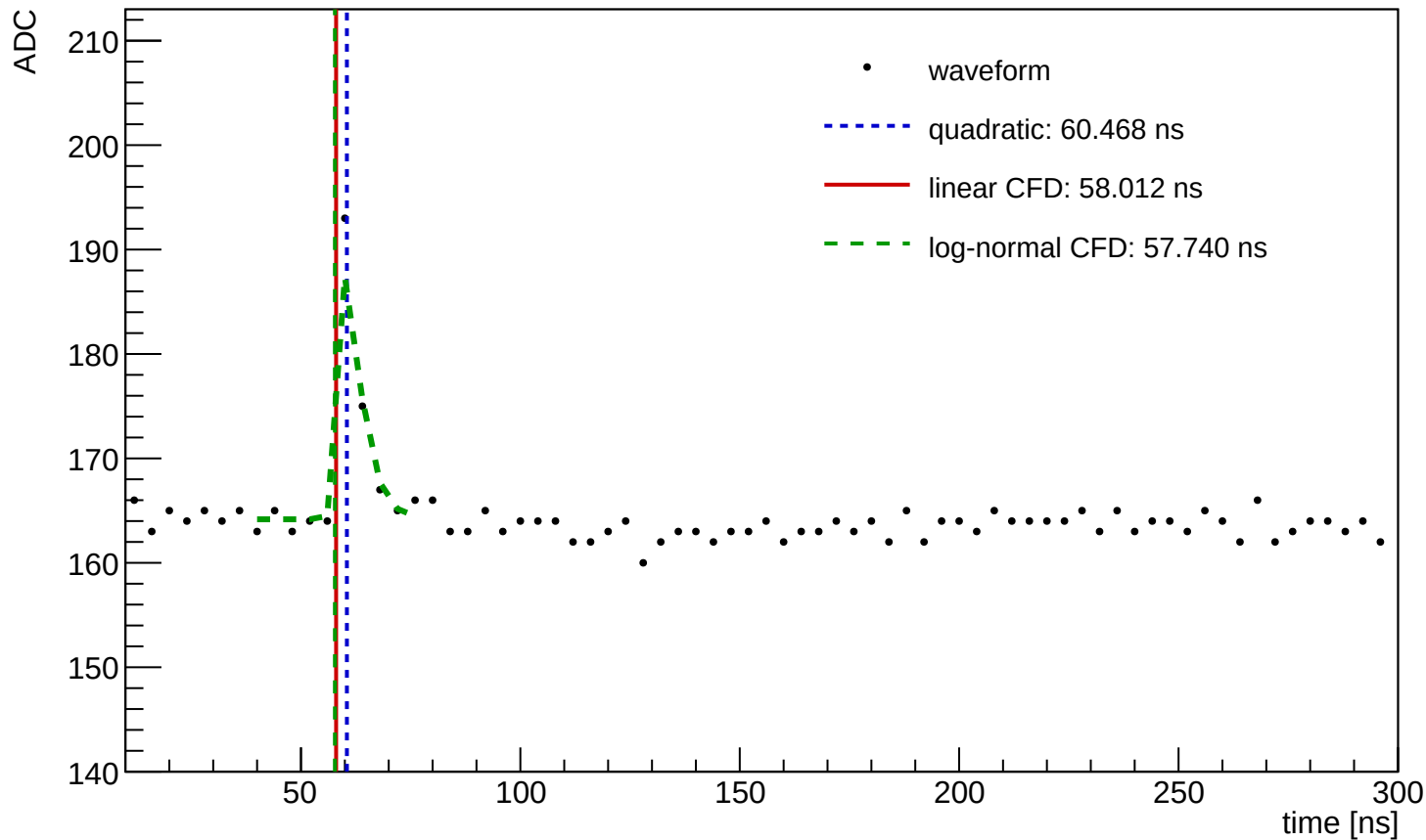
Waveform Time Demo (entry=337, ch=9, module=3002, trigger=SUM)
