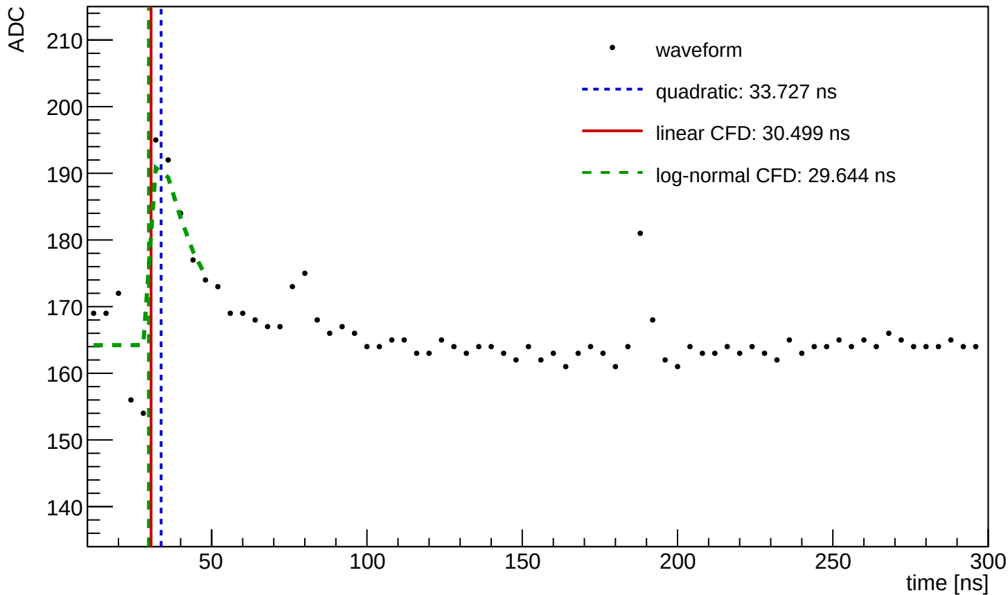
Waveform Time Demo (entry=2984, ch=0, module=3002, trigger=SUM)
