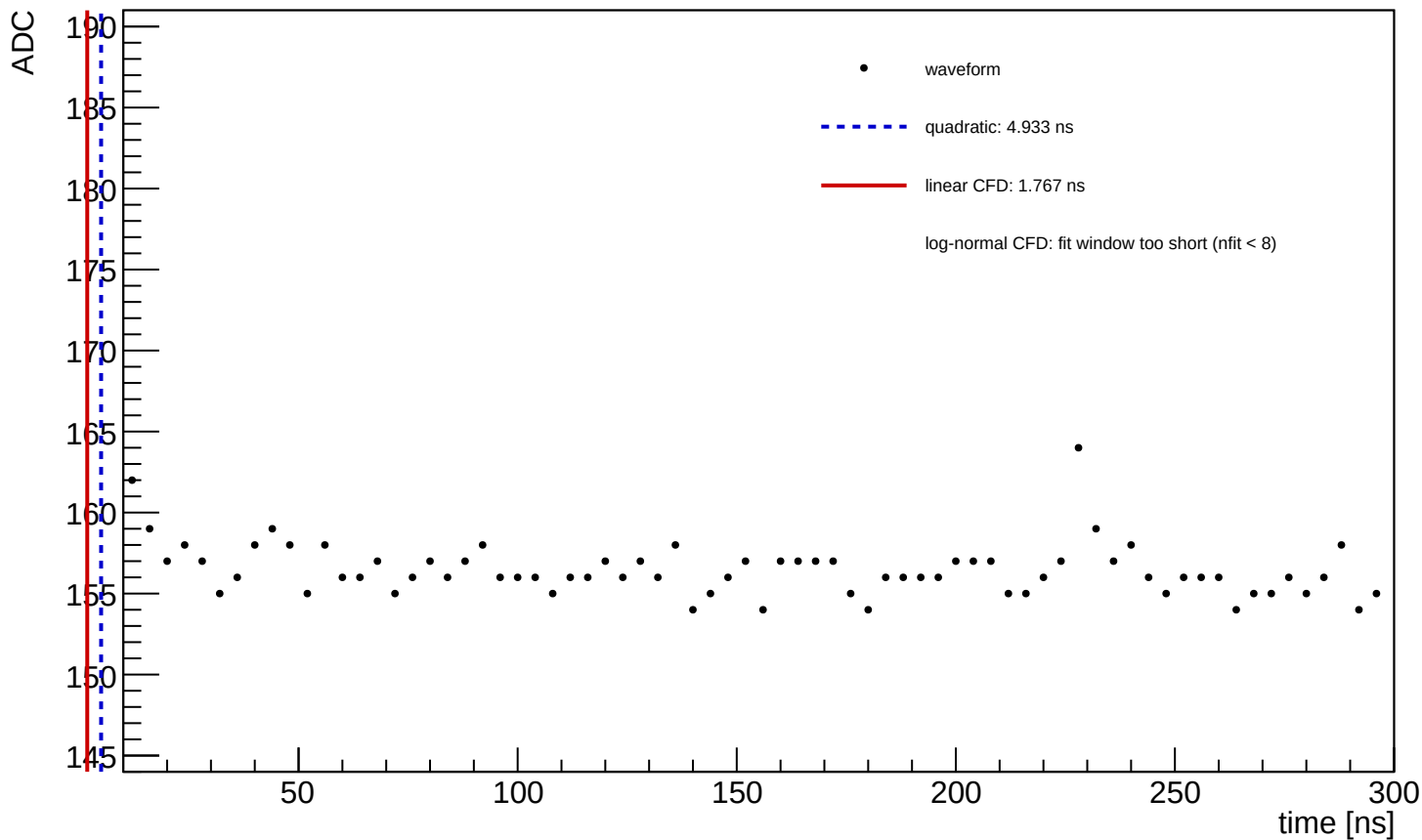
Waveform Time Demo (entry=1766, ch=10, module=3001, trigger=SUM)
