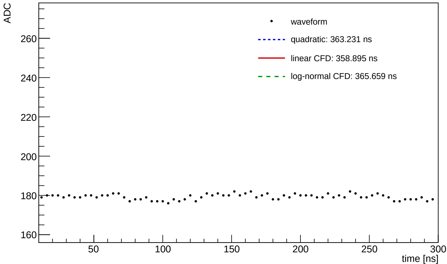
Waveform Time Demo (entry=803, ch=1, module=3003, trigger=SUM)
