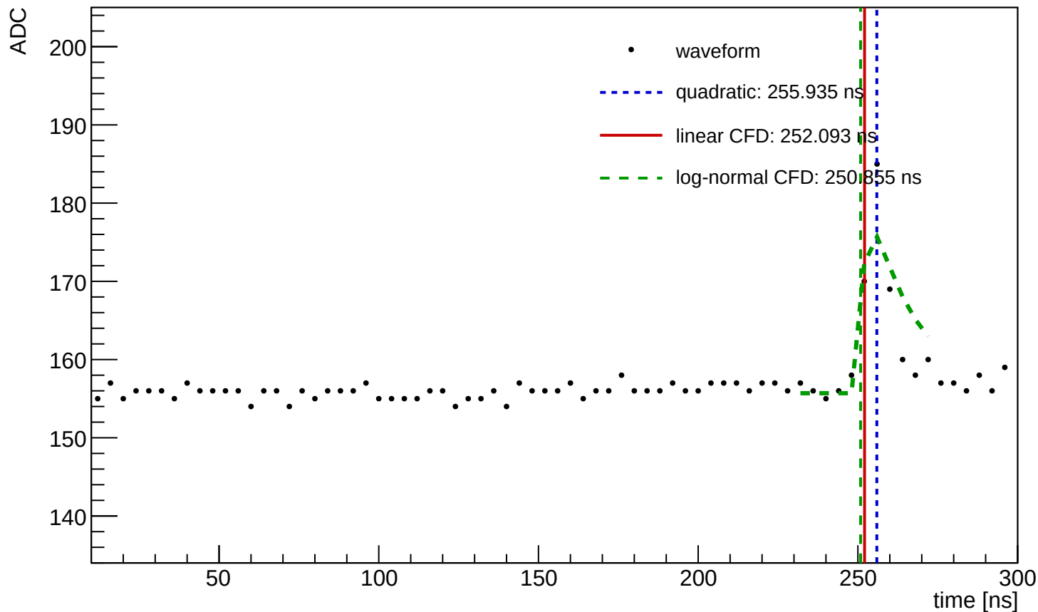
Waveform Time Demo (entry=1394, ch=5, module=3001, trigger=SUM)
