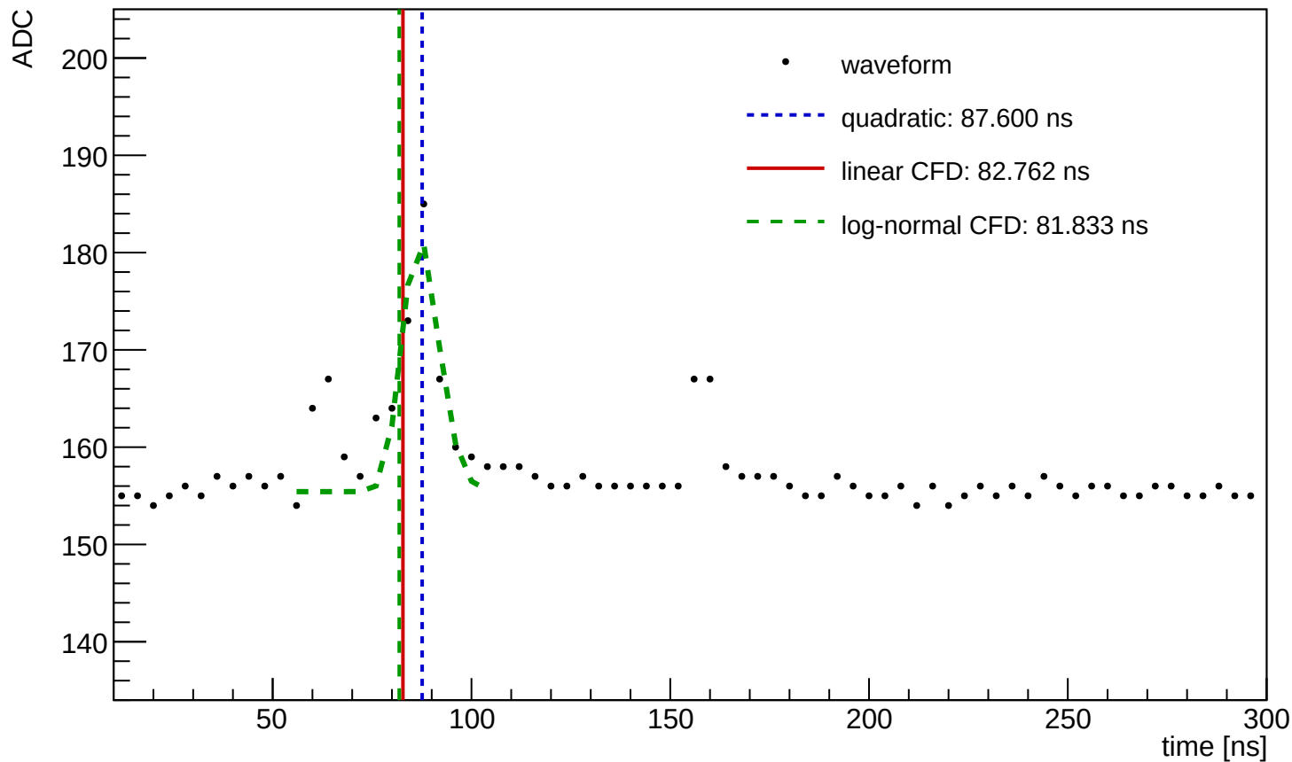
Waveform Time Demo (entry=530, ch=6, module=3001, trigger=SUM)
