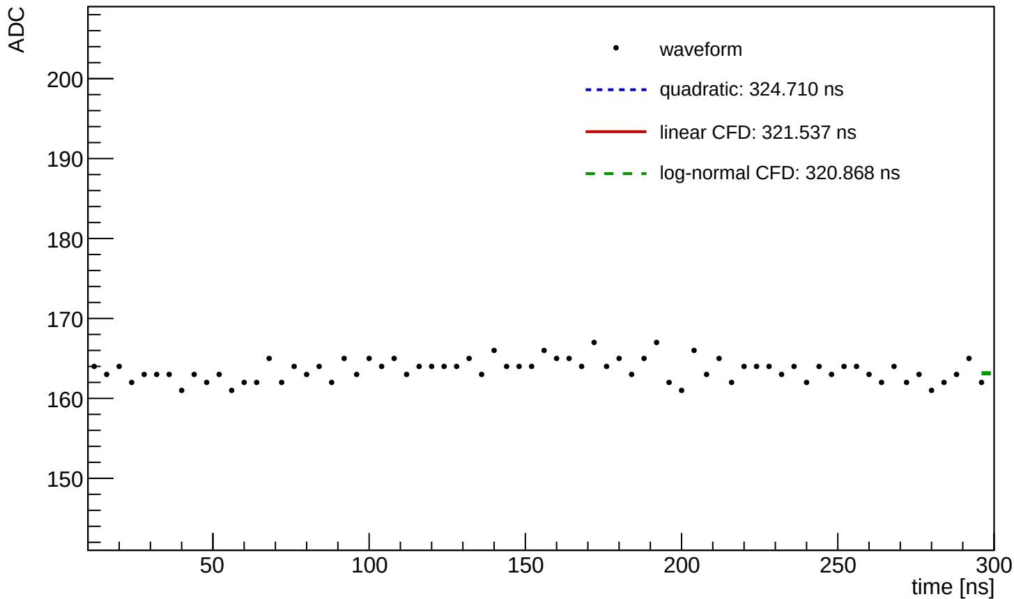
Waveform Time Demo (entry=831, ch=0, module=3002, trigger=SUM)
