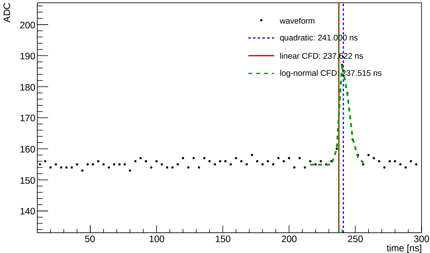
Waveform Time Demo (entry=2600, ch=1, module=3001, trigger=SUM)
