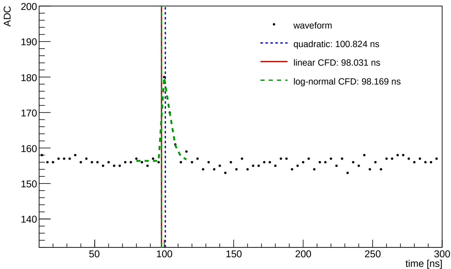
Waveform Time Demo (entry=156, ch=8, module=3001, trigger=SUM)
