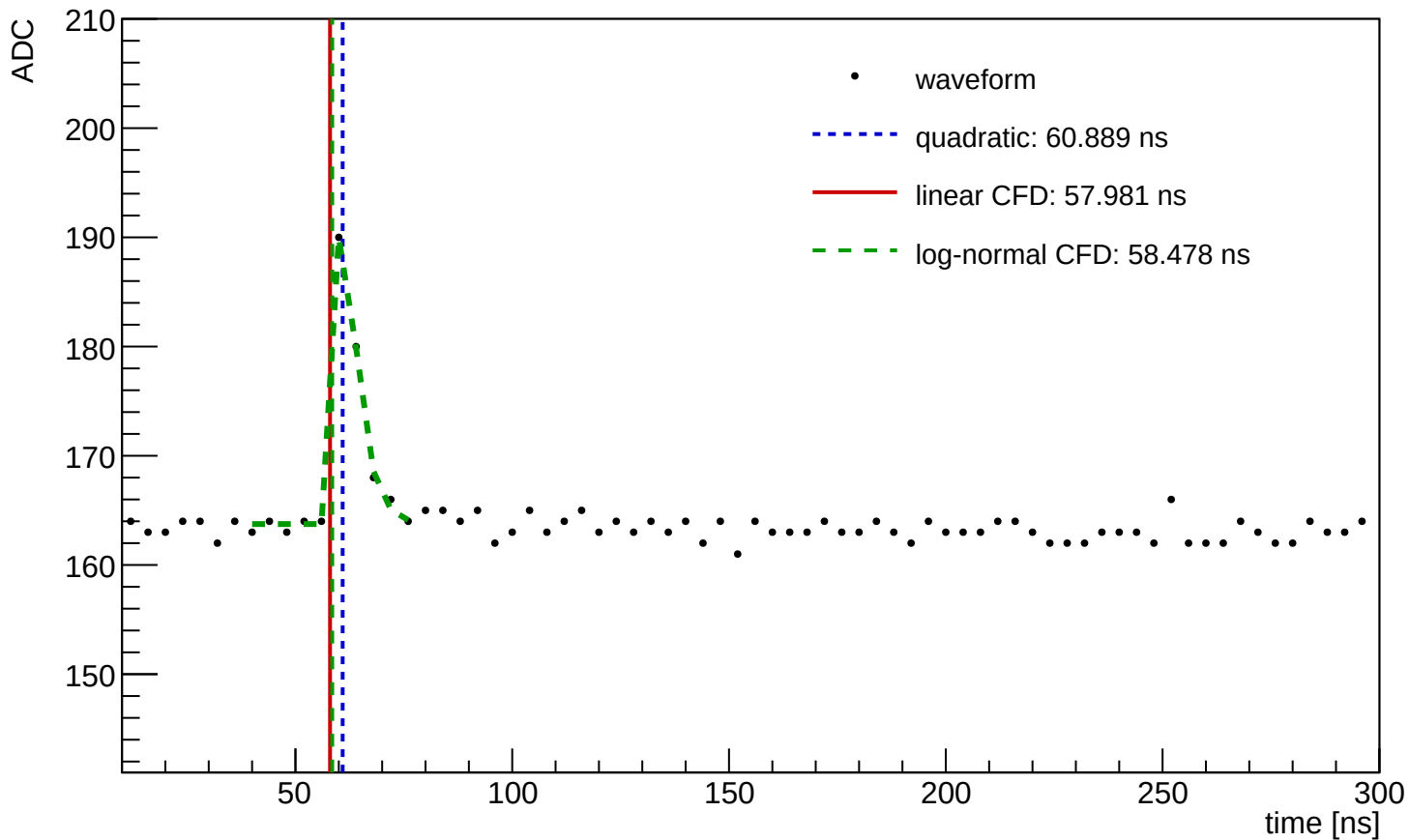
Waveform Time Demo (entry=1611, ch=0, module=3002, trigger=SUM)
