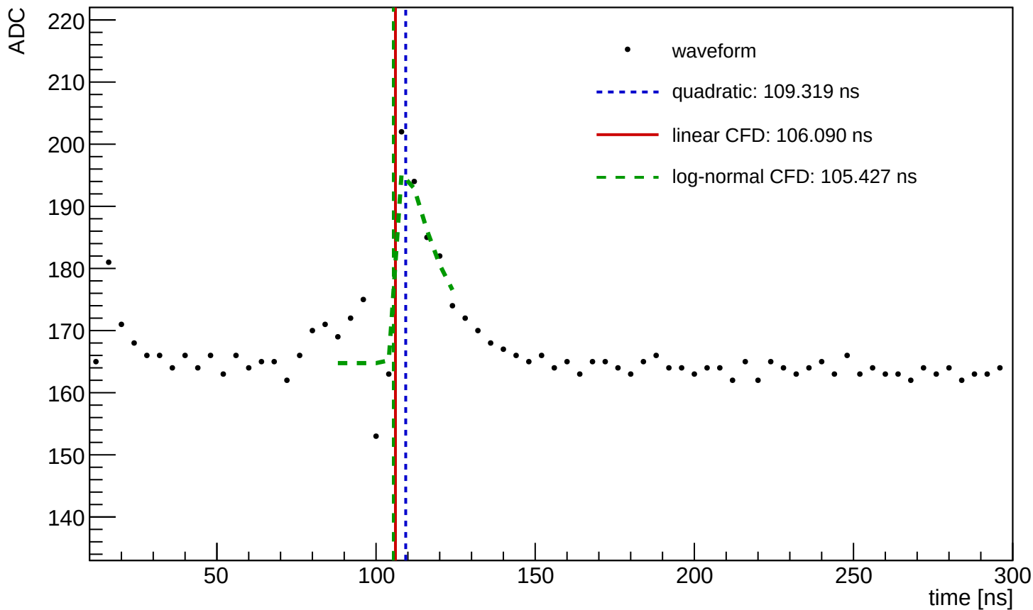
Waveform Time Demo (entry=1970, ch=0, module=3002, trigger=SUM)
