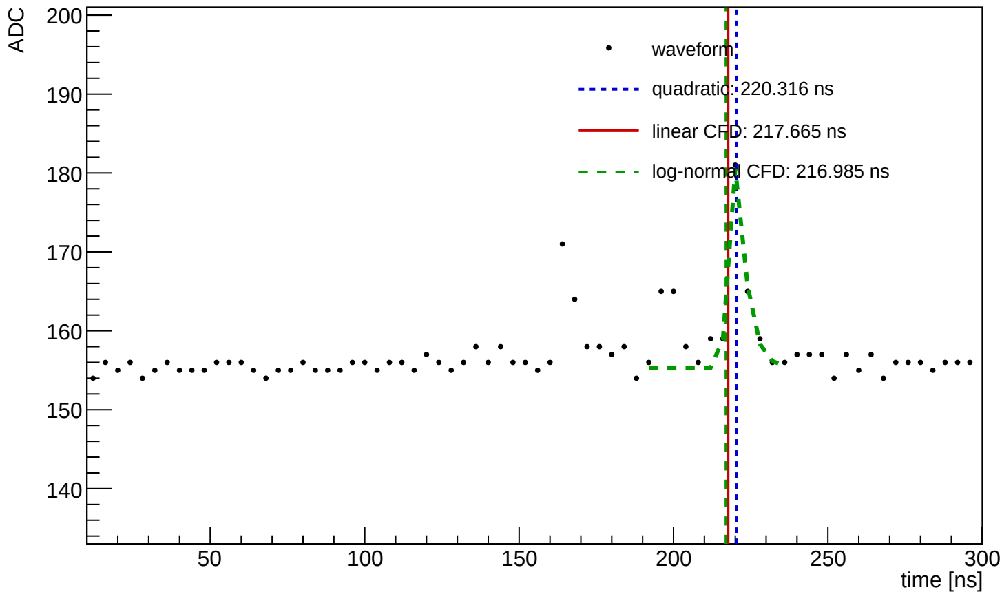
Waveform Time Demo (entry=1516, ch=1, module=3001, trigger=SUM)
