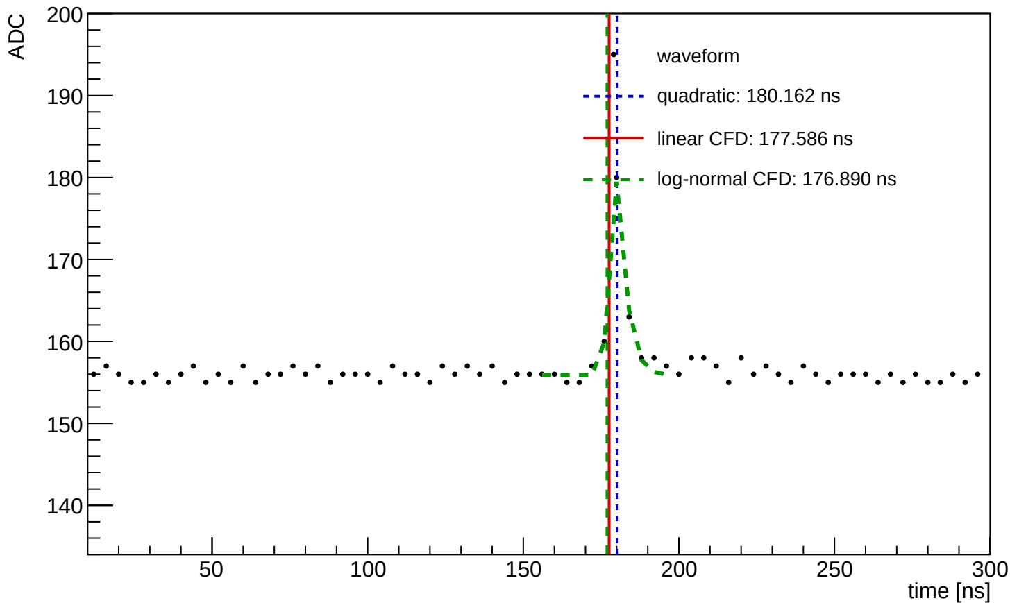
Waveform Time Demo (entry=3099, ch=0, module=3001, trigger=SUM)
