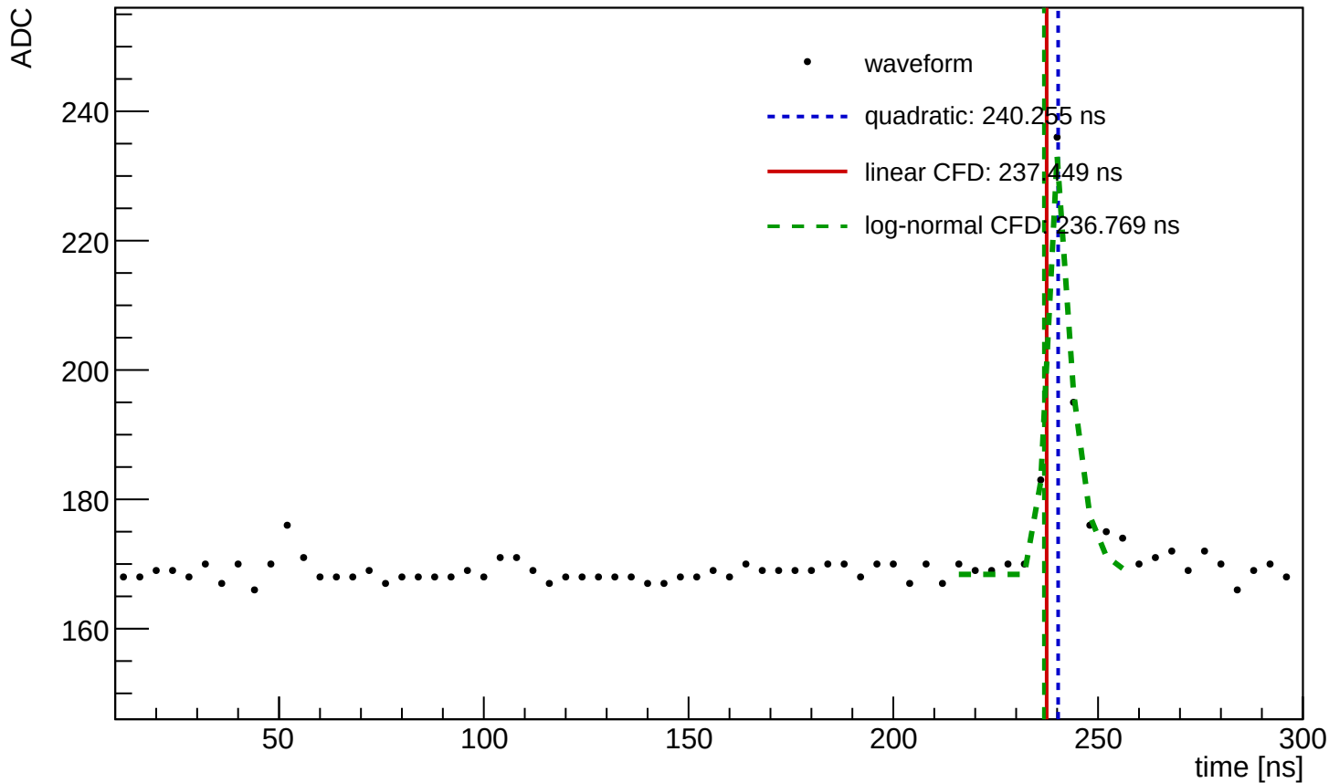
Waveform Time Demo (entry=1942, ch=6, module=3004, trigger=SUM)
