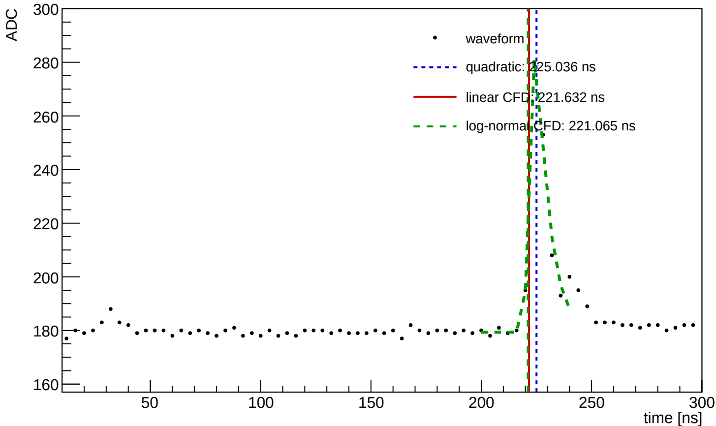
Waveform Time Demo (entry=614, ch=10, module=3003, trigger=SUM)
