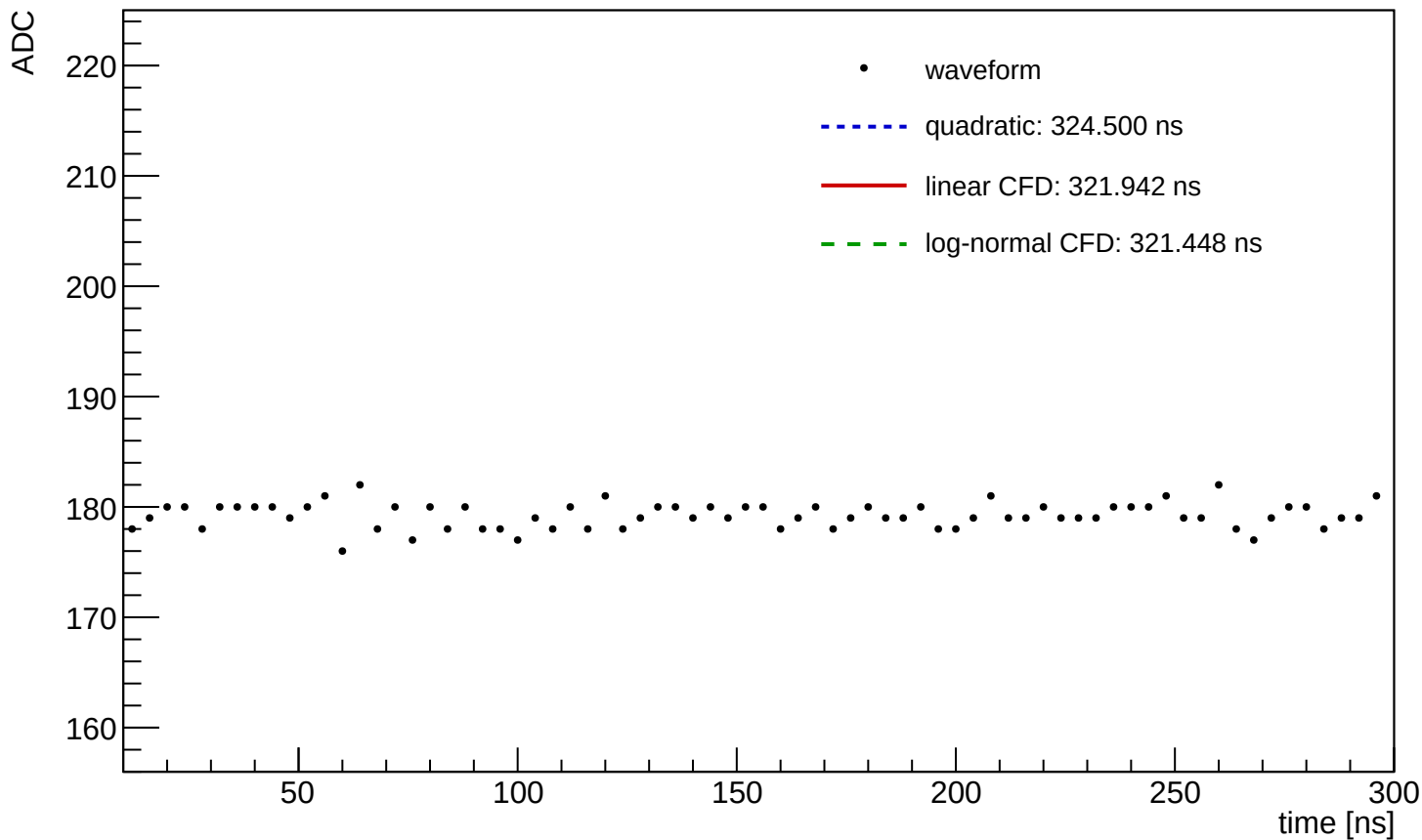
Waveform Time Demo (entry=917, ch=0, module=3003, trigger=SUM)
