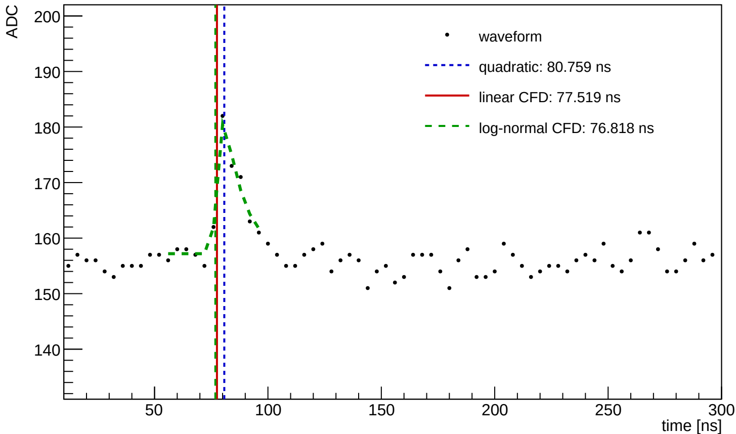
Waveform Time Demo (entry=989, ch=9, module=3001, trigger=SUM)
