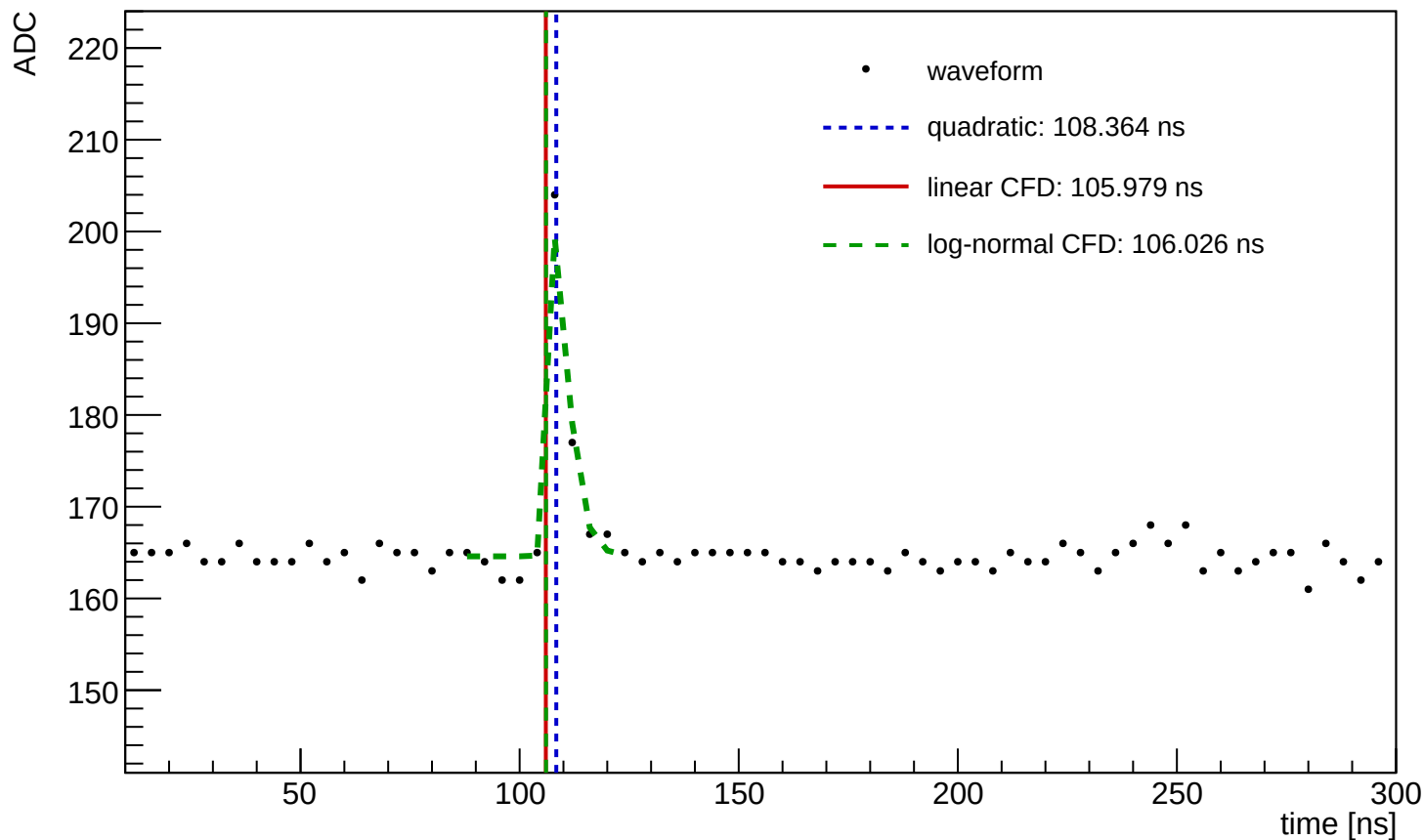
Waveform Time Demo (entry=468, ch=4, module=3002, trigger=SUM)
