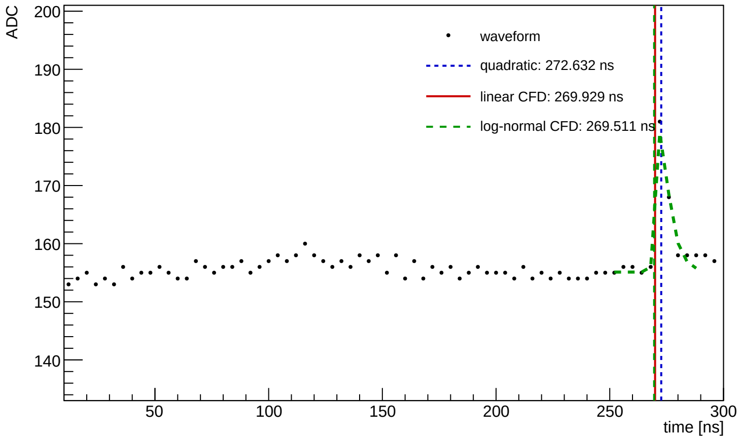
Waveform Time Demo (entry=1866, ch=0, module=3001, trigger=SUM)
