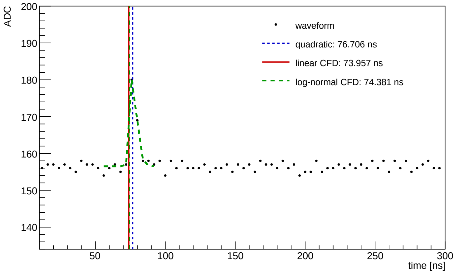
Waveform Time Demo (entry=472, ch=0, module=3001, trigger=SUM)
