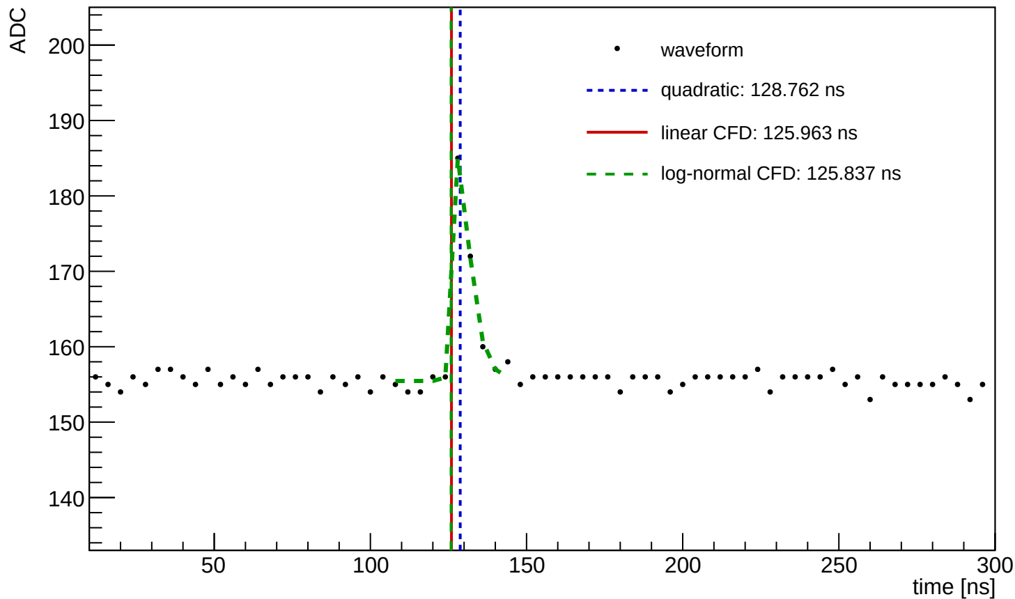
Waveform Time Demo (entry=2343, ch=3, module=3001, trigger=SUM)
