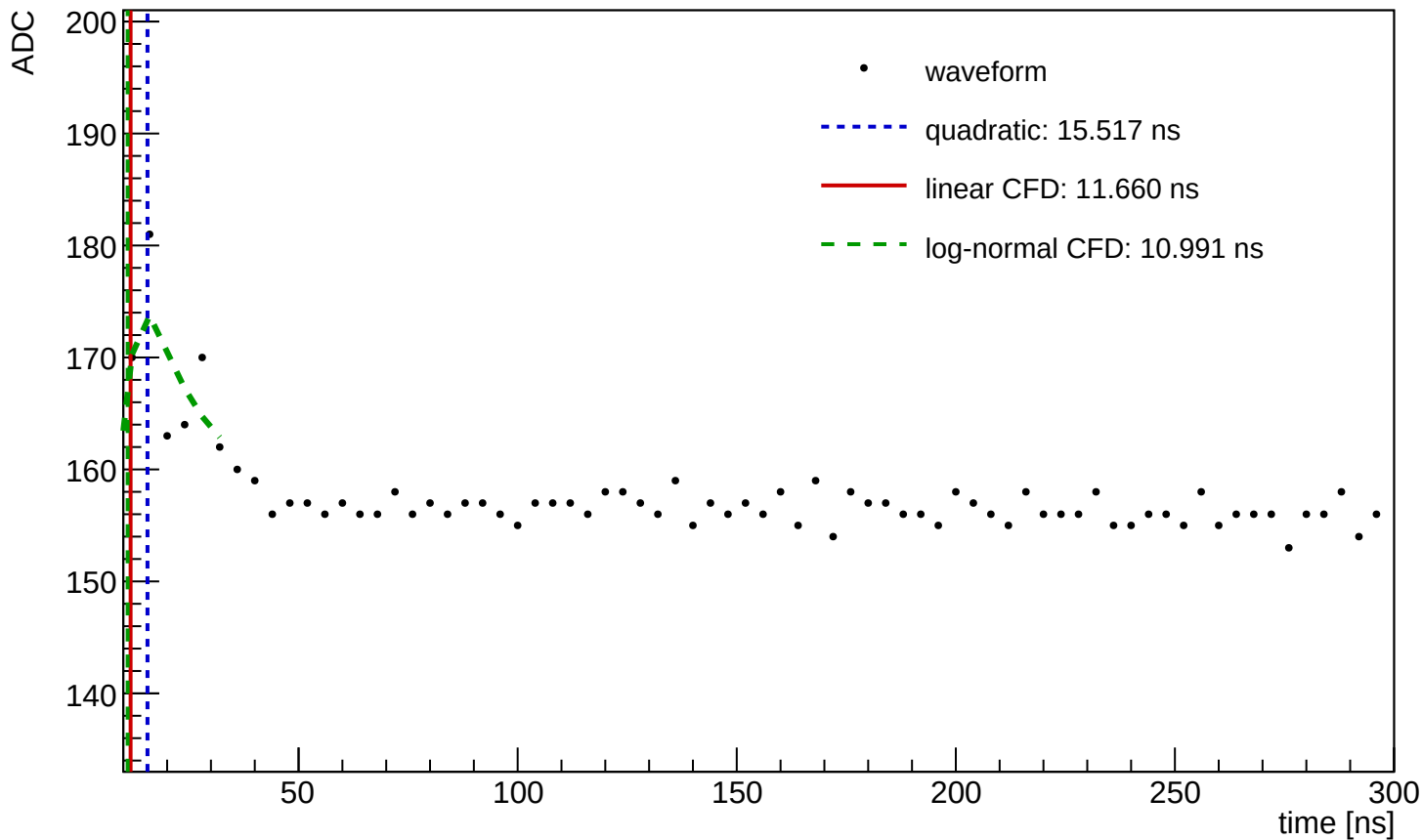
Waveform Time Demo (entry=1405, ch=2, module=3001, trigger=SUM)
