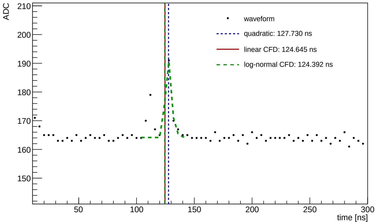
Waveform Time Demo (entry=1289, ch=0, module=3002, trigger=SUM)
