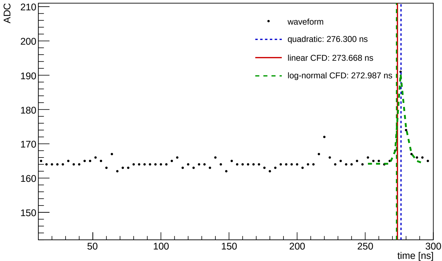
Waveform Time Demo (entry=344, ch=5, module=3002, trigger=SUM)
