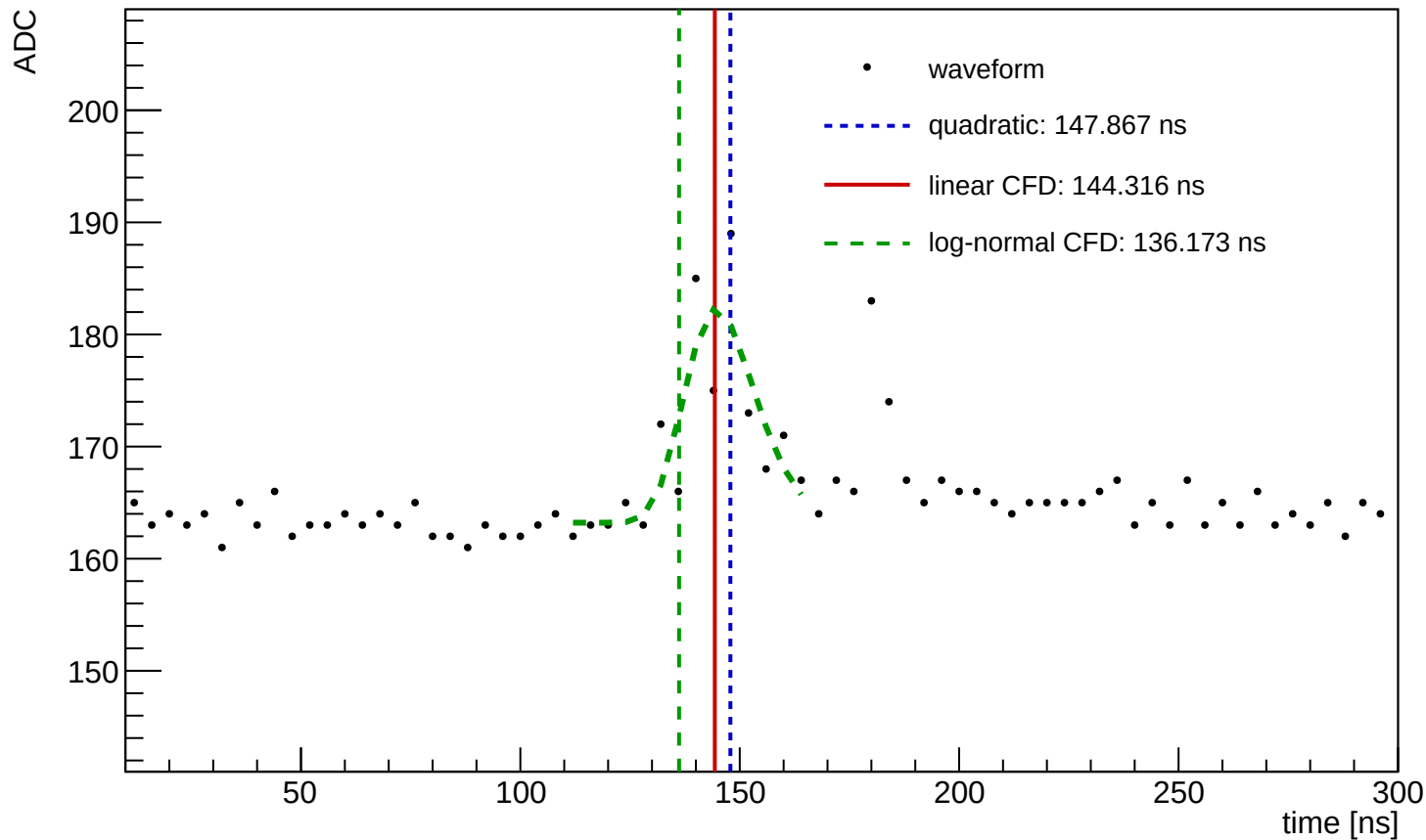
Waveform Time Demo (entry=800, ch=0, module=3002, trigger=SUM)
