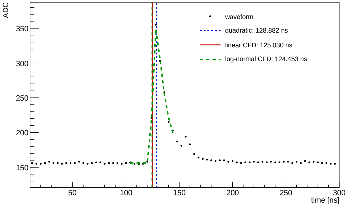
Waveform Time Demo (entry=556, ch=0, module=3001, trigger=SUM)
