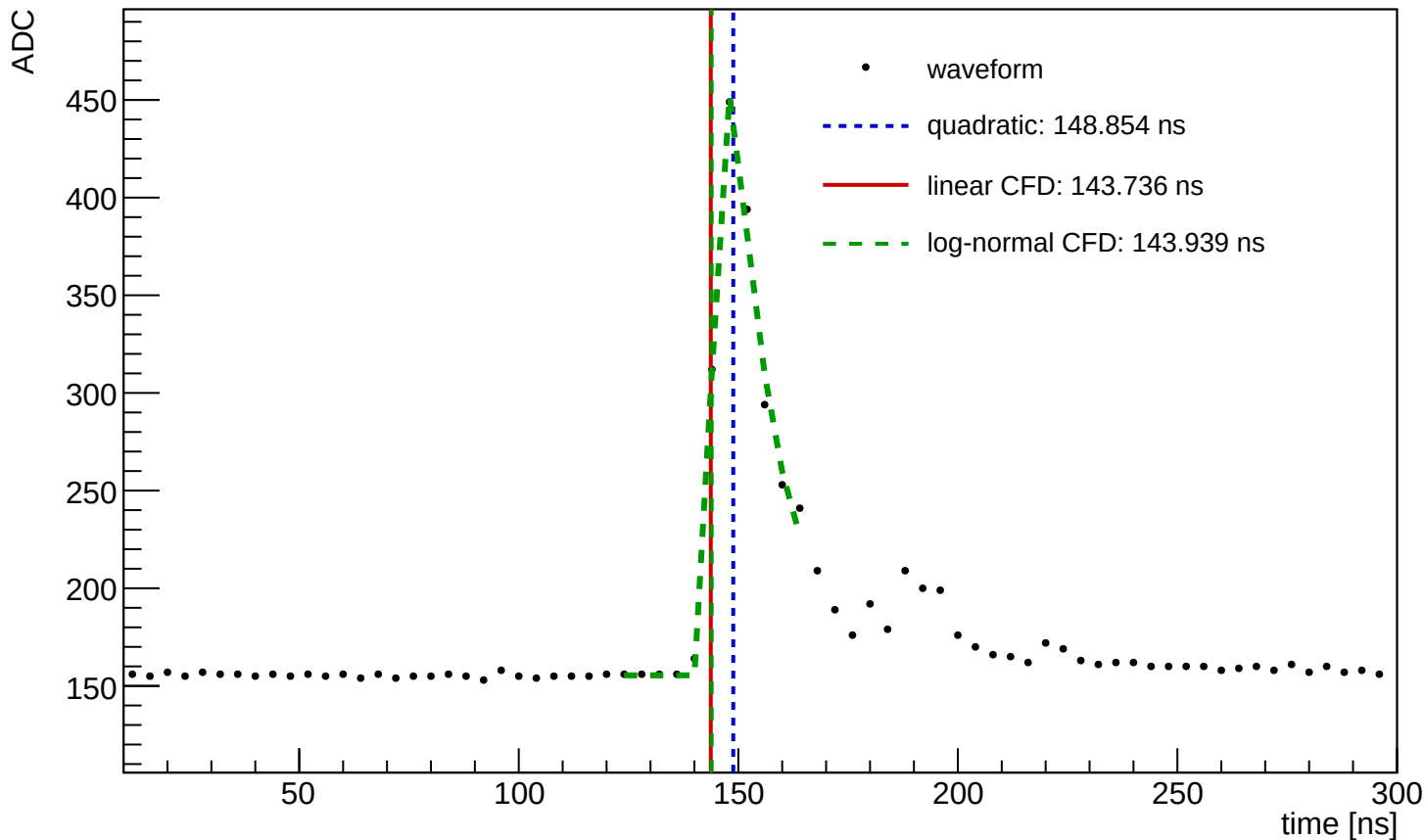
Waveform Time Demo (entry=2161, ch=9, module=3001, trigger=SUM)
