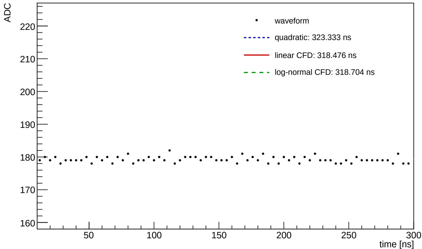
Waveform Time Demo (entry=2458, ch=5, module=3003, trigger=SUM)
