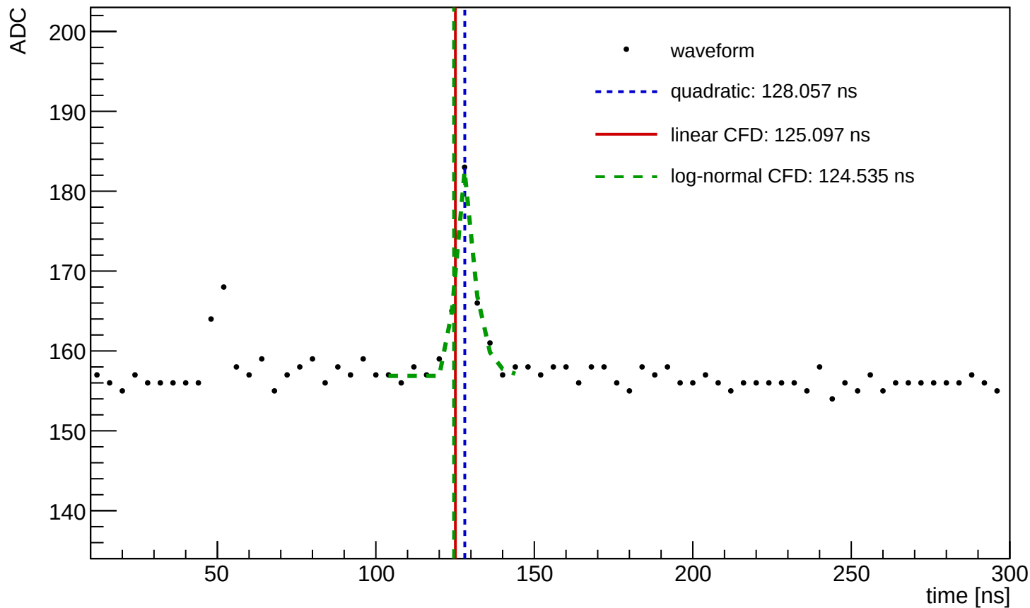
Waveform Time Demo (entry=2217, ch=1, module=3001, trigger=SUM)
