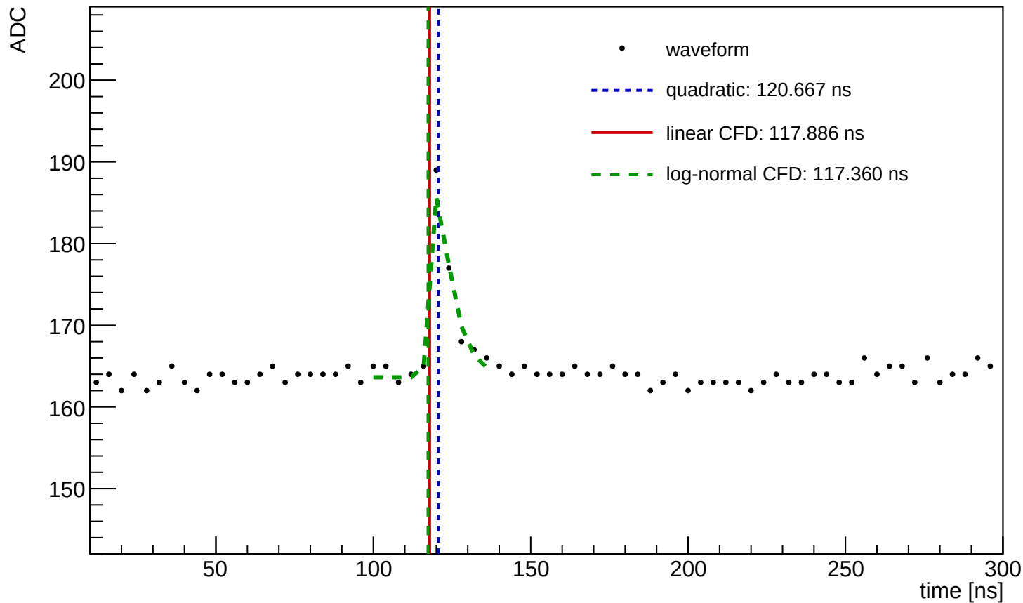
Waveform Time Demo (entry=2234, ch=1, module=3002, trigger=SUM)
