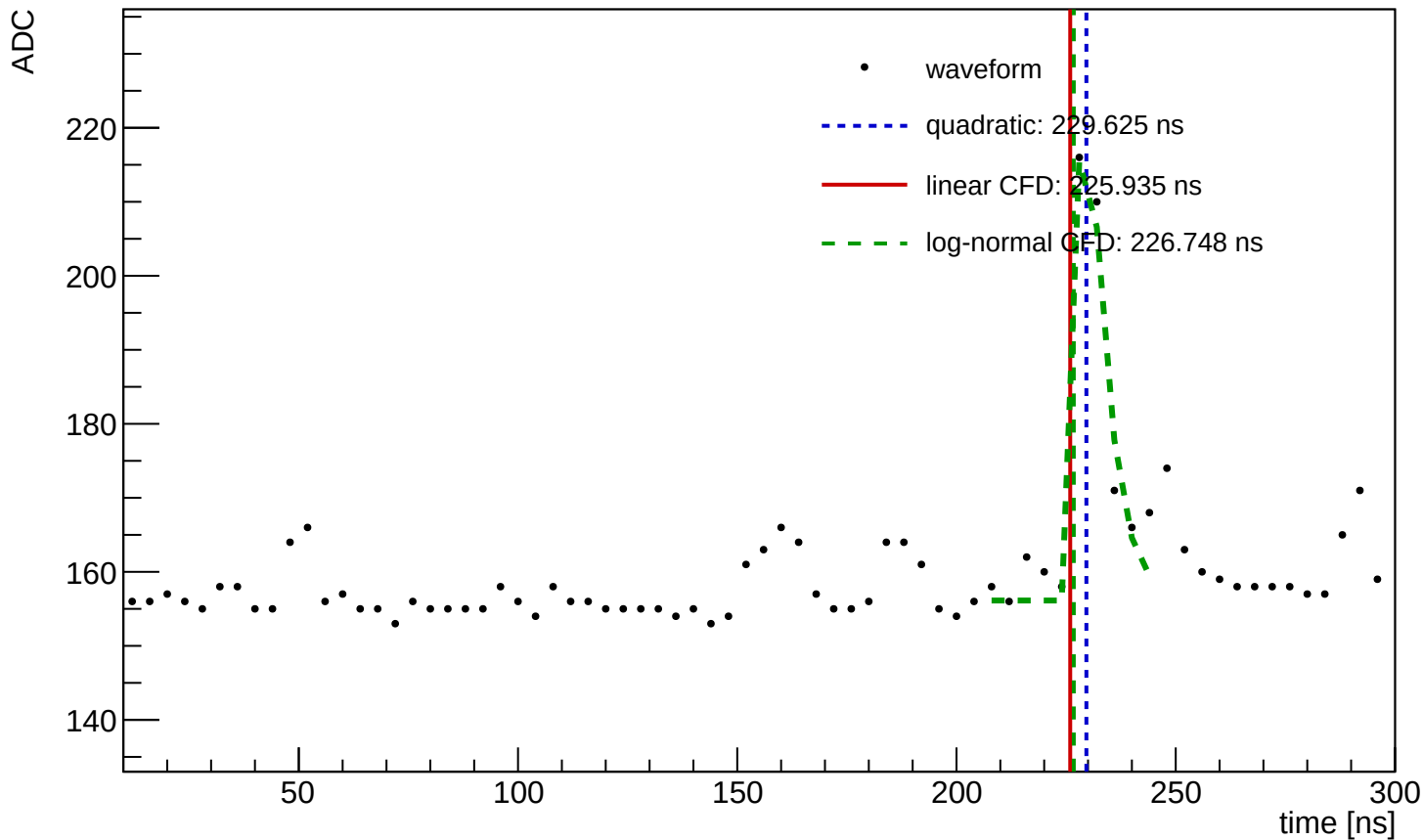
Waveform Time Demo (entry=2691, ch=2, module=3001, trigger=SUM)
