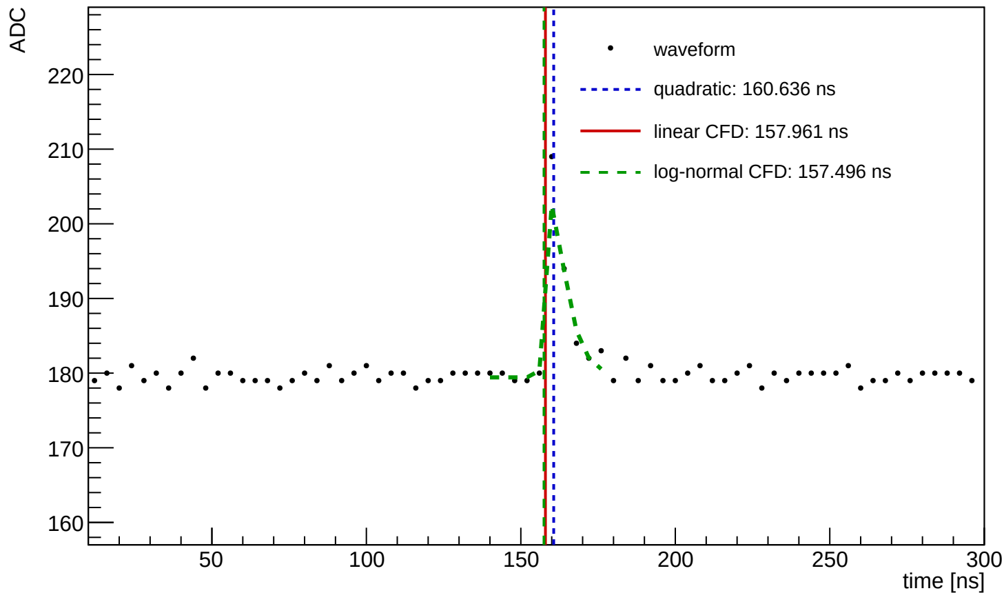
Waveform Time Demo (entry=2107, ch=6, module=3003, trigger=SUM)
