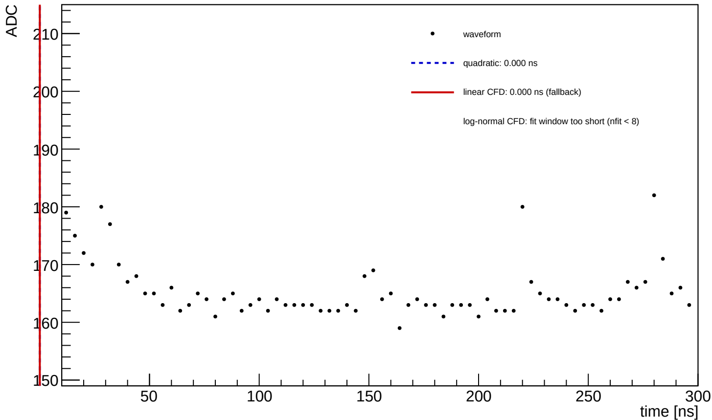
Waveform Time Demo (entry=1063, ch=6, module=3002, trigger=SUM)
