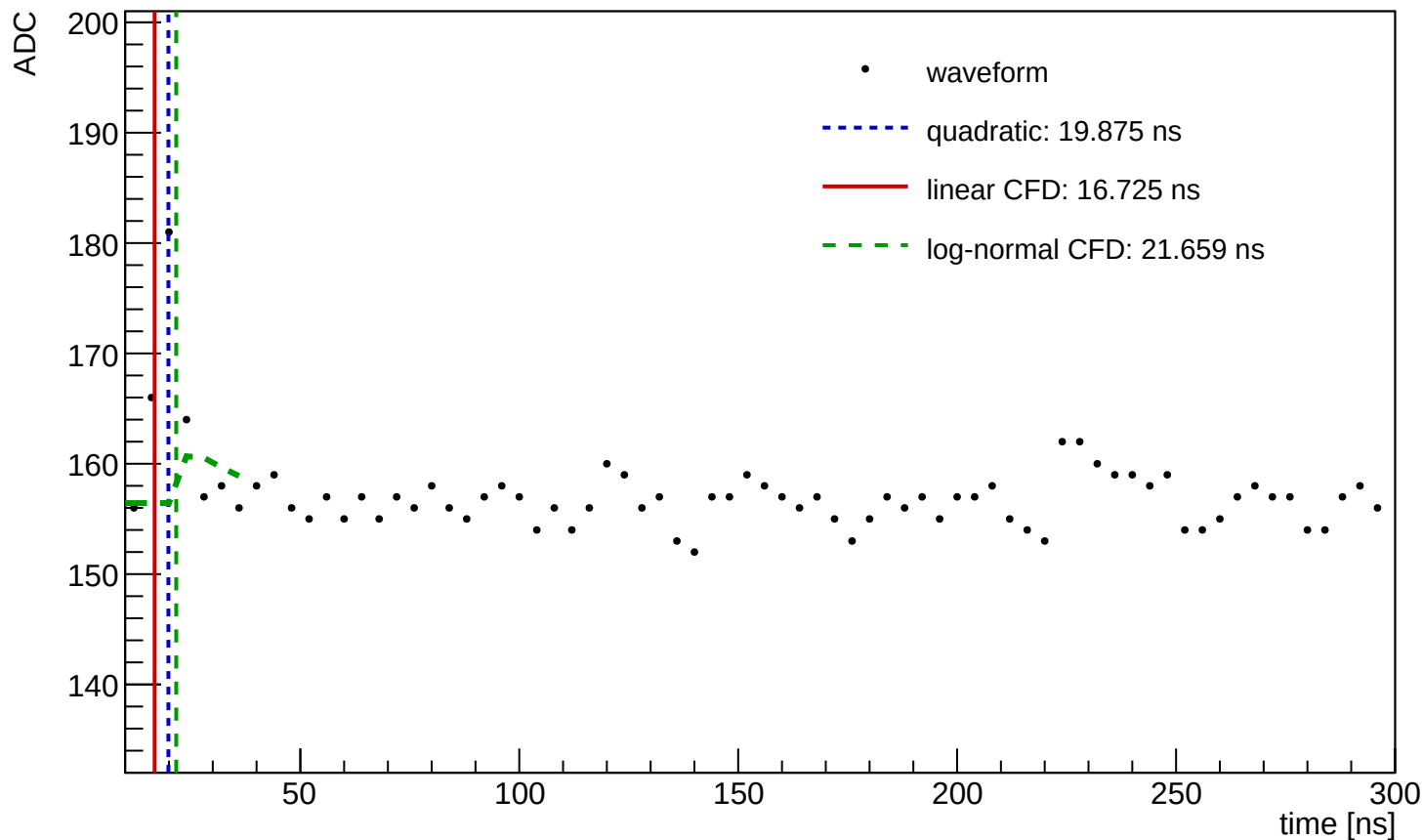
Waveform Time Demo (entry=1128, ch=0, module=3001, trigger=SUM)
