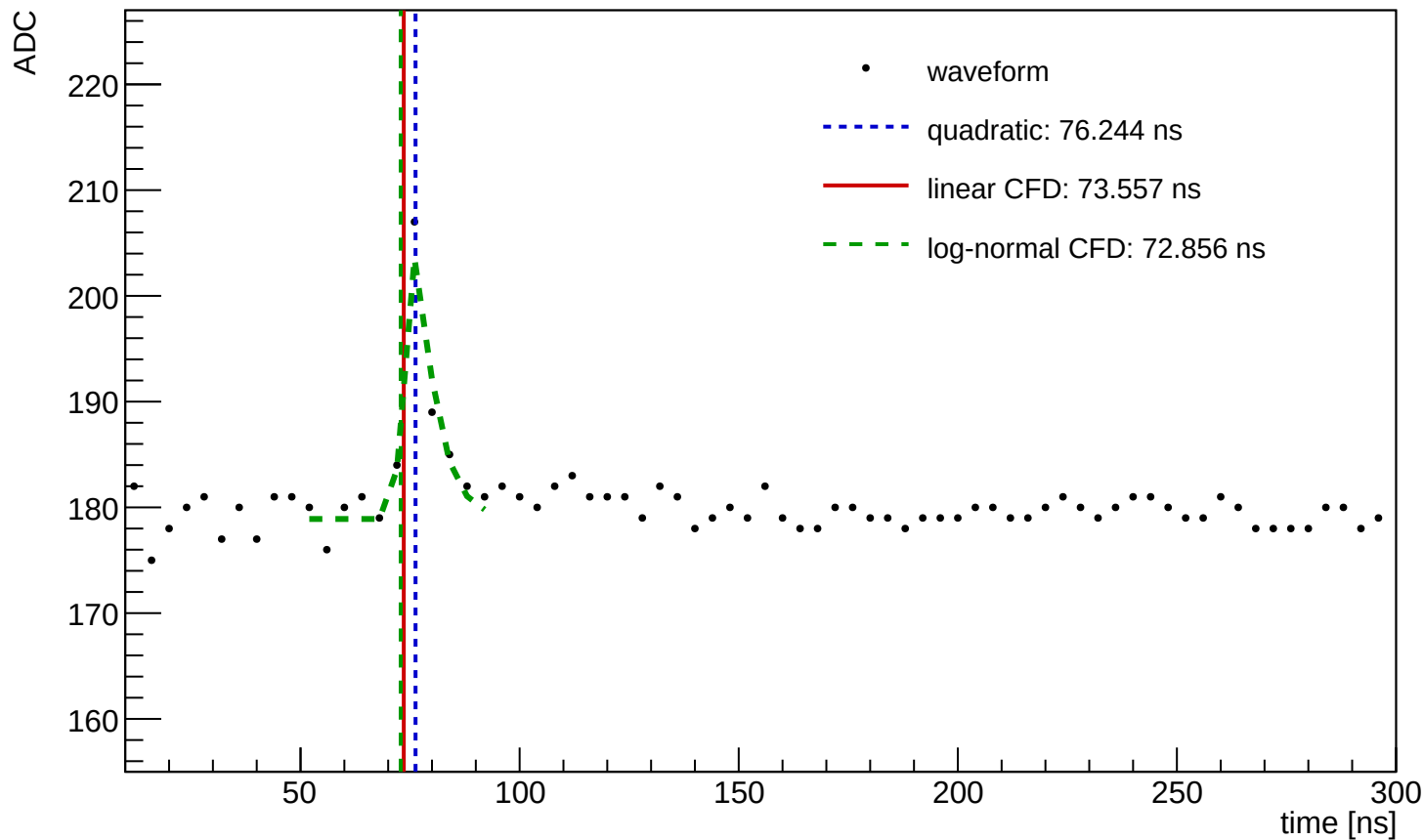
Waveform Time Demo (entry=1594, ch=3, module=3003, trigger=SUM)
