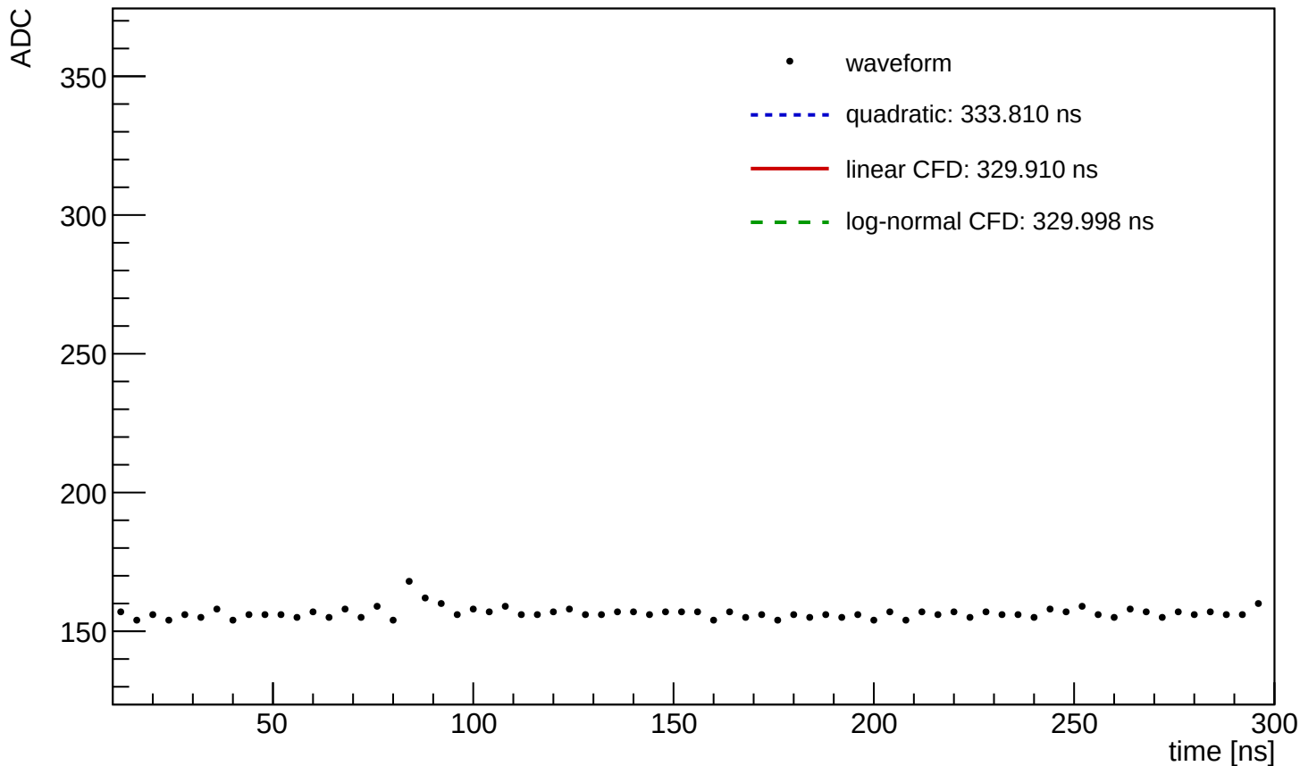
Waveform Time Demo (entry=984, ch=0, module=3001, trigger=SUM)
