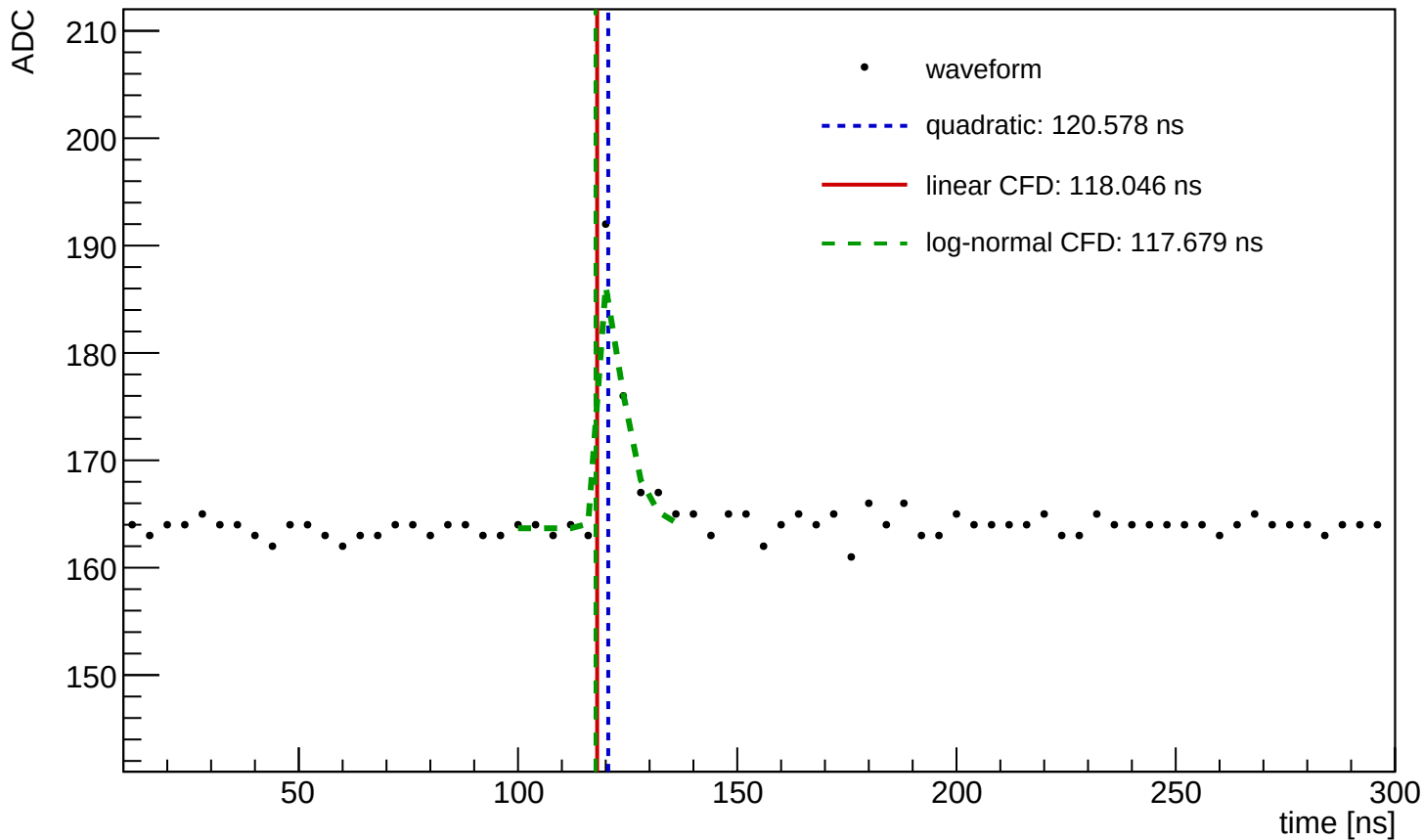
Waveform Time Demo (entry=1248, ch=0, module=3002, trigger=SUM)
