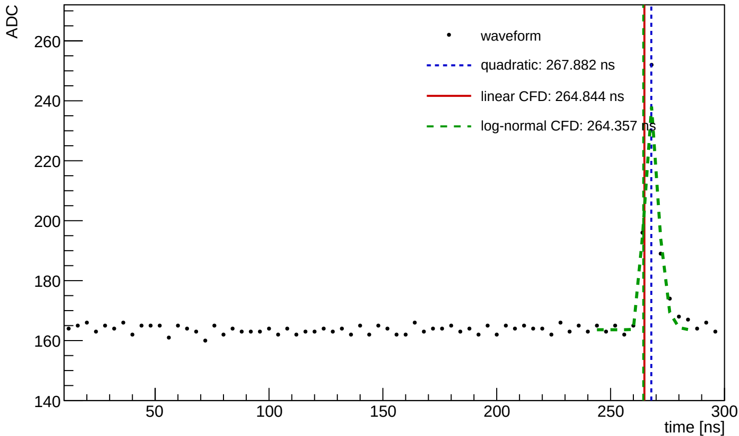
Waveform Time Demo (entry=1886, ch=0, module=3002, trigger=SUM)
