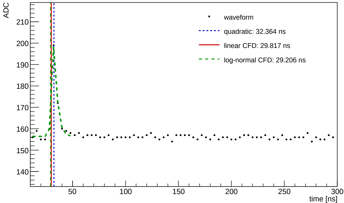
Waveform Time Demo (entry=823, ch=0, module=3001, trigger=SUM)
