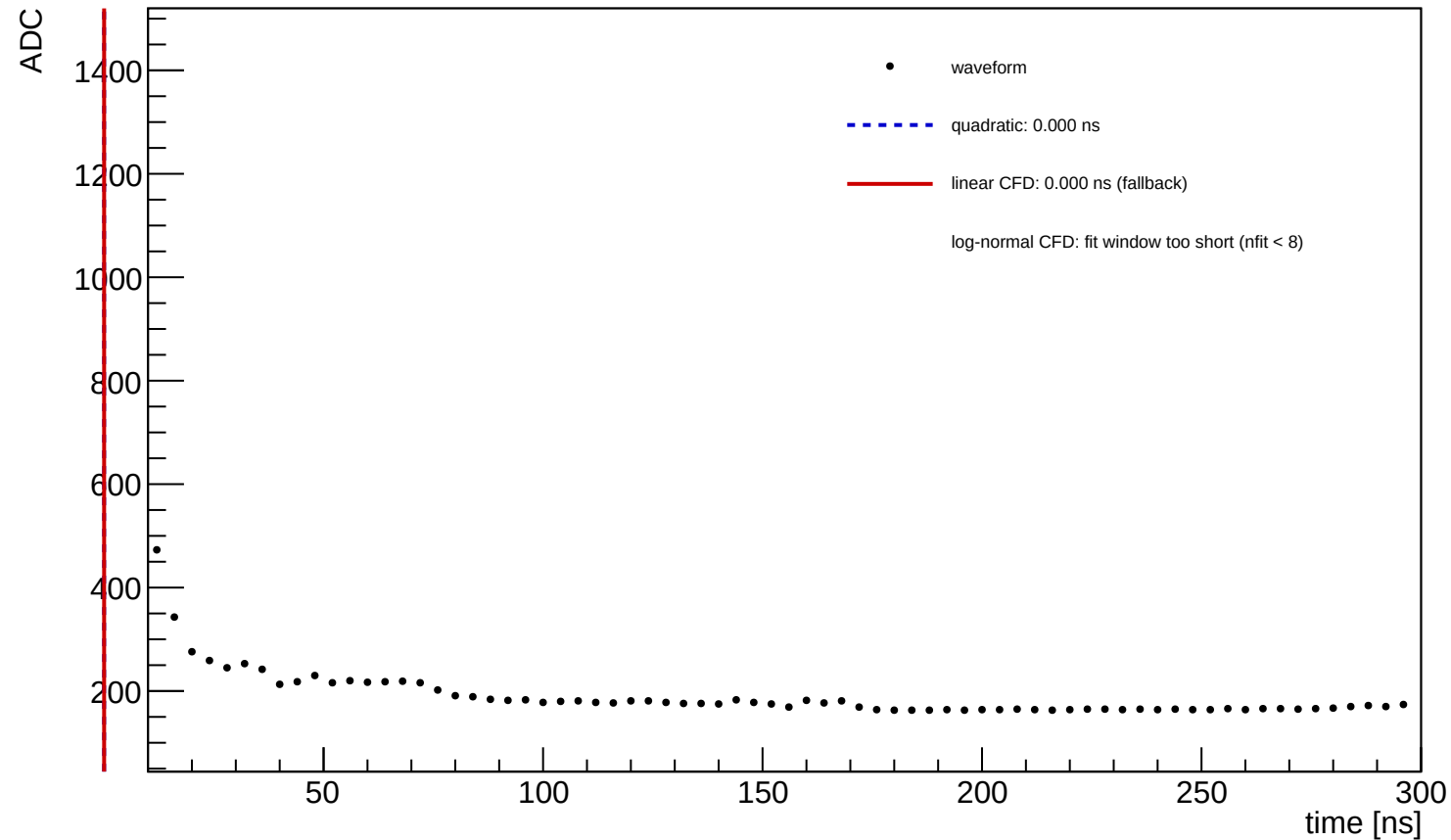
Waveform Time Demo (entry=3159, ch=1, module=3002, trigger=SUM)
