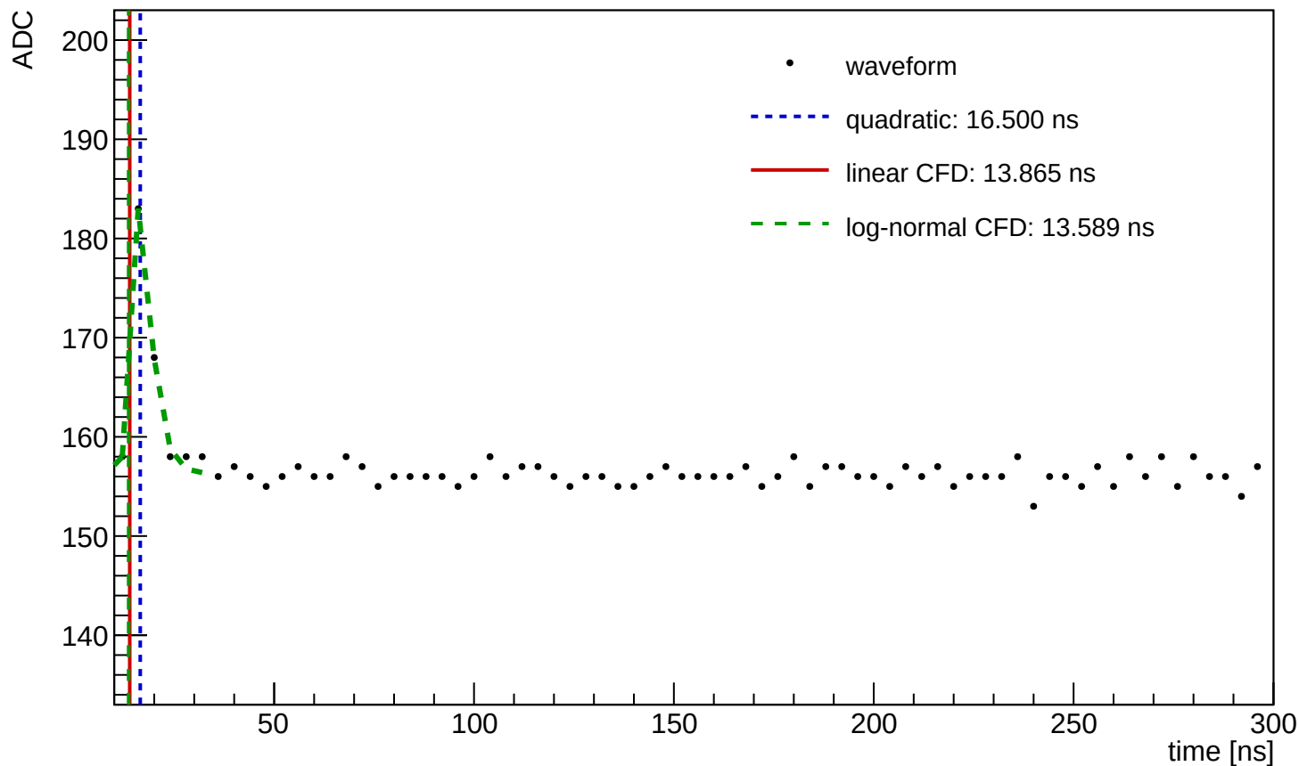
Waveform Time Demo (entry=2645, ch=6, module=3001, trigger=SUM)
