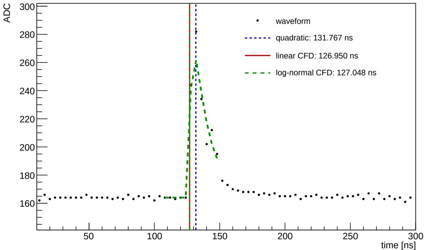
Waveform Time Demo (entry=1626, ch=0, module=3002, trigger=SUM)
