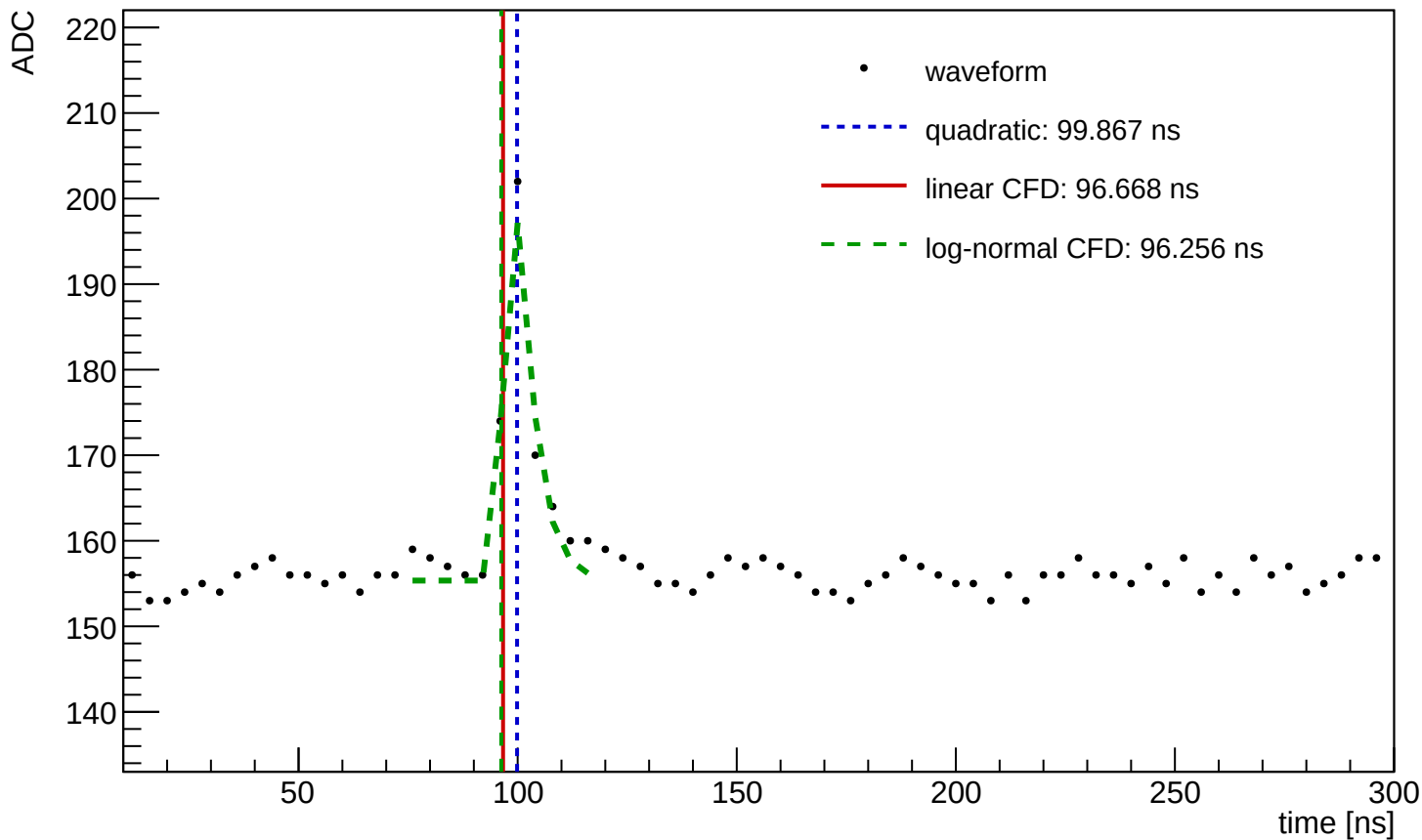
Waveform Time Demo (entry=180, ch=3, module=3001, trigger=SUM)
