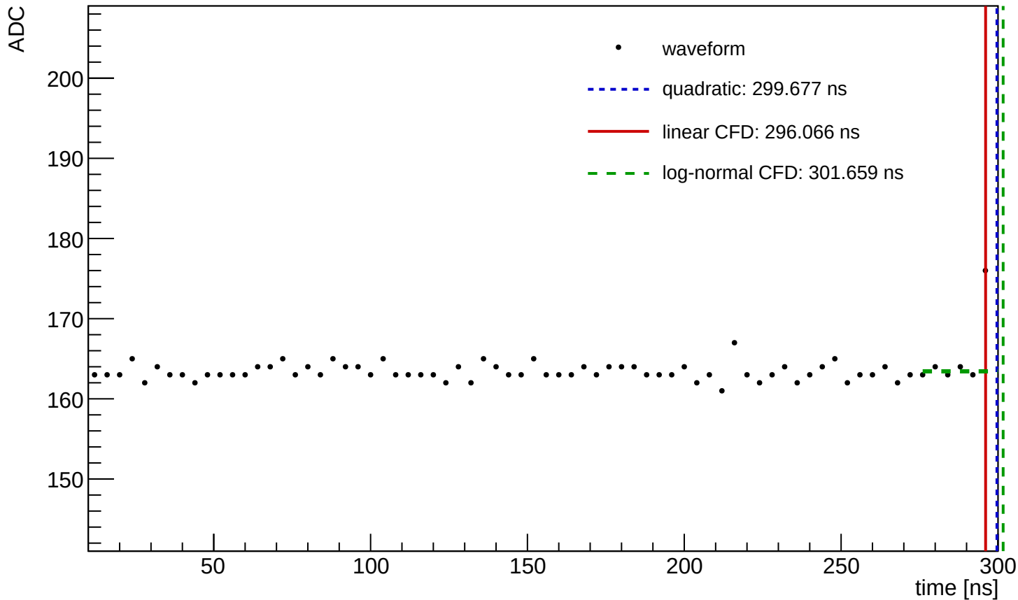
Waveform Time Demo (entry=1566, ch=2, module=3002, trigger=SUM)
