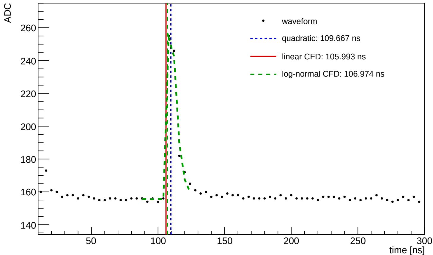
Waveform Time Demo (entry=2795, ch=0, module=3001, trigger=SUM)
