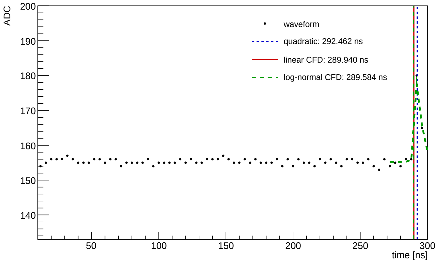
Waveform Time Demo (entry=1884, ch=5, module=3001, trigger=SUM)
