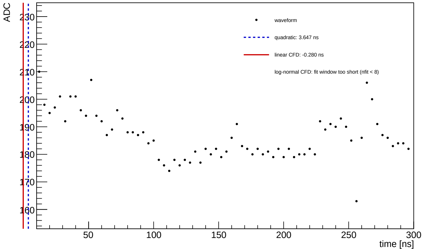
Waveform Time Demo (entry=307, ch=5, module=3003, trigger=SUM)
