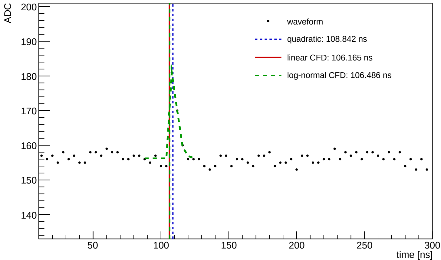
Waveform Time Demo (entry=1236, ch=5, module=3001, trigger=SUM)
