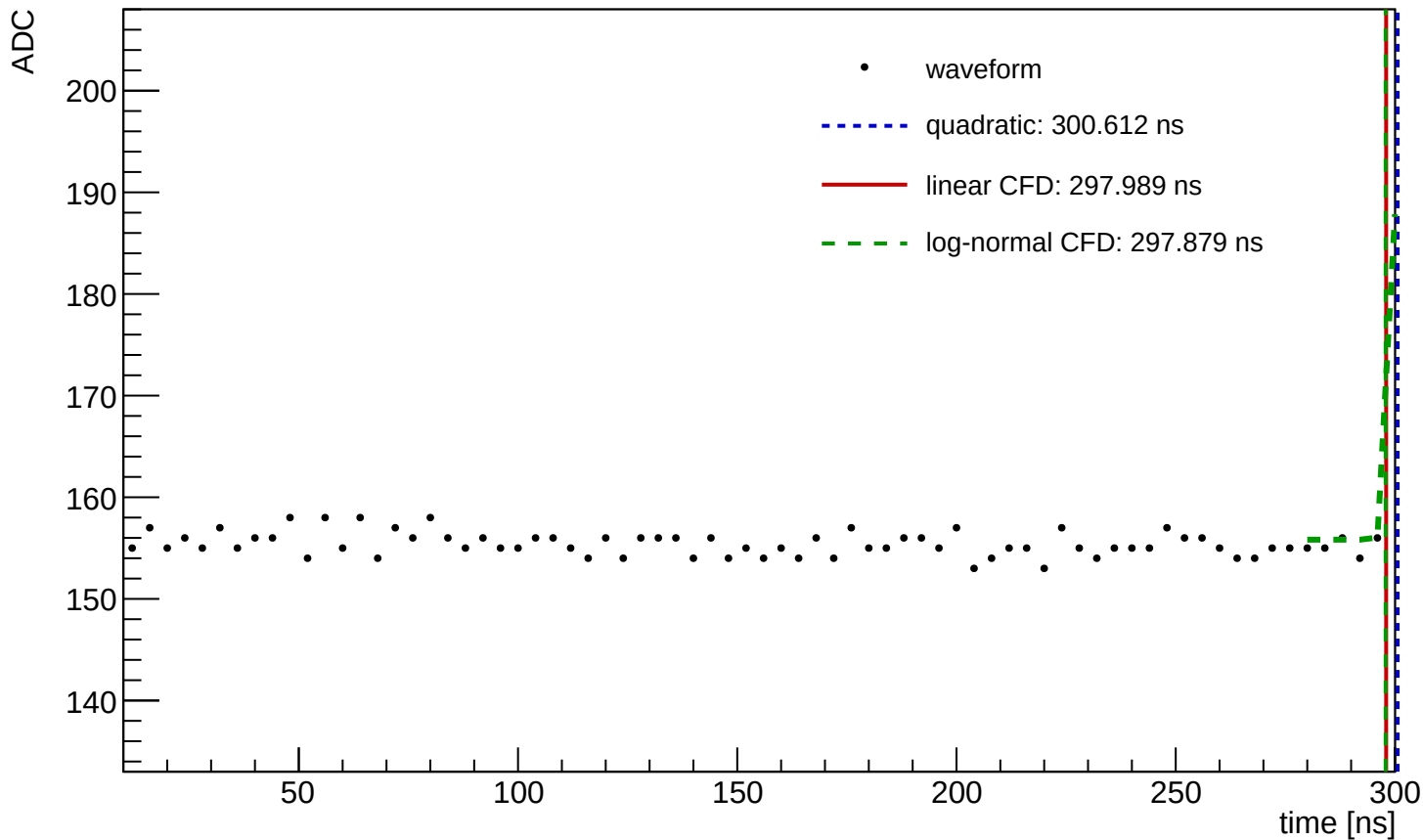
Waveform Time Demo (entry=1135, ch=8, module=3001, trigger=SUM)
