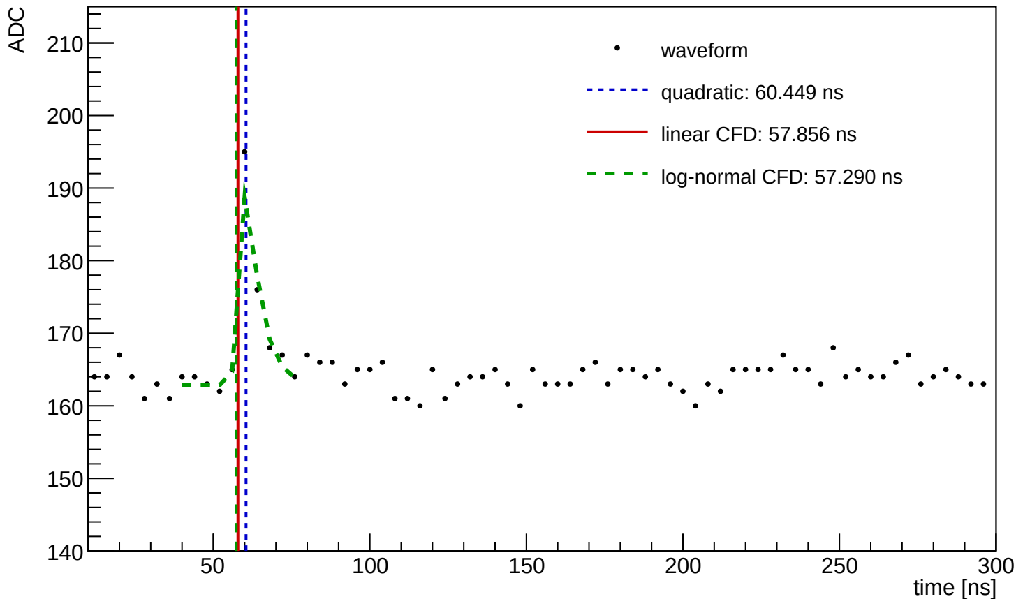
Waveform Time Demo (entry=840, ch=1, module=3002, trigger=SUM)
