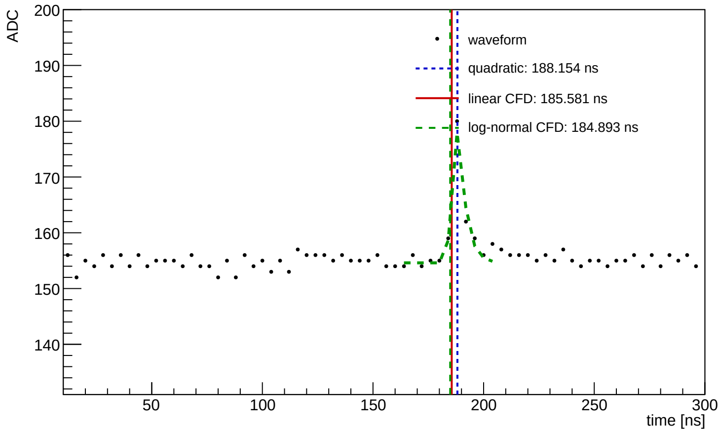
Waveform Time Demo (entry=2345, ch=1, module=3001, trigger=SUM)
