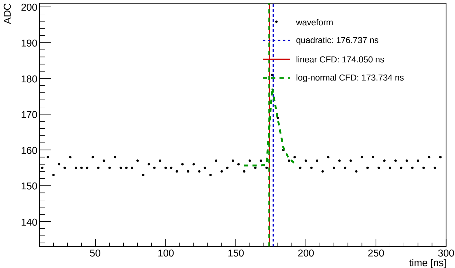
Waveform Time Demo (entry=1398, ch=1, module=3001, trigger=SUM)
