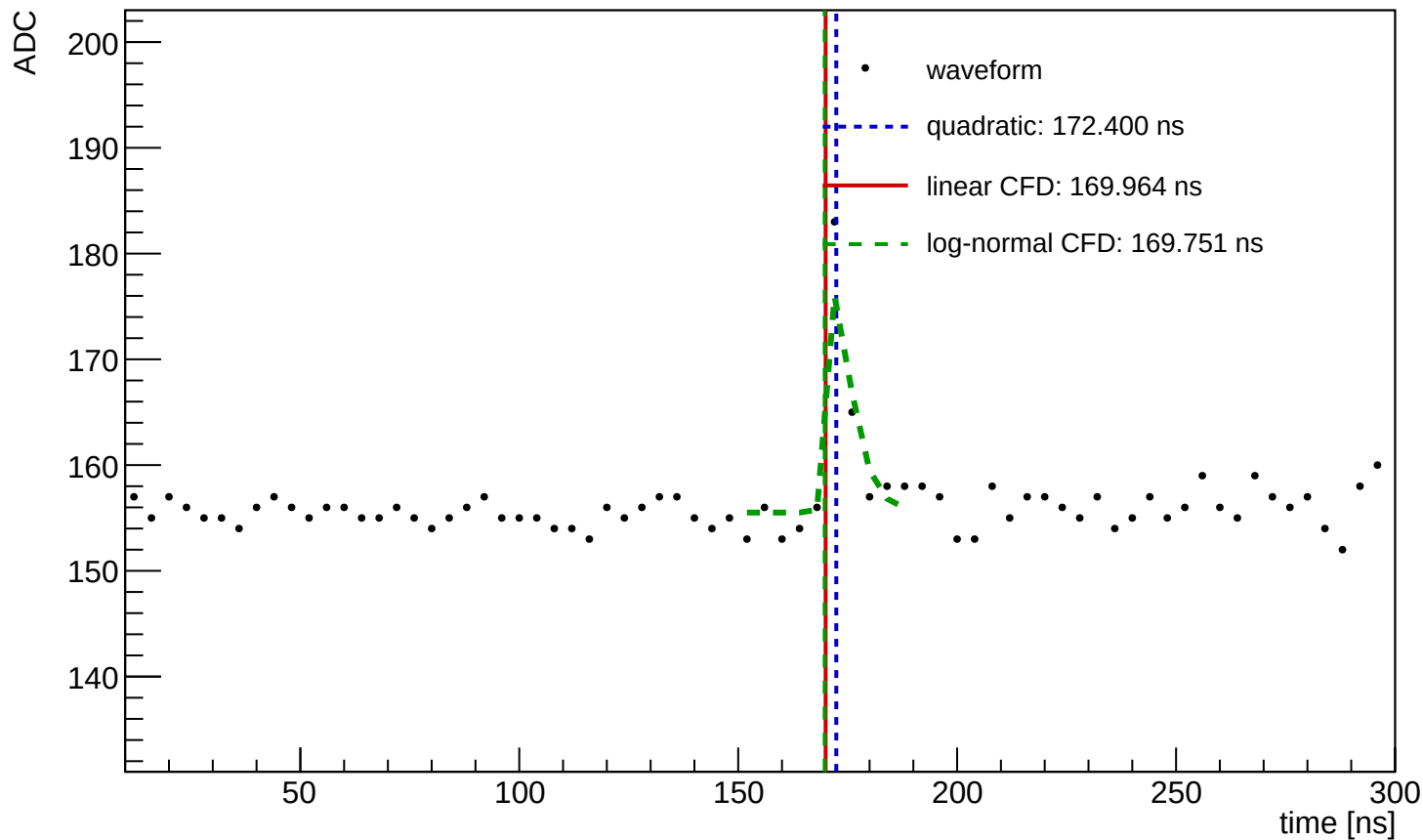
Waveform Time Demo (entry=2754, ch=6, module=3001, trigger=SUM)
