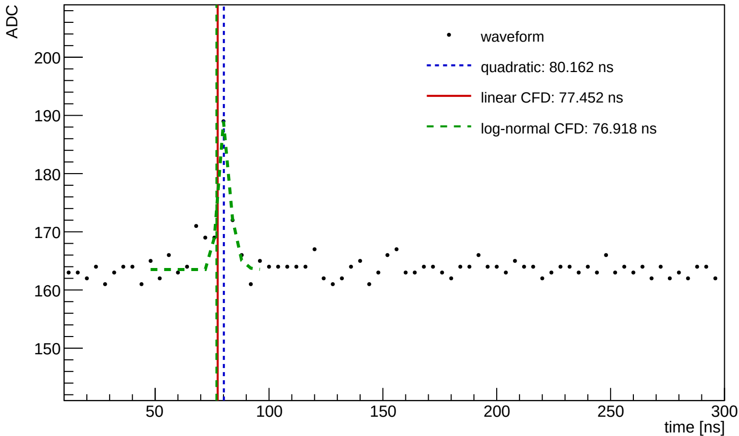
Waveform Time Demo (entry=1863, ch=2, module=3002, trigger=SUM)
