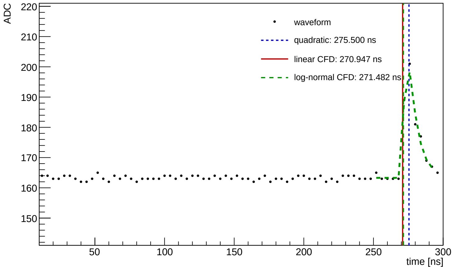
Waveform Time Demo (entry=1643, ch=3, module=3002, trigger=SUM)
