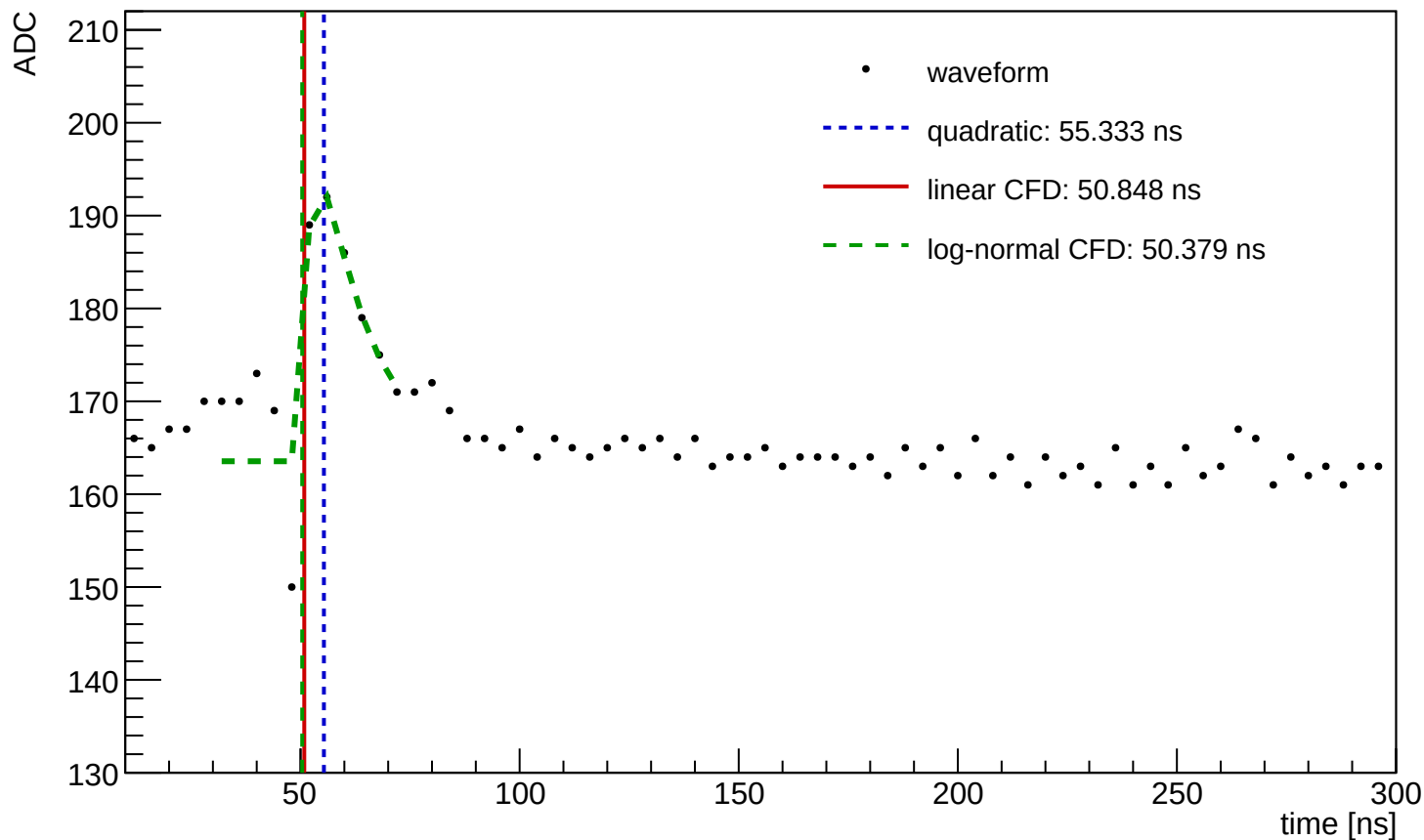
Waveform Time Demo (entry=1568, ch=0, module=3002, trigger=SUM)
