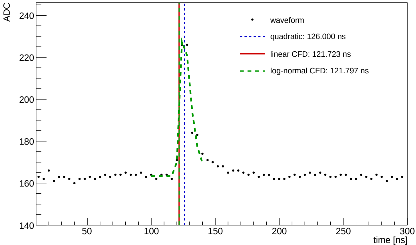
Waveform Time Demo (entry=3041, ch=7, module=3002, trigger=SUM)
