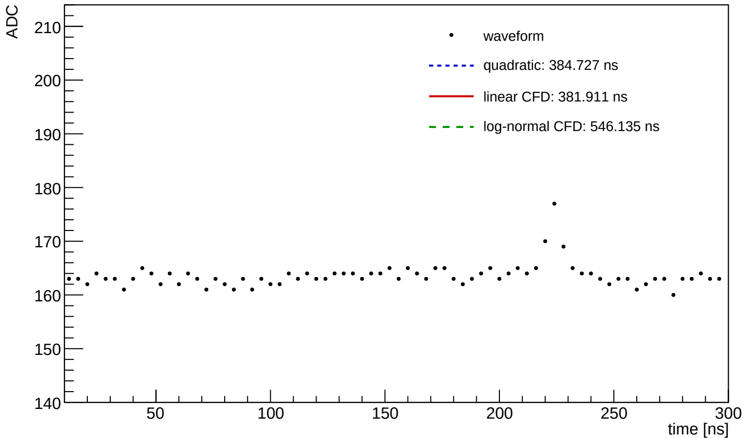
Waveform Time Demo (entry=3040, ch=0, module=3002, trigger=SUM)
