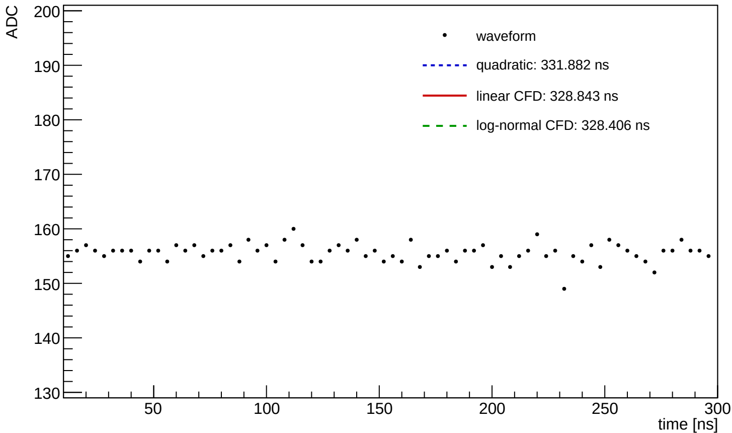
Waveform Time Demo (entry=1652, ch=0, module=3001, trigger=SUM)
