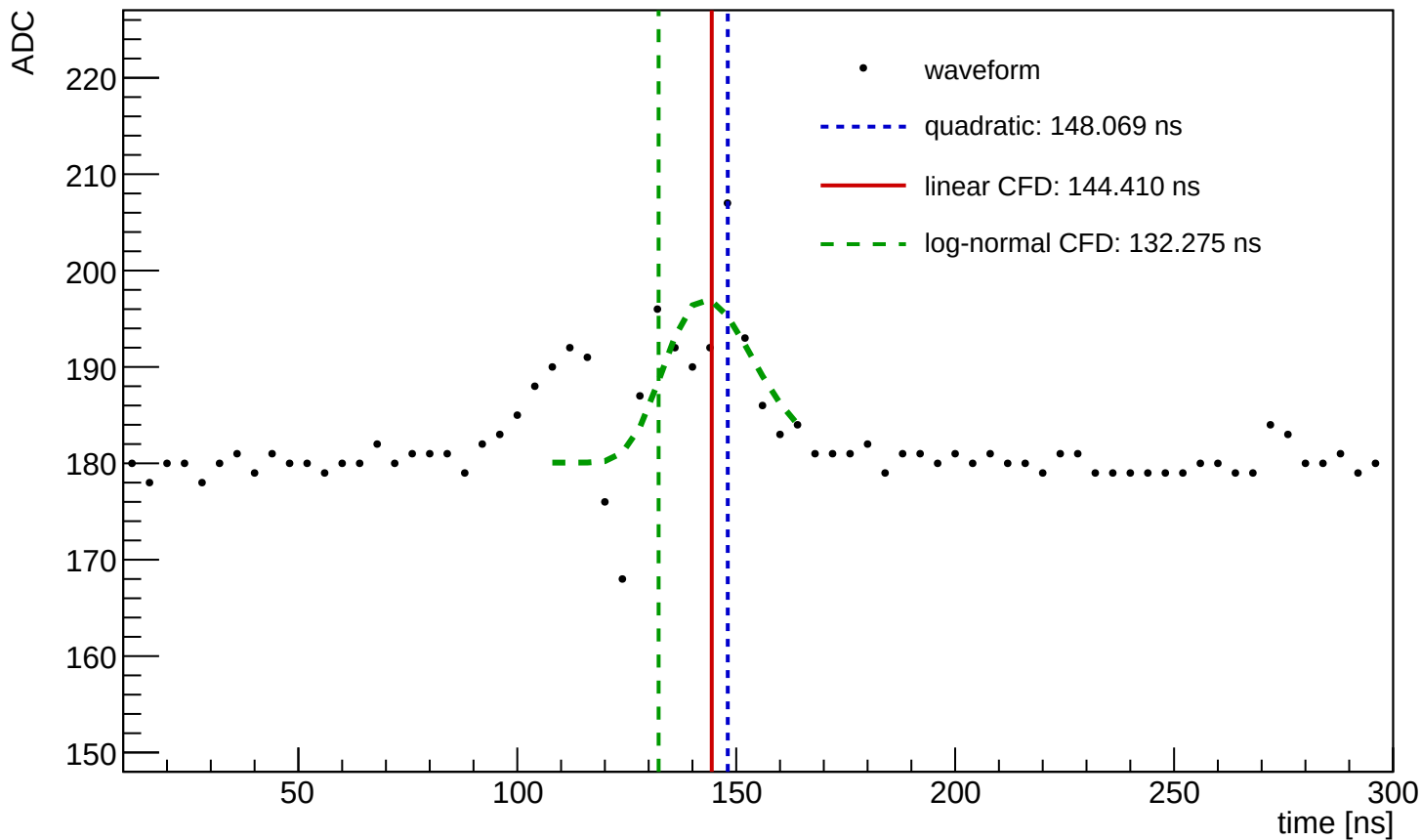
Waveform Time Demo (entry=2580, ch=4, module=3003, trigger=SUM)
