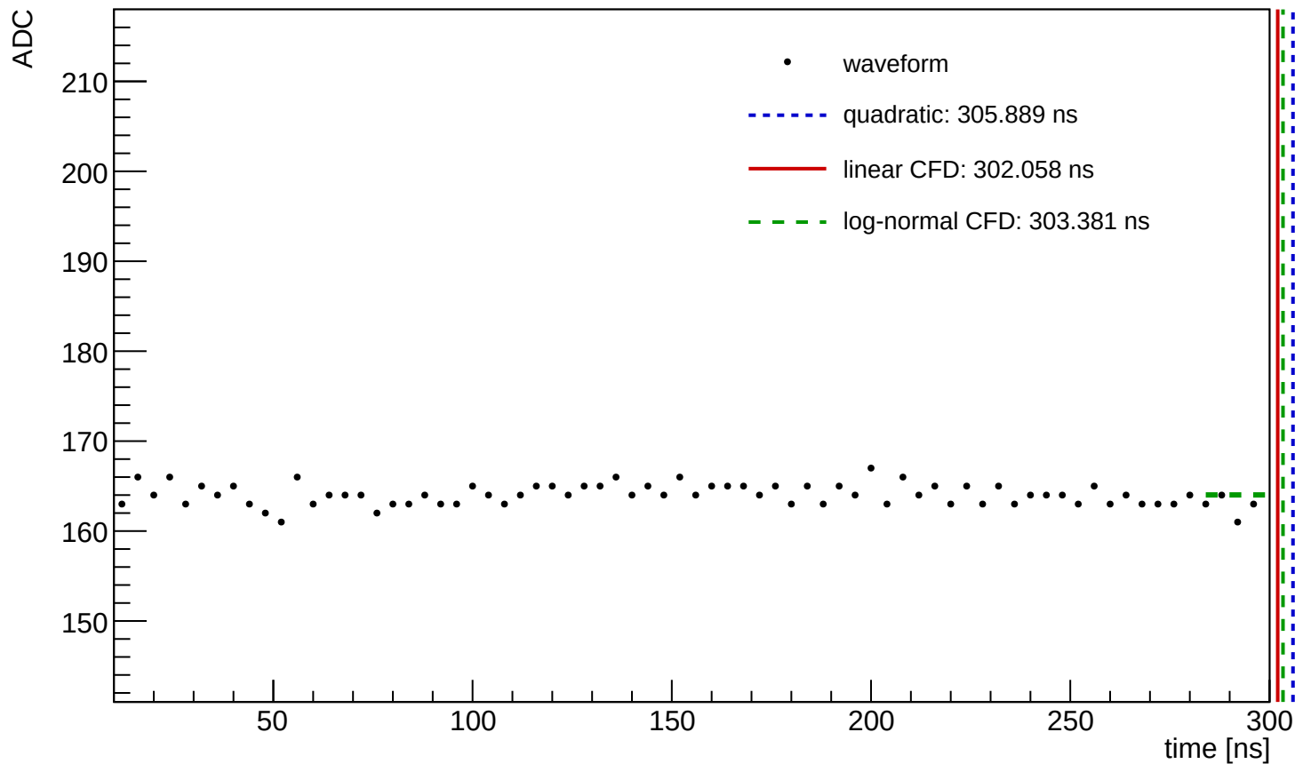
Waveform Time Demo (entry=2003, ch=5, module=3002, trigger=SUM)
