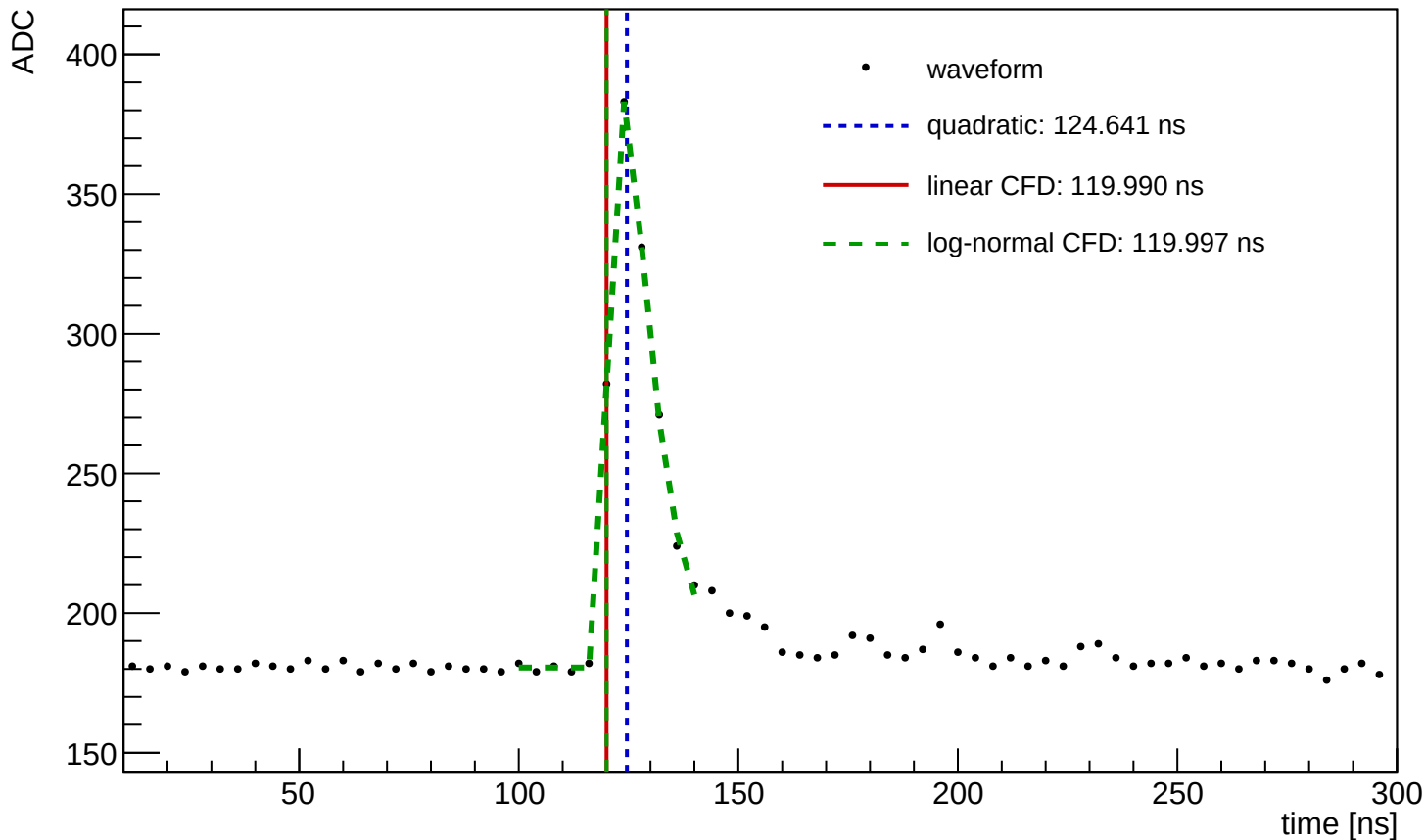
Waveform Time Demo (entry=2510, ch=1, module=3003, trigger=SUM)
