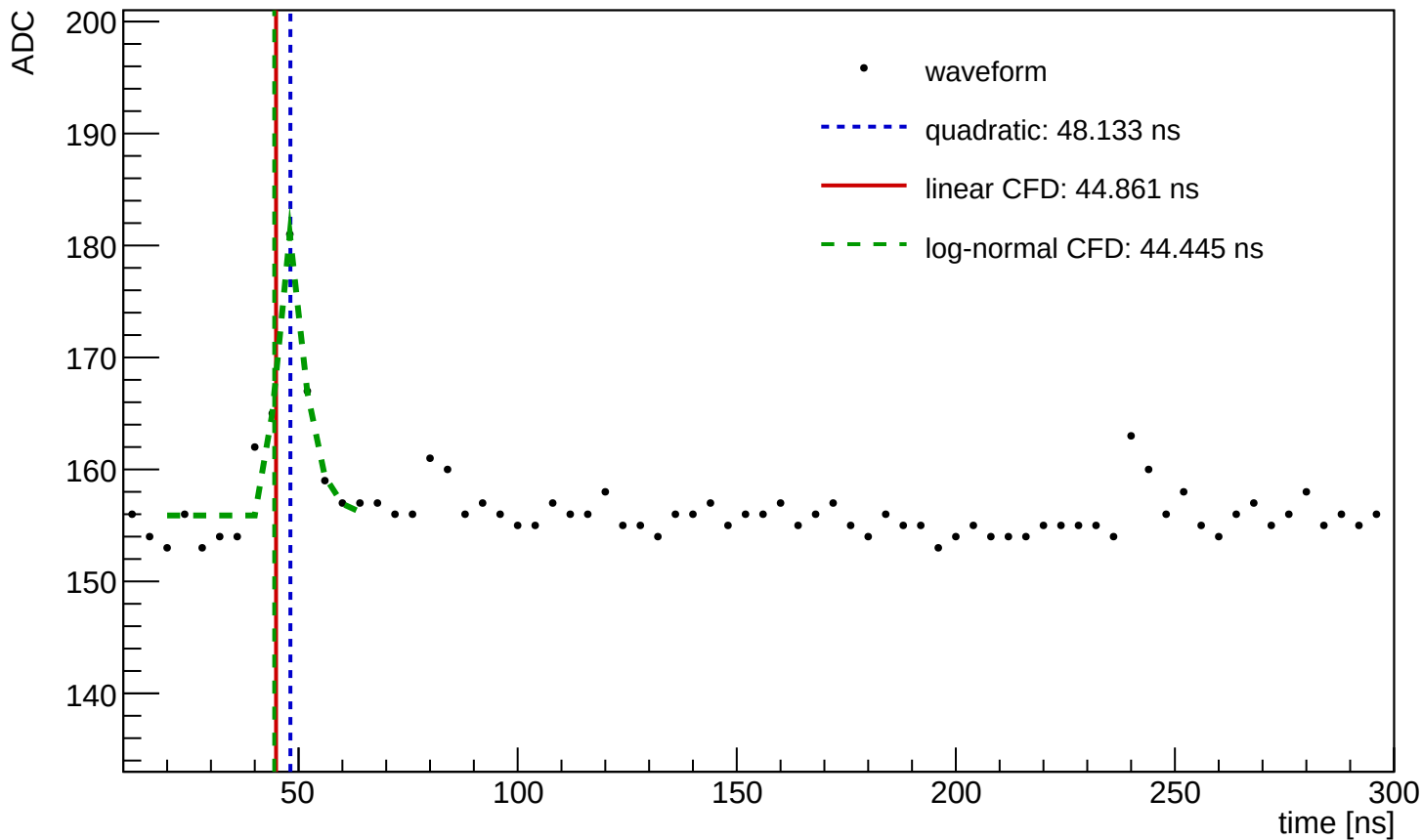
Waveform Time Demo (entry=538, ch=1, module=3001, trigger=SUM)
