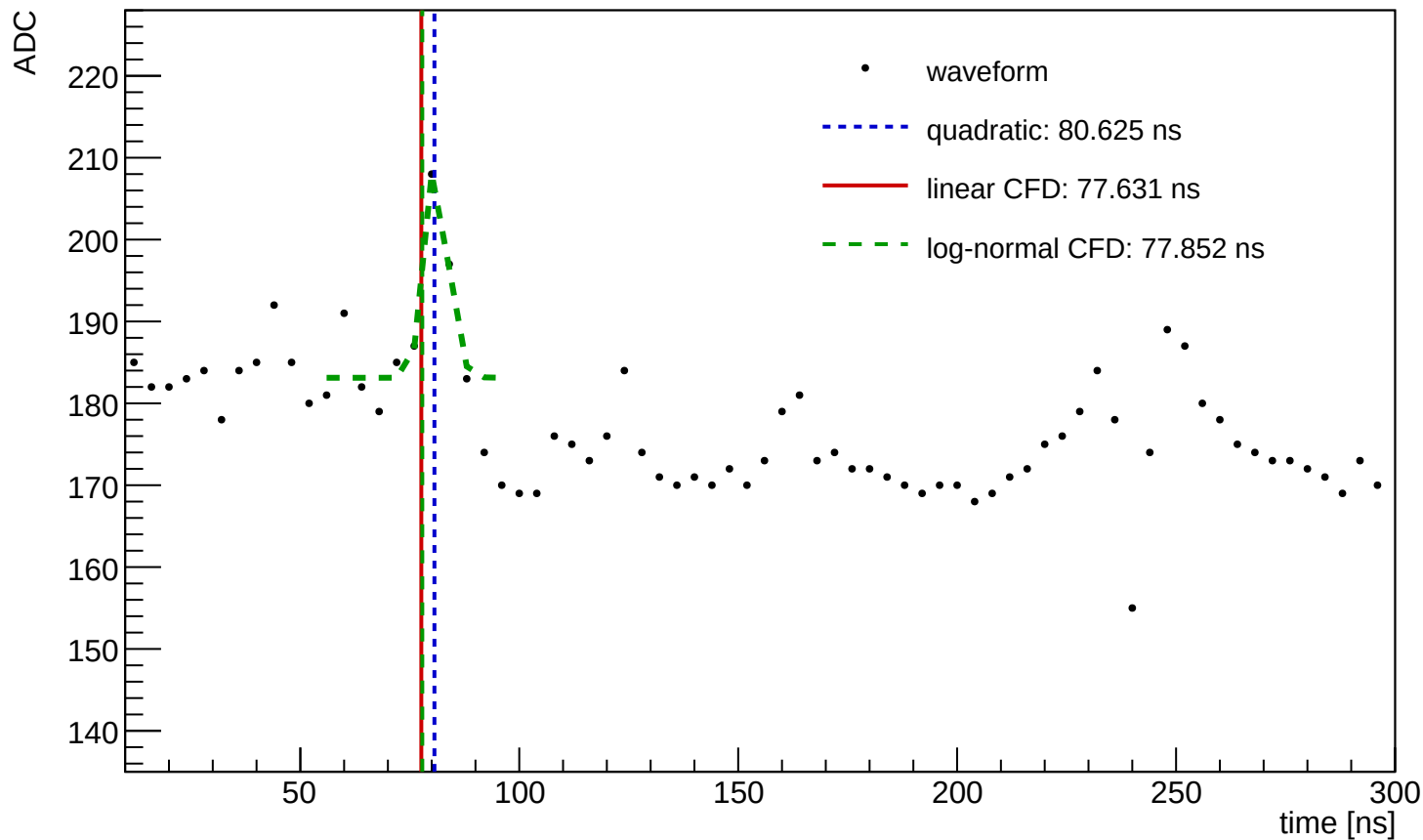
Waveform Time Demo (entry=3048, ch=1, module=3004, trigger=SUM)
