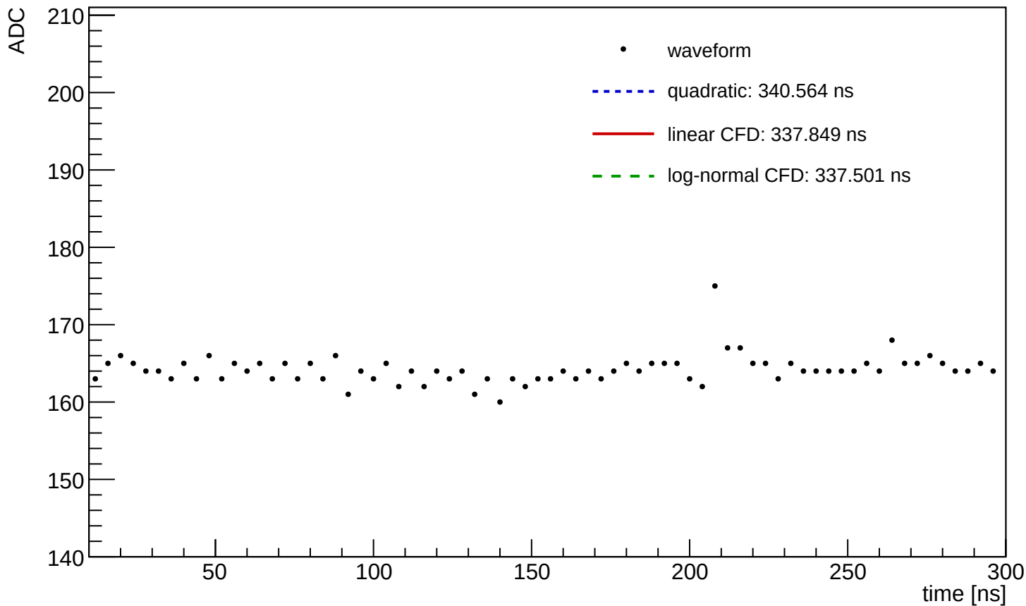
Waveform Time Demo (entry=2105, ch=0, module=3002, trigger=SUM)
