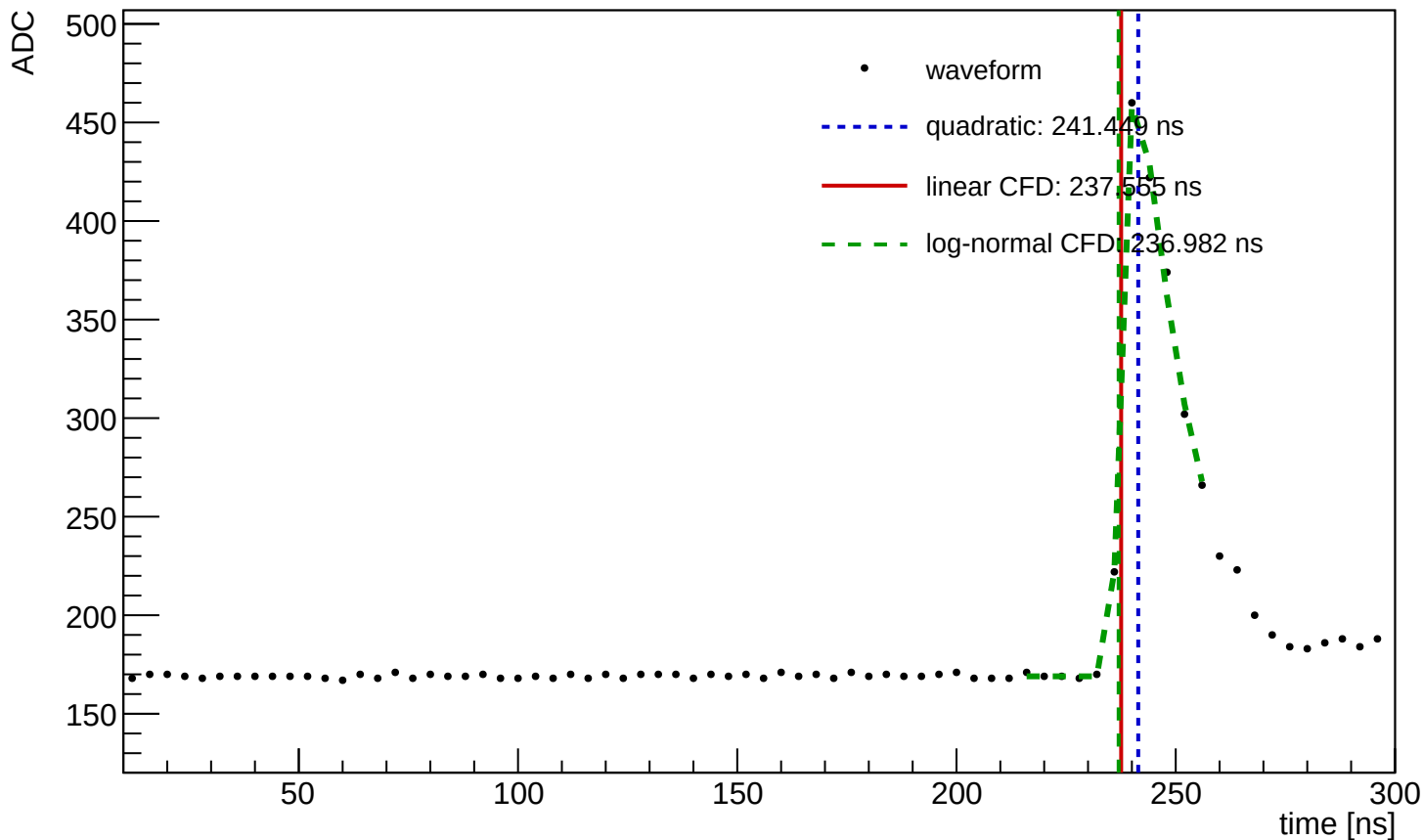
Waveform Time Demo (entry=2452, ch=3, module=3004, trigger=SUM)
