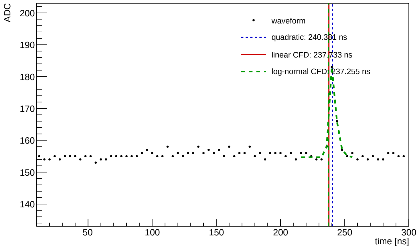
Waveform Time Demo (entry=1406, ch=0, module=3001, trigger=SUM)
