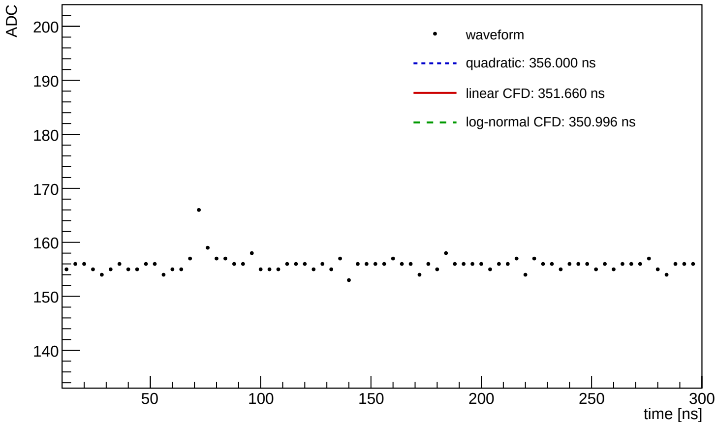
Waveform Time Demo (entry=2874, ch=0, module=3001, trigger=SUM)
