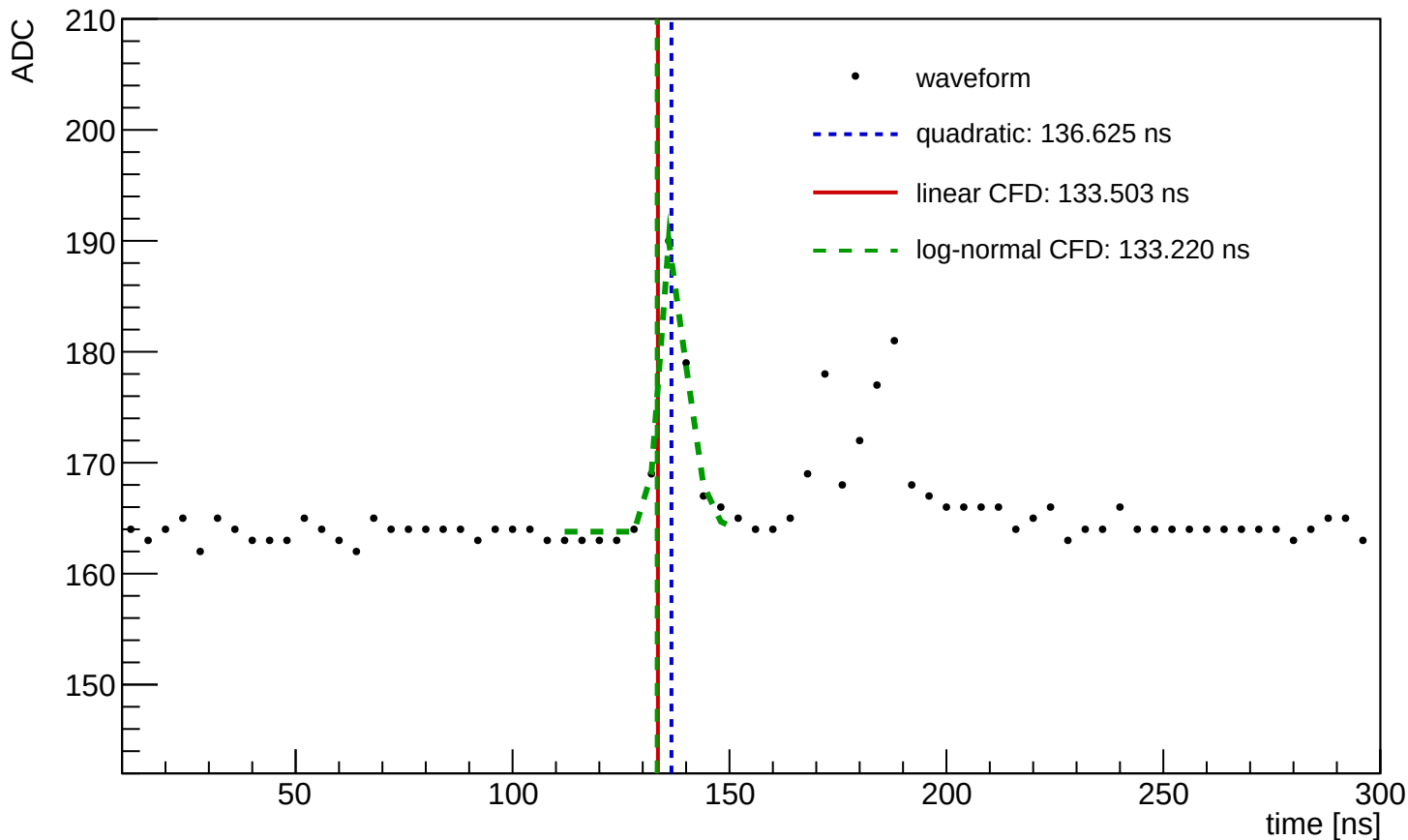
Waveform Time Demo (entry=846, ch=0, module=3002, trigger=SUM)
