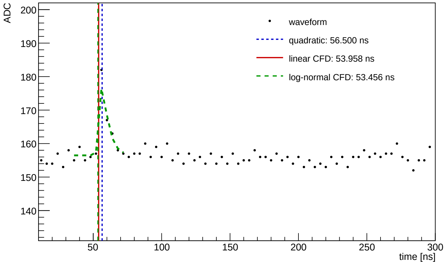
Waveform Time Demo (entry=105, ch=0, module=3001, trigger=SUM)
