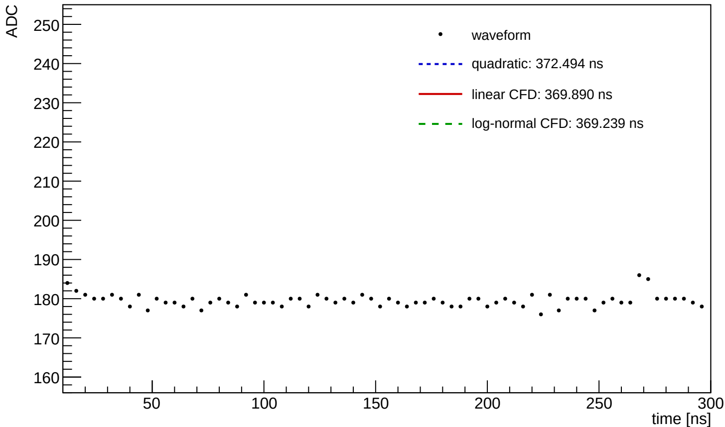
Waveform Time Demo (entry=2785, ch=0, module=3003, trigger=SUM)
