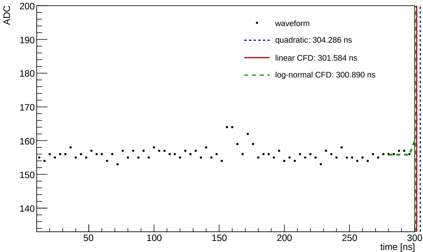
Waveform Time Demo (entry=2057, ch=2, module=3001, trigger=SUM)
