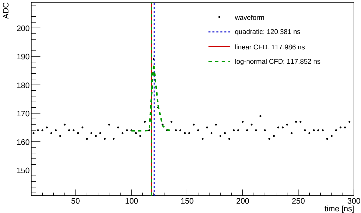
Waveform Time Demo (entry=1280, ch=0, module=3002, trigger=SUM)
