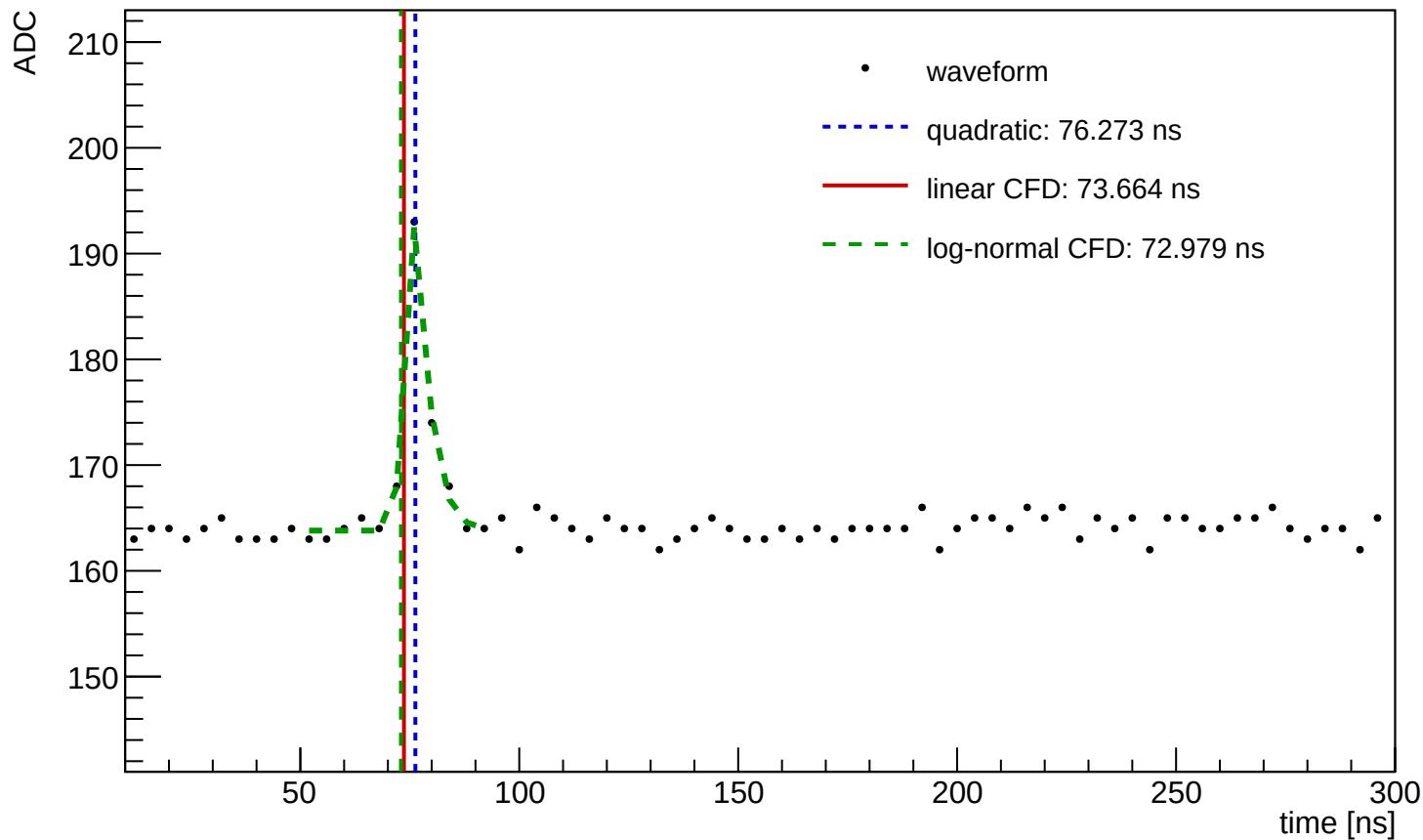
Waveform Time Demo (entry=2847, ch=6, module=3002, trigger=SUM)
