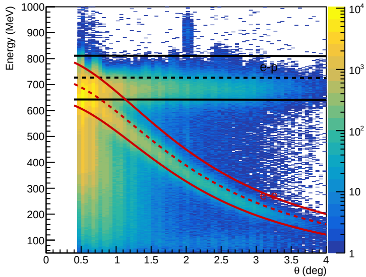
0.7 GeV Reconstructed Energy vs. Angle
