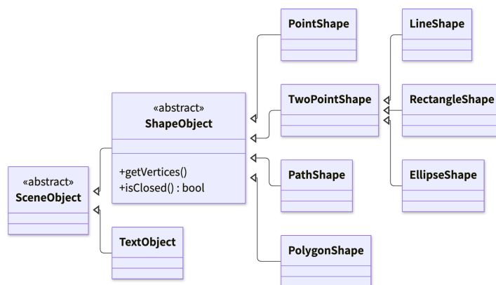
Figure 20: Scene 物件的類別圖
