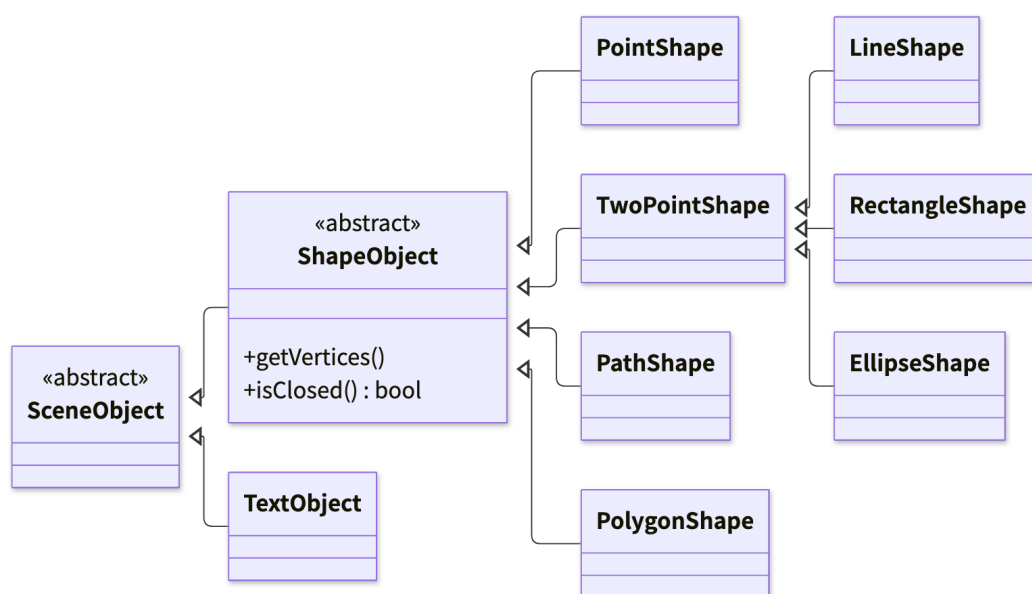
Figure 20: Scene 物件的類別圖
