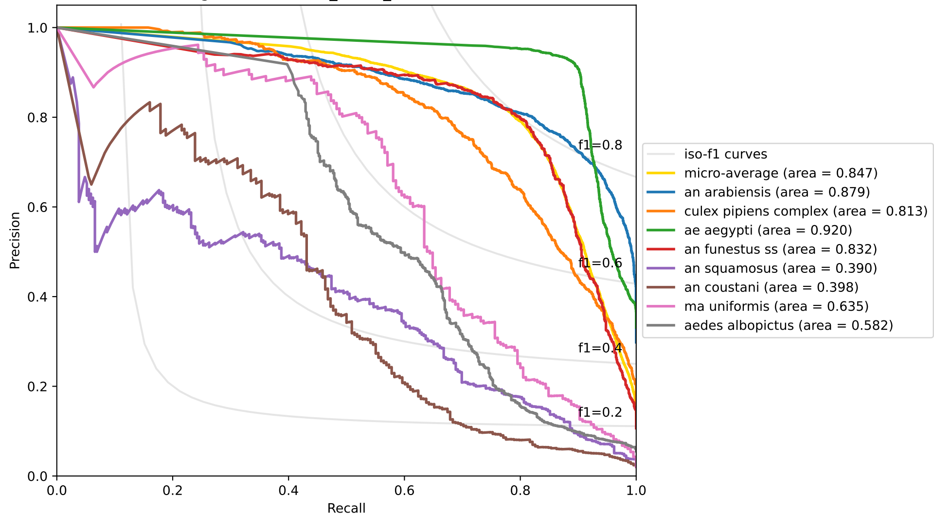
Average Precision / PR_Curve_AUC micro: 0.8465
