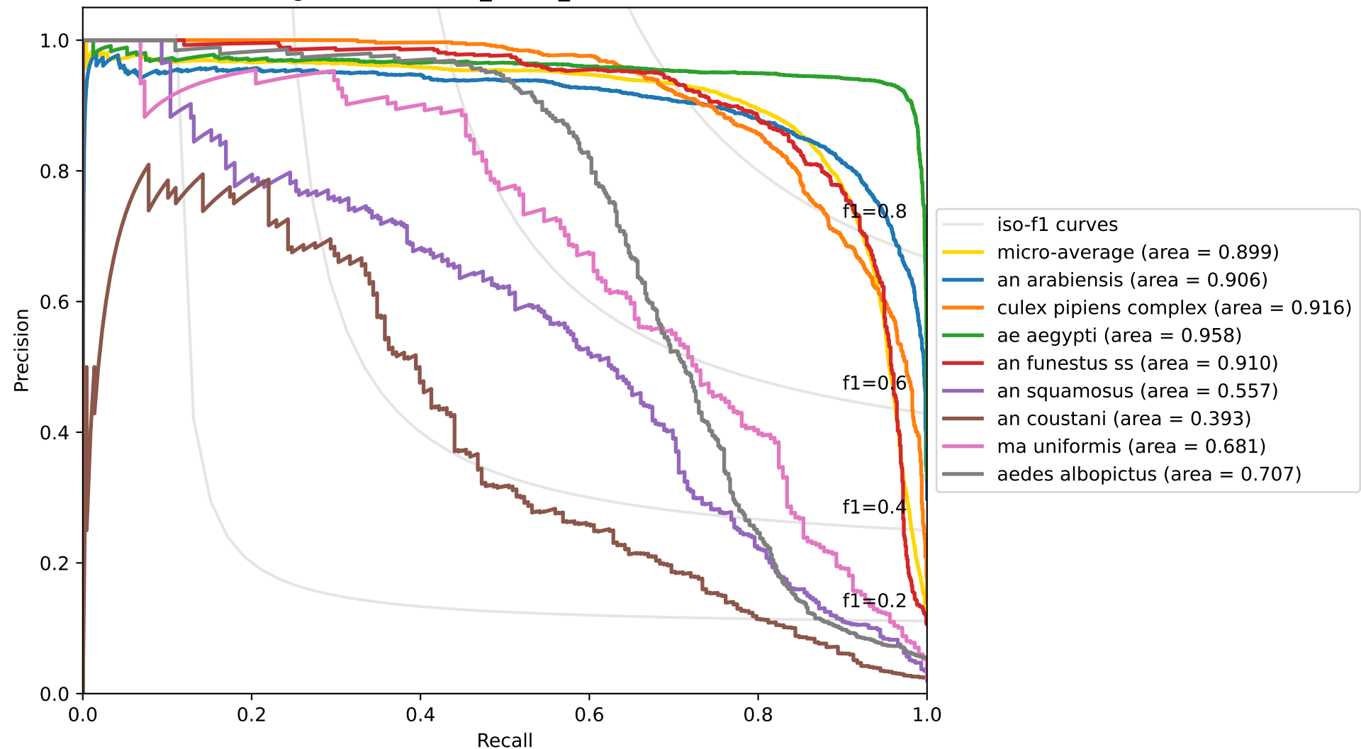
Average Precision / PR_Curve_AUC micro: 0.8992
