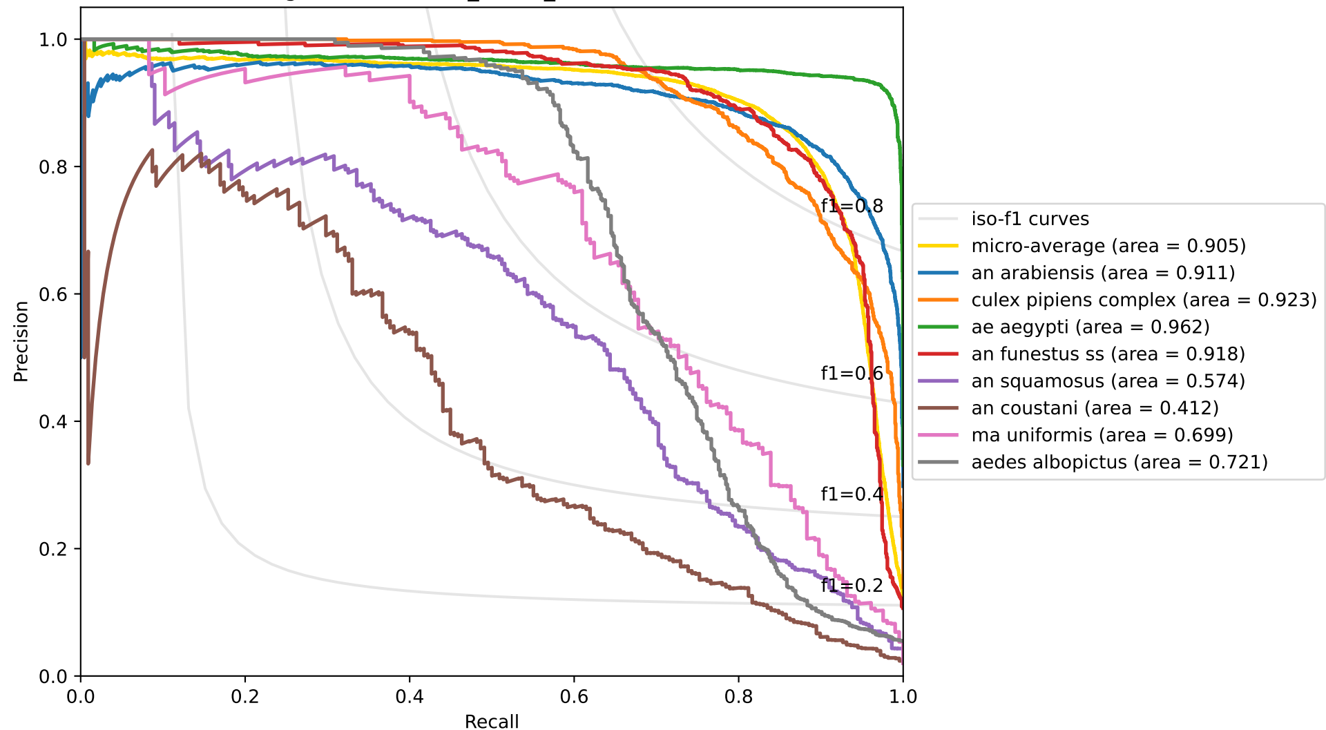
Average Precision / PR_Curve_AUC micro: 0.9050
