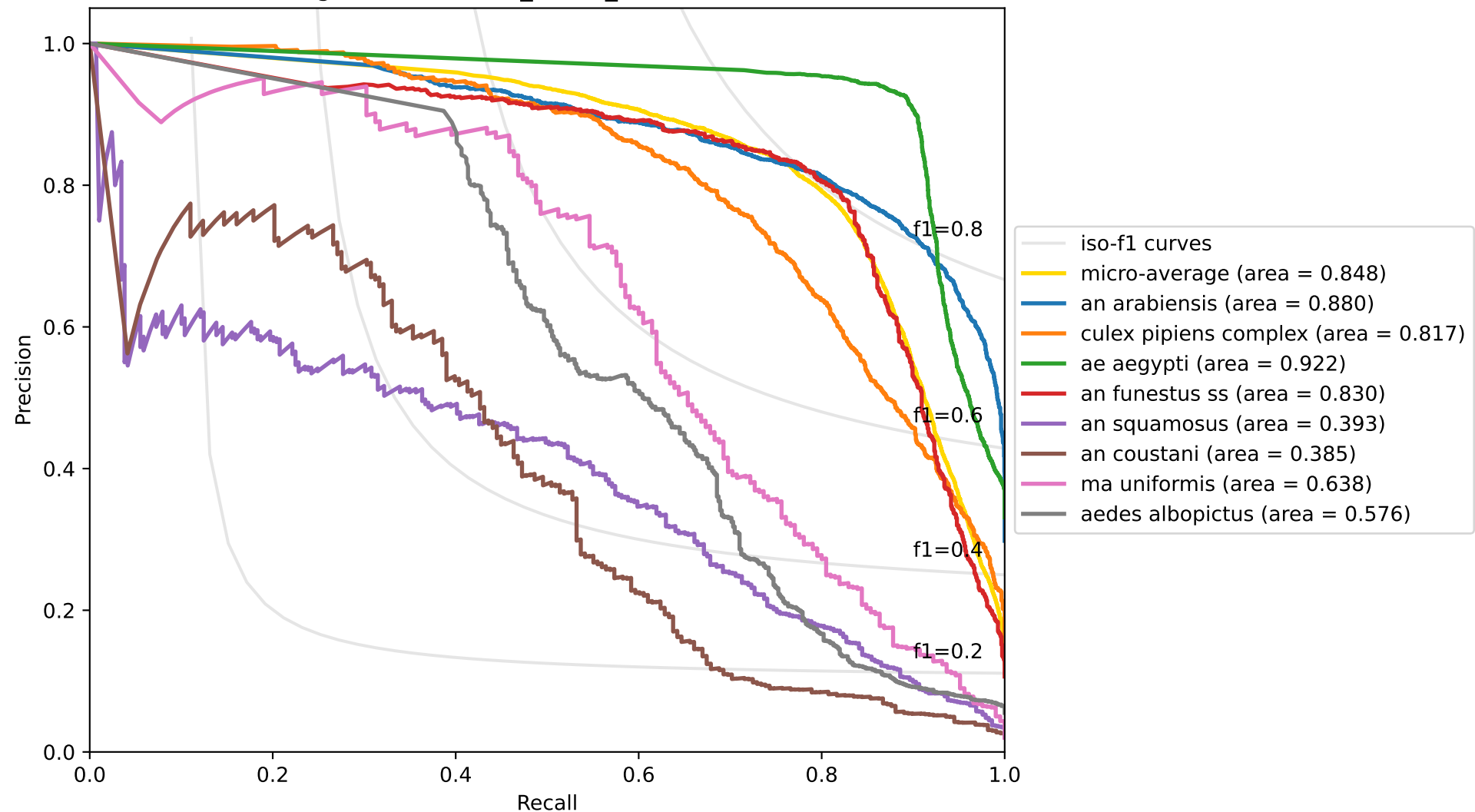
Average Precision / PR_Curve_AUC micro: 0.8481
