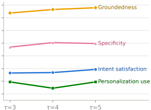
Final-answer quality
