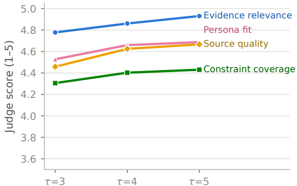
Retrieval quality
