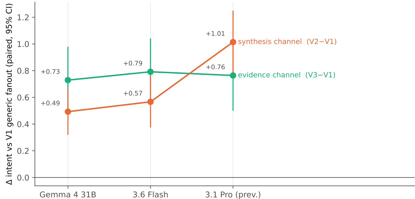
Evidence channel is model-invariant; synthesis channel scales with capability
