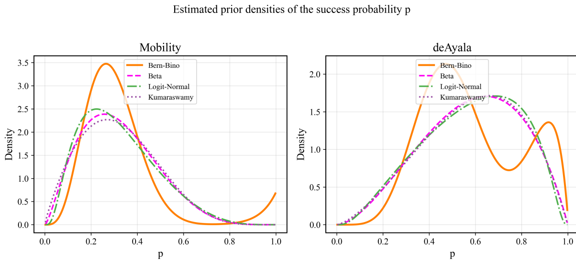
Figure 9: Estimated prior densities \pi(p) of the success probability under the four prior-based models for the two datasets.
