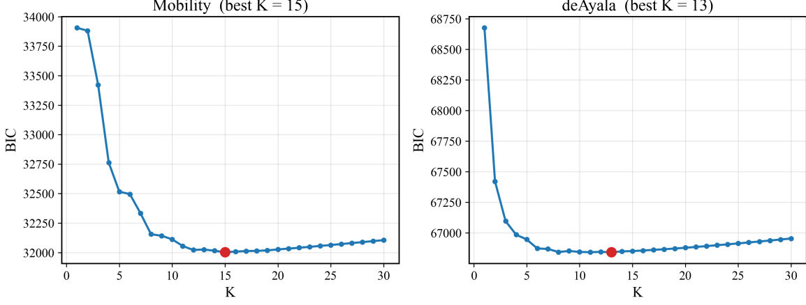
Figure 10: BIC curves for selecting the Bernstein degree K ; the red points mark the minima ( K = 15 and K = 13 ).
