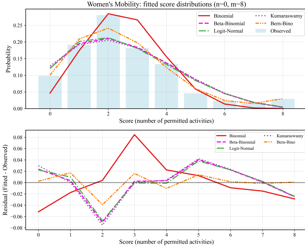
Figure 7: Women’s Mobility data: (upper) observed score distribution and fitted pmfs of the five models; (lower) corresponding residuals.
