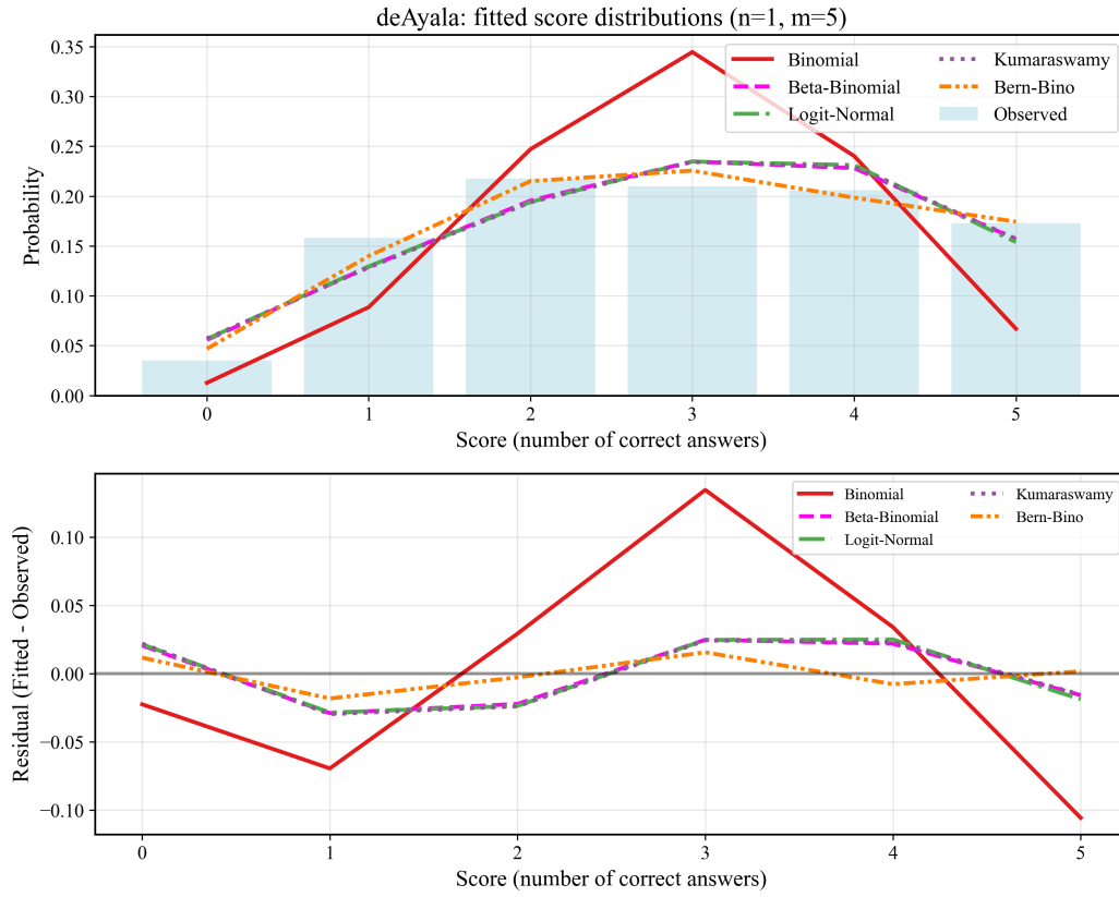
Figure 8: de Ayala mathematics test data: (upper) observed score distribution and fitted pmfs of the five models; (lower) corresponding residuals.
