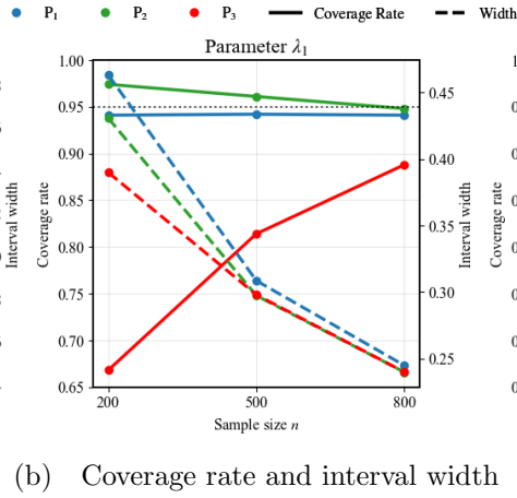
Figure 4: Performance indicators versus sample size under different priors for S_1 .
