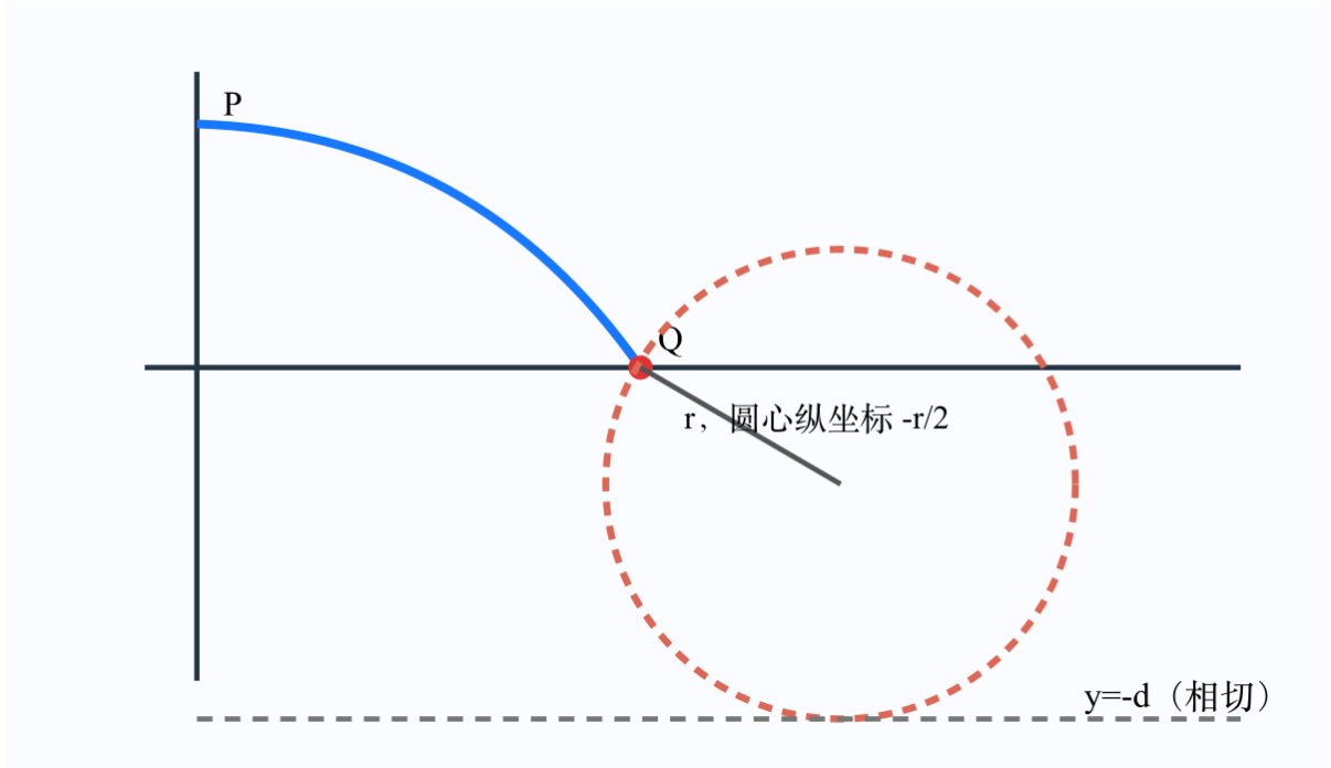
Figure 2: 电场抛物线与磁场相切轨迹
